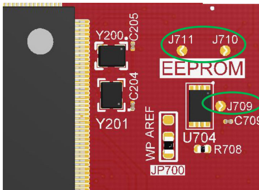
Figure 2-10. Board Location
