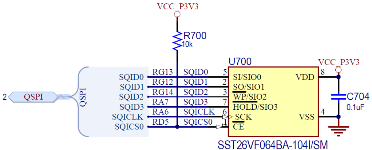
Figure 2-11. Schematic
