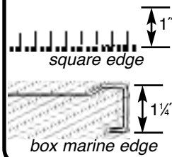
countertop with plywood (shown adjoined to cabinet)
