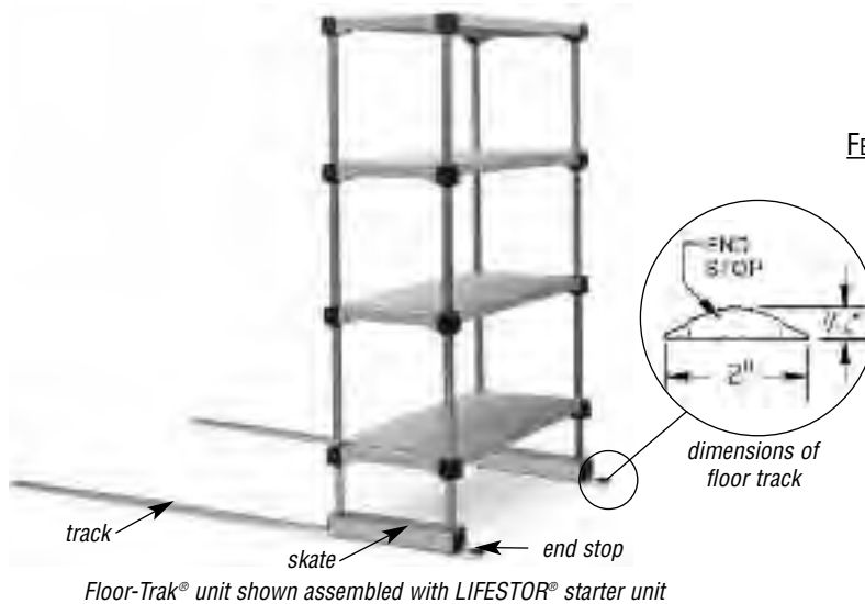
Floor-Trak® unit shown assembled with LIFESTOR® starter unit
