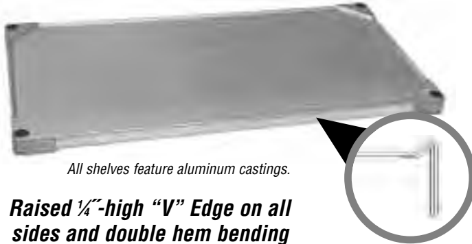
side view of solid shelf, showing raised "V" edge
