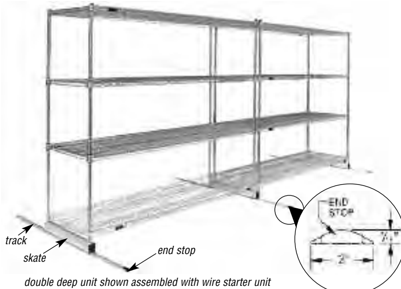
dimensions of floor track
