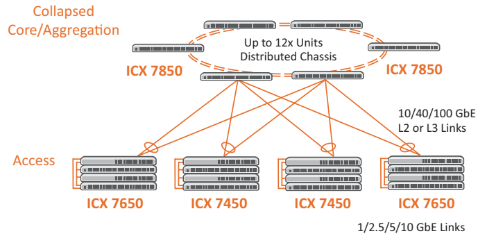
Figure 5: Distributed two-tier campus network.
