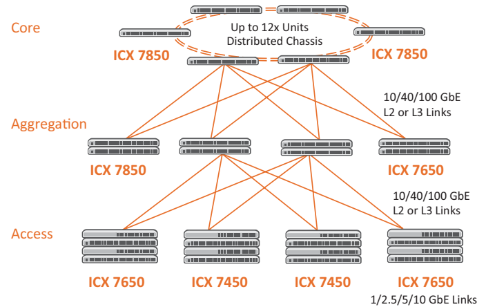
Figure 3: Traditional three-tier campus architecture.
