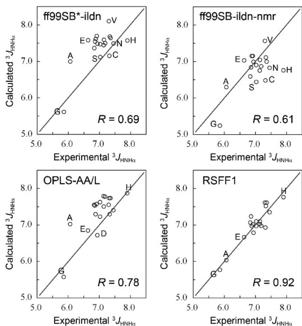
Figure 7. Calculated {}^3J_{\text{HNH}_x} coupling constant in 19 dipeptides plotted against the corresponding experimental data. Each plot shows the results from simulations using each force fields, calculated using a recent (2007) Karplus parameter set.
