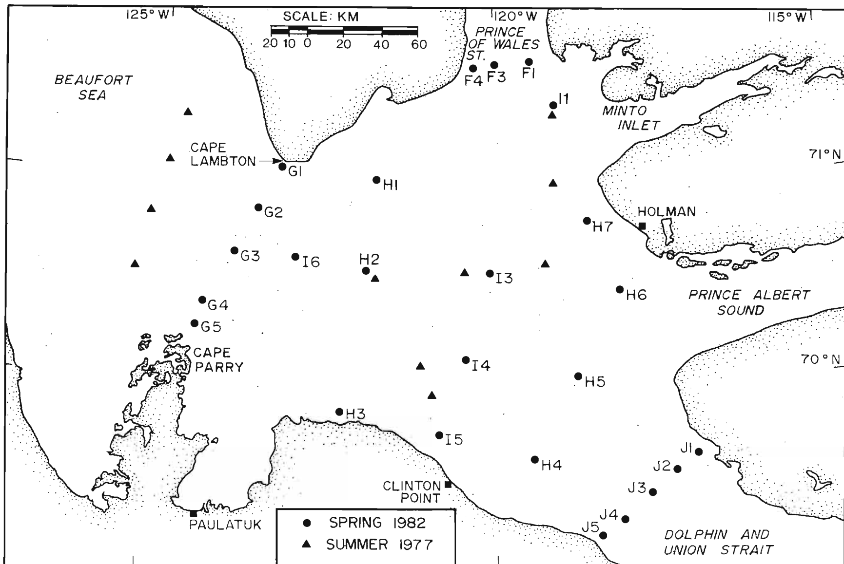
Figure 27: The locations of CTD stations occupied from March 29–April 2, 1982 in Amundsen Gulf. Also shown are locations of bottle cast data collected in the summer of 1977 (Macdonald et al., 1978).
