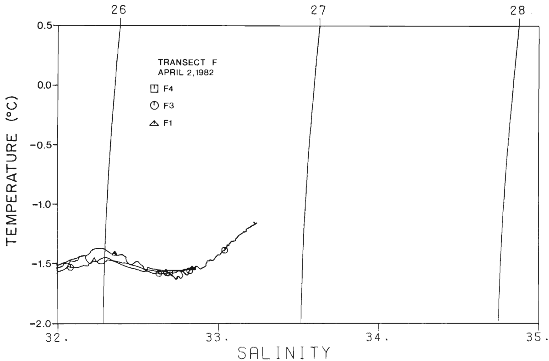
Figure 7: The TS curves of CTD stations of section F, April 2, 1982.
