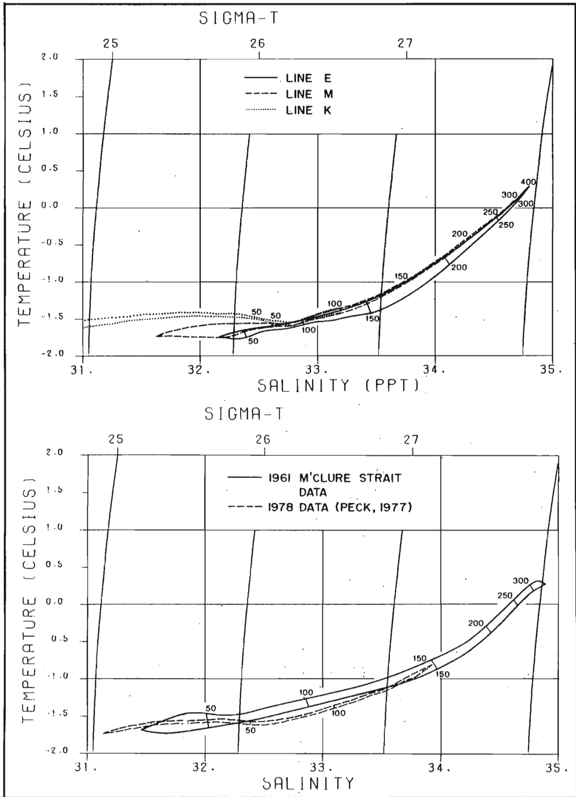
Figure 22: (upper) The envelope enclosing TS curves of lines E (M'Clure Strait), M (northern M'Clintock Channel) and K (southern M'Clintock Channel). (lower) The envelope enclosed TS curves of bottle data obtained in M'Clure Strait in 1961 and CTD data obtained in northern M'Clintock Channel in 1978.
