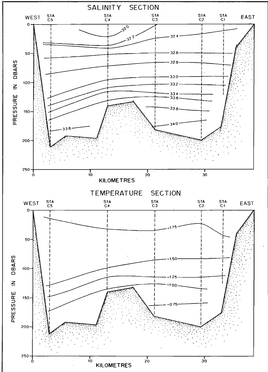
Figure 16: Vertical sections of temperature and salinity through line C in Byam Martin Channel, March 26, 1982.
