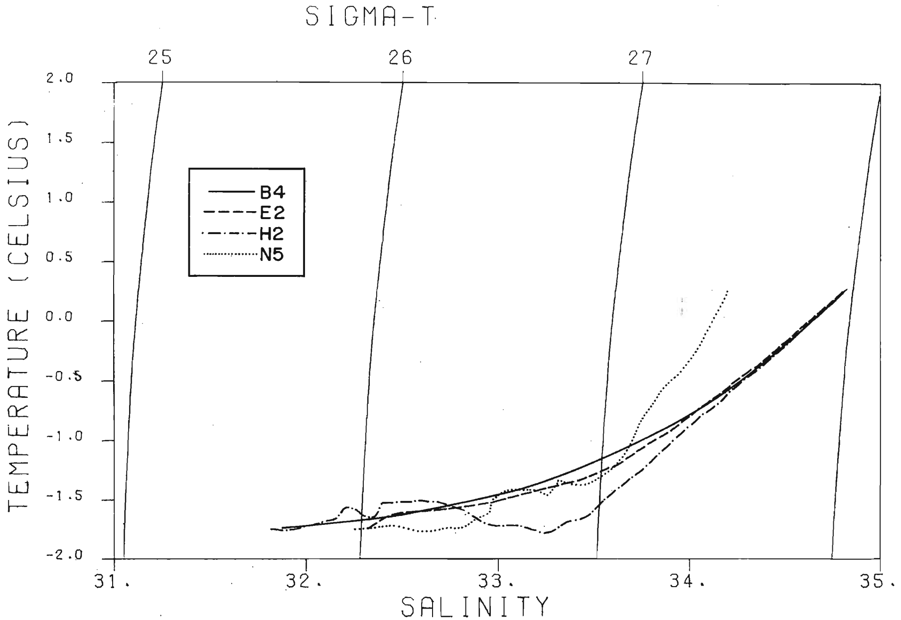
Figure 44: The TS curves of representative stations of the Sverdrup Basin (B4), M'Clure Strait (E2), Amundsen Gulf (H2) and Lancaster Sound (N5).
