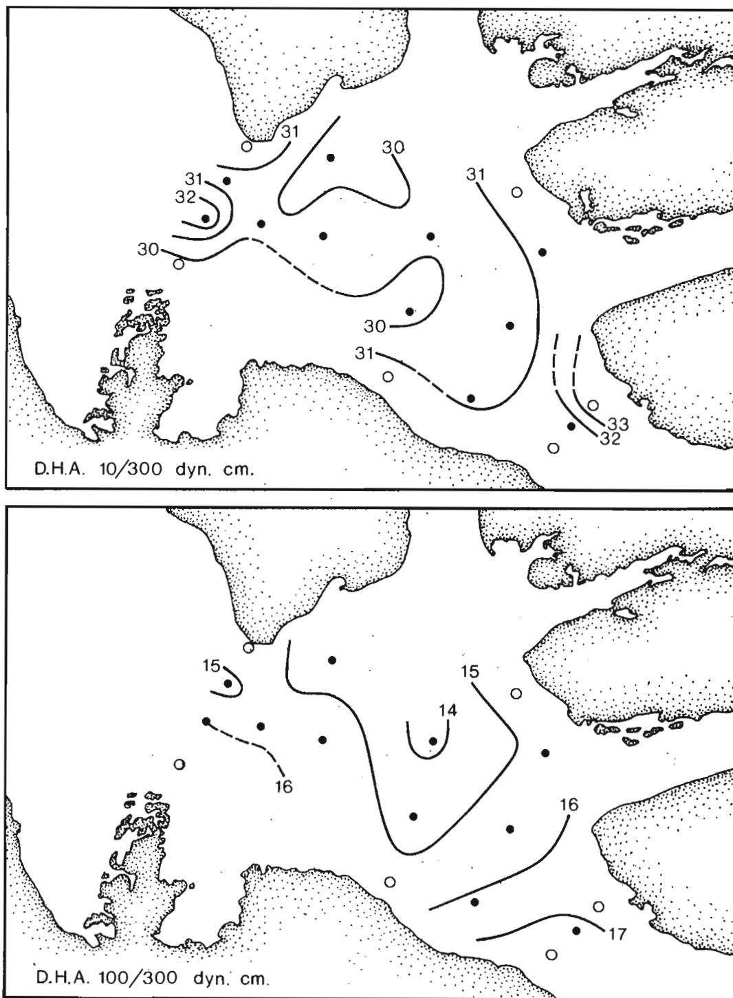
Figure 37: (upper) A map of the dynamic height anomaly in dynamic centimetres in Amundsen Gulf, at 10 dbar relative to 300 dbar, and (lower) at 100 dbar relative to 300 dbar. The data at stations indicated by open circles were extrapolated to 300 dbar.
