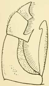
9 muscorum
