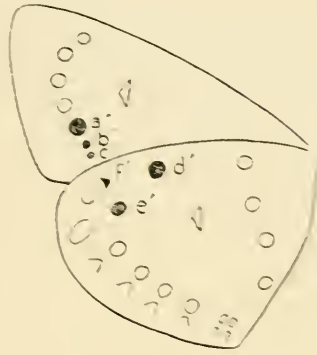
2. thersites
