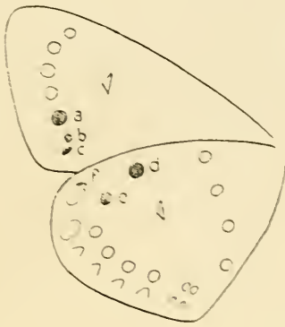
1. icarinus
