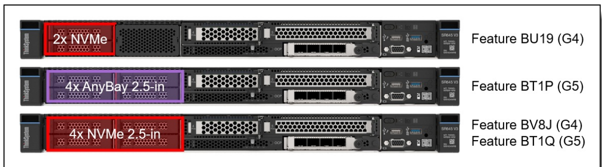
Figure 10. SR645 V3 front drive bay configurations - 2.5-inch drive bays with front PCIe slot support
