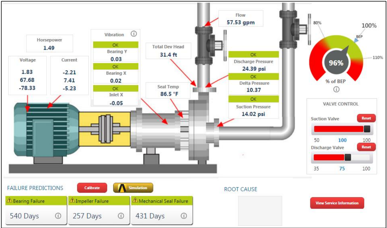
Figure 14. ThingWorx Dashboard showing real-time analytics and predictive maintenance
