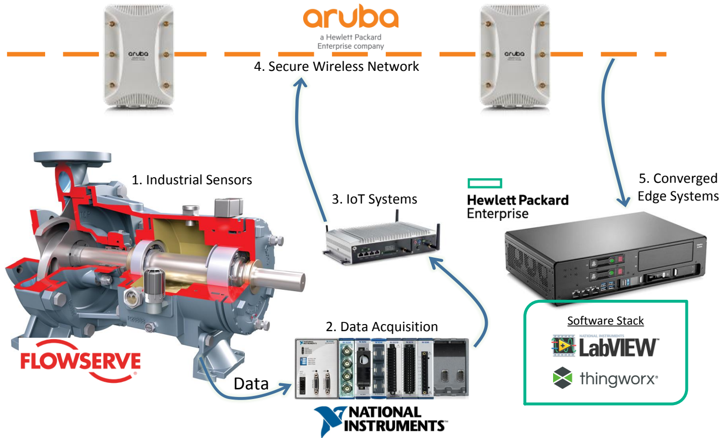
Figure 2 Solution Diagram and Data Path
