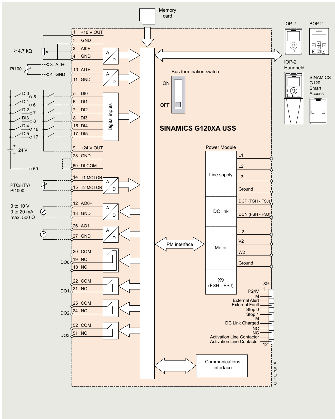
SINAMICS G120XA, version USS, connection diagram
