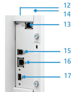
Rear I/O panel close-up
