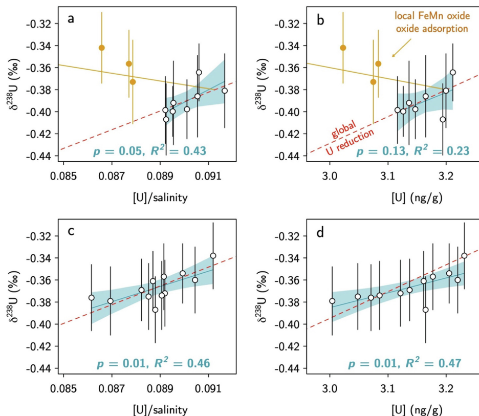
Fig. 8. \delta^{238}\text{U} vs [U]/salinity and [U] in (a,b) North Atlantic and (c,d) South Pacific. In both basins, \delta^{238}\text{U} positively correlates with [U]/salinity and [U] concentration. These positive correlations are depicted as linear regression lines with 95 % confidence intervals shaded ( p and R^2 values reported in each panel). The positive correlation is best explained by the global isotopic impact of U reduction in anoxic sediments with a fractionation of +0.6 ‰ (Andersen et al., 2017; Lau et al., 2019); red dashed lines denote isotopic trend of this removal pathway. In the North Atlantic, anomalous samples that likely show effects of U adsorption to Fe- or Mn- oxides are shown in orange. Solid orange lines in (a) and (b) denote isotopic trend of U removal onto Fe- or Mn- oxides with an isotopic effect of -0.24 ‰ (Goto et al., 2014). (For interpretation of the references to colour in this figure legend, the reader is referred to the web version of this article.)
