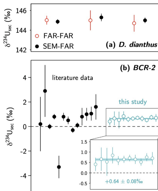
Fig. 5. Accuracy of \delta^{234}\text{U}_{\text{sec}} analyses. SEM = secondary electron multiplier used to measure ^{234}\text{U} ; FAR = Faraday cup used to measure ^{234}\text{U} . Panels denote: (a) comparison of SEM-FAR and FAR-FAR measurements of three D. dianthus specimens from Cruise TN-228, and (b) comparison of measured \delta^{234}\text{U}_{\text{sec}} values for USGS BCR-2 geostandard with literature reports (references in Section 4.3).
