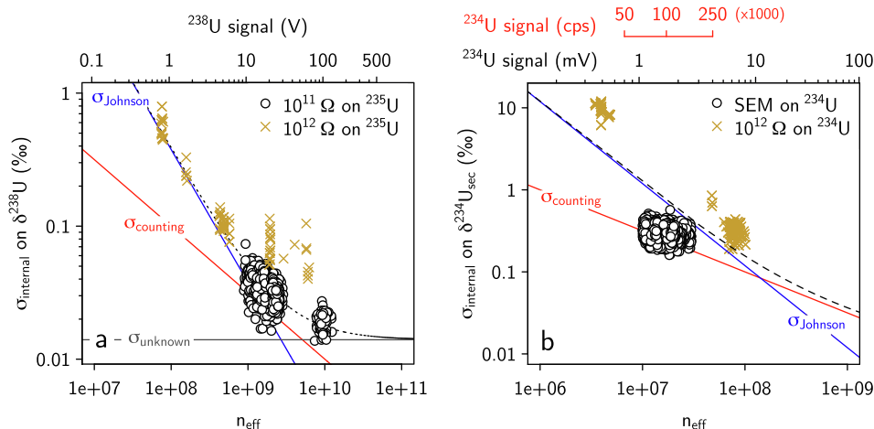
Fig. 3. Limits on internal precision of U isotope analyses. Internal precision on (a) \delta^{238}\text{U} and (b) \delta^{234}\text{U}_{sec} measurements is limited by Johnson noise ( \sigma_{Johnson} ; blue lines) and counting statistics ( \sigma_{counting} ; red lines). All sample data (white circles) plot at the theoretical maximum internal precision (represented by the dashed black curve, which is the sum of the red and blue lines). Standards analyzed with a 10^{12} \Omega amplifier on ^{235}\text{U} show poorer internal precision (gold crosses, panel a). The subset of samples for which ^{234}\text{U} was measured in a Faraday cup (gold crosses, panel b; 10^{12} \Omega amplifier) are limited by both Johnson noise and counting statistics; all other samples for which ^{234}\text{U} was measured in the SEM (white circles) were only limited by counting statistics. Theoretical error from Johnson noise was calculated for a 10^{11} \Omega amplifier on ^{235}\text{U} in panel (a) and 10^{12} \Omega amplifier on ^{234}\text{U} in panel (b); 10^{11} \Omega amplifier was used for ^{238}\text{U} in all calculations. Top x-axes denote signal intensity on ^{238}\text{U} and ^{234}\text{U} in panels (a) and (b), respectively. In panel (b), the secondary (red) top x-axis denotes the signal in cps registered on the SEM for SEM-FAR measurements; the primary (black) top x-axis denotes the signal in mV registered on the Faraday cup for FAR-FAR measurements. For both panels, the signal intensity is directly related to n_{eff} since all analyses were comprised of 50 cycles of 4.194 s each. (For interpretation of the references to colour in this figure legend, the reader is referred to the web version of this article.)
