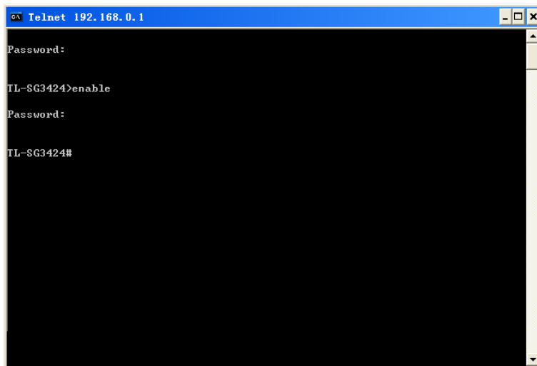
Figure 1-14 Enter into the Privileged EXEC Mode
