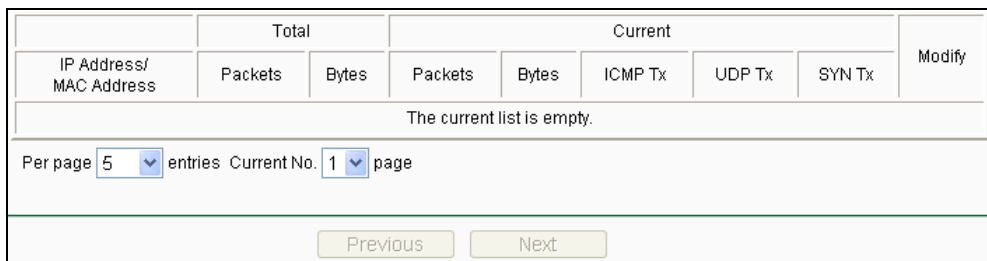
Figure 5-83 Statistics Table
