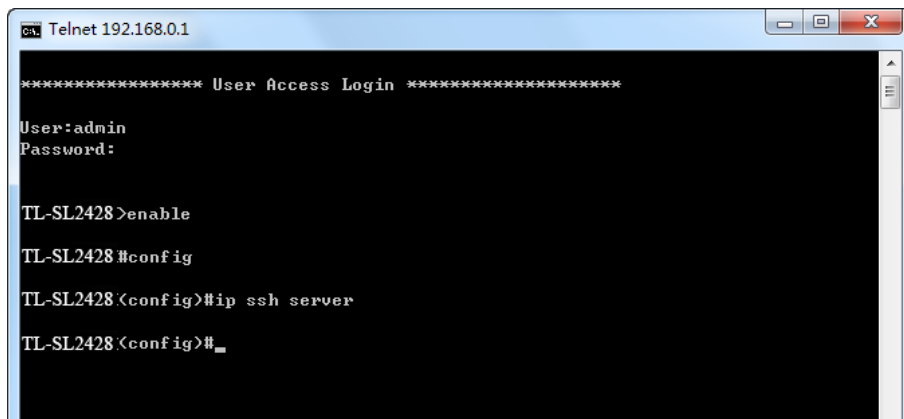
Figure 1-5 Enable SSH function
