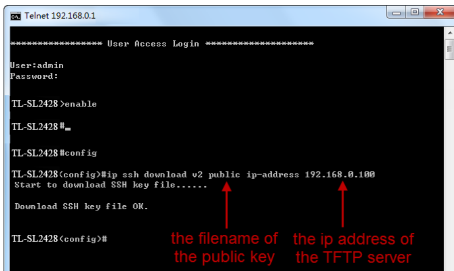
Figure 1-10 Download the Public Key
