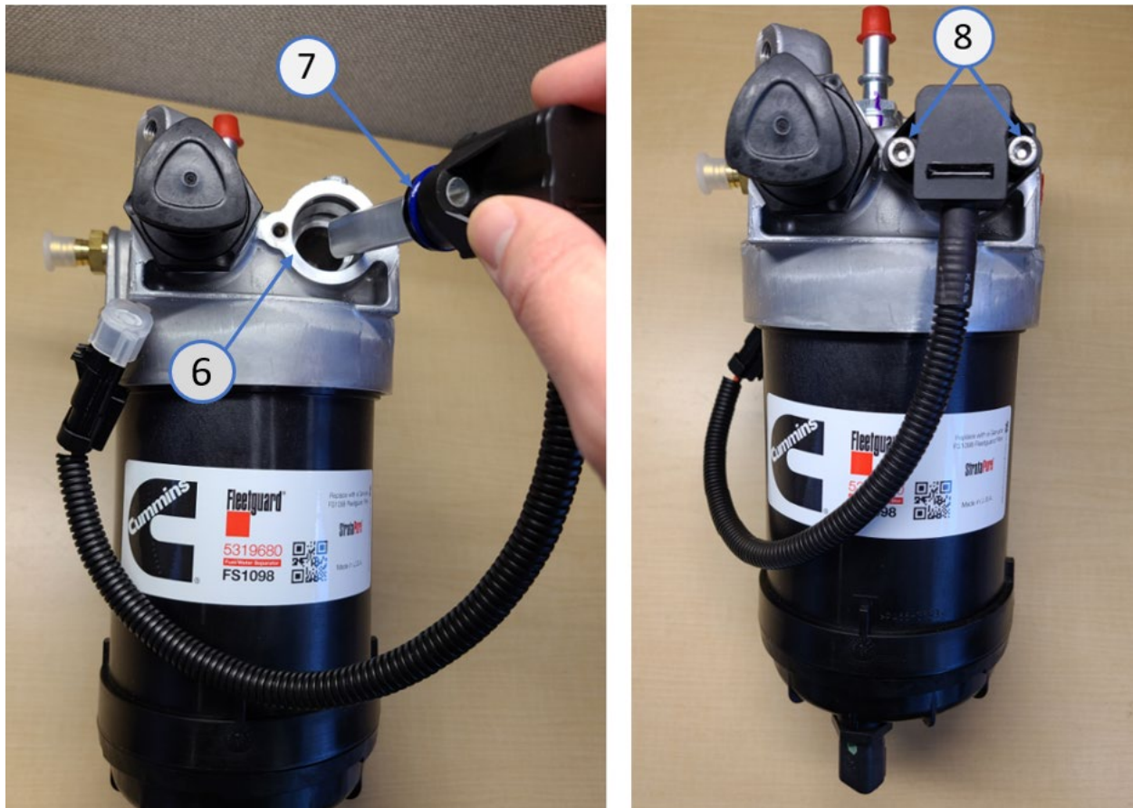
Figure 4: Installation of New Heating Element
