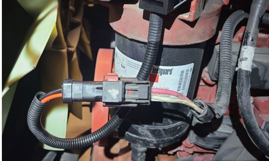
Figure 11: Fuel Heater Harness Connection
