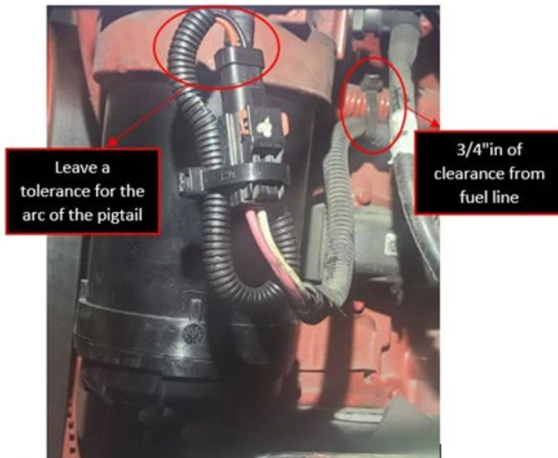
Figure 12: Fuel Heater Harness Routing and Zip Tie Location
