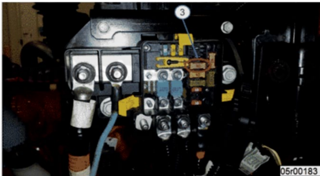
Figure 10: Location of 30A Fuse on Navistar MV/HV/TC
