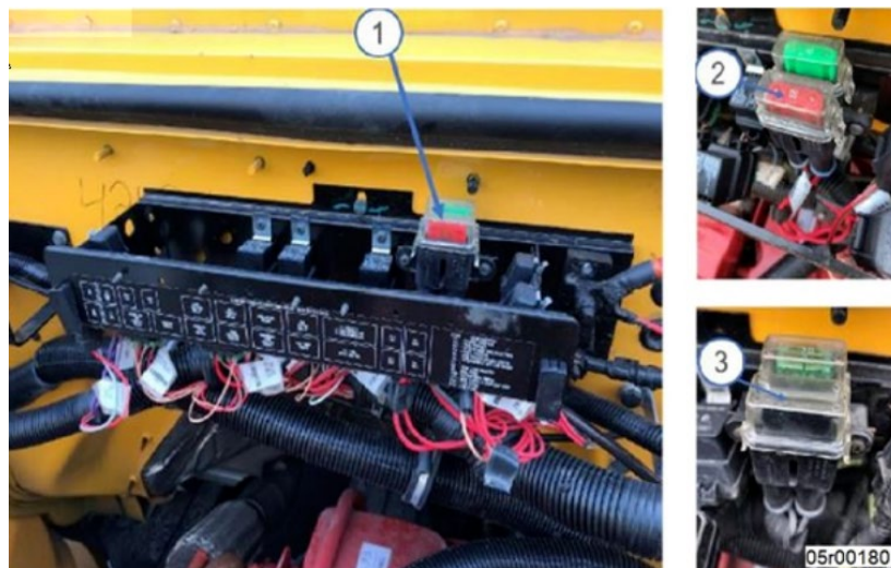
Figure 5: Location of Fuse on Dash Panel
