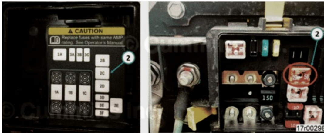
Figure 7: Location of Fuse on Navistar Durastar (4300) / WorkStar (7300) / HC Commercial Bus
