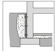
Insulation of basement perimeter/foundation walls
