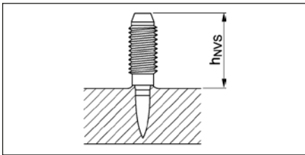
X-ST-GR M8/5 P8, h_{NVS} = 12.0 - 15.0 \text{ mm} X-ST-GR M8/10 P8, h_{NVS} = 17.0 - 20.0 \text{ mm}
