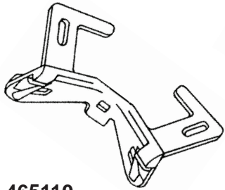
465110 75546-22030 Windshield Moulding Clip Toyota Cressida '81 - '82 Box Qty. 10
