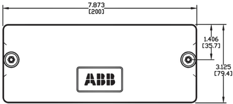
FIG 1. FT-14 WITH CLEAR COVER
