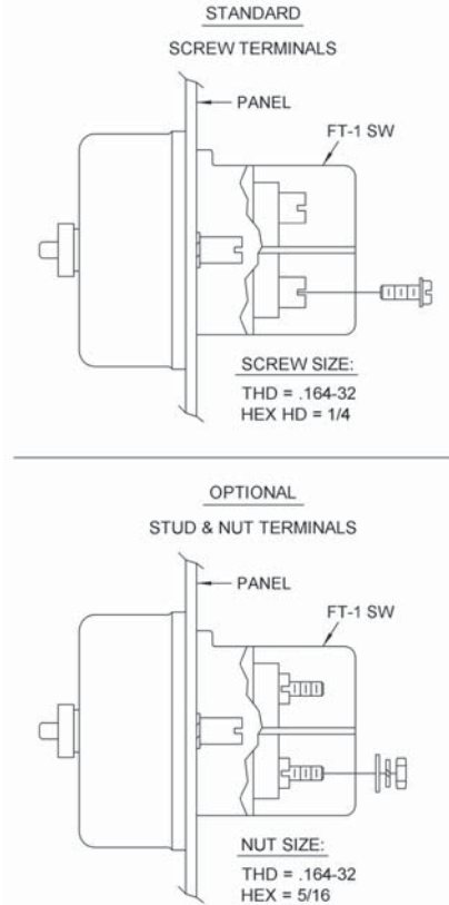
Figure 4. FT Switch terminals, rear view (FT-1 shown)
