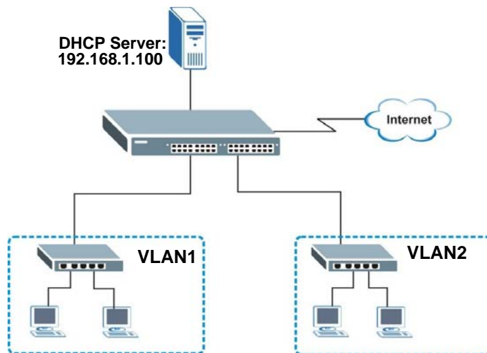
Figure 177 Global DHCP Relay Network Example
