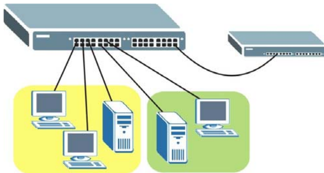
Figure 43 Protocol Based VLAN Application Example
