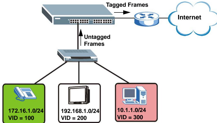
Figure 41 Subnet Based VLAN Application Example
