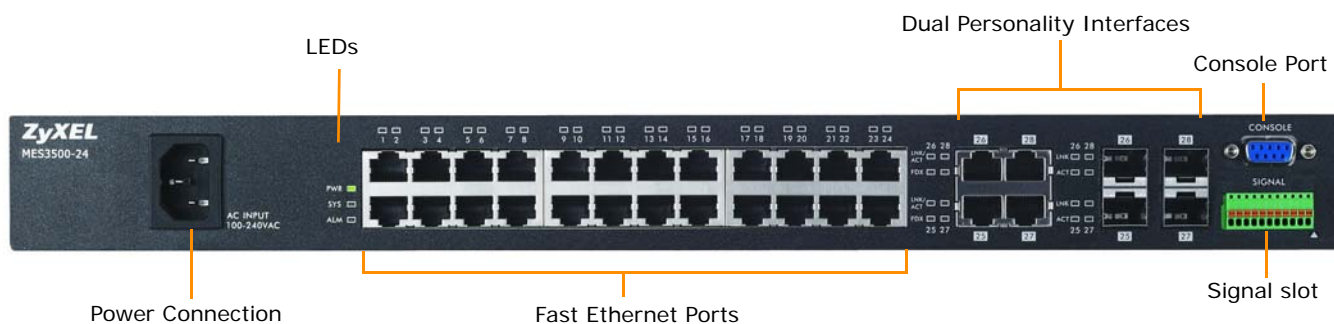
Figure 9 MES3500-24 Front Panel: DC Model
