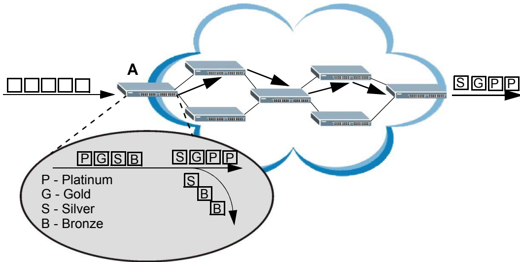
Figure 165 DiffServ Network
