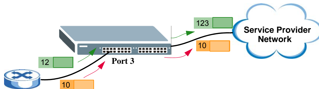
Figure 141 VLAN mapping example
