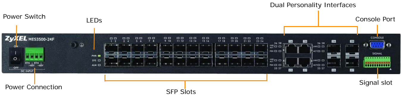
Figure 11 MES3500-24F Front Panel: DC Model
