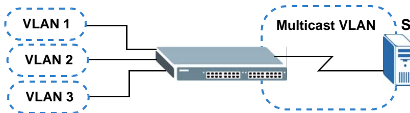
Figure 108 MVR Network Example
