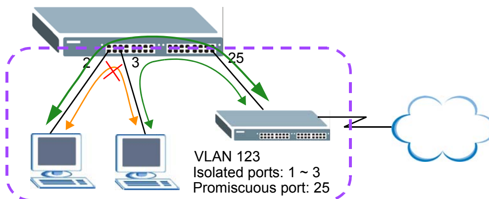
Figure 160 Private VLAN Example
