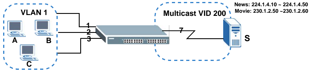
Figure 112 MVR Configuration Example
