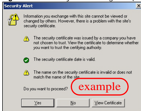
Figure 204 Security Alert Dialog Box (Internet Explorer 6)
