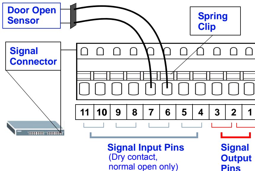
Figure 18 Connecting a Sensor to the Signal Slot
