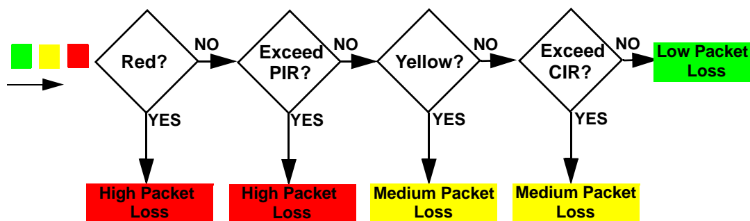
Figure 167 TRTCM-Color-aware Mode
