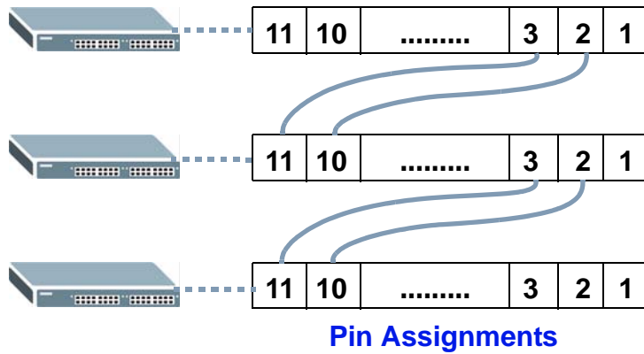
Figure 19 Daisy-chaining an External Alarm Sensor to Other Switches of the Same Model
