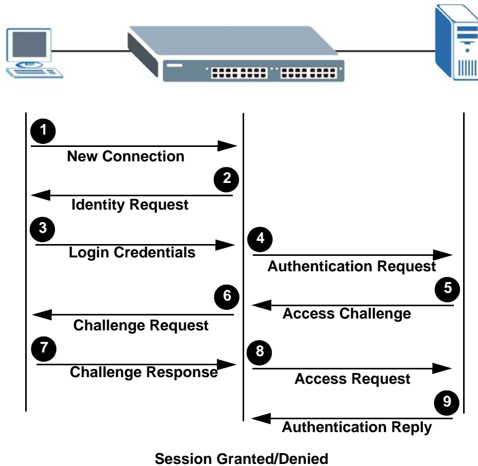
Figure 80 IEEE 802.1x Authentication Process
