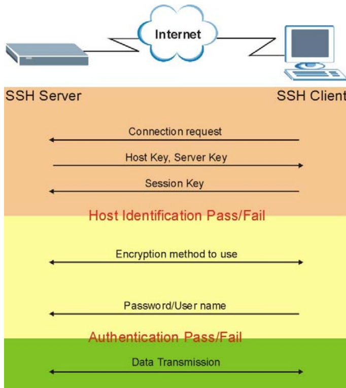
Figure 202 How SSH Works
