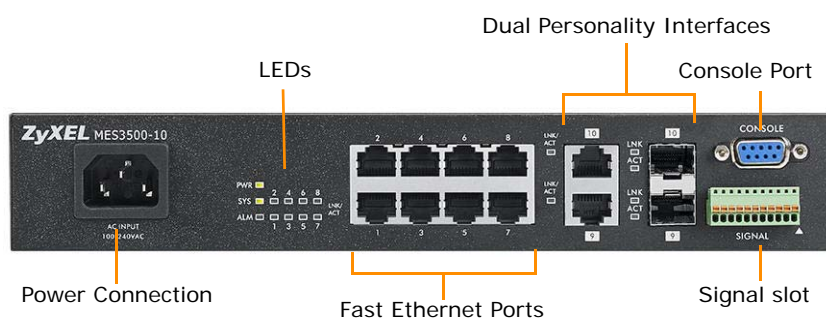
Figure 12 MES3500-10 Front Panel: AC Model
