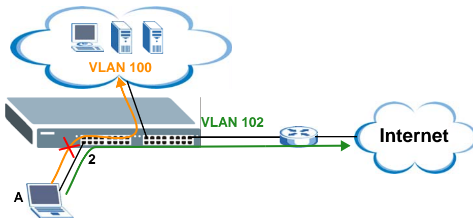
Figure 84 Guest VLAN Example
