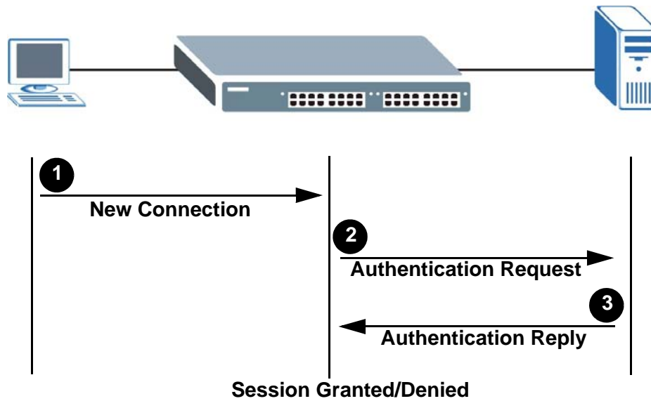
Figure 81 MAC Authentication Process
