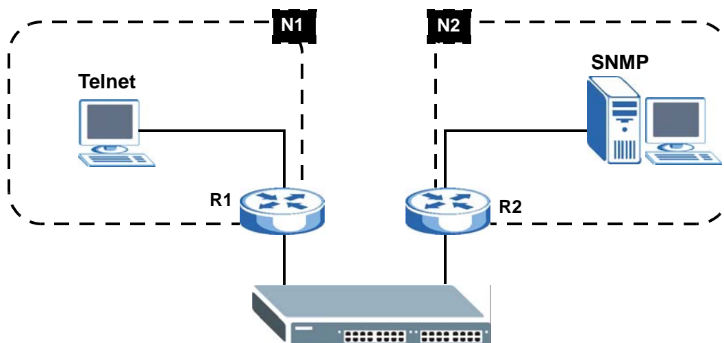
Figure 162 Static Routing Overview
