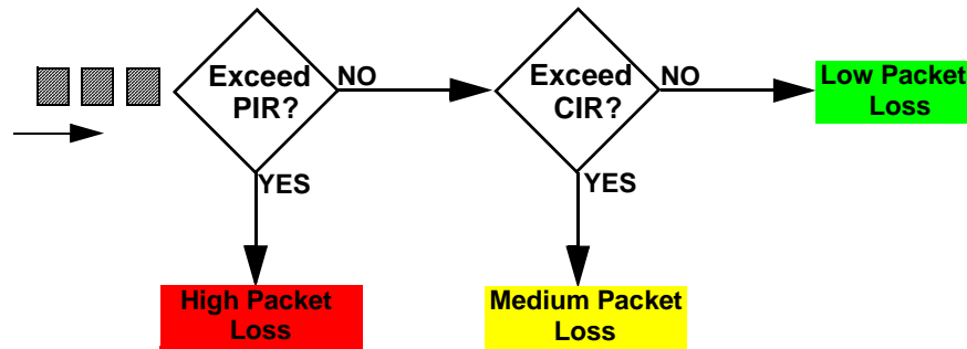
Figure 166 TRTCM-Color-blind Mode
