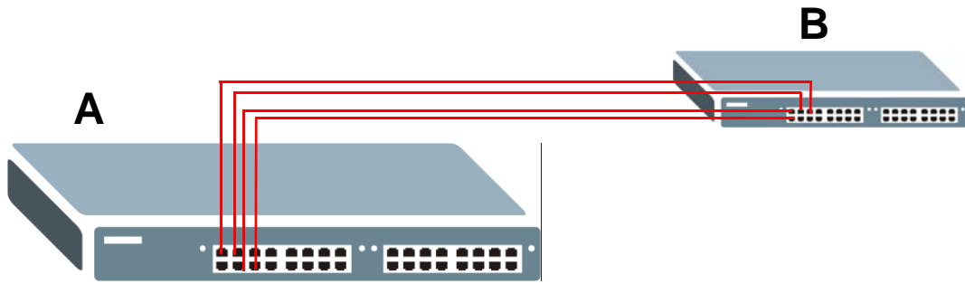
Figure 78 Trunking Example - Physical Connections
