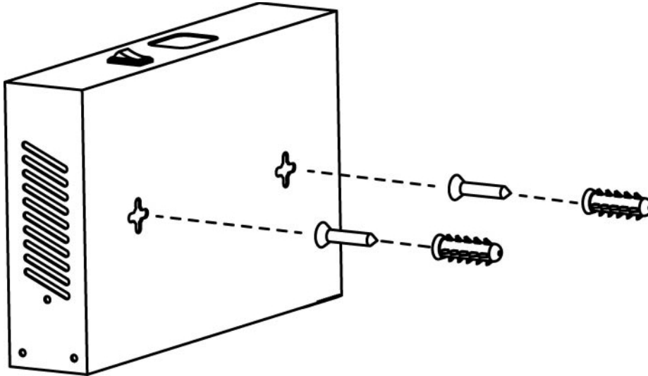
Figure 7 Wall Mounting Example
