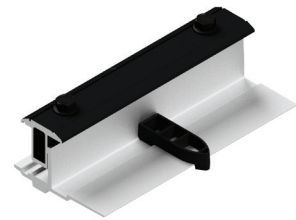
RL Universal Link
