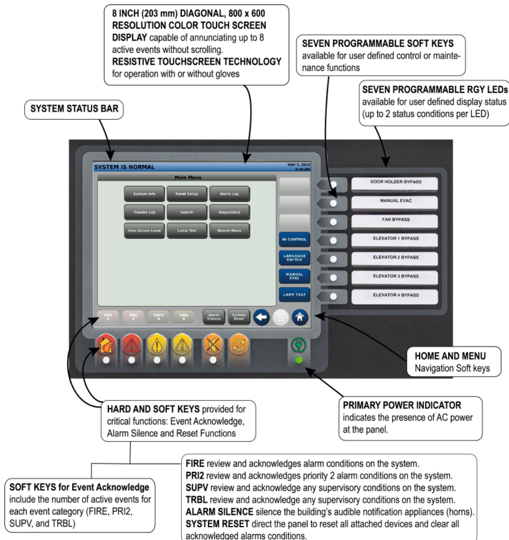
Figure 4: ES Touch Screen Display Operator Interface
