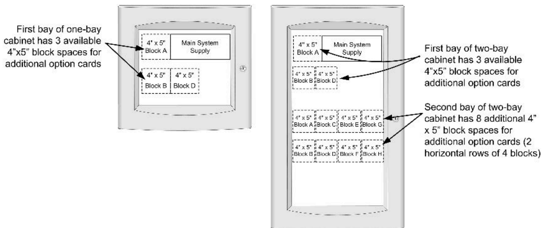
Figure 13: Loading reference
