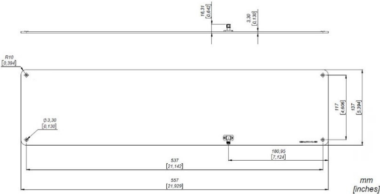
With flange straight or flange right angle connector
