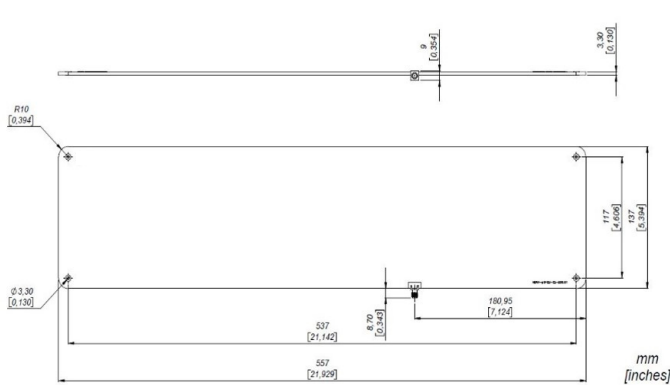
With edge mount connector
