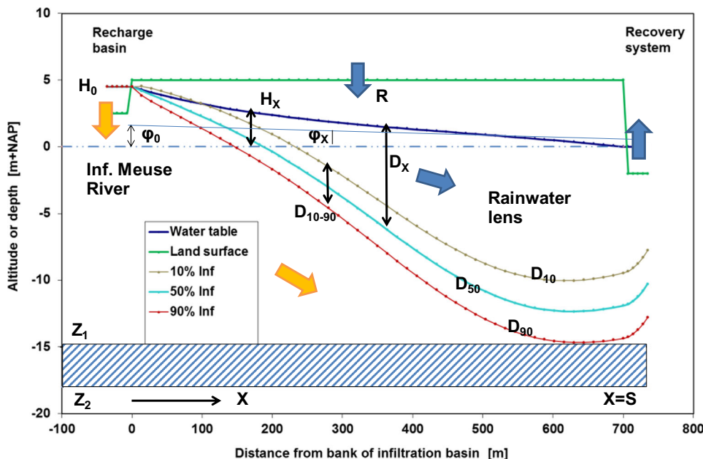
Fig. 13 Schematic of a rain water lens on top of infiltrated Meuse River water migrating seaward, with important parameters for calculating its thickness ( D_X ), and the mixing zone D_{10-90} between both watertypes. For definition of parameters, see explanation to Eqs.20–25
