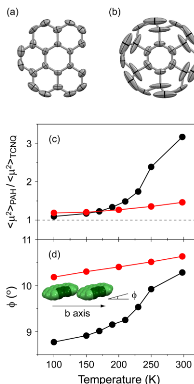
Fig. 7 Thermal fluctuations of (a) bper in 1 and (b) coronene in (coronene)(TCNQ) 9 at 298 K viewed perpendicular to the molecular plane. Hydrogen atoms are omitted for clarity, and the 50% probability thermal ellipsoids are shown. Temperature dependence of (c) relative \langle \mu^2 \rangle values of PAH (bper or coronene) with respect of that of TCNQ ( \langle \mu^2 \rangle_{\text{PAH}} / \langle \mu^2 \rangle_{\text{TCNQ}} ) and (d) angles between the PAH plane and the crystallographic axis along the side-by-side direction ( \phi ) in each CT solid (red circles: 1 , black circles: (coronene)(TCNQ)). 9 The inset shows the arrangement of bper molecules in 1 along the b axis.
