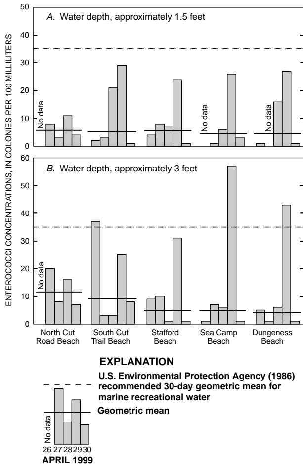
Figure 8. Enterococci concentrations of the near-shore Atlantic Ocean at five Cumberland Island beaches, Georgia, April 26–30, 1999.
