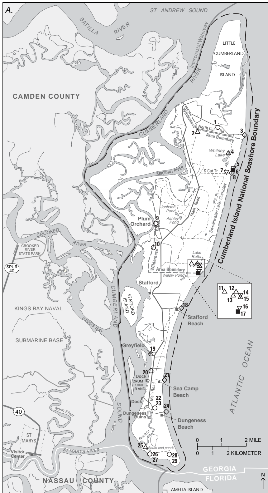
Figure 1. Location of Cumberland Island National Seashore, Georgia; (A) sampling sites, April 1999 to July 2000; and (B) wells with historical data.
