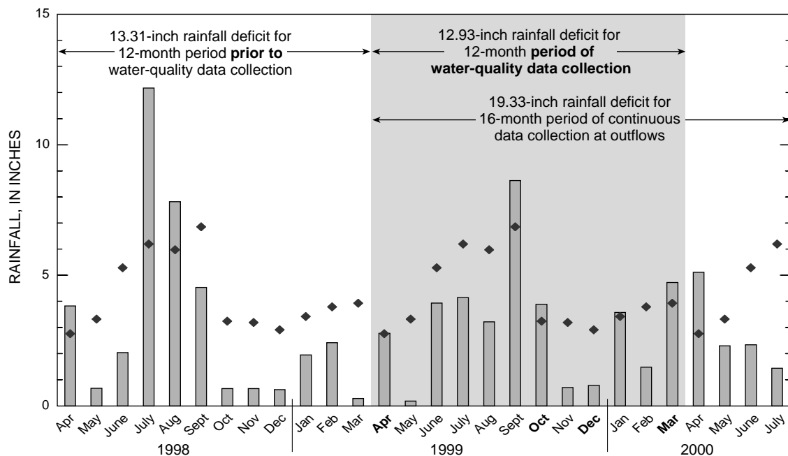
Figure 6. Monthly rainfall, April 1998 through July 2000, and 30-year-average monthly rainfall, 1961–90, at Fernandina Beach, Florida. Thirty-year-average annual rainfall is 50.83 inches. (Data source: National Climatic Data Center, http://cdo.ncdc.noaa.gov/plclimprod/plsql/poemain.poe , accessed on July 12, 2001.)
