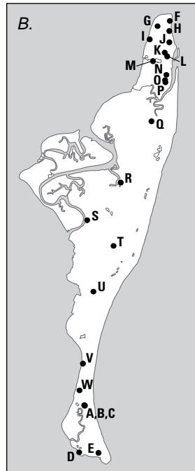
Figure 1. Location of Cumberland Island National Seashore, Georgia; (A) sampling sites, April 1999 to July 2000; and (B) wells with historical data.
