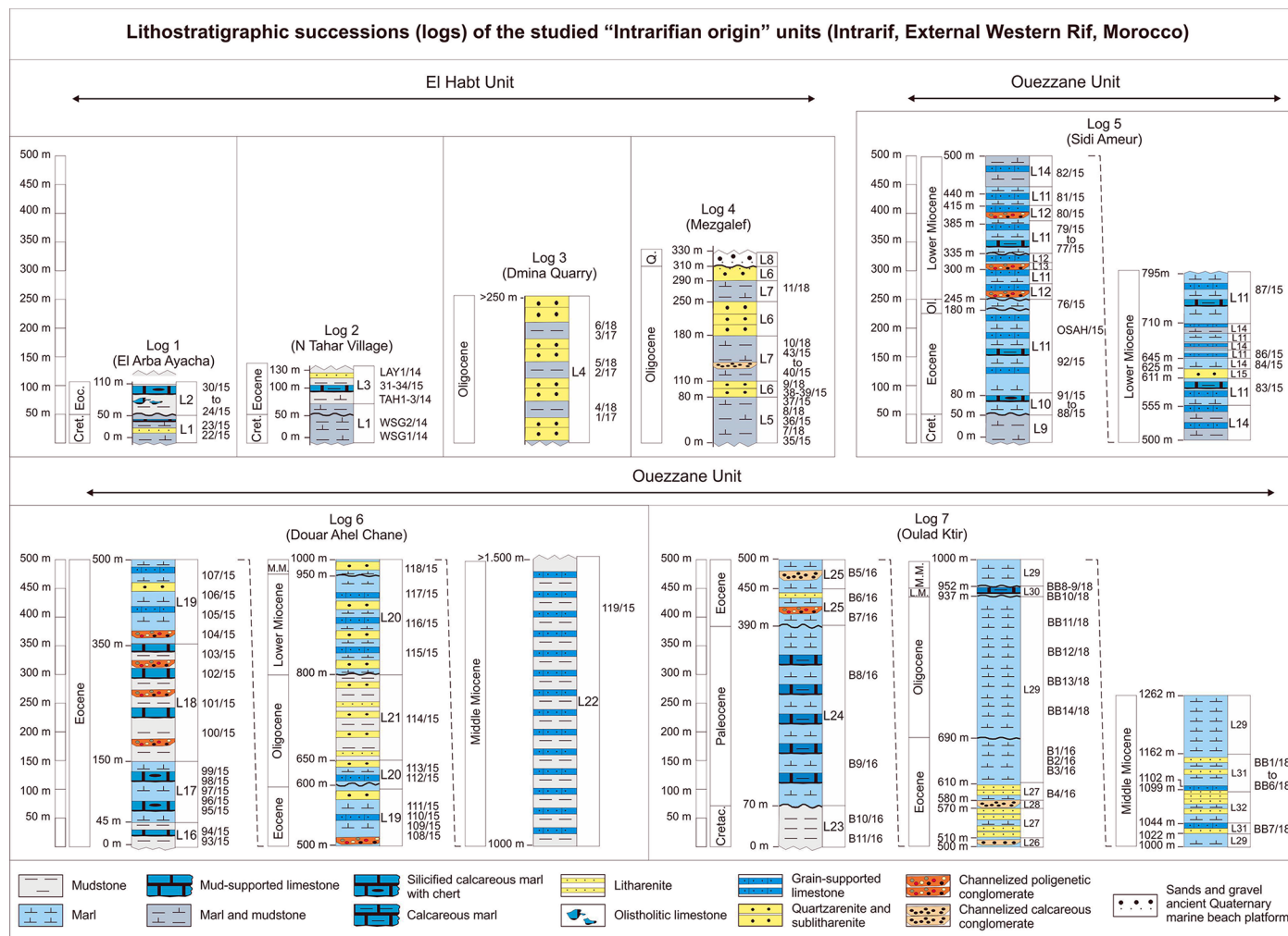
Figure 3. Lithostratigraphic successions studied are shown with the defined lithofacies analyzed and positions of samples (see numbers to the right of lithofacies corresponding with Table 1). The locations of the stratigraphic successions measured are shown in Figure 2.
