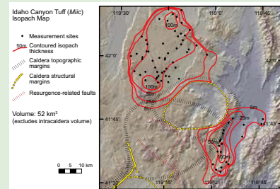
Figure 1: Supplemental Figure 1. Isopach maps for ignimbrites in the High Rock caldera complex. Please visit http://dx.doi.org/10.1130/GES01162.S4 or the full-text article on www.gsapubs.org to view Supplemental Figure 1.
