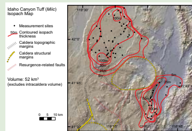
'Supplemental Figure 1. Isopach maps for ignimbrites in the High Rock caldera complex. Please visit http://dx.doi.org/10.1130/GES01162.S4 or the full-text article on www.gsapubs.org to view Supplemental Figure 1.
