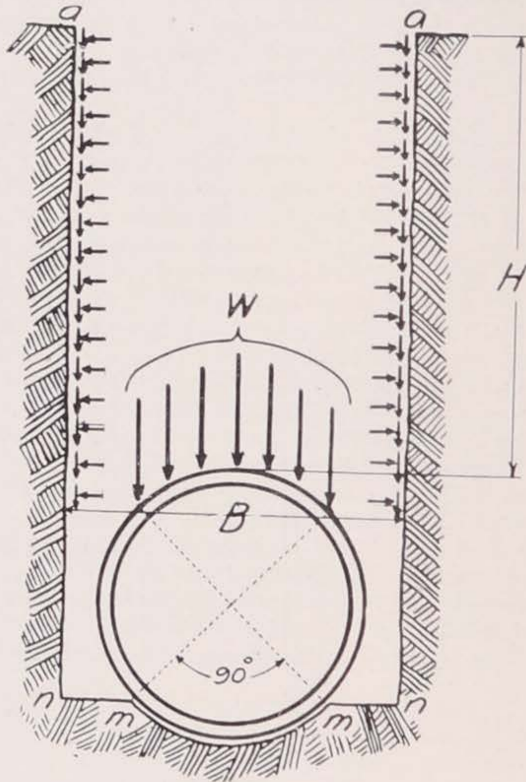
Fig. 11. Typical Conditions of Bedding and Loading of Pipe in Ditches. the ditch develops a frictional resistance, which helps to carry part of the weight.
