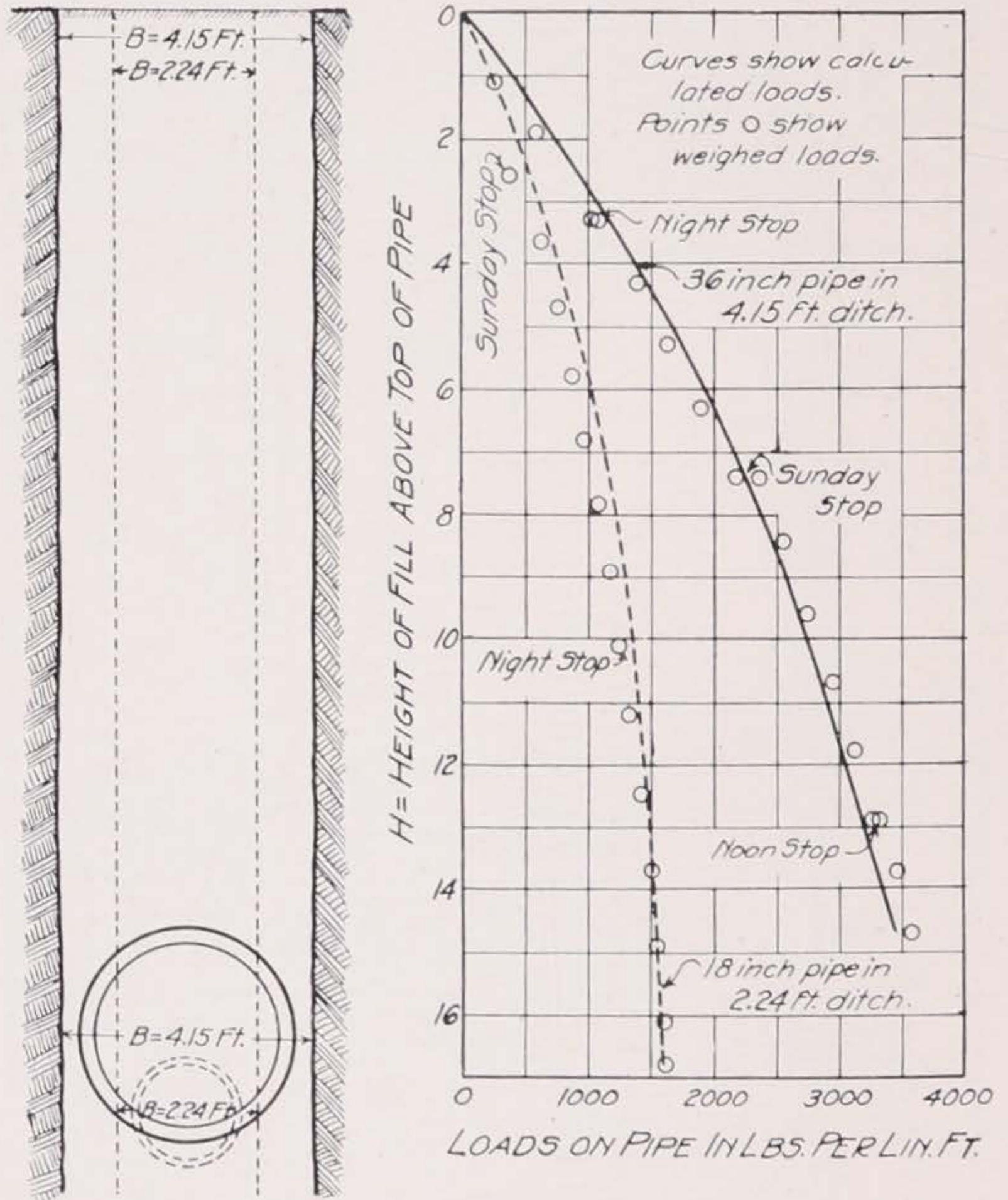
Fig. 21. Diagram Showing Comparison of the Weighings of Actual Loads on Pipes in Ditches in Experiments Nos. 7 and 9 with the Calculated Loads.
