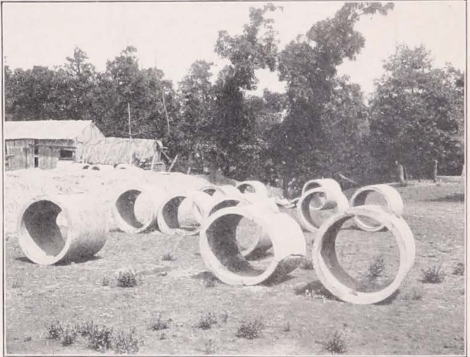
Fig. 5. View of Cracked 36 Inch Drain Tile from Ditch in Drainage District No. 48, Boone County, Iowa.
