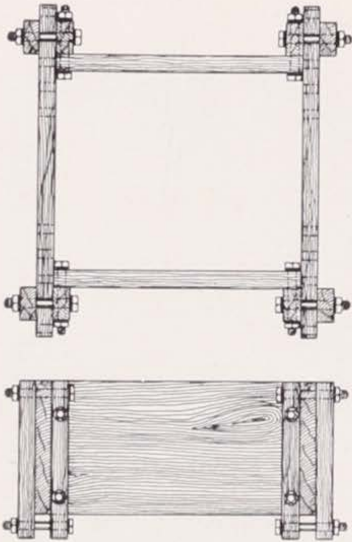
Fig. 36. Plans for Sand Bearing Frame for Iowa Standard Tests.
