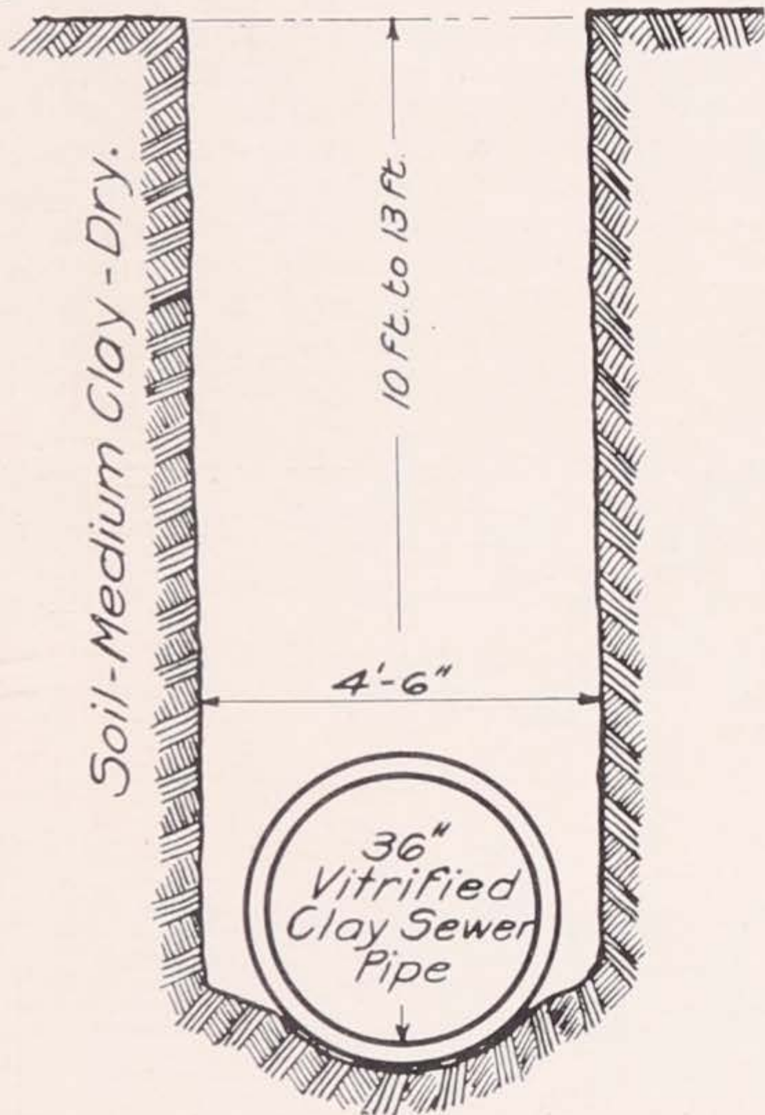
Fig. 6. Cracking of 36 Inch Vitrified Clay Sewer Pipe in Ash Street Sewer, Clinton, Iowa.
