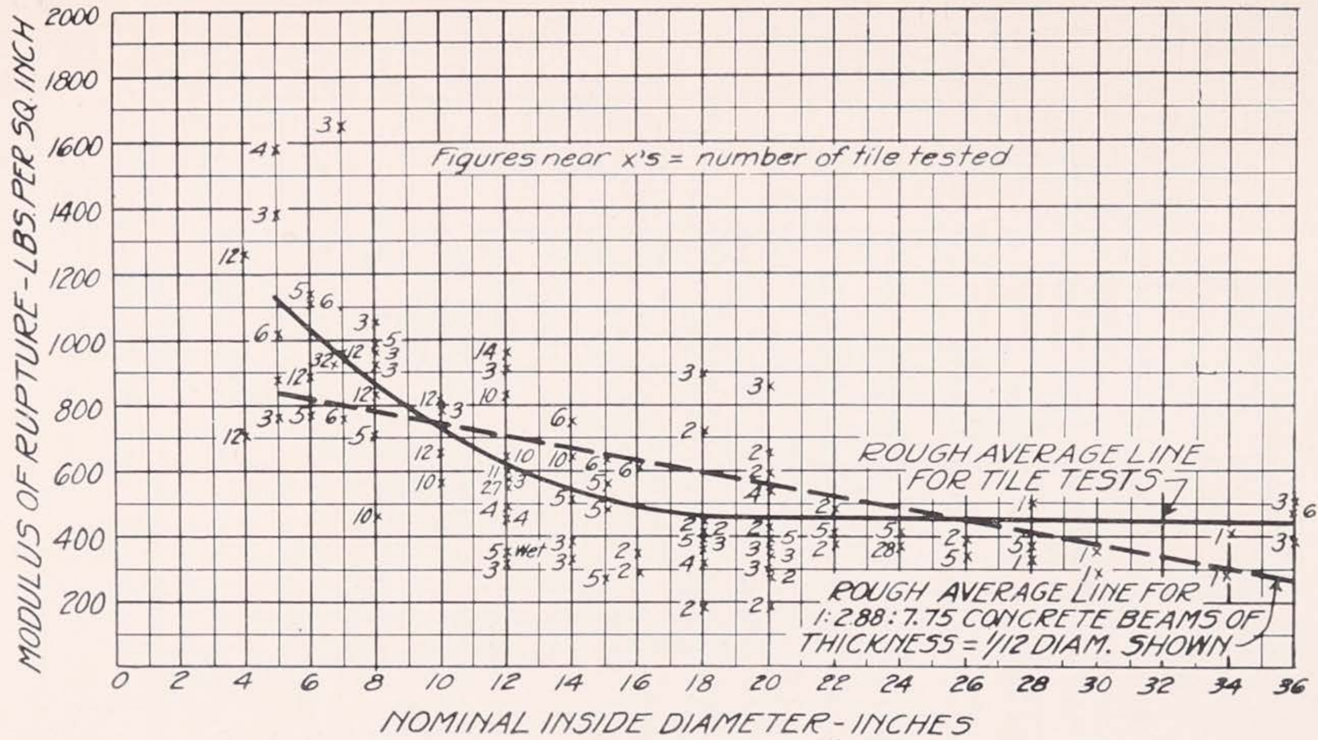
Fig. 28. Values of the Modulus of Rupture of Cement Drain Tile.
