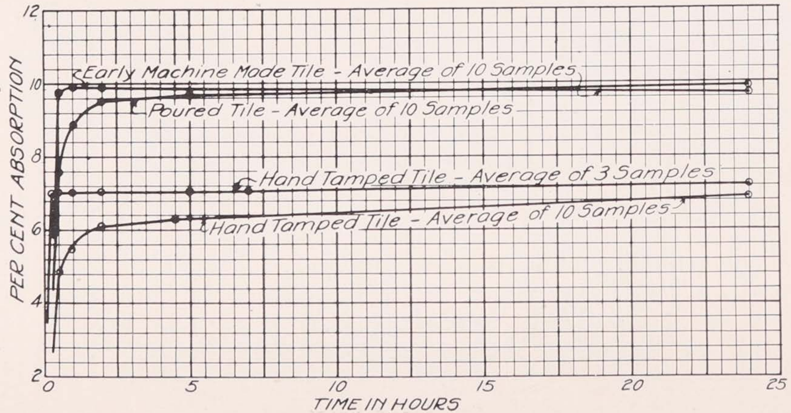
Fig. 30. The Rate of Absorption of Water by Cement Drain Tile.
