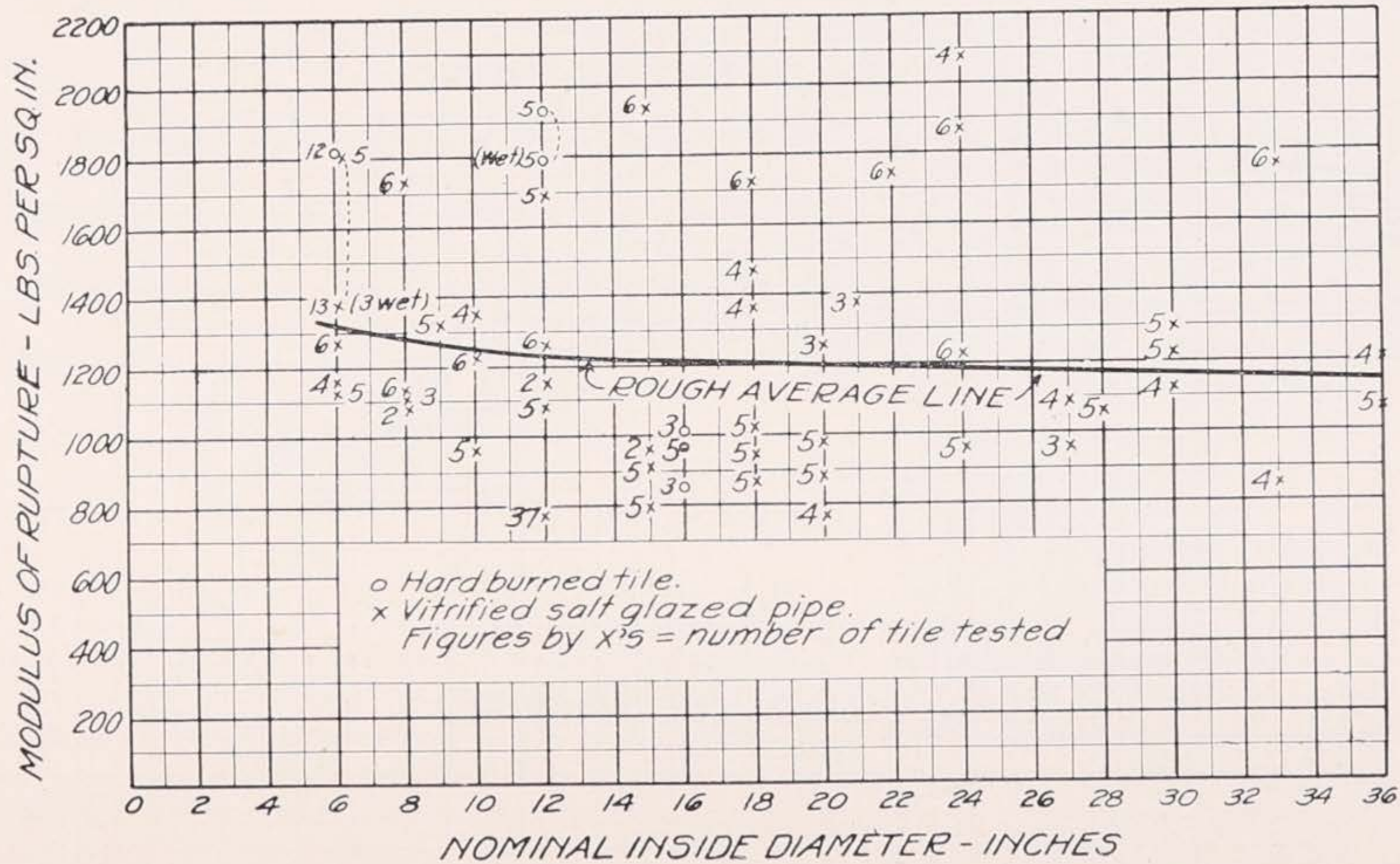
Fig. 29. Values of the Modulus of Rupture of Clay Drain Tile and Sewer Pipe.
