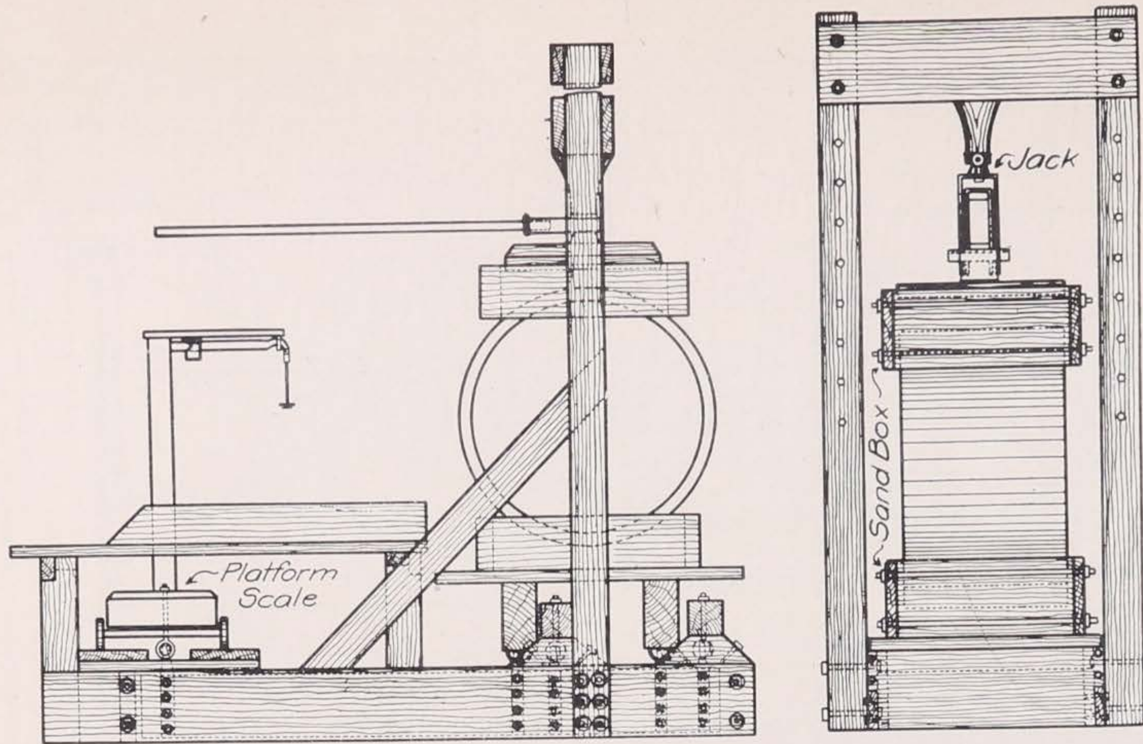
Fig. 31. The Ames Standard Testing Machine, for Testing the Strength of Drain Tile and Sewer Pipe. Cost, about $95, not including the 2000 lbs. Platform Scales.
