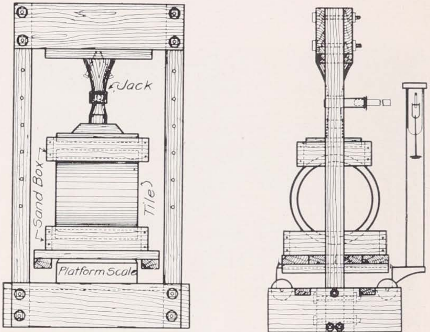
Fig. 34. The Ames Junior Testing Machine, for Testing Drain Tile up to 18 Inches Diameter. Cost about $20, not Including 2000 lbs. Platform Scales.
