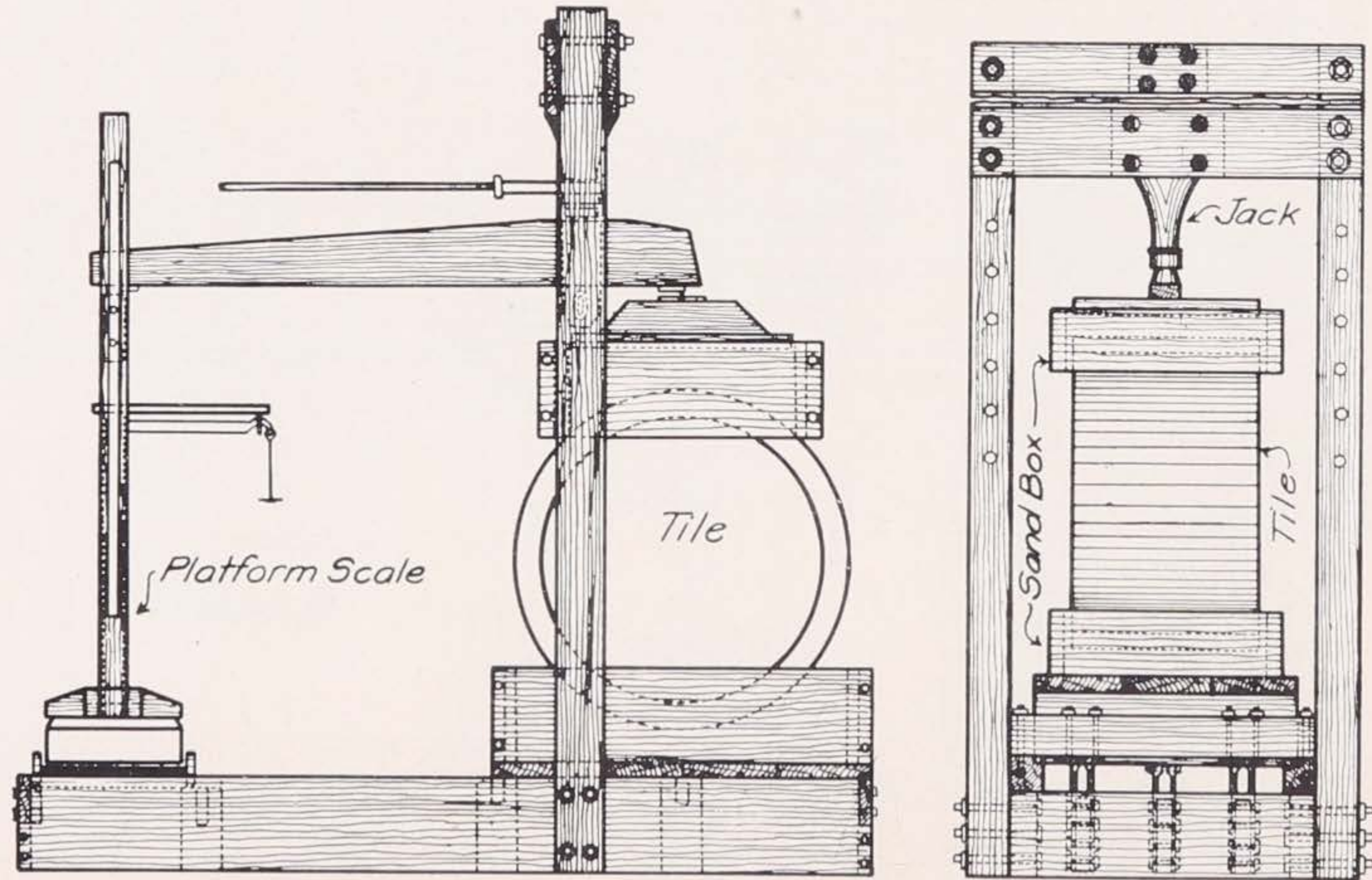
Fig. 32. The Ames Senior Testing Machine, for Testing the Strength of Drain Tile and Sewer Pipe. Cost about $40, not Including the 2000 lbs. Platform Scales.
