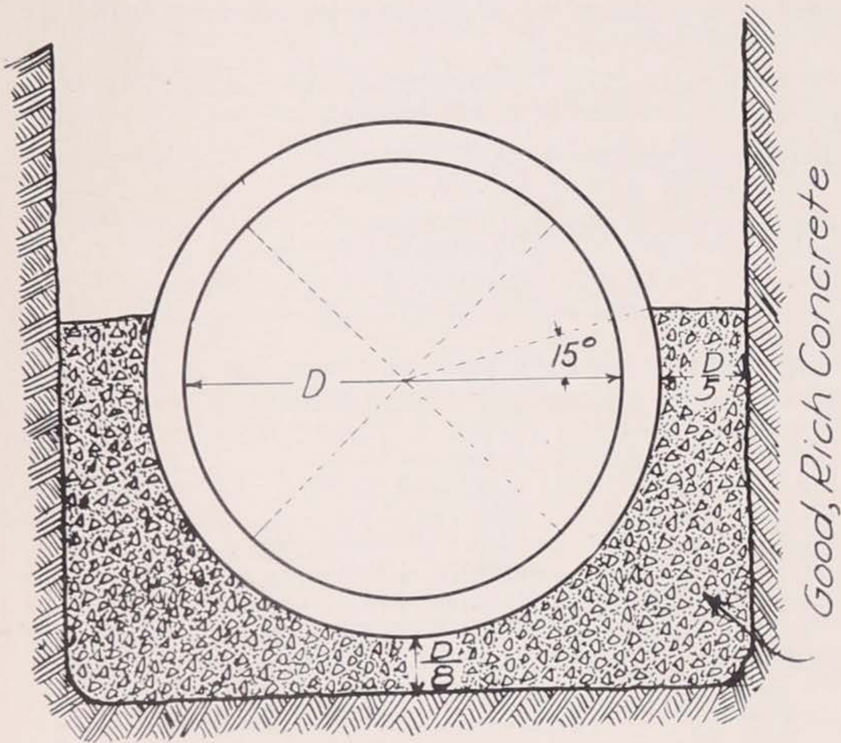
Fig. 39. Method of Strengthening Drain Tile and Sewer Pipe to Carry Heavy Loads, by Bedding in Concrete, in Yielding Soils.
