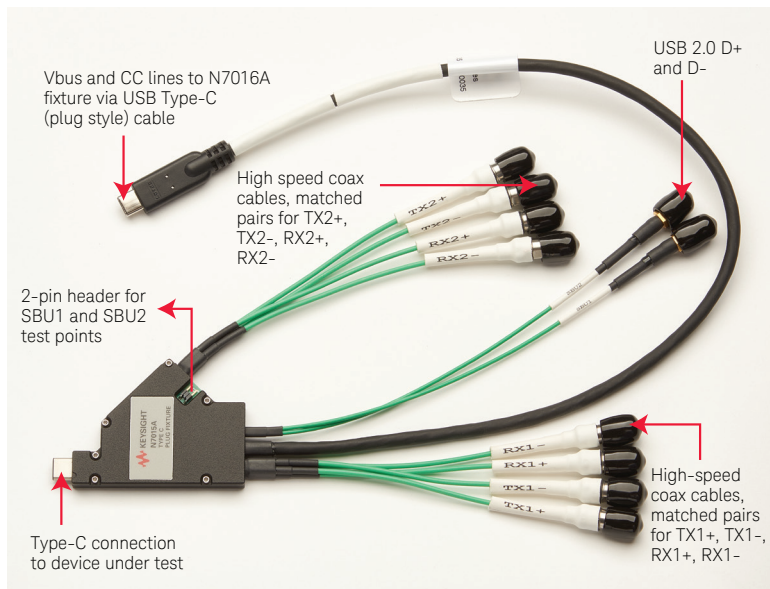
Figure 1. N7015A Type-C high-speed fixture.
