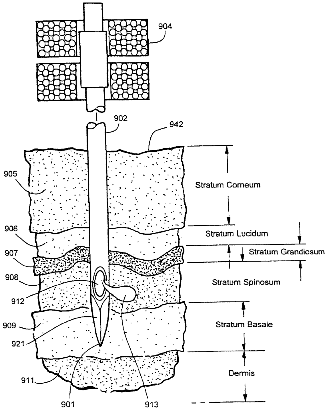
Syringe Needle
