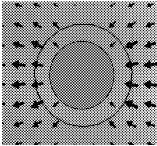
Hybrid mode (HE11) 2057
