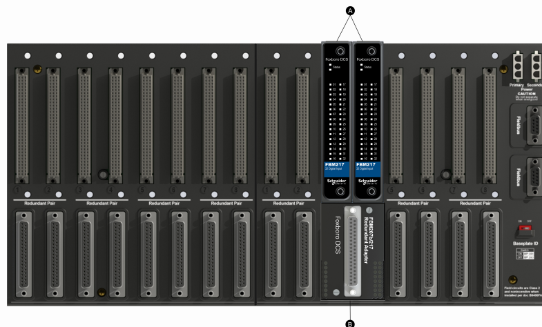
Figure 1 - Compact FBM217 Redundant Module Configuration
