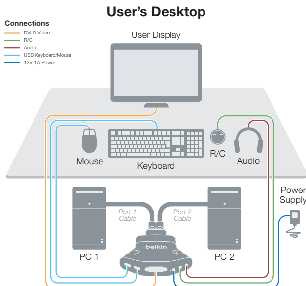
F1DN102F-3 Belkin Advanced Secure 2-Port Flip KVM
