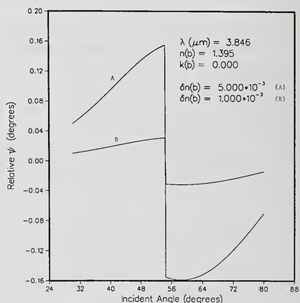
Figure 2. Difference function D\psi(\theta) for \delta n = (A) 0.005 and (B) = 0.001; both are evaluated at n = 1.395 and k = 0 . The deviations in \psi for \theta from 40 to 70^\circ for curve B are about 0.02 to 0.03^\circ . Since the instrumental error of \psi is 0.01^\circ , the precision in n is expected to be better than 0.001.
