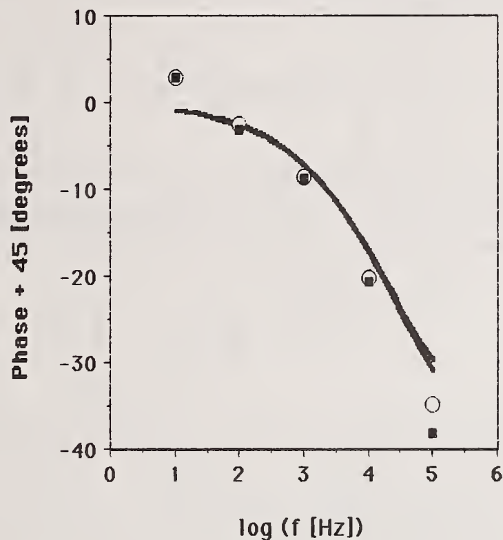
Fig. 1. 1 \mu\text{m} RF Sputtered Ni Coating on Fused Silica
