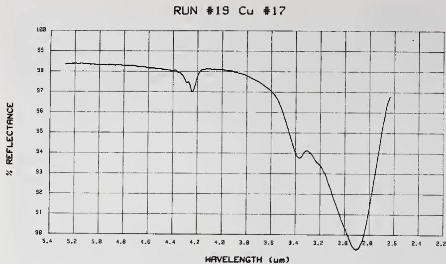
Figure 16. Plot of spectral reflectance versus wavelength shown with wavelength decreasing from left to right for an undosed \text{CaF}_2 film on SPDM Cu. The sample is unbaked. The reflectance minimum at 2.9 \mu\text{m} reflectance is around 89.5%. The additional local minimum at 3.4 \mu\text{m} can be seen.
