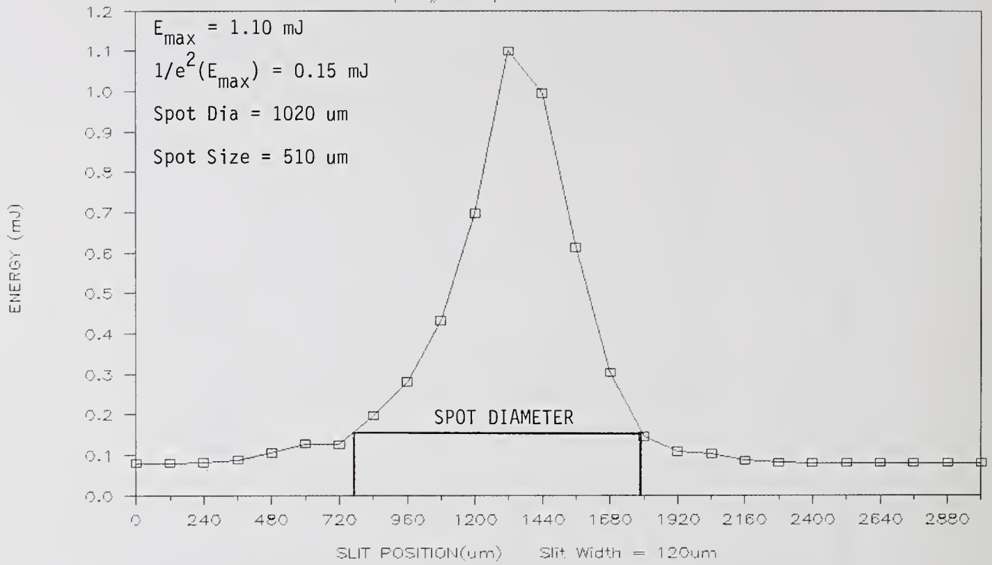
Figure 2. Spatial Energy Distribution of a Focused Beam
