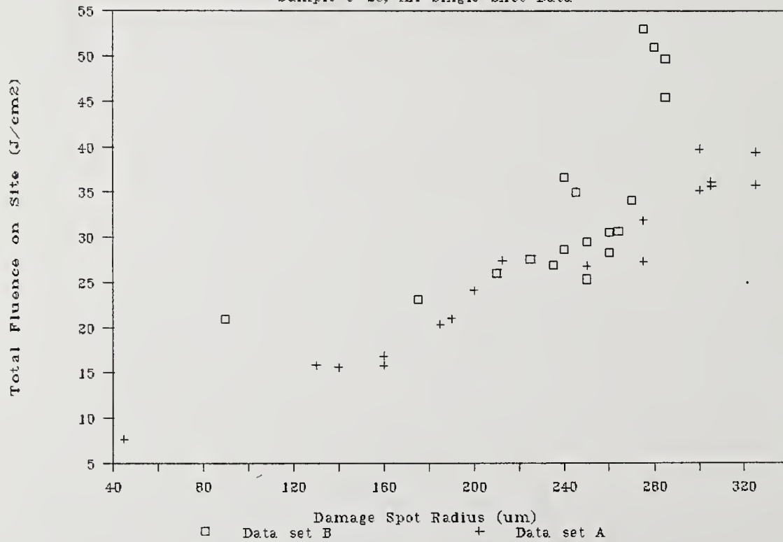
Figure 11. The total fluence (over the entire 1/e 2 radius of the beam) on site versus the damage site radius.
