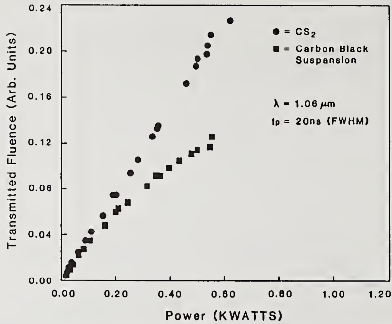
Figure 5. Plot of on set of limiting of CS 2 (circles) and CBS (squares) as a function of input power for 20 ns (FWHM), 1.06 \mu\text{m} pulses.
