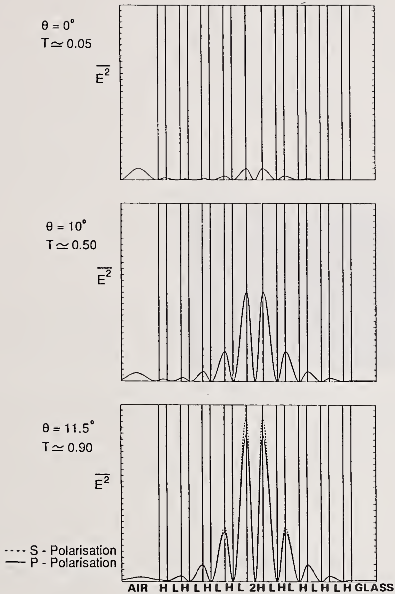
AVERAGE FIELD SQUARED vs. POSITION THROUGH A THIN FILM FABRY-PEROT FILTER FOR DIFFERENT ANGLES OF INCIDENCE
