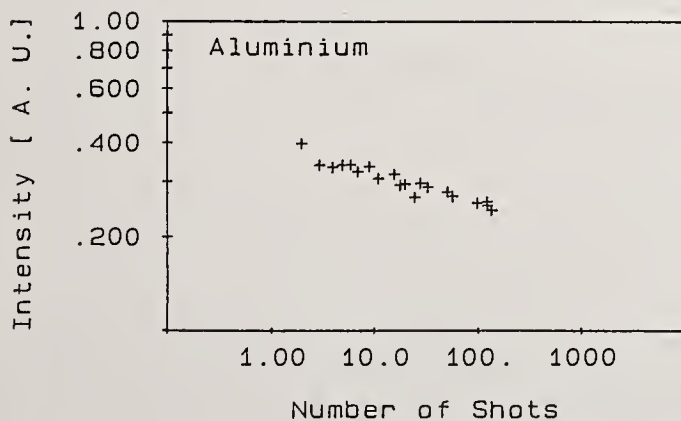
Figure 5: Log-log plot of damage threshold vs. number of shots. Note the deviation from straight lines, which are expected from Eq. (1).
