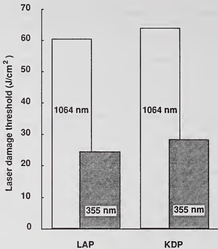
Figure 7. Both LAP and KDP crystals can be grown to yield bulk damage thresholds \geq 60 \text{ J/cm}^2 at 1064 nm with 10-ns pulses. The samples meet or exceed the design goal of 35 \text{ J/cm}^2 at 1064 nm and 25 \text{ J/cm}^2 at 355 nm.
