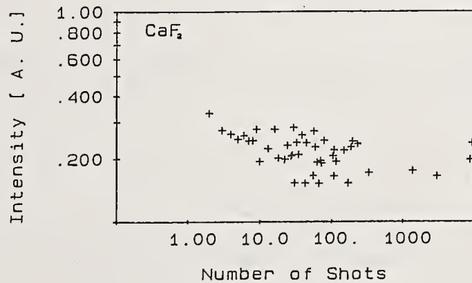
Figure 4: Analysis of incubation effect according to Eq. (1) for PMMA, CaF 2 , Al, and Cu.
