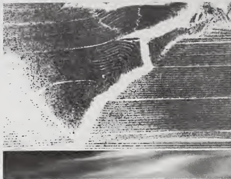
Figure 1. Cross sectional transmission electron micrograph (XTEM) showing stress induced failure of \text{BaF}_2/\text{ZnS} digital multilayer.
