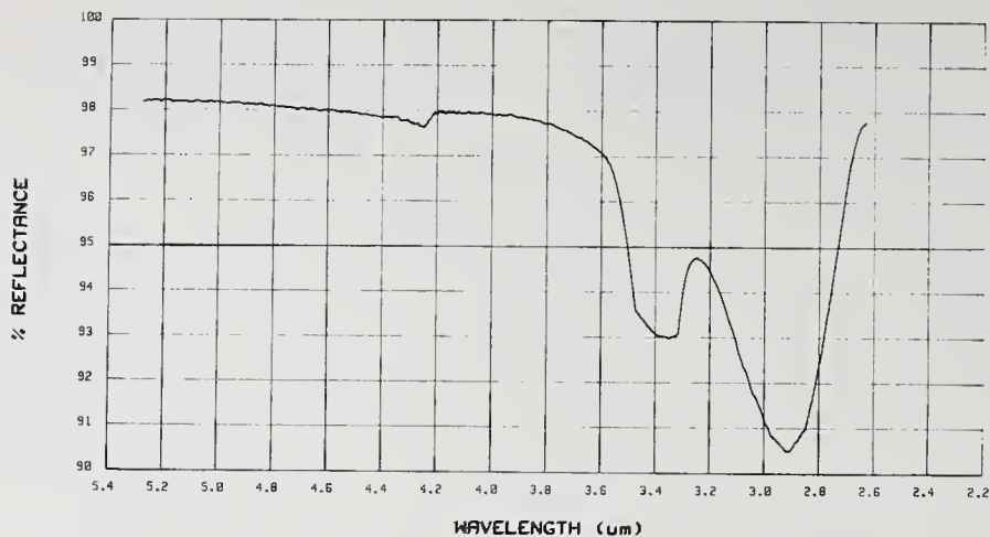
Figure 5. Plot of reflectance versus wavelength shown with wavelength decreasing from left to right for a D 2 O-dosed CaF 2 film on SPDM Cu. The sample has gone through a 12-hr bakeout. The reflectance minimum at 2.9 μm, up from the coating discussed in figure 4 at around 90.5%, is due to H 2 O. The additional local minimum at 3.4 μm has increased dramatically over the undosed film and has saturated the detector. No evidence of absorption related to the D 2 O dosing is evidenced.
