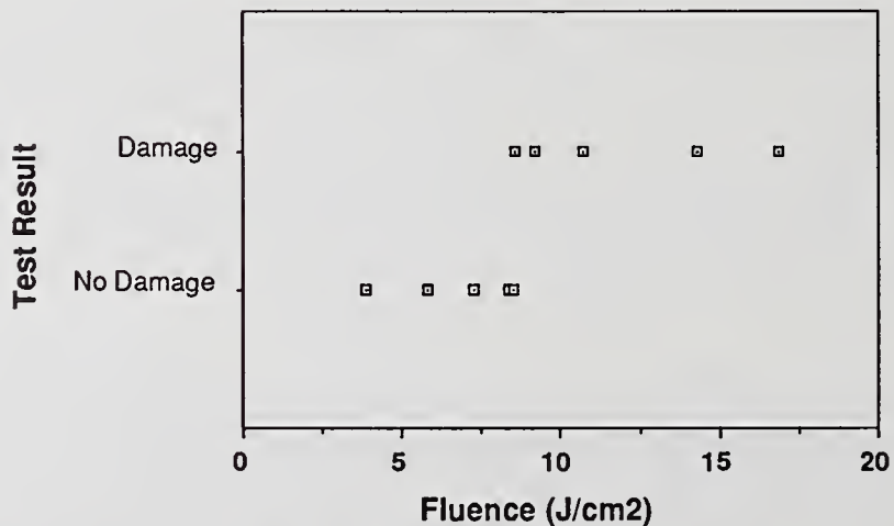
Figure 3c. Unconditioned results for sample B with a 1.00 mm spot size.
