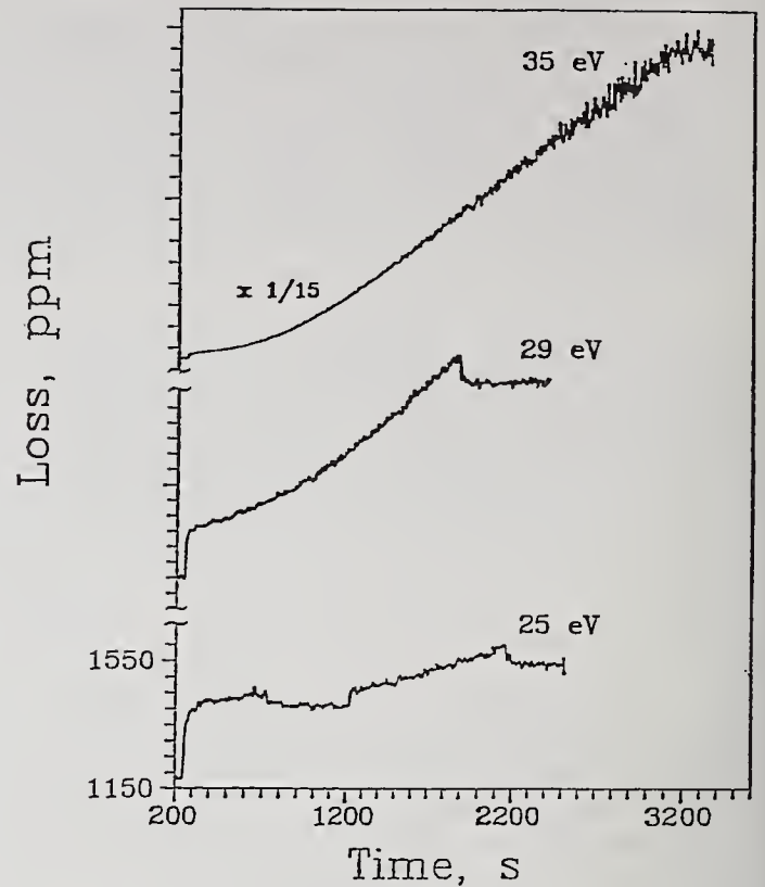
Figure 5. Exposure data is shown for higher photon energies where a new loss mechanism appears. The induced absorption varies in a nonlinear way with the fluence and can reach extremely high levels. The intensities were, from bottom to top, 300, 276, and 1000 \text{mW}/\text{cm}^2 respectively.
