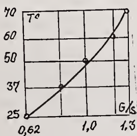
FIGURE 11B. Experimental dependence of water consumption on temperature T with voltage amplitude of U=80\text{ V} , angle of inclination 90\text{ grad} and height of a capillary pipe 220\text{ mm} .
