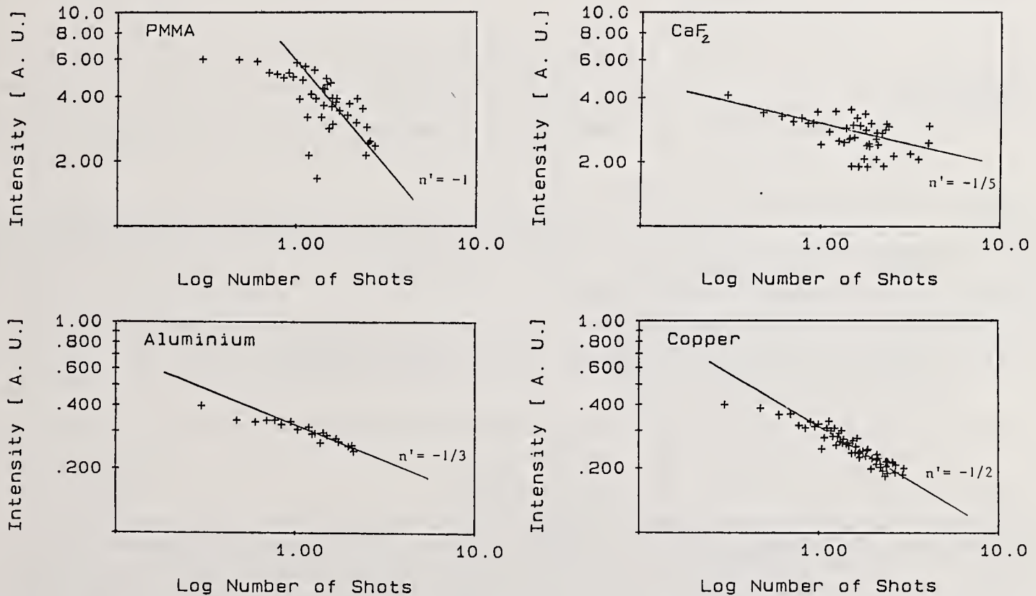
Figure 6: Analysis of incubation effect along the lines of the defect creation model ( \log [threshold intensity] vs. \log [ \log (number of shots)]). For large N , all data may be represented by Eq. (12). The slopes n' are obtained by assuming integer orders of nonlinear energy input.
