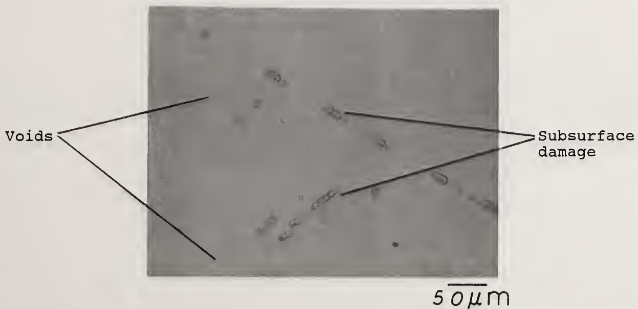
Figure 3. Nomarski micrographs showing representative subsurface defect on fused silica surface after exposure to selective delineation etch (a) super polish, (b) standard polish
