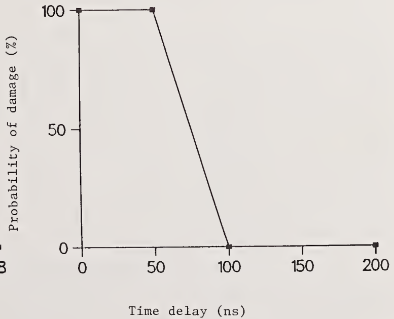
Fig 6 Variation of the probability of damage for differing delays between the UV and IR laser pulses on silicon
