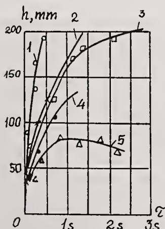
FIGURE 2A. Dependence of the height of water rise in a capillary on time ( d = 1,2 mm; f = 41 kHz; N = 25 wt) for different values of clearance between the source's face and the capillary's cut:
