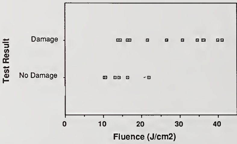
Figure 3b. Unconditioned results for sample B with a 0.5 mm spot size.
