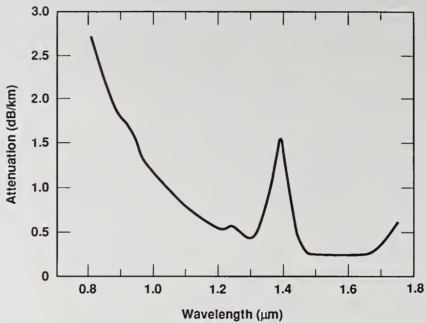
Figure 7. Loss spectrum for a Ge-doped, graded index SiO 2 fiber drawn from a preform made by the PICVD process (see ref. 19).
