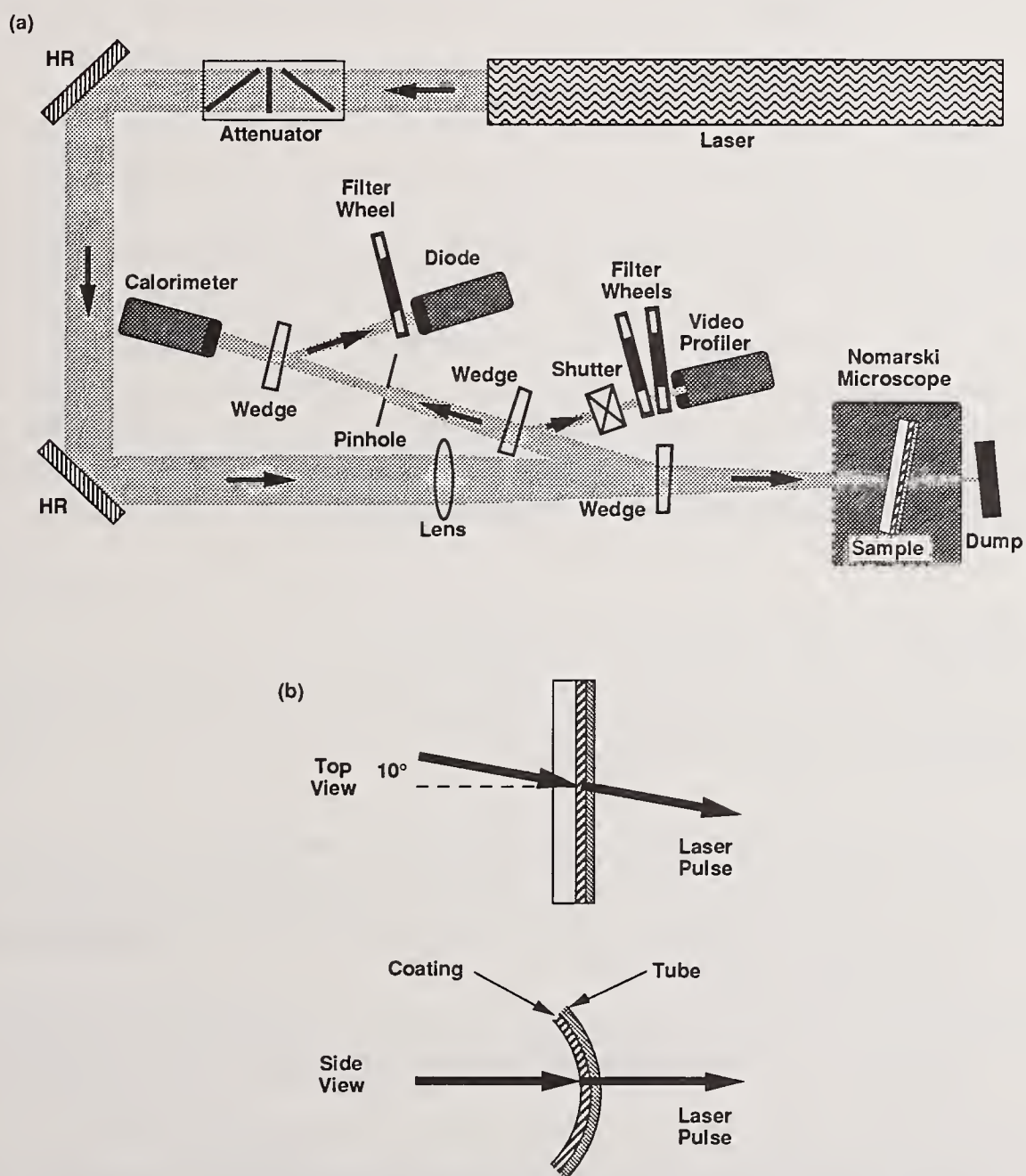
Figure 11. (a) Schematic representation of the 1064 nm laser damage test system used to test the PICVD coatings, and (b) configuration of the damage test sample cut from the 17.2 mm ID SiO 2 tube used as a substrate for the coating process.
