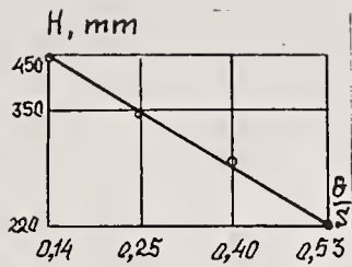
FIGURE 11A. Experimental dependence of consumption on the height of water in a capillary with T=22\text{ }^{\circ}\text{C} , amplitude of GUO voltage U=80\text{ V} and angle of inclination of HP \alpha=90\text{ grad} .
