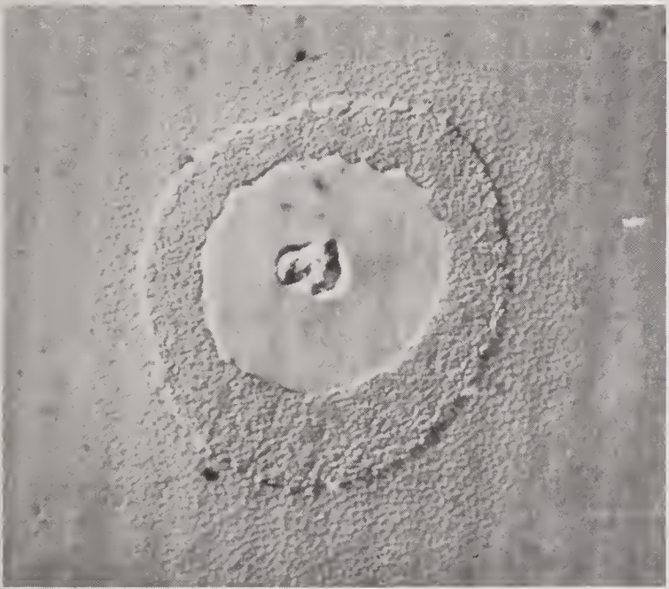
Figure 13. Photograph of HF laser-induced damage of H 2 O-dosed CaF 2 on SPDM Cu. Damage morphology is ablation and "orange-peel-like" surface roughening. Damage has penetrated into the Cu without modifying the damage morphology; 360X magnification.
