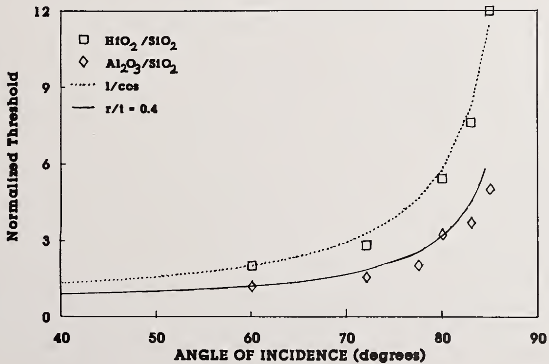
Figure 6. The laser damage threshold values for HfO 2 /SiO 2 and Al 2 O 3 /SiO 2 multilayer dielectric reflectors are compared with 1/\cos\theta and the cylindrical defect model with r/t = 0.4 .
