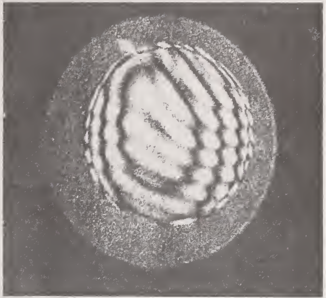
Figure 14. Photograph of the interference fringe pattern for undosed CaF 2 films on thin "stress measurement" sample. If the film is stressed, it will cause the thin, flat SiO 2 sample to bow either positively or negatively depending on whether the stress is compressive or tensile. A few fringes are visible, indicating some low residual stress in the coatings.
