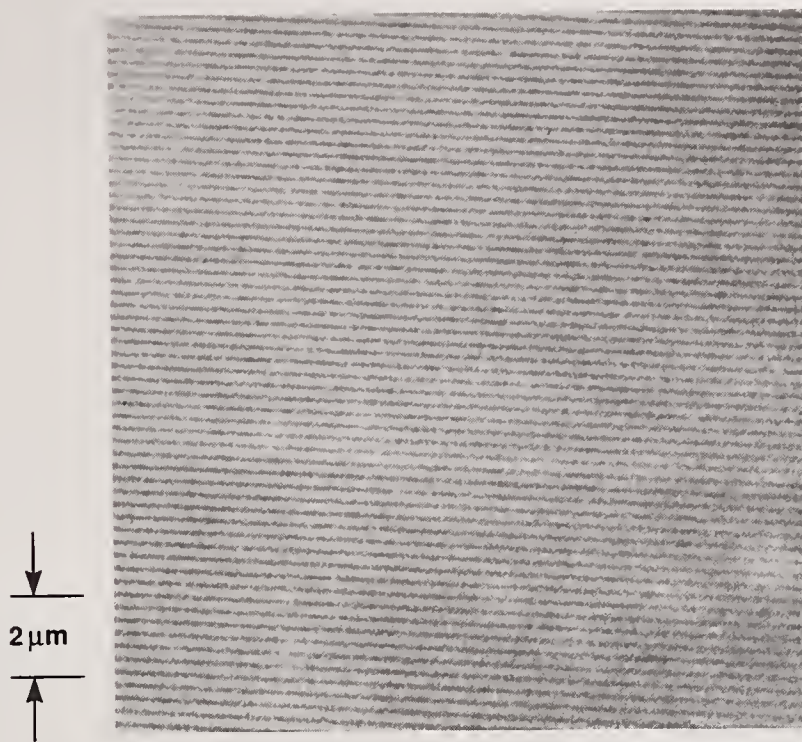
Figure 9. SEM photograph showing the cross-section of a portion of a 2000-layer Ge-doped SiO 2 coating deposited by the PICVD process. Note the 2 μm scale marker.
