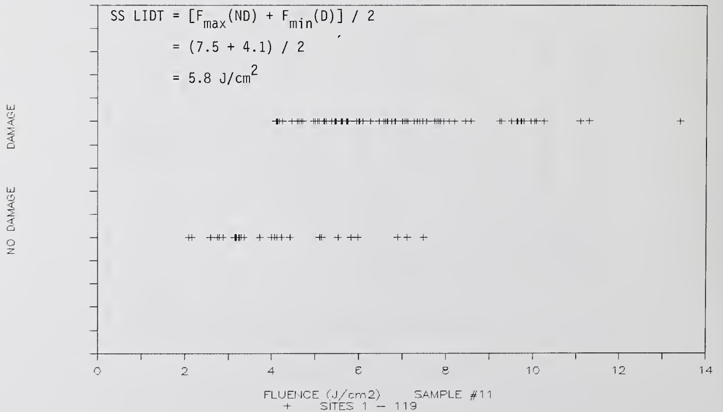
Figure 3. Typical OG-550 SS LIDT Test Results
