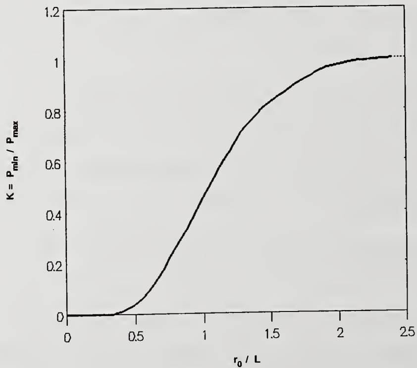
Figure 2. Plot of K versus r_0 / L for a Gaussian beam (Equation (12)).
