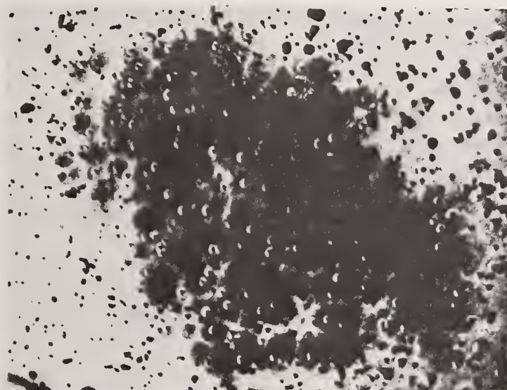
Fig. 5 : (Zr-Si) 7 - Zr sol-gel coating without laser-annealing post-treatment
