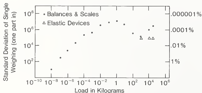
Figure 4. NIST Precision of Weighing for Mass Standards Ranging from 10 -8 to 10 4 Kilograms
