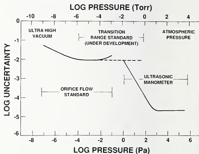
Figure 5. Uncertainties of NIST Low Pressure and Vacuum Standards
