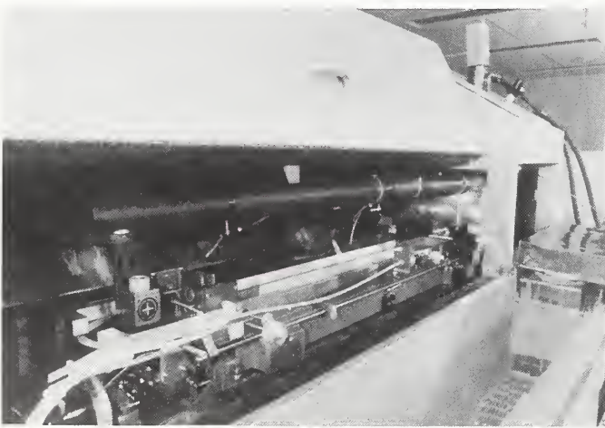
Pictured above is the line scale interferometer used for calibrations of line standards up to 1 meter in length.
