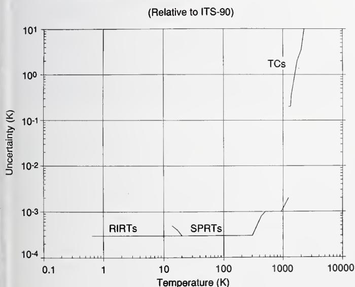
Figure 6. Uncertainties for NIST Calibration of Temperature Measuring Instruments
