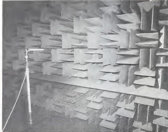
A NIST-owned half-inch microphone, the free-field response level of which has been determined by the reciprocity method, is shown with a small electrodynamic source of sound in the NIST large general-purpose anechoic chamber.
