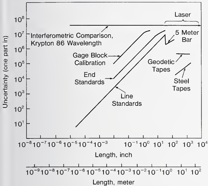
Figure 1. Accuracy of Length Measurements at NIST
