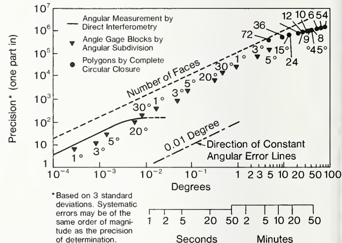
Figure 2. Precision of Angle Calibrations for Master Angle Gage Blocks and Polygons
