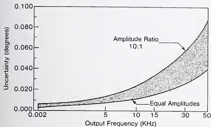
Figure 11. Estimated Total Uncertainties of the NIST Phase Angle Calibration Standard
