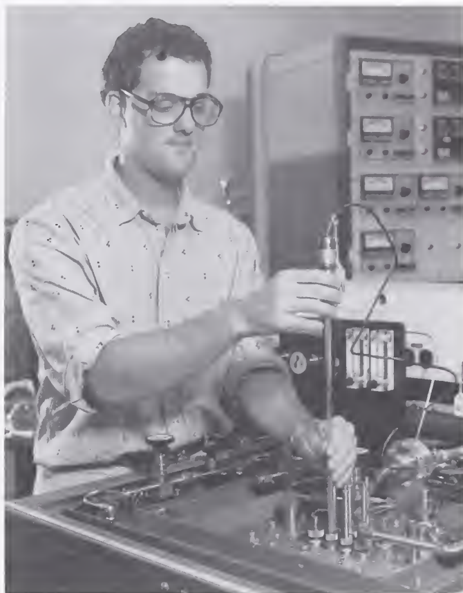
Gregory Strouse is preparing to insert an SPRT into the argon triple-point apparatus. The argon Triple-point temperature is used in the calibration of SPRTs on the ITS-90.
