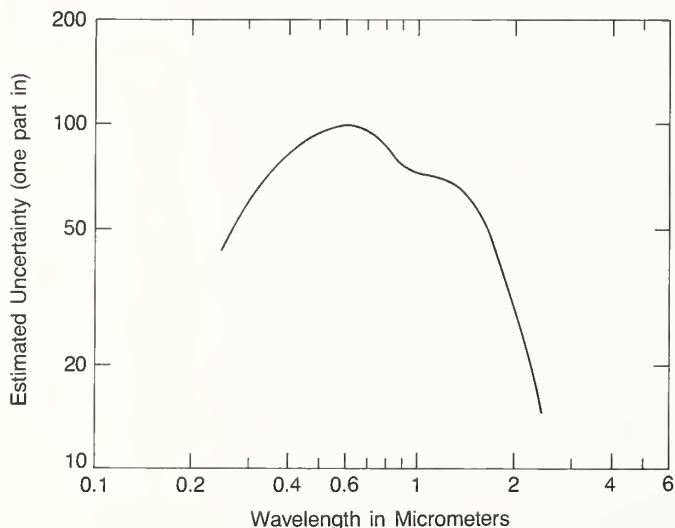
Figure 8. Uncertainties for NIST Spectral Irradiance Calibrations of Type FEL Lamps
