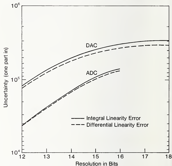
Figure 10. Uncertainty for NIST Data Converter Test System for Resolutions from 12-18 Bits
