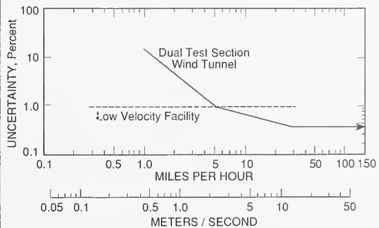
Figure 3. Total Uncertainty for the NIST Airspeed Measurements Capability.
