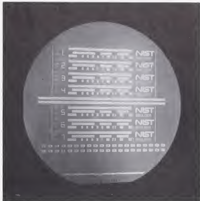
Gallium arsenide wafer on which NIST has fabricated standard transmission lines for the calibration of MMIC (monolithic microwave/millimeter-wave integrated circuit) wafer probe stations from 50 MHz to 40 GHz. The lines are of coplanar configuration from gold films patterned on the wafer surface.
