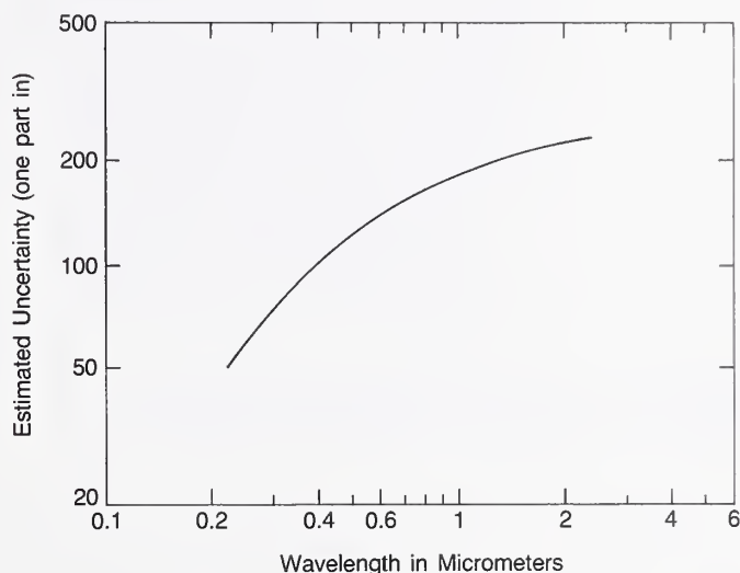
Figure 7. Uncertainties for NIST Spectral Radiance Calibrations
