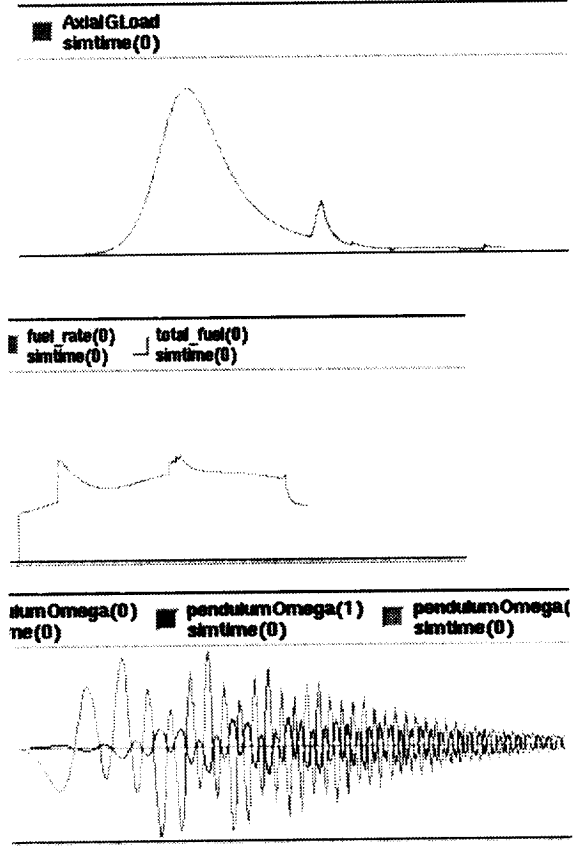
Figure 13. DSENDs Simulation Data Examples for G-Load, Fuel-Consumption, and Parachute Angular Motion.
