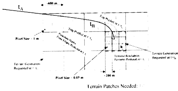
Fig 14. DSEDS Example Usage of Terrain During Spacecraft EDL.
