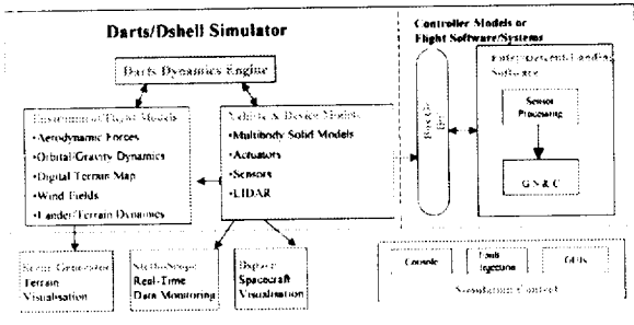
Figure 9. DSEDS Block Diagram.
