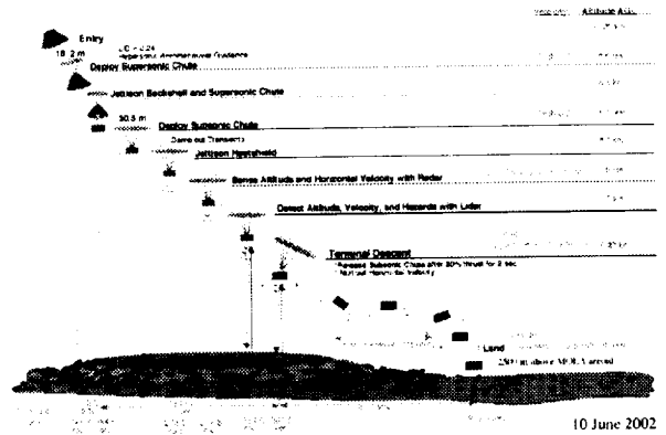
Figure 1. MSL Lander Entry, Descent and Landing Sequence.
