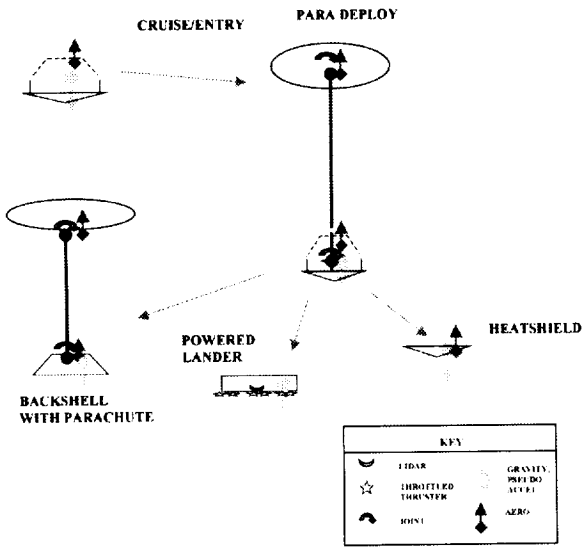
Figure 11. DSENDs Multibody Models for Flight Elements.
