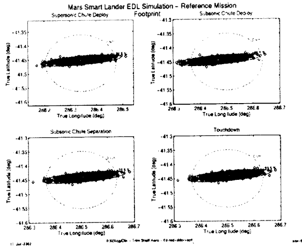
Figure 7. Sample Monte Carlo Results of Footprints Throughout EDL (Trim Shelf Configuration).
