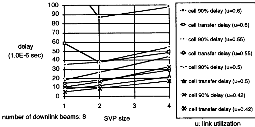
Figure D-17. Cell 90 Percent Delay and Cell Transfer Delay vs. SVP Size for Different Input Link Utilization
