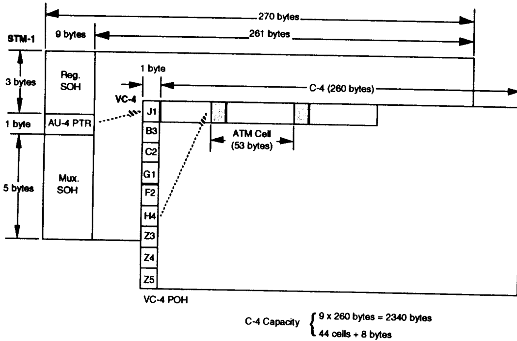
Figure 2-6. STM-1 Frame Format
