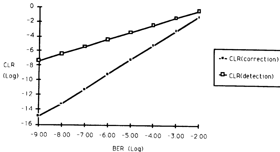
Figure 5-21. Cell Loss Ratio vs. Bit Error Rate for Different Operational Modes
