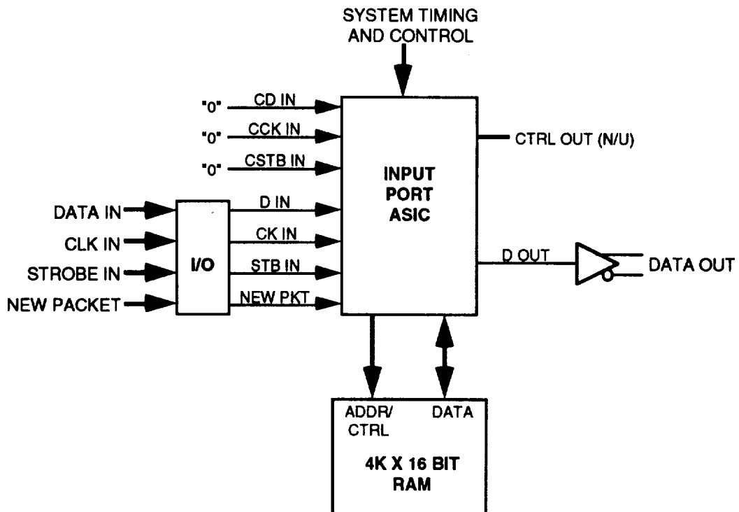
Figure 7-14. Output Port Block Diagram
