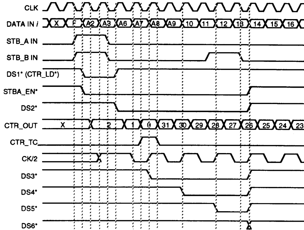
Figure 7-88a. DS2* to DS6* Generation Timing Diagram (Type 1)
