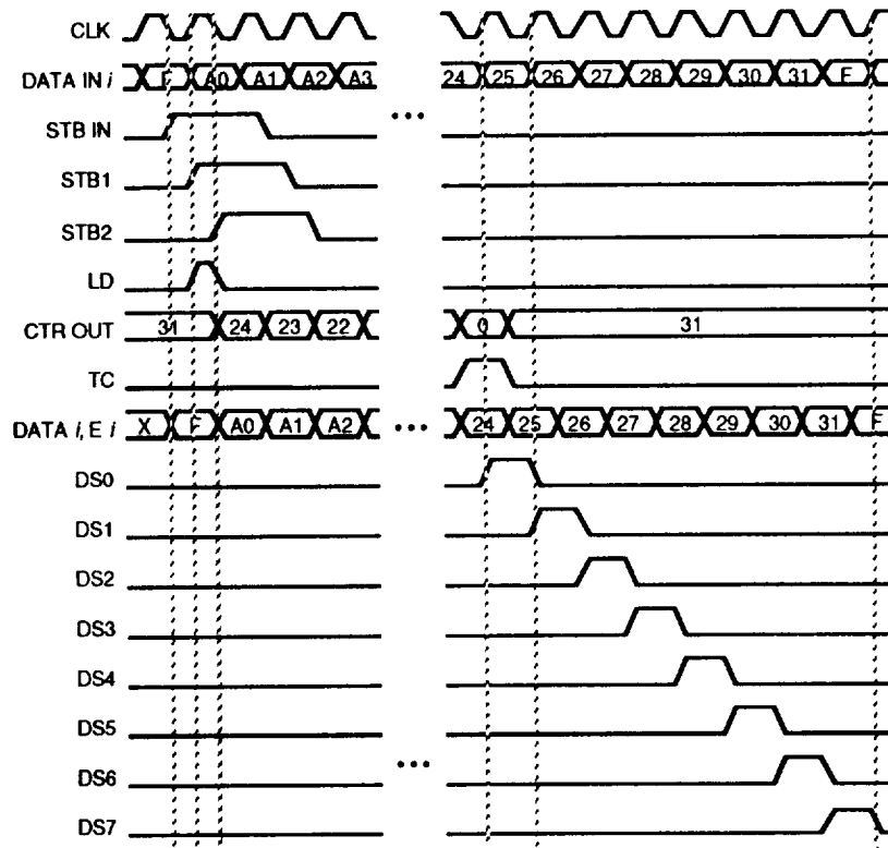
Figure 7-96b. Address Filter Timing Diagram (M1M0 = 01)
