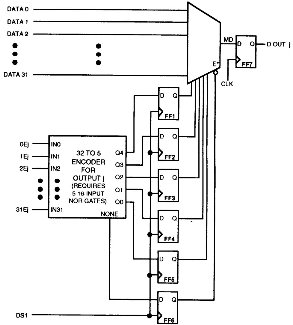
Figure 7-97. Output Selection Block Diagram
