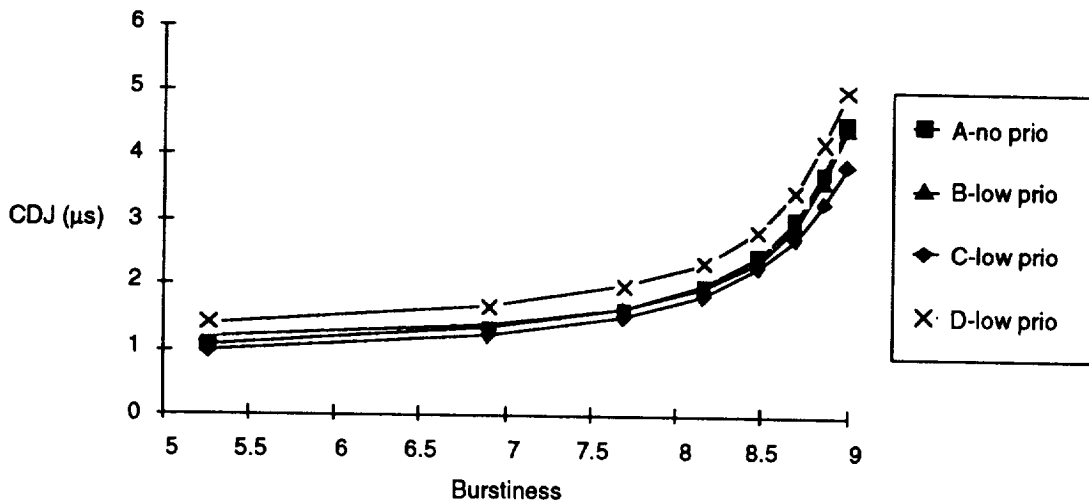
Figure C-39. Cell Delay Jitter of Low Priority Cells vs. Burstiness for Different Models
