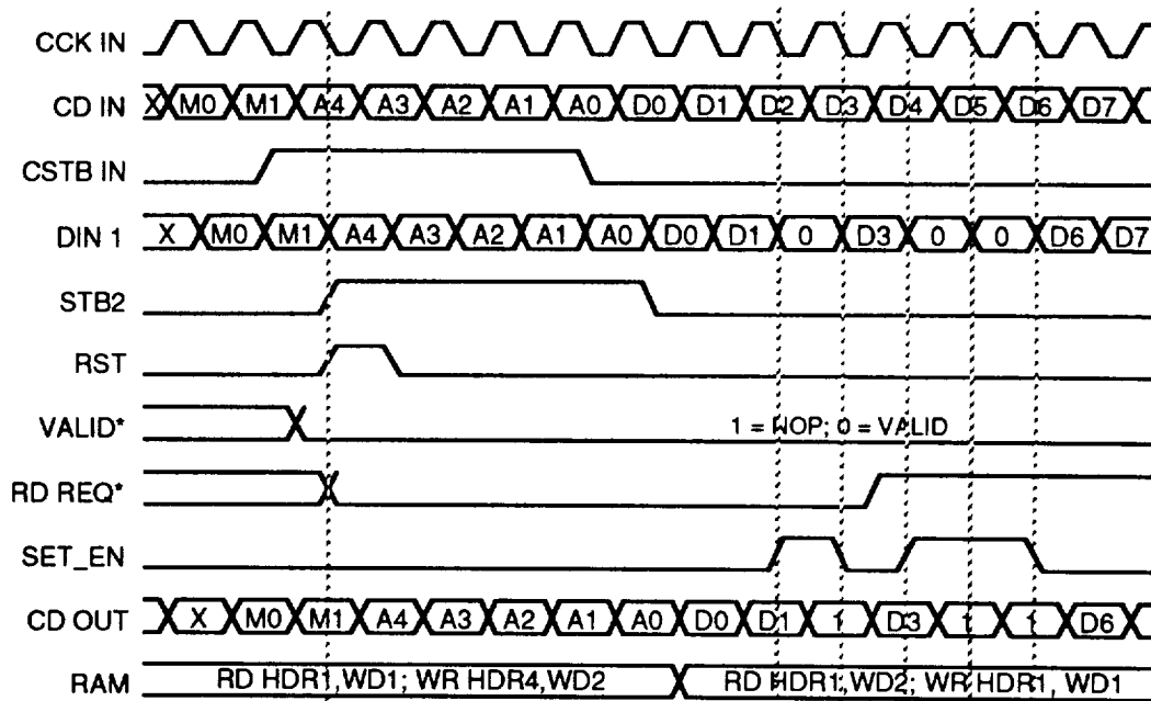
Figure 7-72a. Output Port Selection Timing Diagram (a)
