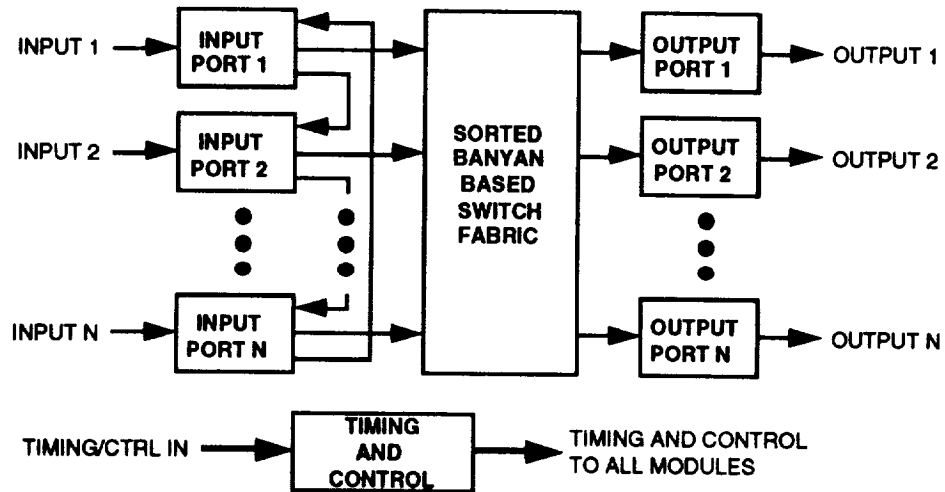
Figure 7-1. Sorted Banyan Network Block Diagram
