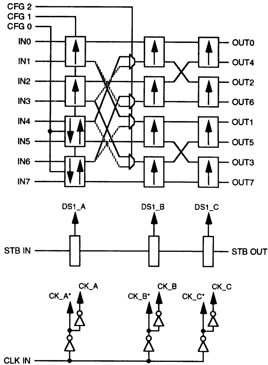
Figure 7-44. Batcher ASIC Block Diagram
