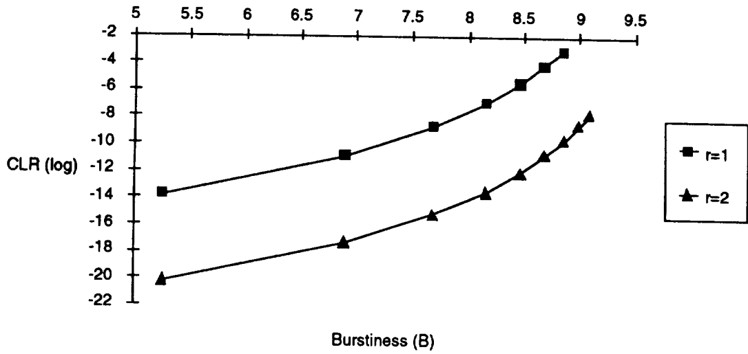
Figure C-9. Cell Loss Ratio vs. Burstiness for Different Output Transmission Rates
