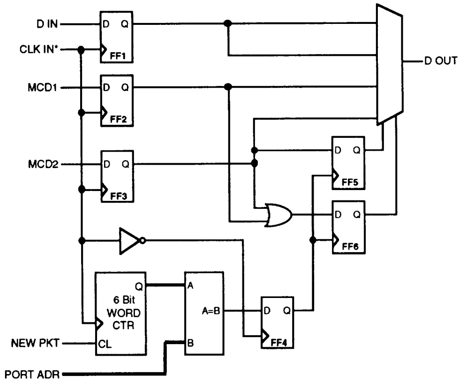
Figure 7-101. Input Data Selector Block Diagram
