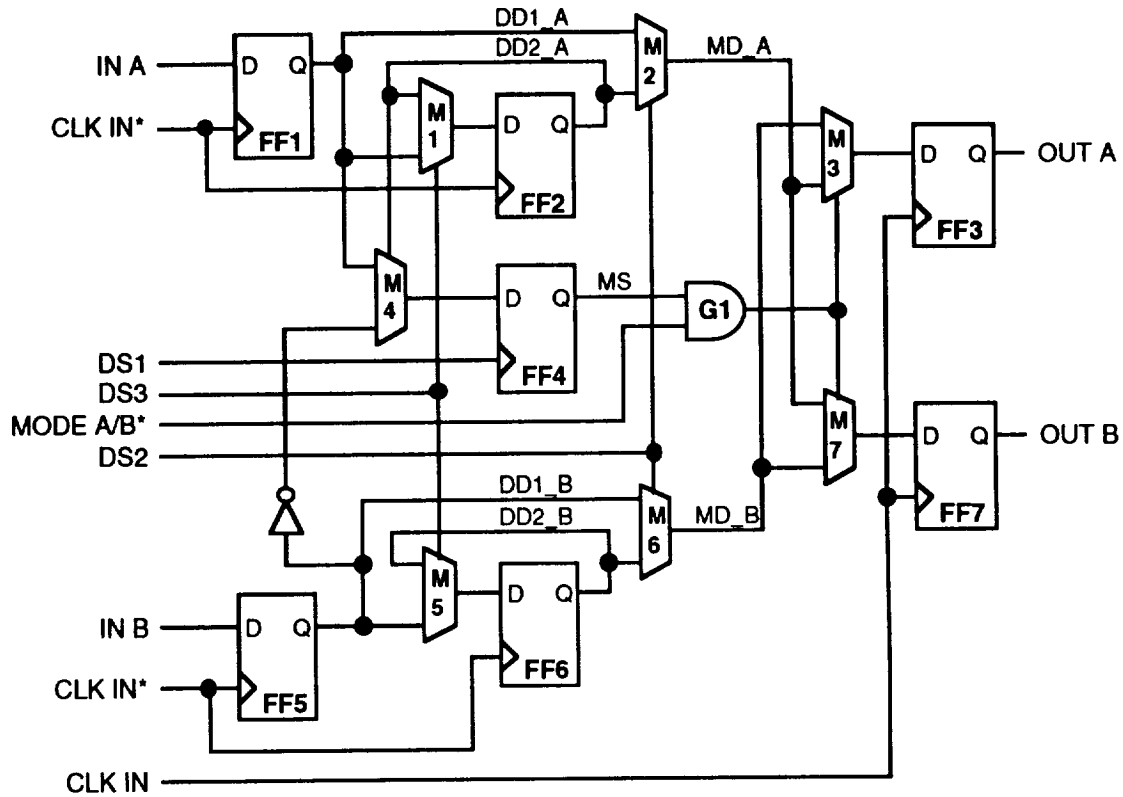
Figure 7-37. Banyan Switching Cell Detailed Block Diagram
