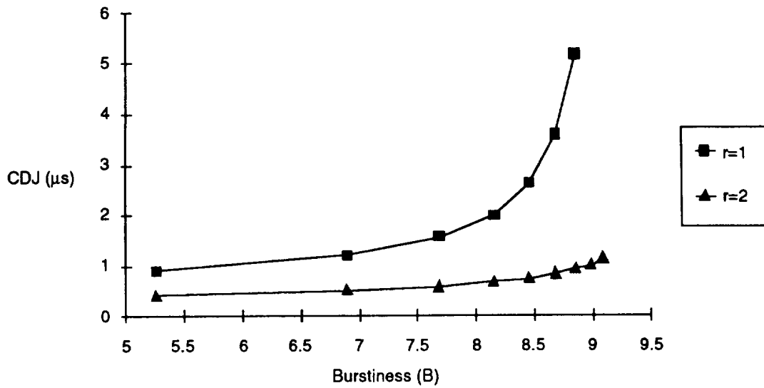
Figure C-11. Cell Delay Jitter vs. Burstiness for Different Output Transmission Rates
