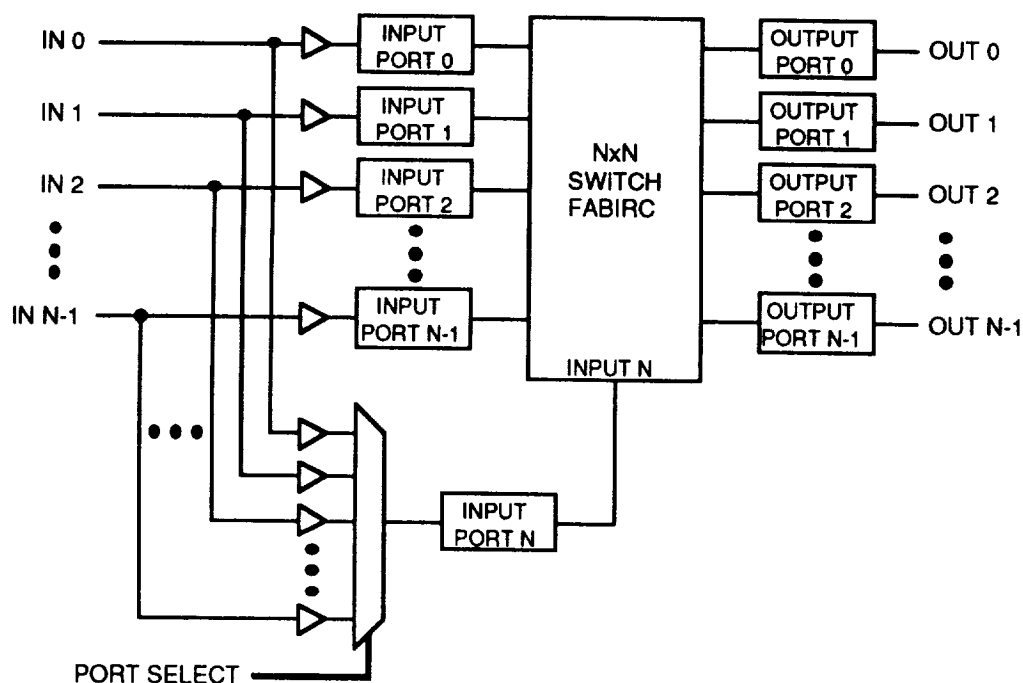
Figure 7-103. 1-For-N Input Port Redundancy Block Diagram
