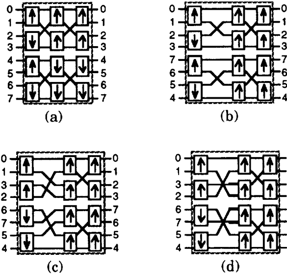
Figure 7-42. MODE A ASIC Reconfiguration Steps
