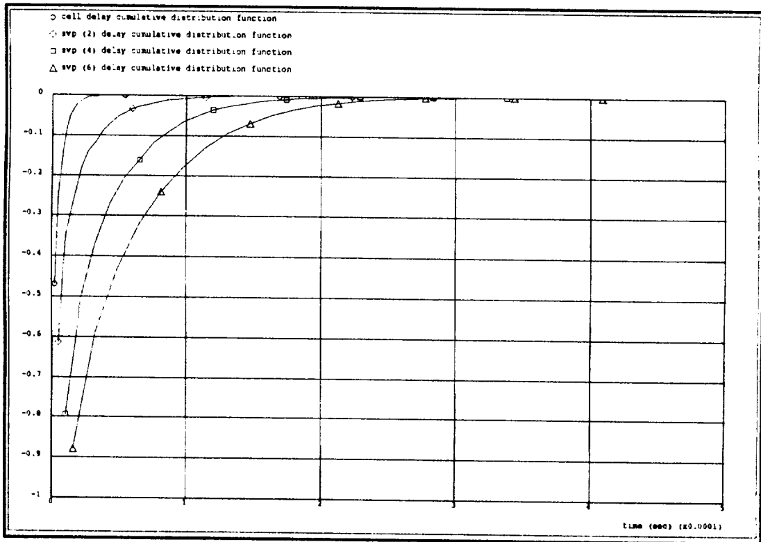
Figure D-6b. Cell Delay Cumulative Distribution for Different SVP Sizes When the Output Link Utilization is 80 Percent
