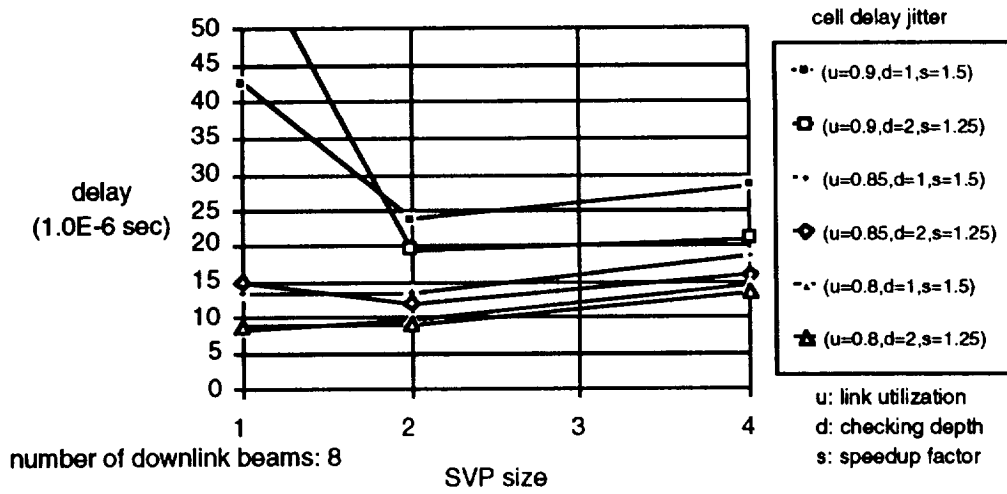
Figure D-25. Cell Delay Jitter vs. SVP Size for Different Link Utilization
