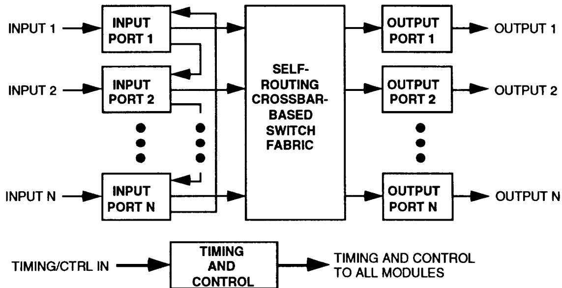
Figure 7-54. Self-Routing Crossbar-Based Network Block Diagram
