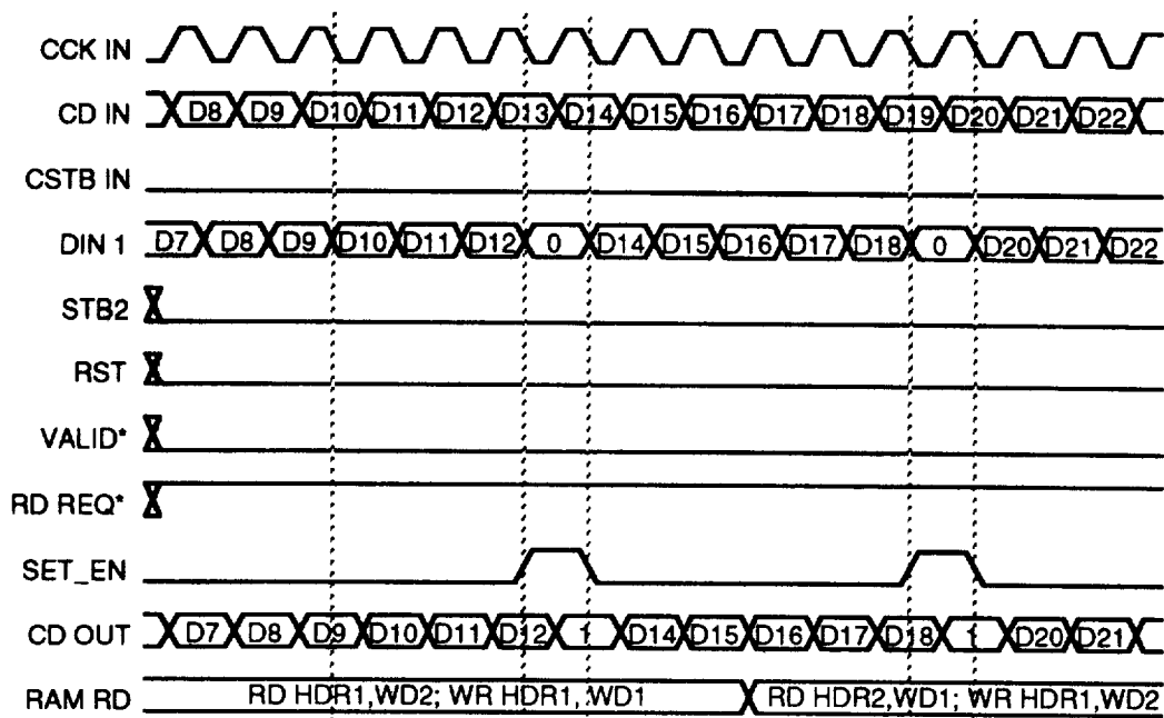
Figure 7-72b. Output Port Selection Timing Diagram (b)
