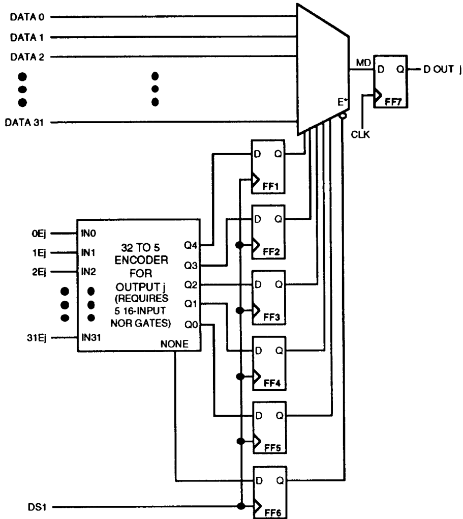
Figure 7-61. Output Selection Block Diagram
