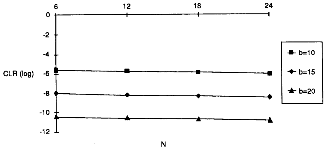
Figure C-21. Cell Loss Ratio vs. Number of Input Lines for Different Buffer Sizes
