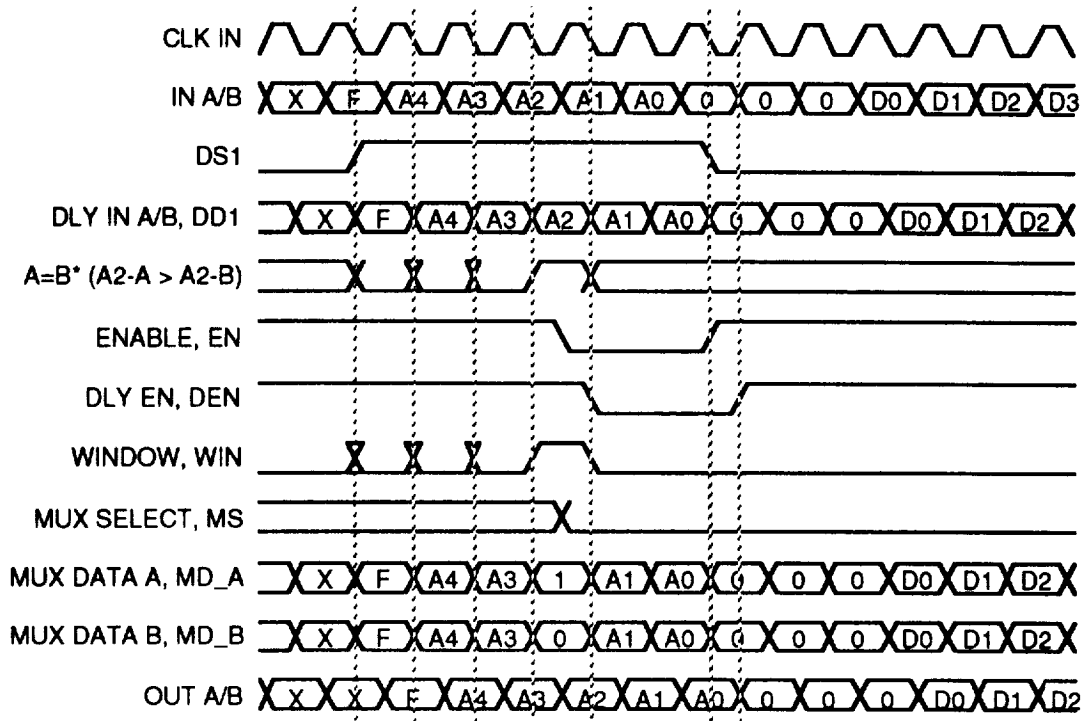
Figure 7-51. Batcher Sorting Cell Timing Diagram
