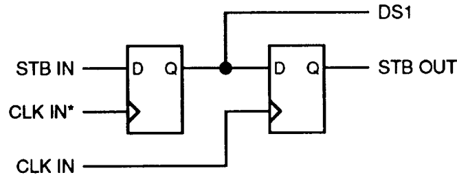
Figure 7-52. Strobe Generation Block Diagram
