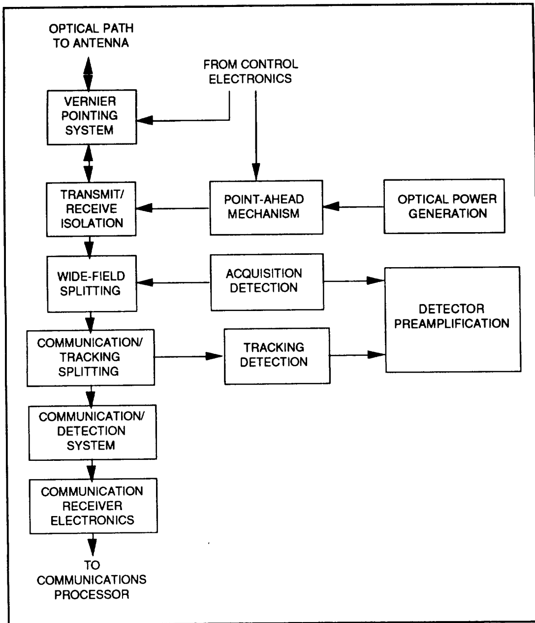
Figure B-7. Major Aspects of Focal Plane Assembly
