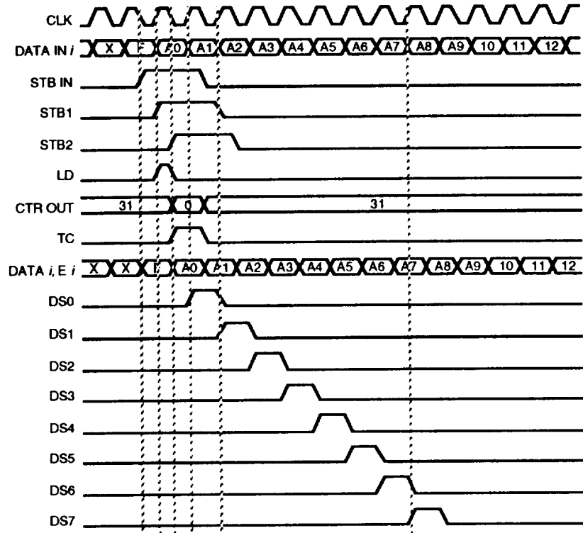
Figure 7-96a. Address Filter Timing Diagram (M1M0 = 00)
