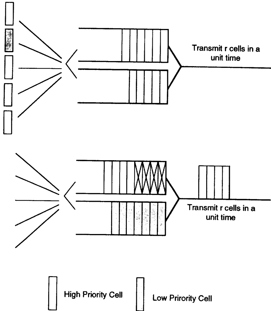
Figure C-6. Cell Priority Concept in Model C
