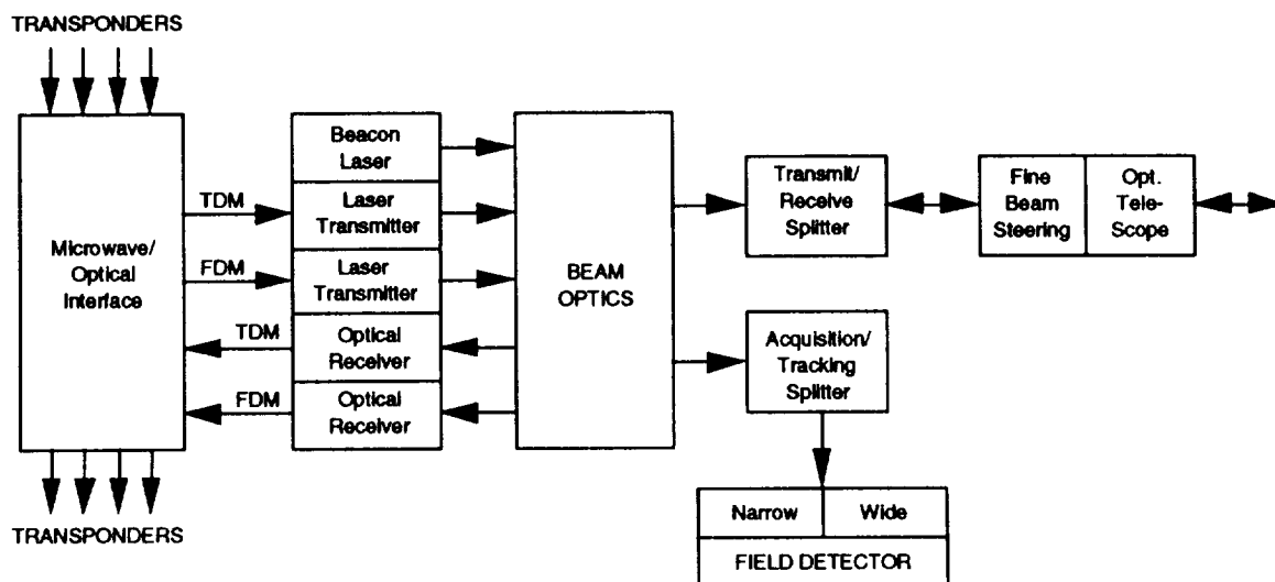
Figure B-1. Baseline Configuration of Optical Satellite Link Payload
