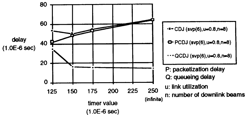
Figure D-15. Cell Delay Jitter vs. Time-out Value When the Input Link Utilization is 80 Percent
