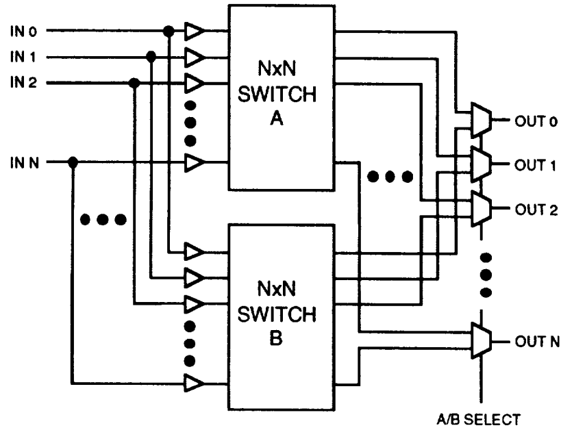
Figure 7-102. 1-For-1 Switch Network Redundancy Block Diagram
