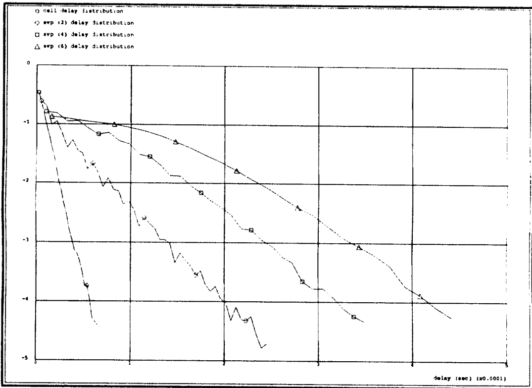
Figure D-6a. Cell Delay Distribution for Different SVP Sizes When the Output Link Utilization is 80 Percent
