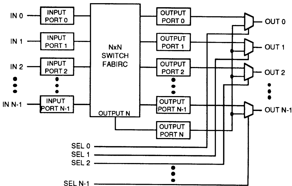
Figure 7-106. 1-For-N Output Port Redundancy Block Diagram
