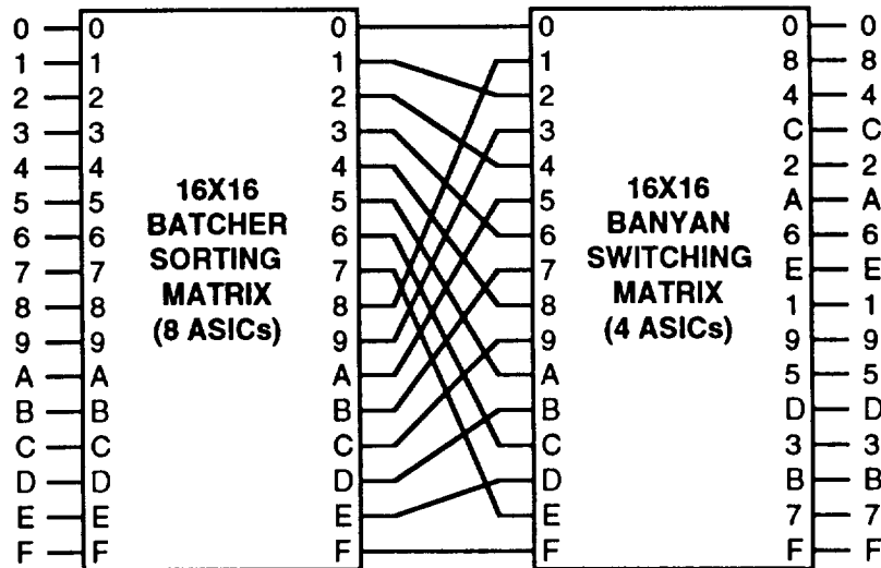
Figure 7-31. 16 x 16 Sorted Banyan Switch Fabric
