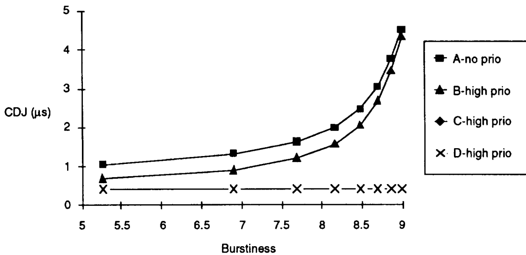
Figure C-37. Cell Delay Jitter of High Priority Cells vs. Burstiness for Different Models
