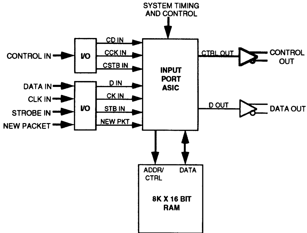
Figure 7-4. Sorted Banyan Input Port Block Diagram
