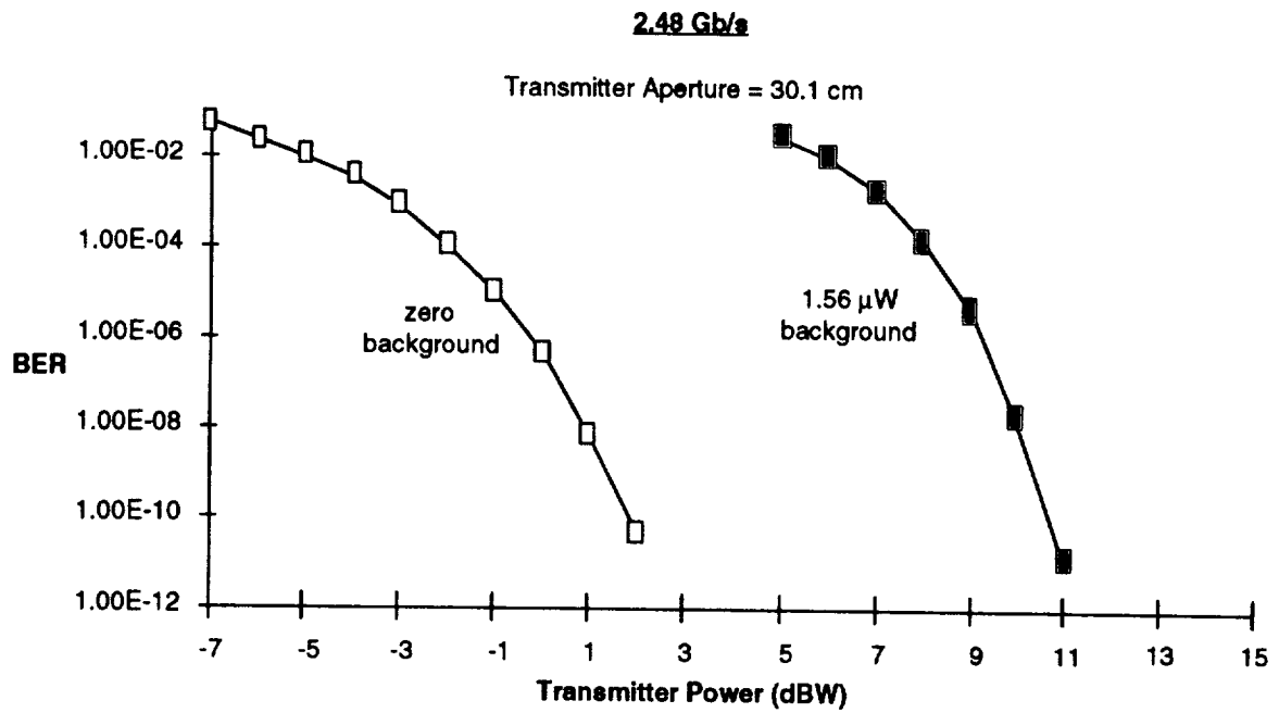
Figure B-6. BER as a function of transmitter power with & without background radiation
