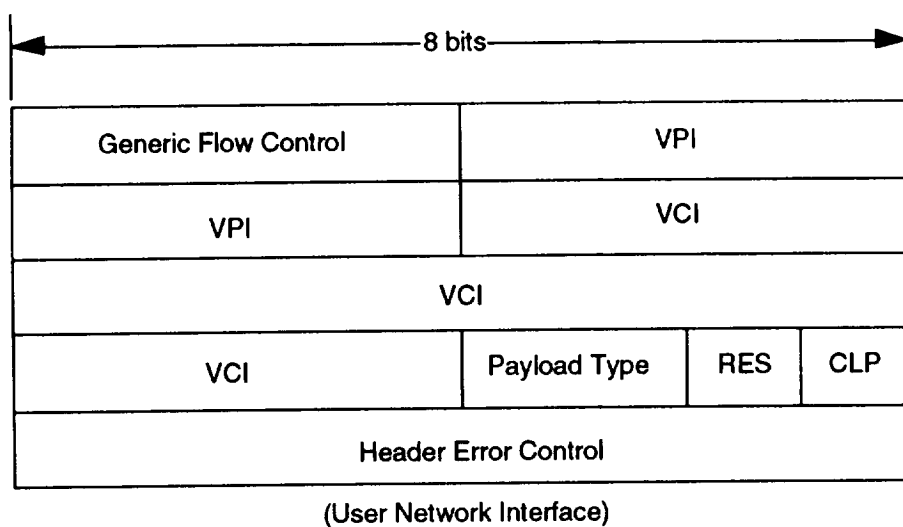
Figure 2-4. UNI ATM Cell Format
