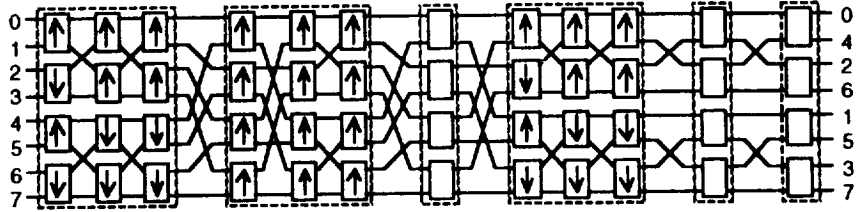
Figure 7-75. 8 x 8 Multicast Banyan Switch Fabric
