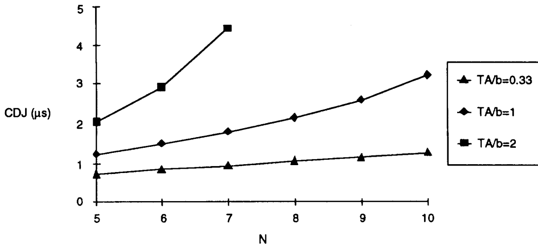
Figure C-26. Cell Delay Jitter vs. Number of Input Lines for Different Ratios of Average Burst Size and Buffer Size
