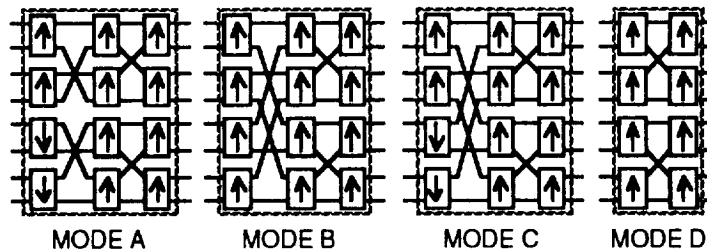
Figure 7-43. Batcher Configurations To Be Implemented In ASIC
