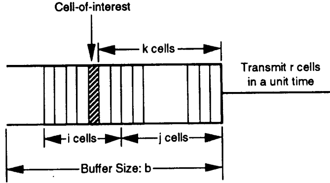
Figure C-4. Cell Transfer Delay for Cell k+1
