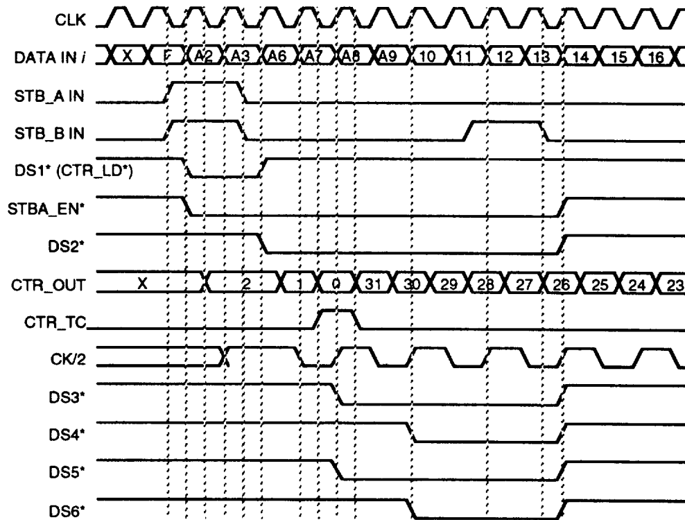
Figure 7-88b. DS2* to DS6* Generation Timing Diagram (Type 2)
