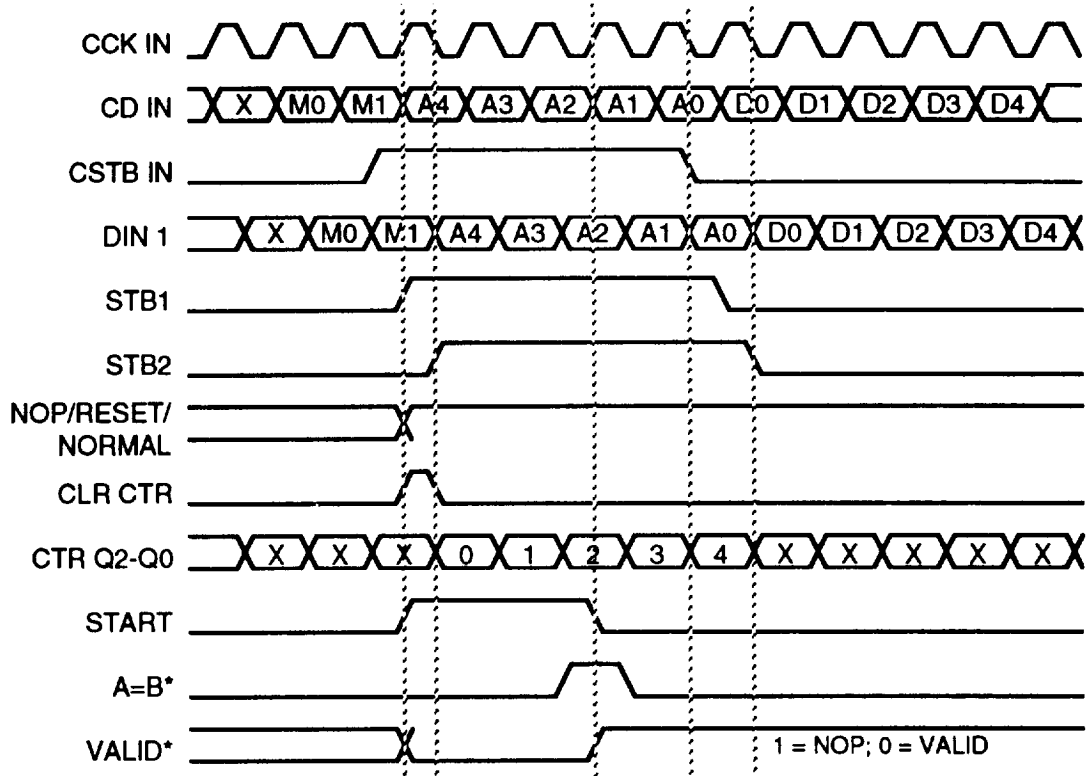
Figure 7-10. Mode Control And Address Filter Timing Diagram
