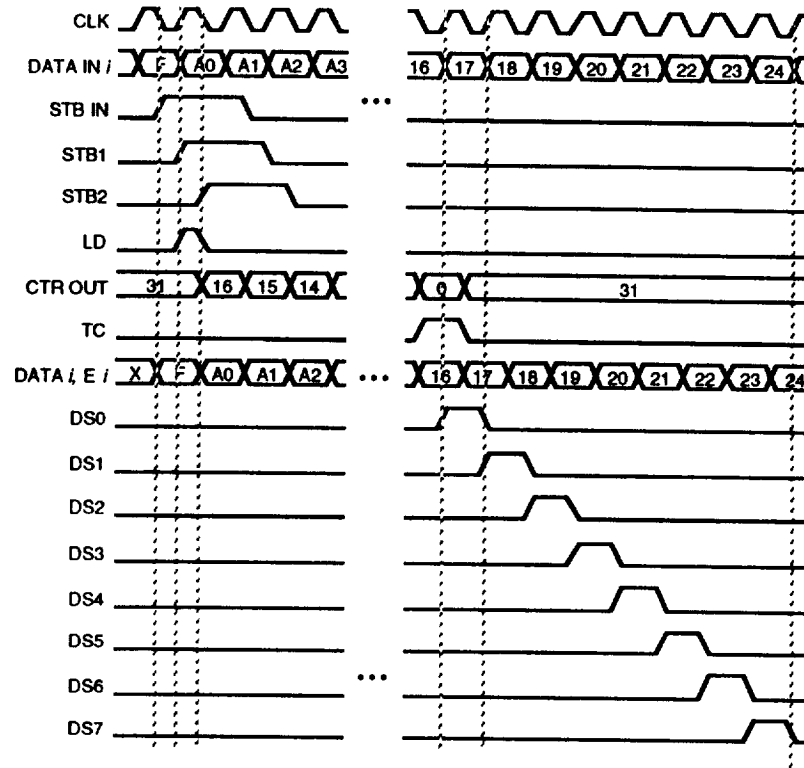
Figure 7-96c. Address Filter Timing Diagram ( M1M0 = 10 )
