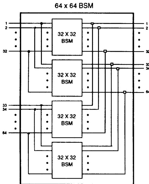
Figure 4-16. A 64 x 64 Baseband Switch Matrix Composed of 32 x 32 Switch Matrices
