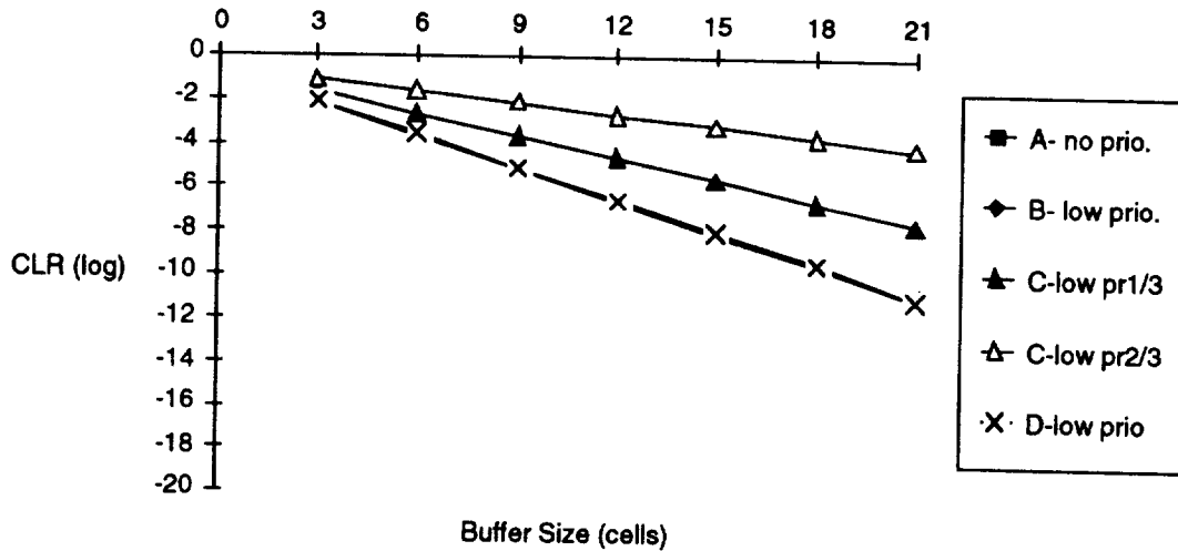
Figure C-28. Cell Loss Ratio of Low Priority Cells vs. Buffer Size for Different Models
