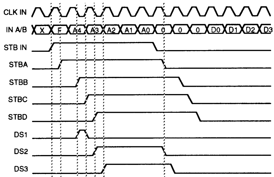
Figure 7-40. Strobe Generation Timing Diagram
