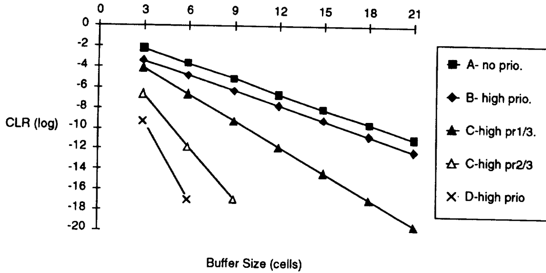
Figure C-27. Cell Loss Ratio of High Priority Cells vs. Buffer Size for Different Models
