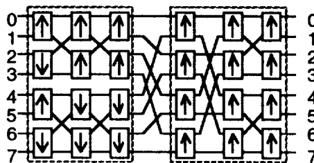
Figure 7-25. 8 x 8 Batcher Matrix Implementation
