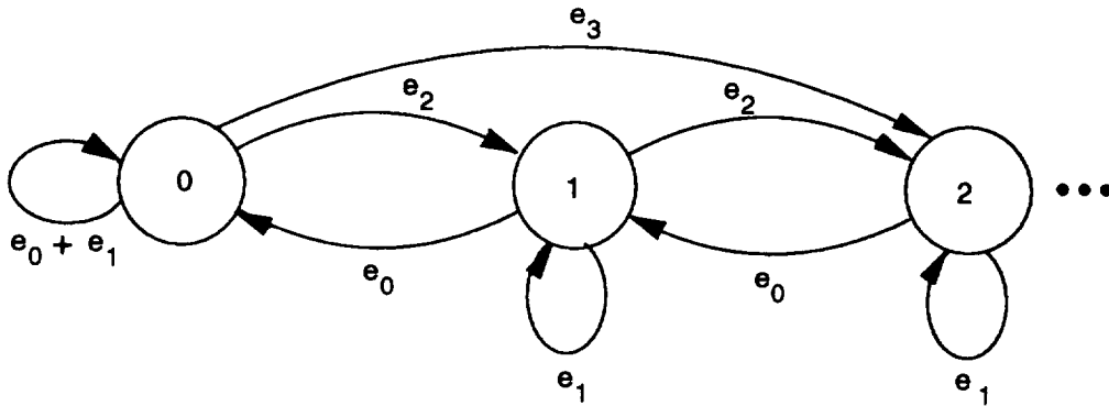
Figure C-3. Discrete-Time Markovian Chain State Transition for the Buffer Occupancy
