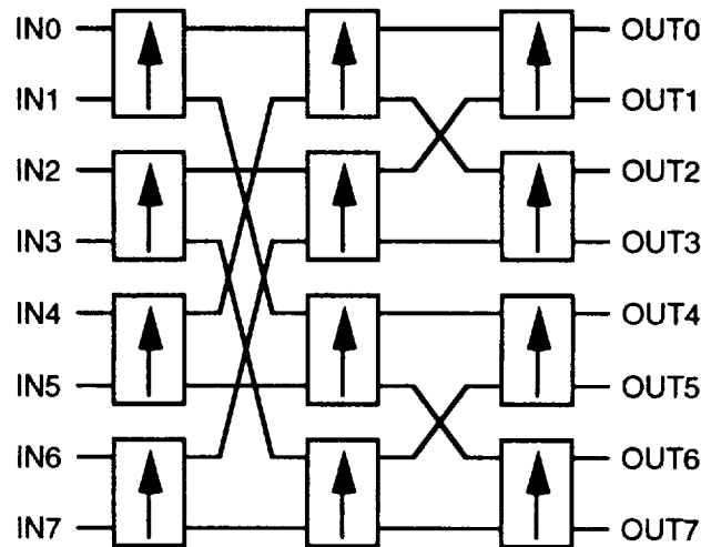
Figure 7-46. MODE B ASIC Configuration (CFG 2,1,0 = "010")
