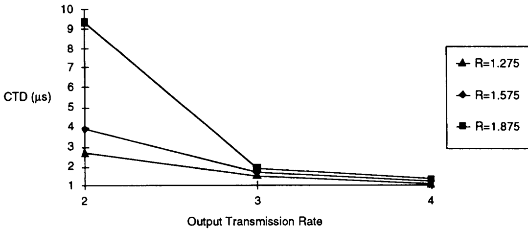
Figure C-19. Cell Transfer Delay vs. Output Transmission Rate for Different Average Arrival Rates
