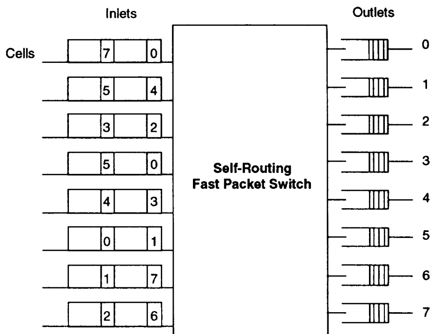
Figure C-8. An 8 x 8 Fast Packet Switch with Output Buffering
