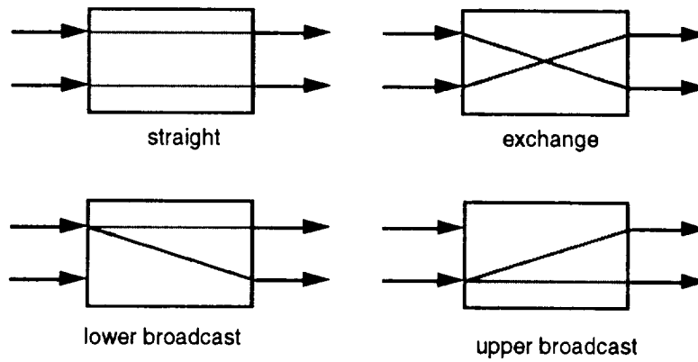
Figure 6-1. Four States of a 2 x 2 Self-Routing Switching Element
