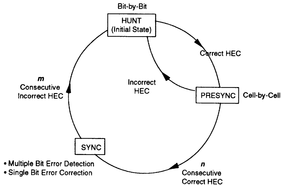
Figure 5-17. Cell Delineation State Diagram
