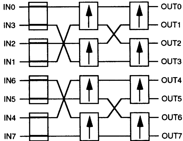
Figure 7-48. MODE D ASIC Configuration (CFG 2,1,0 = "110")
