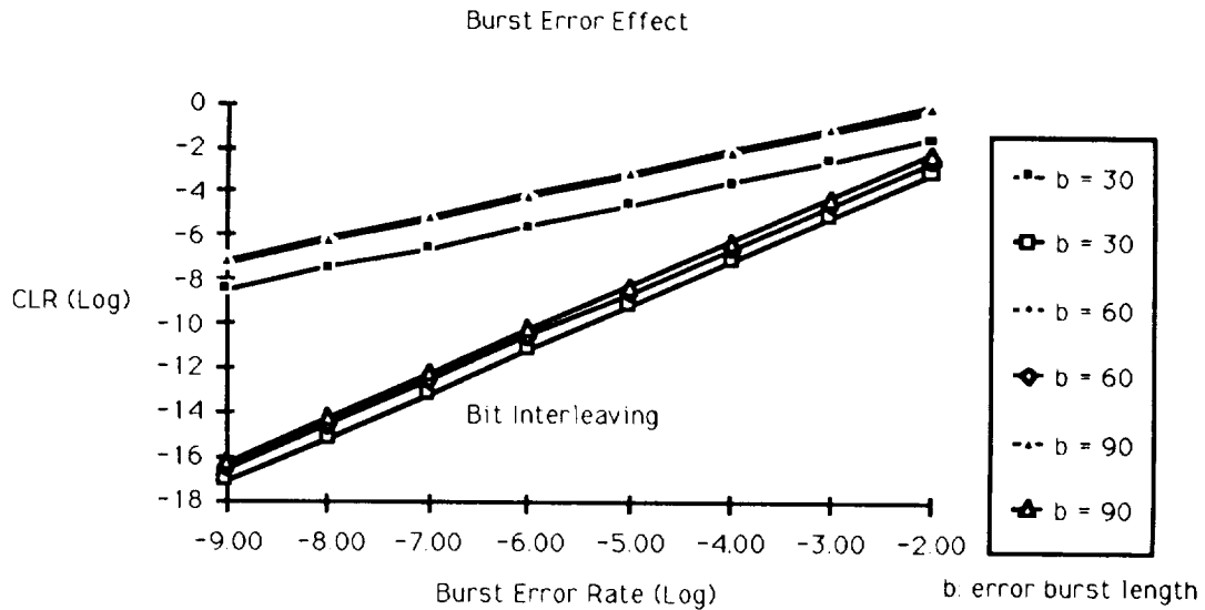
Figure 5-23. Cell Loss Ratio vs. Burst Error Rate for Different Error Burst Length
