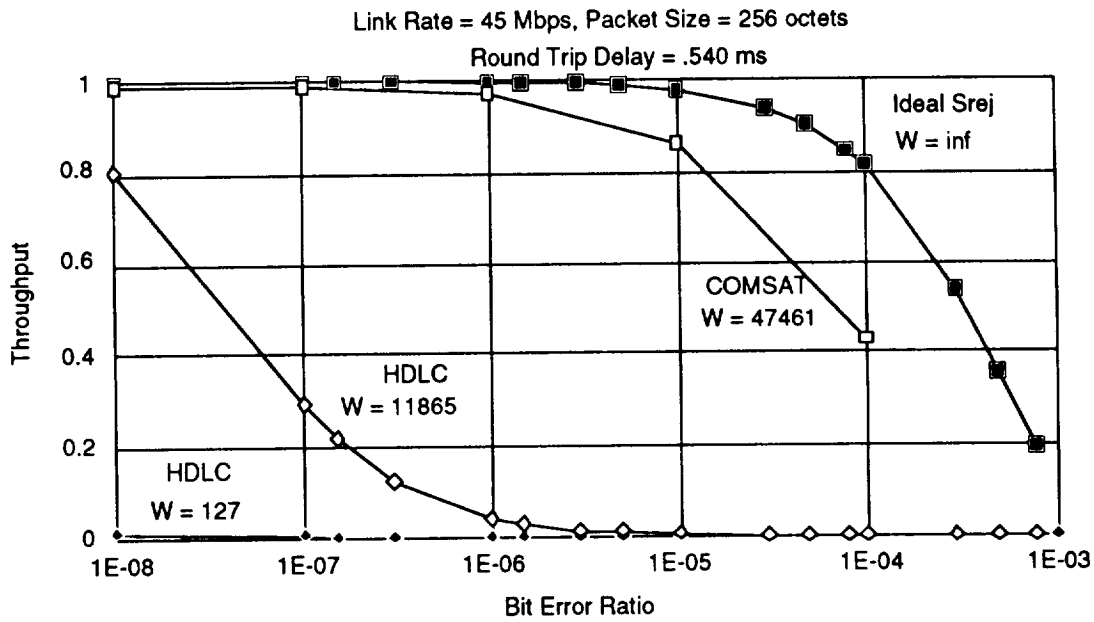
Throughput Performance
