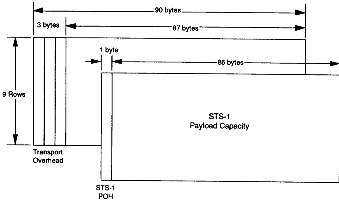
Figure 2-9. STS-1 Frame Format
