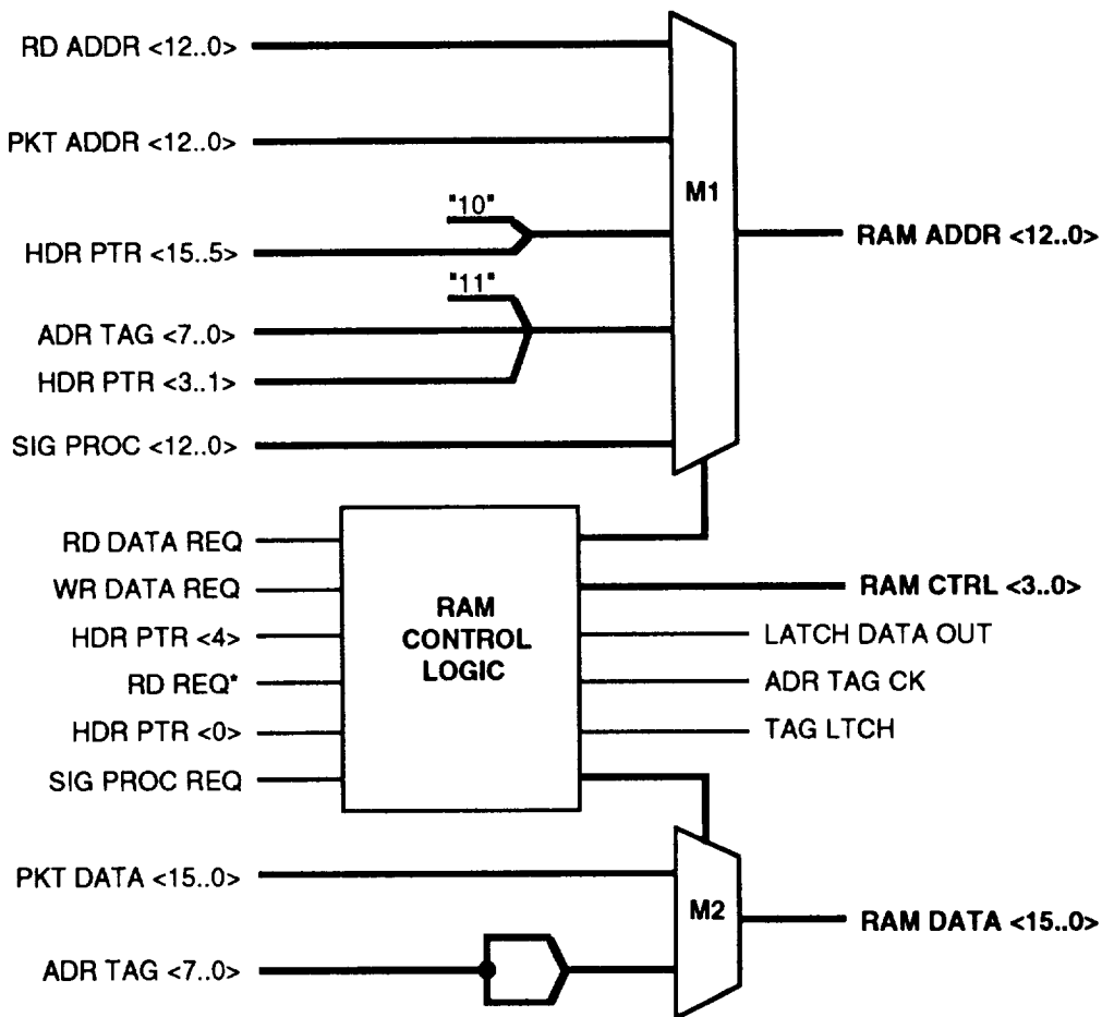
Figure 7-13. RAM Processing Block Diagram
