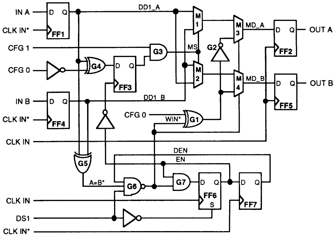
Figure 7-50. Batcher Sorting Cell Detailed Block Diagram
