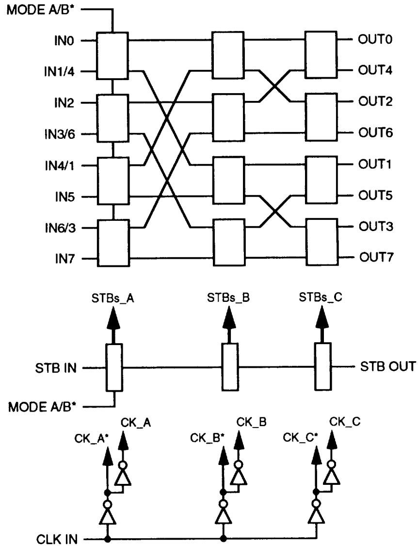
Figure 7-33. Banyan ASIC Block Diagram
