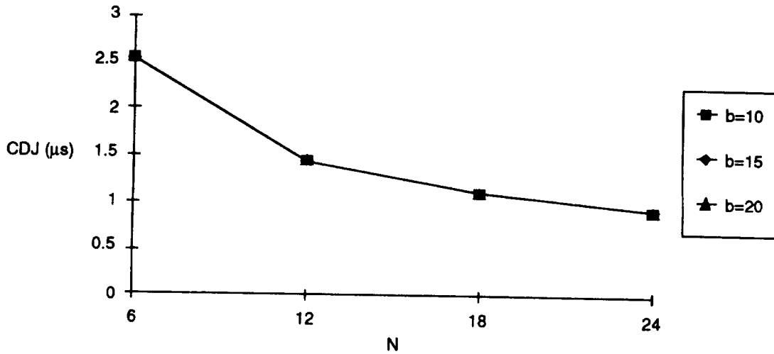
Figure C-23. Cell Delay Jitter vs. Number of Input Lines for Different Buffer Sizes
