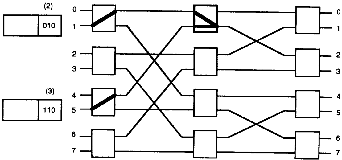
Figure 6-6. Internal Blocking
