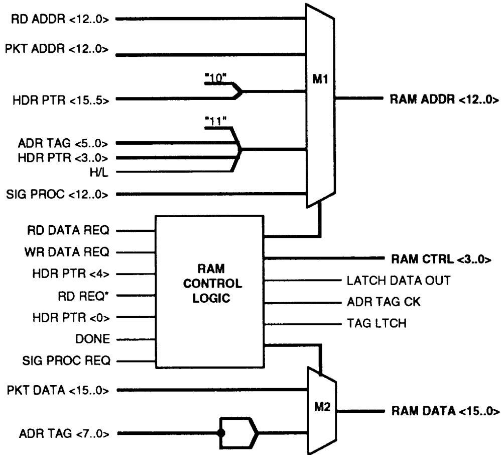
Figure 7-74. RAM Processing Block Diagram
