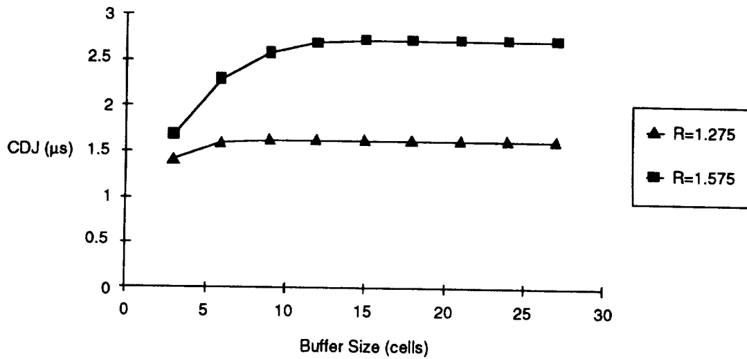
Figure C-16. Cell Delay Jitter vs. Buffer Size for Different Average Arrival Rates
