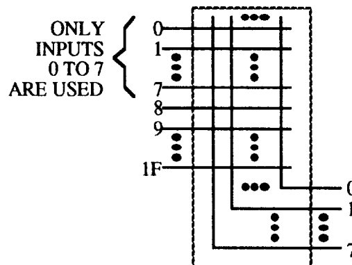
Figure 7-55. 8 x 8 Crossbar-Based Switch Fabric
