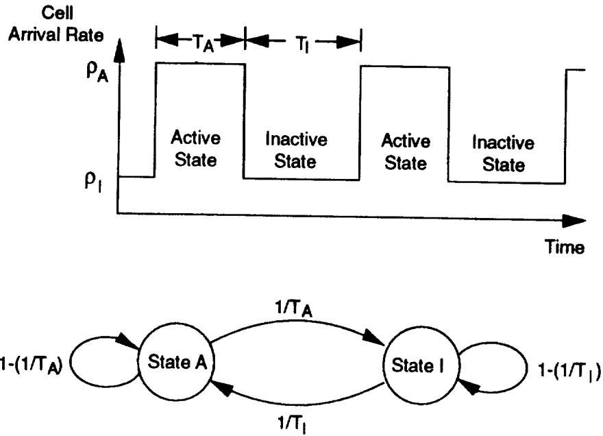
Figure C-2. Two-State Markovian Cell Arrival Model for Bursty Traffic
