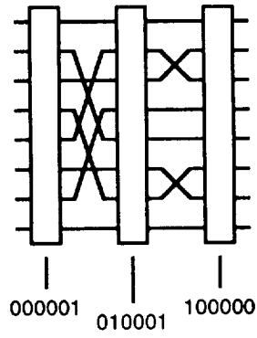
Figure 7-79. CELL POS Values for 8 x 8 Switch Fabric
