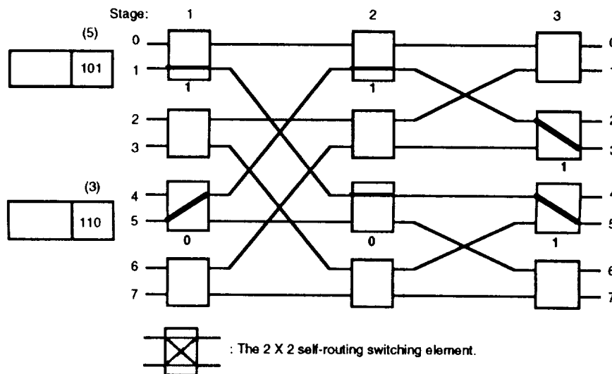
Figure 6-3. The 8 x 8 Banyan Network
