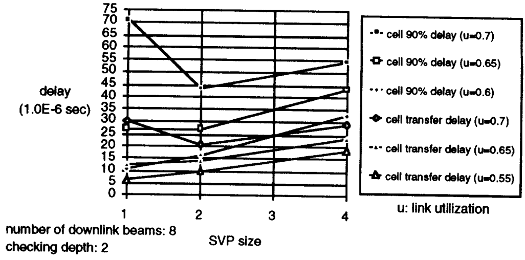
Figure D-20. Cell 90 Percent Delay and Cell Transfer Delay vs. SVP Size for Different Input Link Utilization
