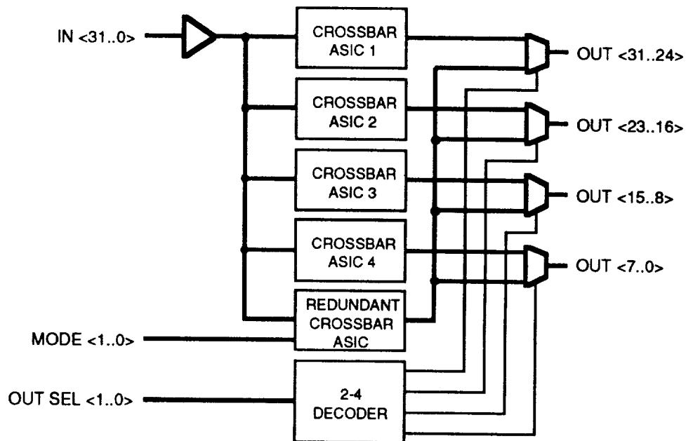
Figure 7-105. 1-For-N Switch Fabric ASICs Redundancy Block Diagram
