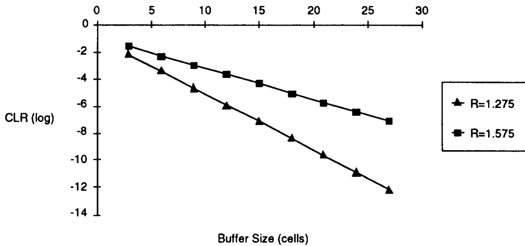
Figure C-14. Cell Loss Ratio vs. Buffer Size for Different Average Arrival Rates
