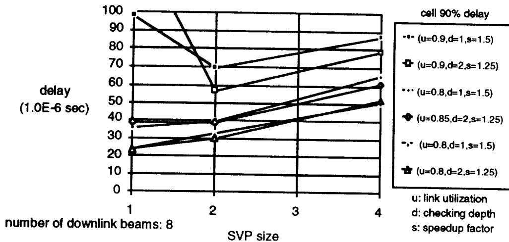
Figure D-27. Cell 90 Percent Delay vs. SVP Size for Different Link Utilization and Configurations
