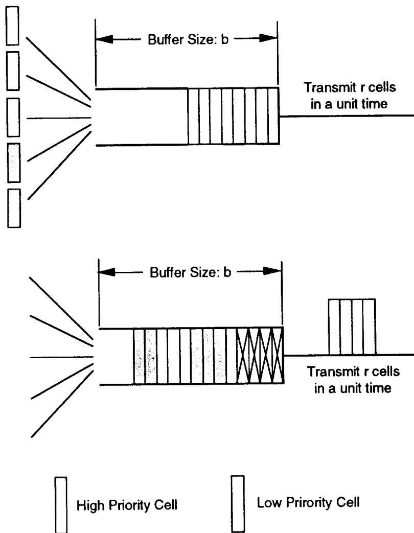
Figure C-5. Cell Priority Concept in Model B
