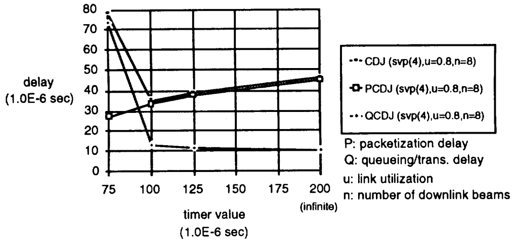
Figure D-12. Cell Delay Jitter vs. Time-out Value When the Input Link Utilization is 80 Percent
