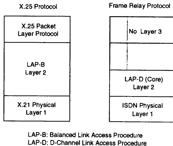
Figure 5-29. Difference Between X.25 and Frame Relay Protocols
