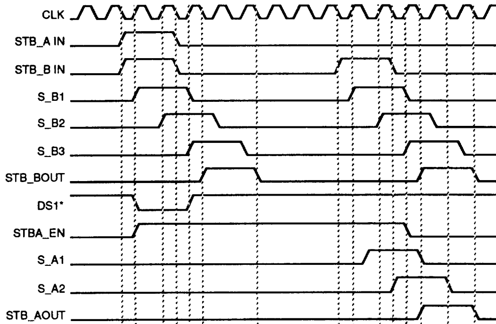
Figure 7-86. DS1*, STB_AOUT, STB_BOUT Generation Timing Diagram
