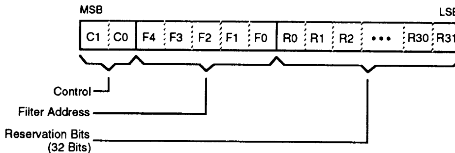
Figure 7-3. Sorted Banyan Congestion Control Message Format
