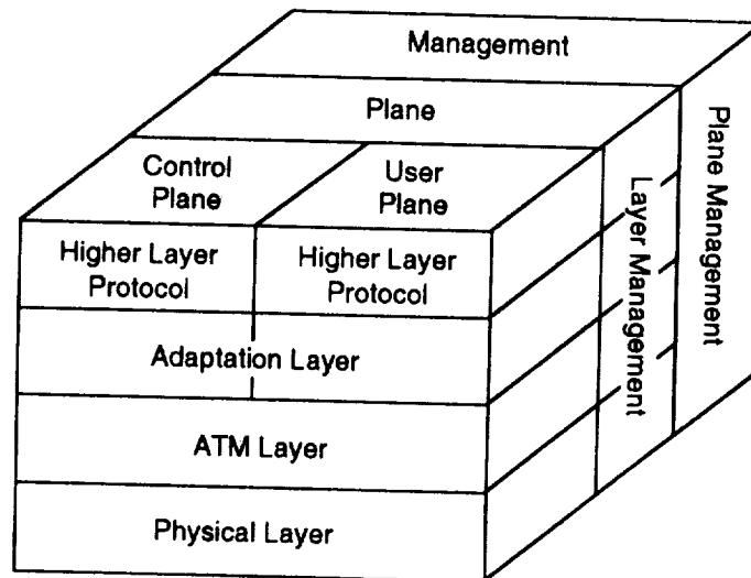
Figure 2-2. B-ISDN Protocol Reference Model
