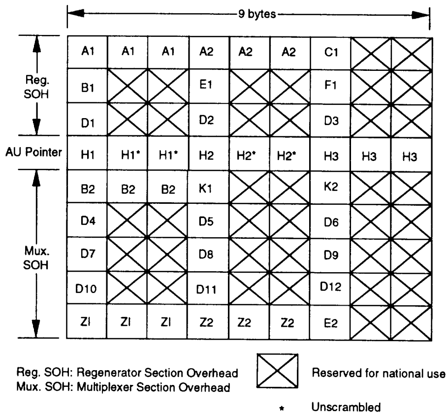
Figure 2-10. STS-3c Transport Overhead Format
