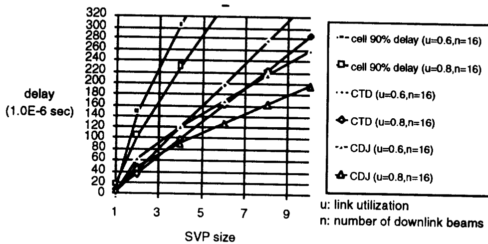
Figure D-4. Cell Delay Performance vs. SVP Sizes for Different Output Link Utilization
