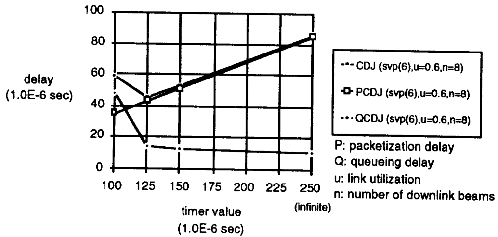
Figure D-14. Cell Delay Jitter vs. Time-out Value When the Input Link Utilization is 60 Percent
