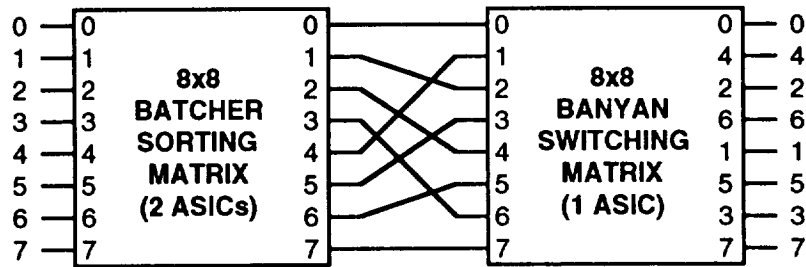
Figure 7-30. 8 x 8 Sorted Banyan Switch Fabric
