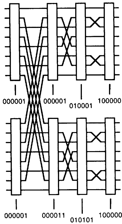
Figure 7-80. CELL POS Values for 16 x 16 Switch Fabric
