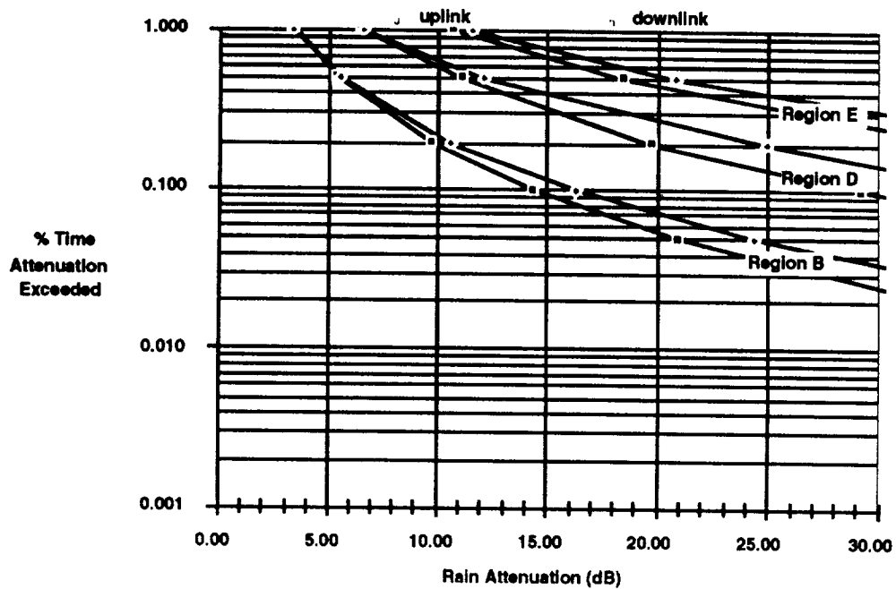
Figure A-4. Rain Attenuation at 40/50 GHz
