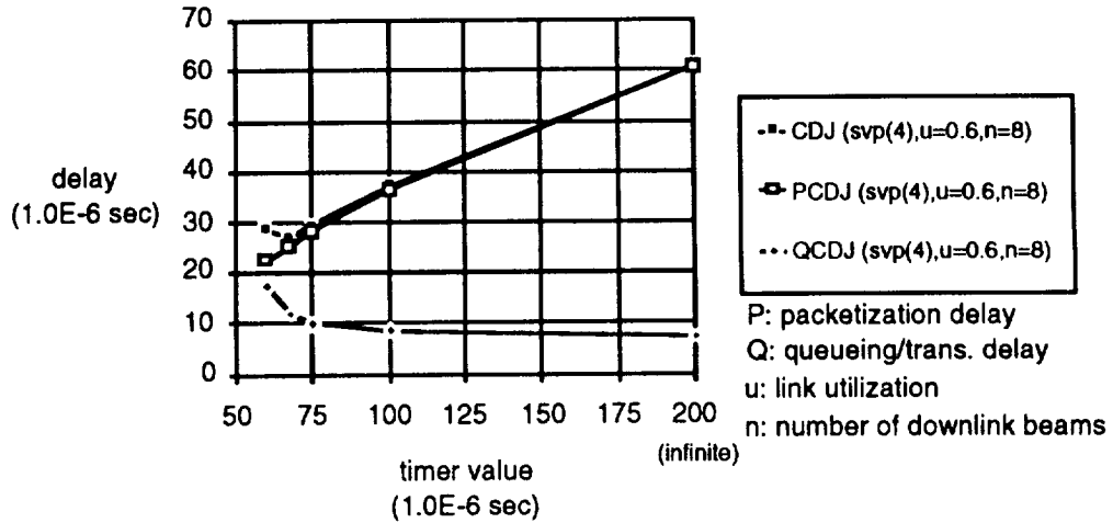
Figure D-11. Cell Delay Jitter vs. Time-out Value When the Input Link Utilization is 60 Percent
