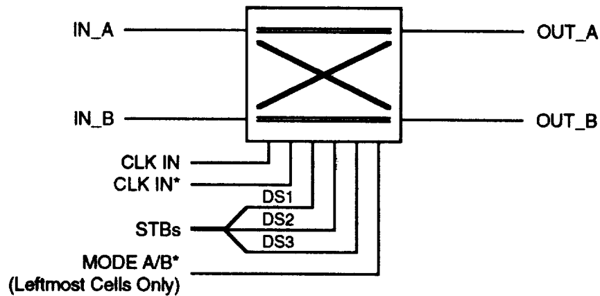
Figure 7-36. Banyan Switching Cell Block Diagram
