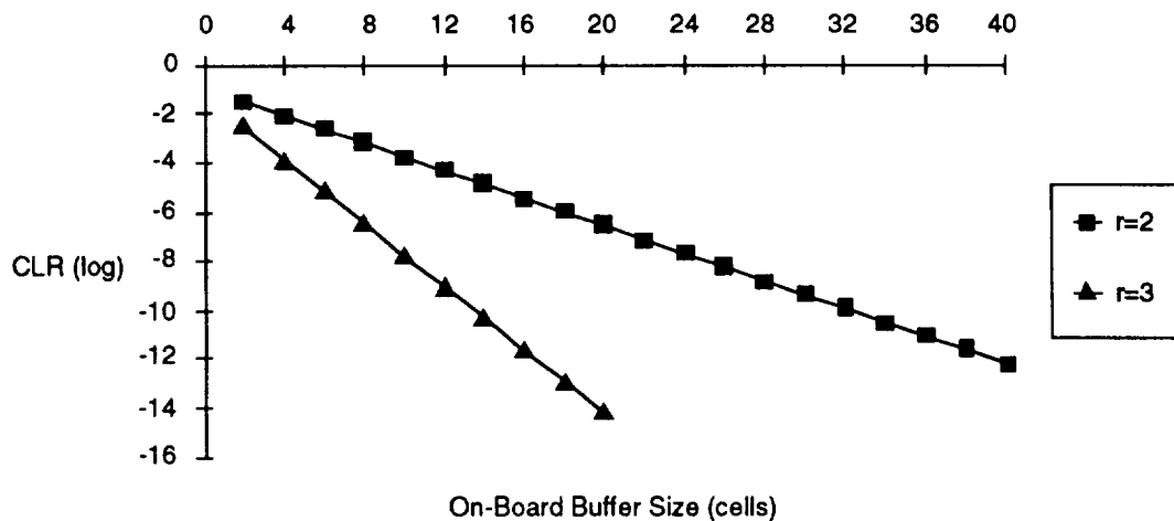
Figure C-40. Space Segment Cell Loss Ratio vs. On-Board Buffer Size for Different Output Transmission Rates
