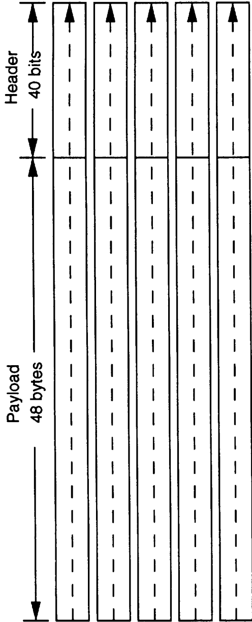
Bit Transmission Order Without Interleaving
