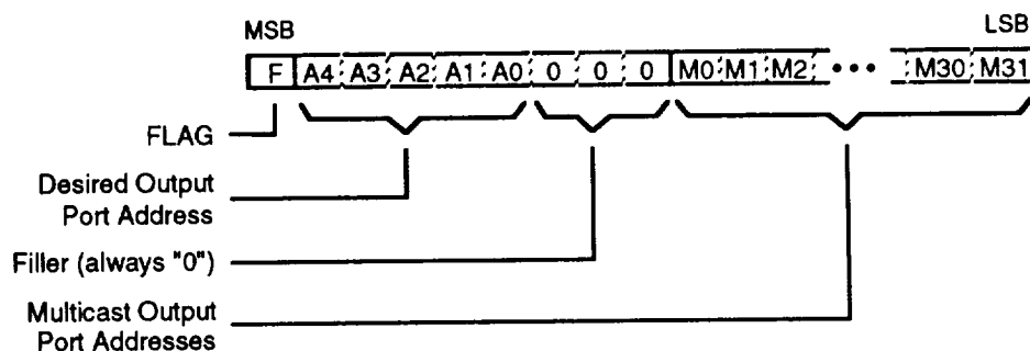
Figure 7-100. Multicast Output Port Scheme Routing Tag Format
