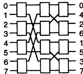
Figure 7-15. Standard 8 \times 8 Banyan Matrix Configurations
