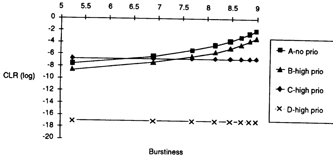
Figure C-34. Cell Loss Ratio of High Priority Cells vs. Burstiness for Different Models
