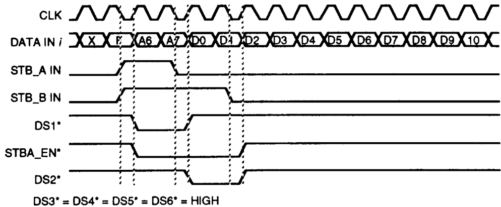
Figure 7-88c. DS2* to DS6* Generation Timing Diagram (Type 3)
