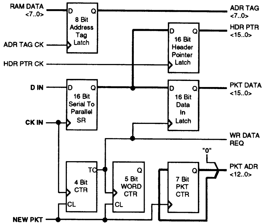
Figure 7-69. Port Side Processing Block Diagram
