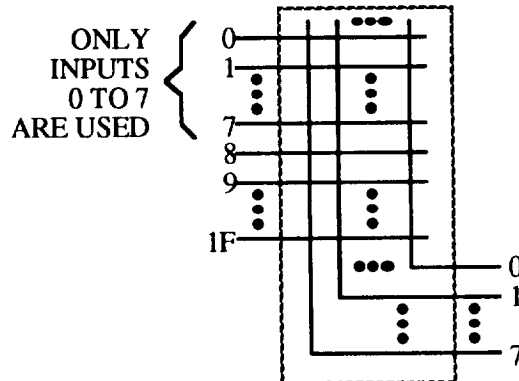
Figure 7-91. 8 x 8 Multicast Crossbar-Based Switch Fabric
