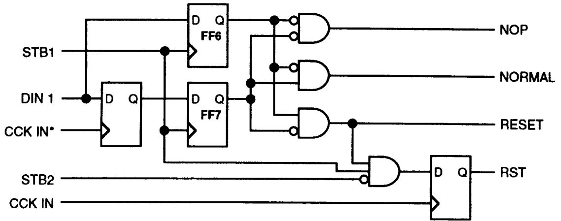
Figure 7-8. Mode Circuitry Block Diagram
