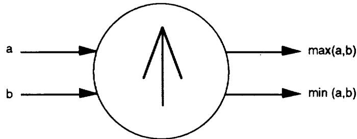
Figure 6-4. A 2 x 2 Sorting Element
