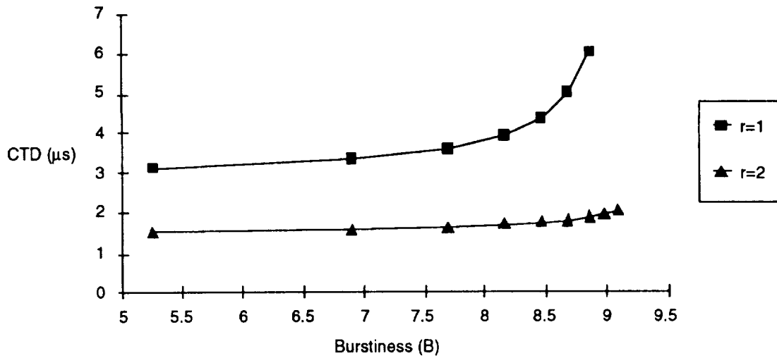
Figure C-12. Cell Transfer Delay vs. Burstiness for Mixed Traffic Scenario
