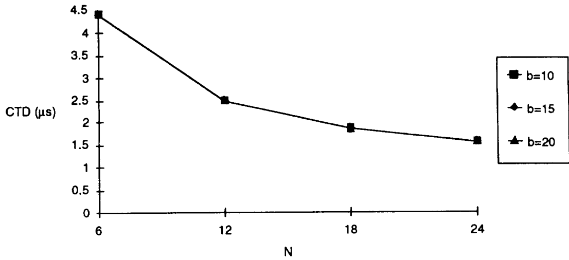
Figure C-22. Cell Transfer Delay vs. Number of Input Line for Different Buffer Sizes
