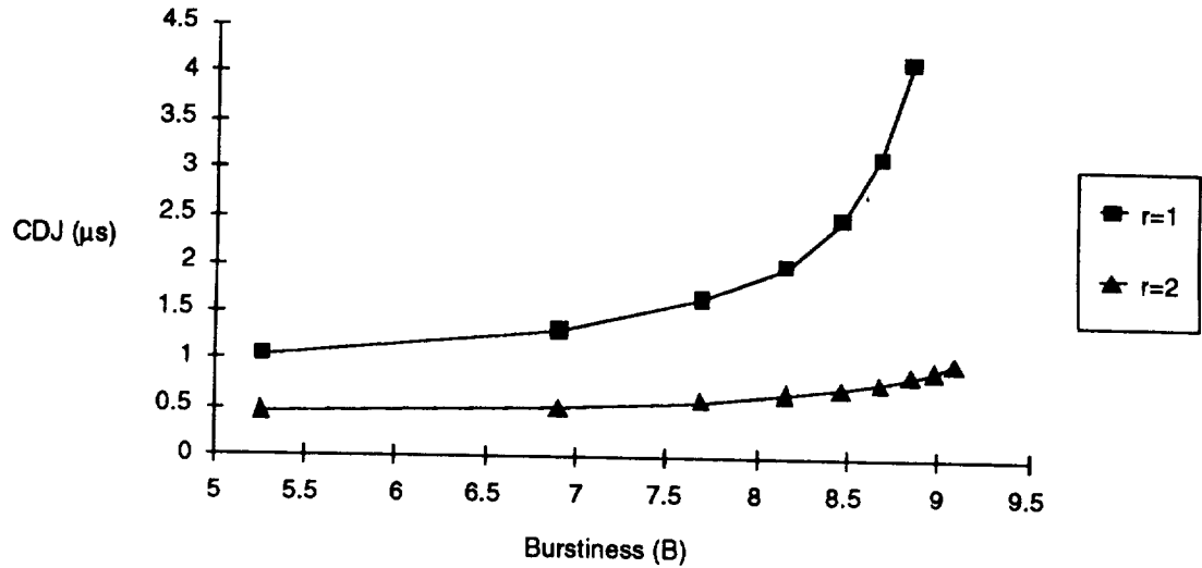
Figure C-13. Cell Delay Jitter vs. Burstiness for Mixed Traffic Scenario
