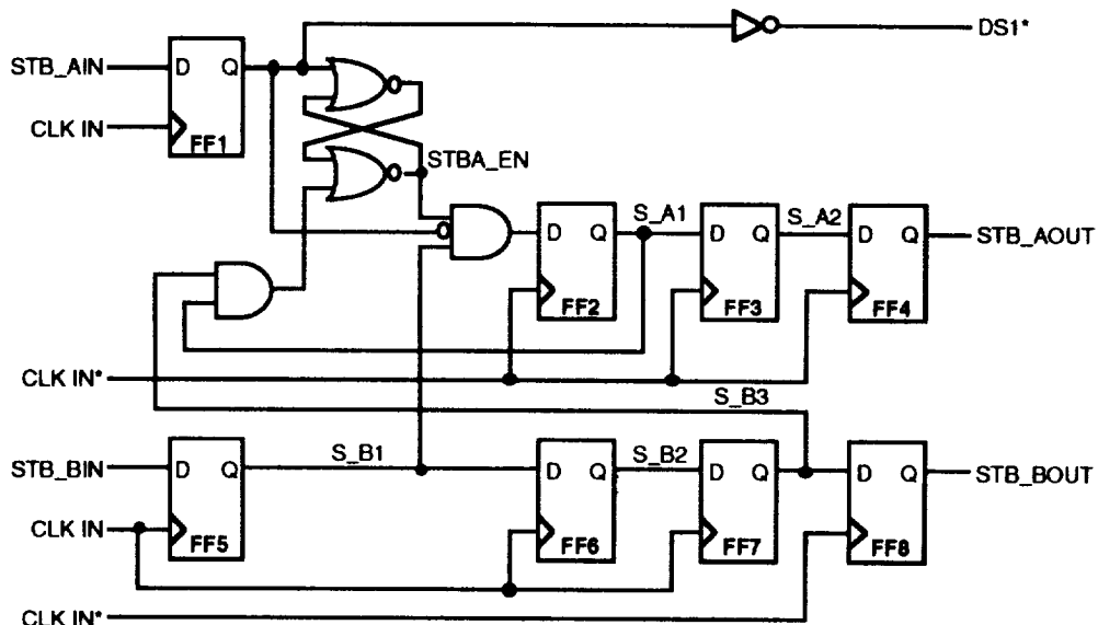
Figure 7-85. DS1*, STB_AOUT, STB_BOUT Generation Block Diagram
