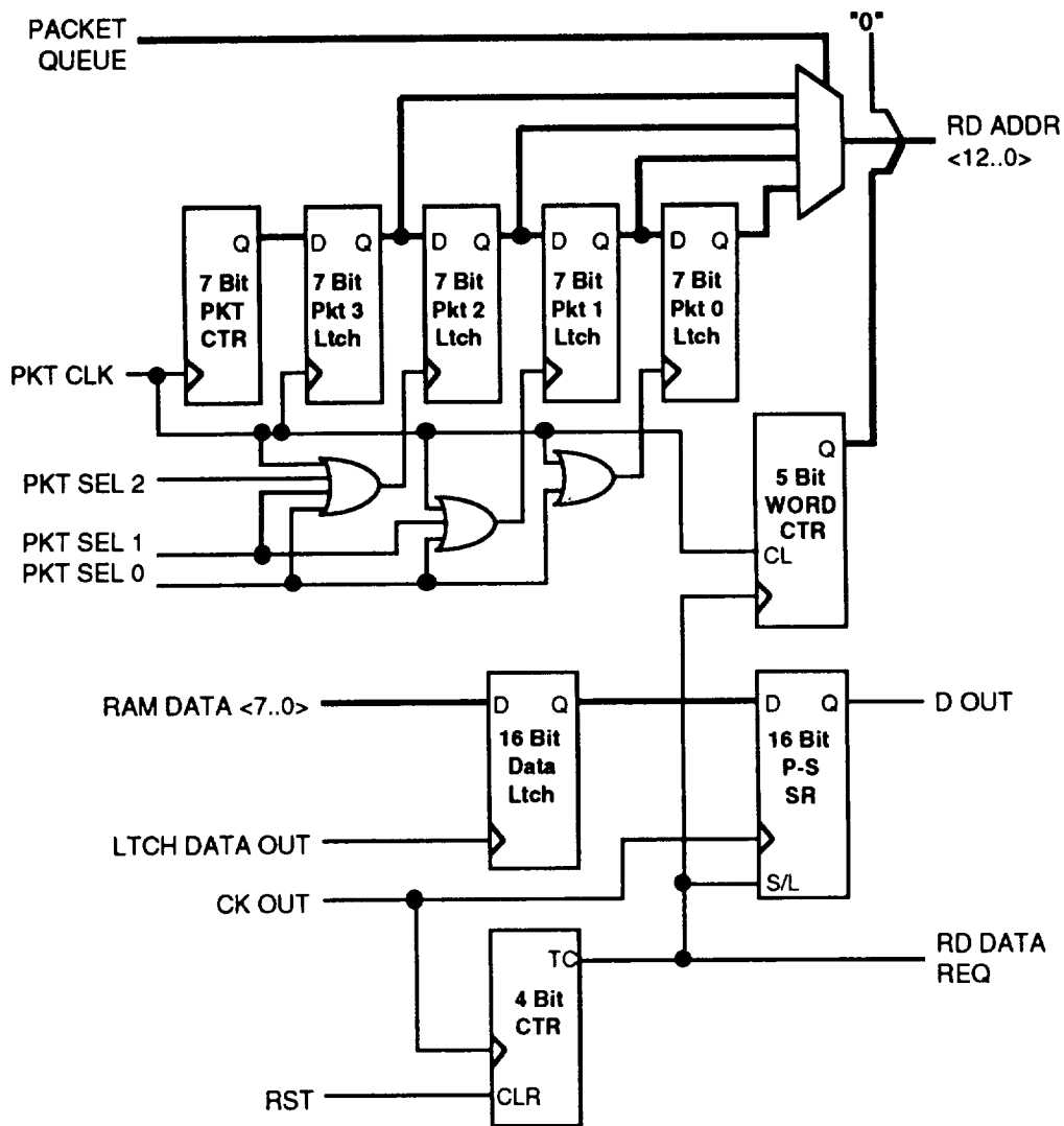
Figure 7-73. Switch Fabric Side Processing Block Diagram
