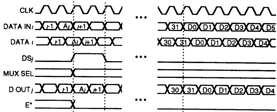
Figure 7-98. Output Selection Timing Diagram
