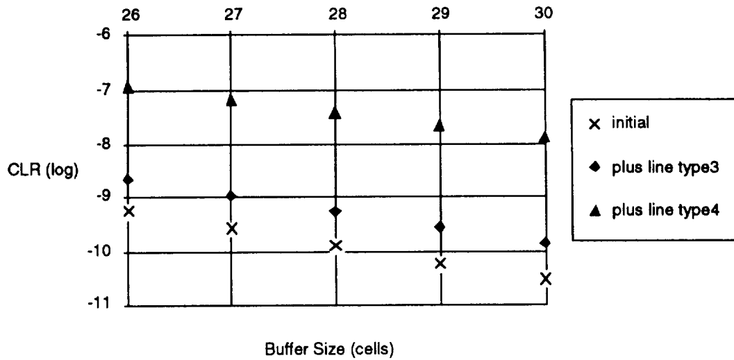
Figure C-42. Example of Connection Admission Control
