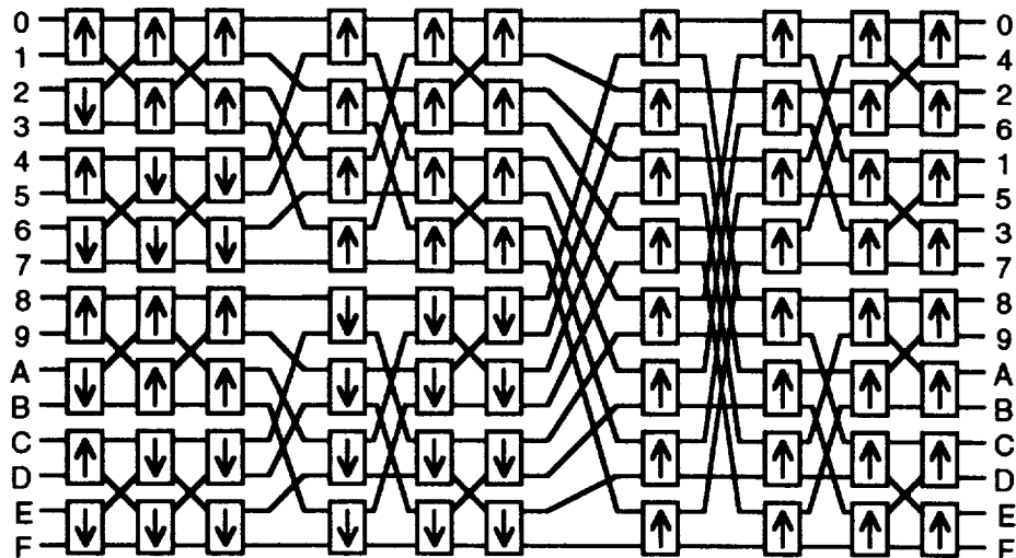
Figure 7-22. Standard 16 \times 16 Batcher Sorting Matrix Configuration
