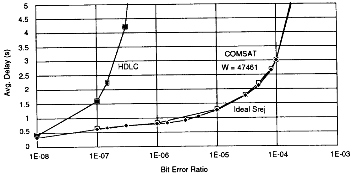
Delay Performance
