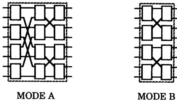
Figure 7-18. Banyan ASIC Configurations
