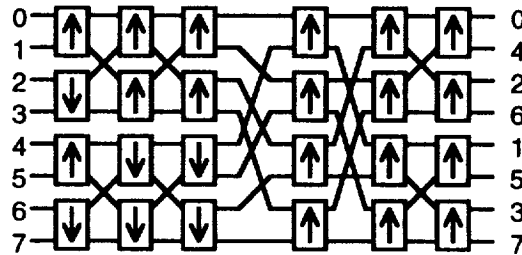
Figure 7-21. Standard 8 \times 8 Batcher Sorting Matrix Configuration
