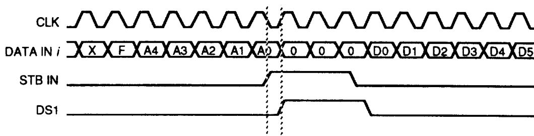
Figure 7-64. Strobe Generation Timing Diagram
