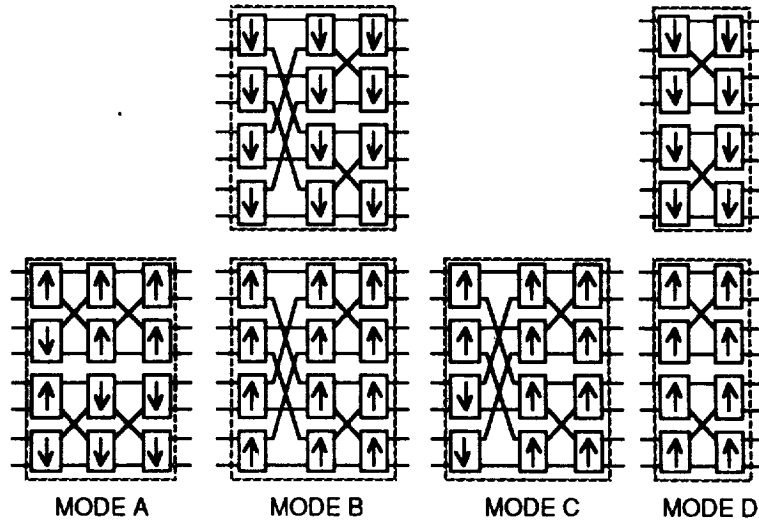
Figure 7-24. Batcher ASIC Configurations
