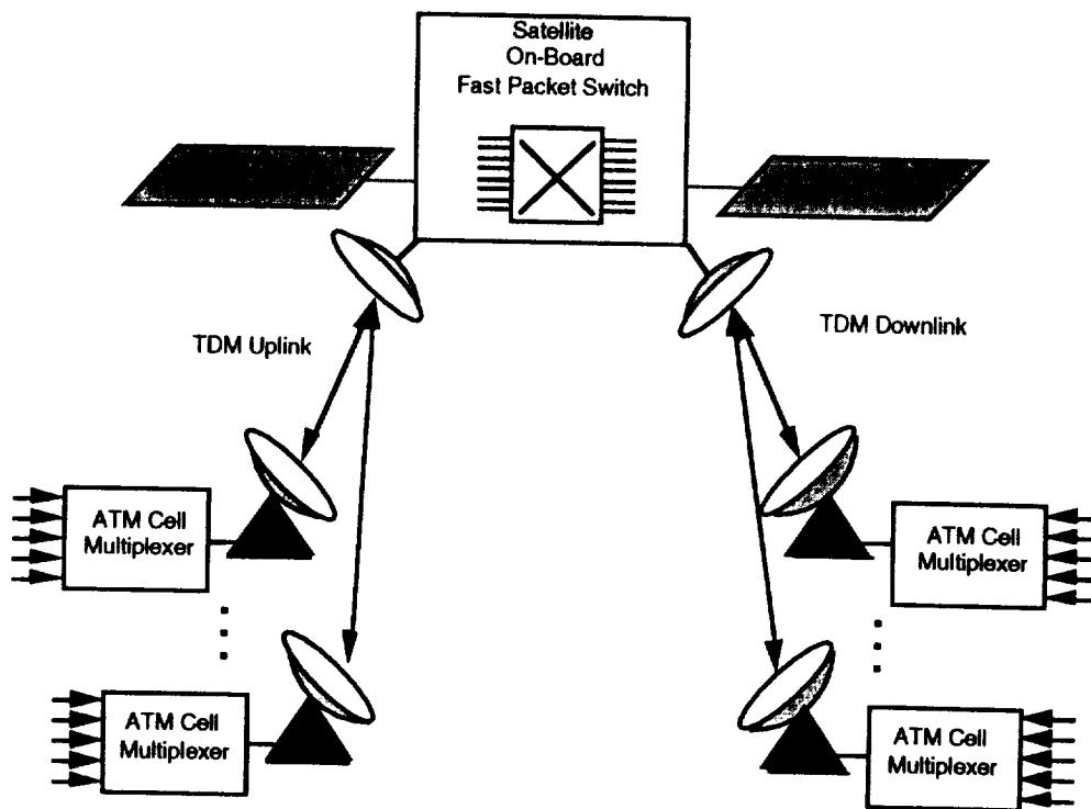
Figure D-2. Satellite B-ISDN Simulation Model
