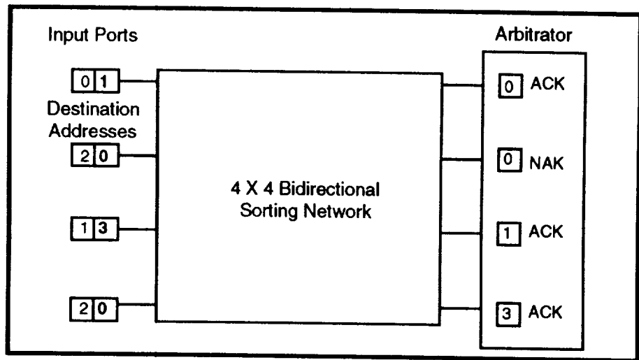
Figure 6-24. Output Contention Resolution Using a Sorting Network
