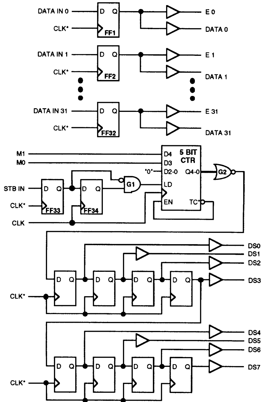
Figure 7-95. Address Filter Block Diagram
