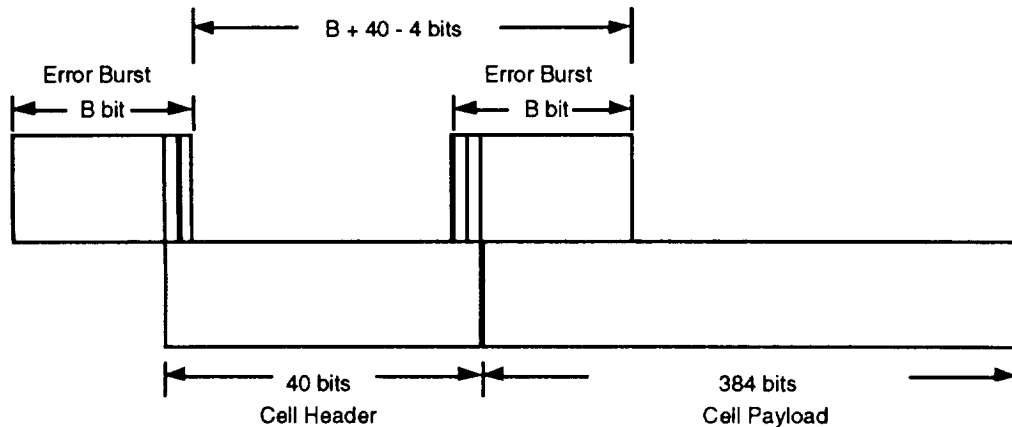
Figure 5-22. Possible Positions of the Error Burst Which Causes the Loss of a Cell
