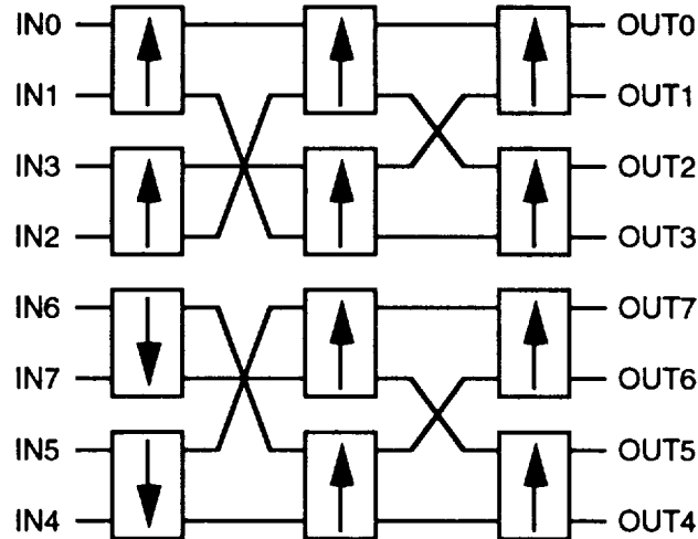
Figure 7-45. MODE A ASIC Configuration (CFG 2,1,0 = "111")
