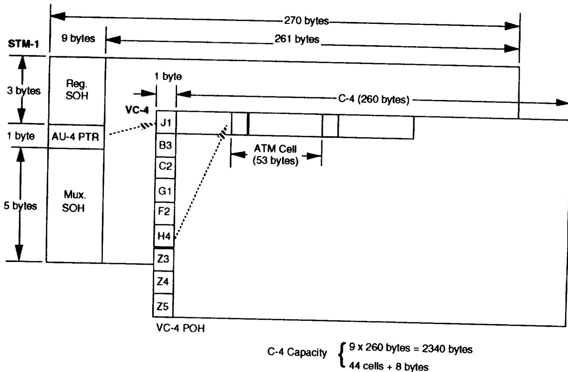
Figure 5-5. SDH Frame Structure
