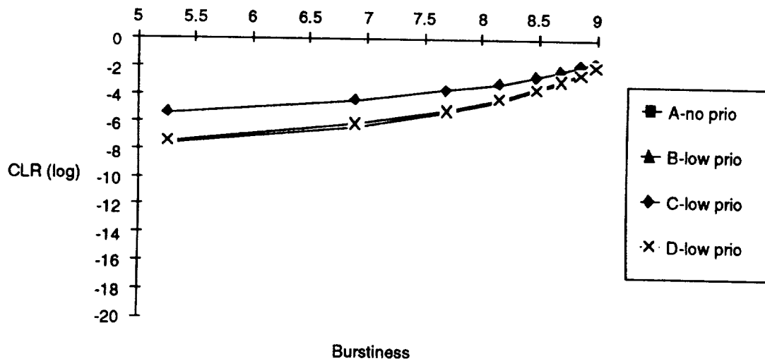
Figure C-35. Cell Loss Ratio of Low Priority Cells vs. Burstiness for Different Models
