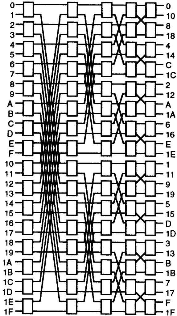
Figure 7-17. Standard 32 x 32 Banyan Matrix Configurations
