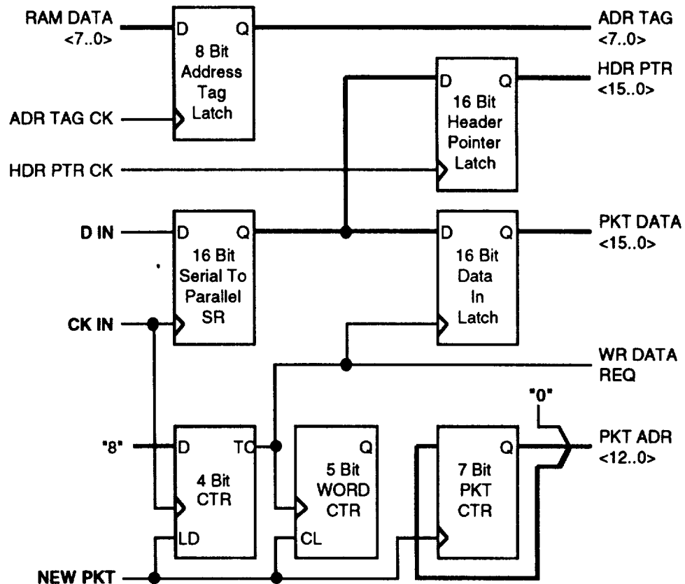
Figure 7-6. Port Side Processing Block Diagram
