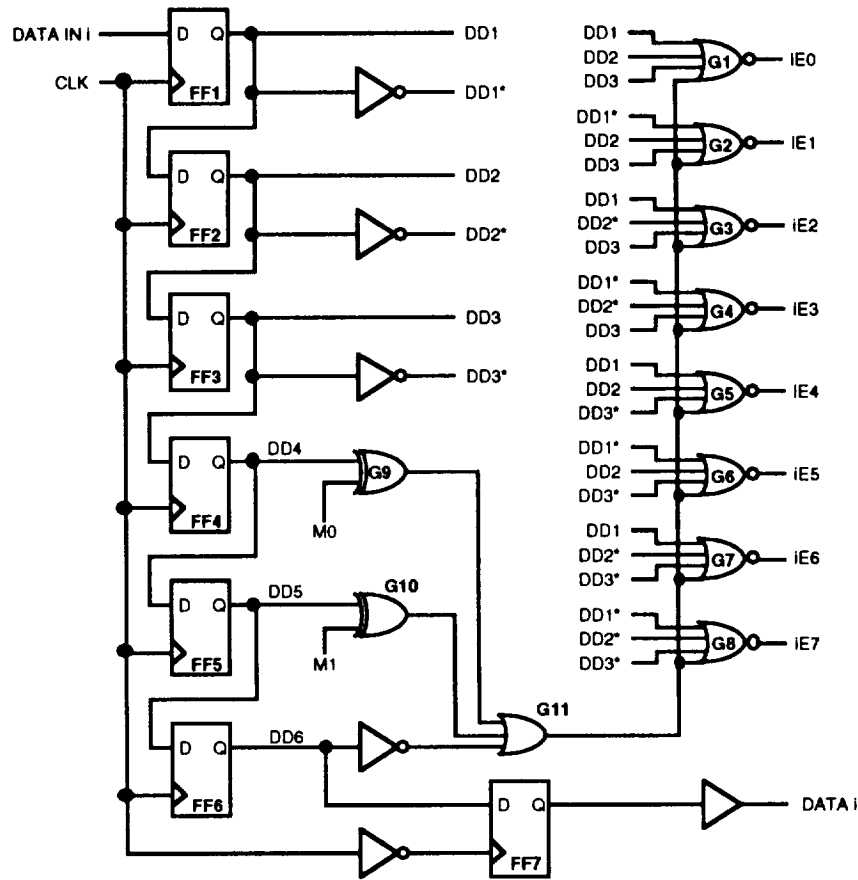
Figure 7-59. Address Filter Block Diagram
