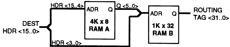
Figure 7-68. Routing Tag Memory Mapping
