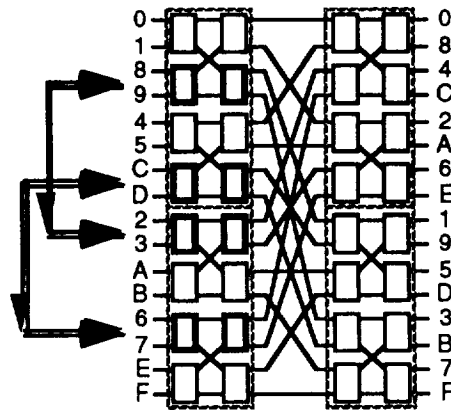
Figure 7-19. 16 x 16 Banyan Matrix Implementation
