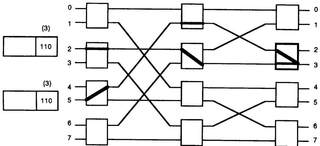
Figure 6-7. Output Contention
