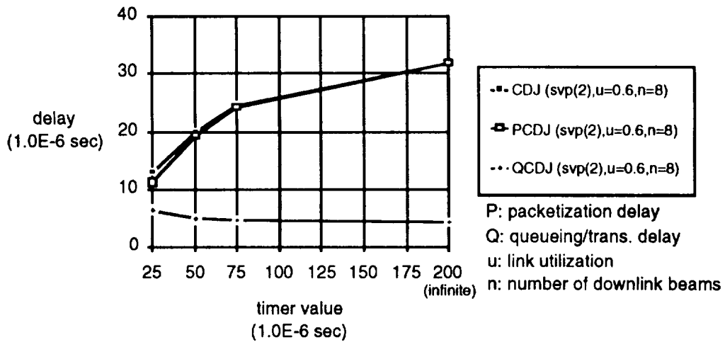
Figure D-8. Cell Delay Jitter vs. Time-out Value When the Input Link Utilization is 60 Percent
