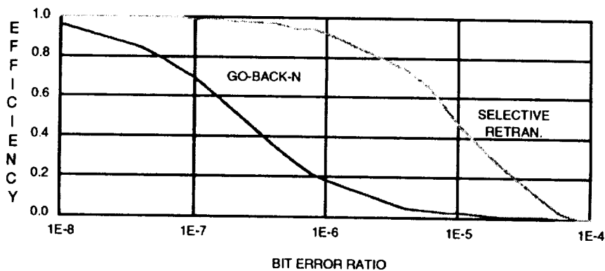
Efficiency of a 45 Mbit/s Terrestrial Link for a Frame Size of 4096 Bytes
