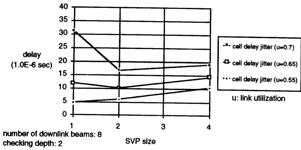
Figure D-19. Cell Delay Jitter vs. SVP Size for Different Input Link Utilization
