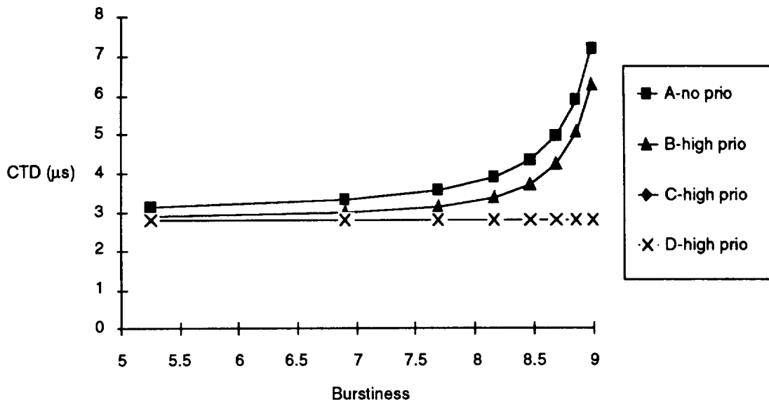
Figure C-36. Cell Transfer Delay of High Priority Cells vs. Burstiness for Different Models
