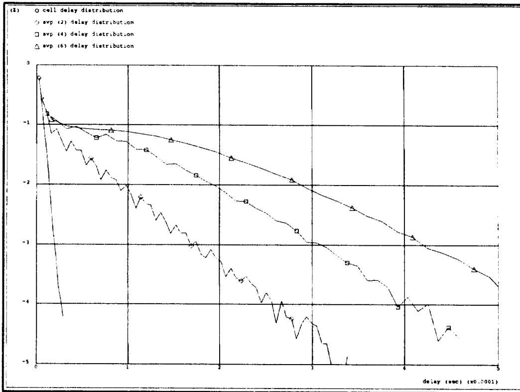
Figure D-5a. Cell Delay Distribution for Different SVP Sizes When the Output Link Utilization is 60 Percent
