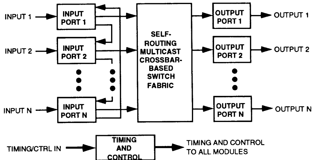
Figure 7-89. Self-Routing Multicast Crossbar-Based Network Block Diagram
