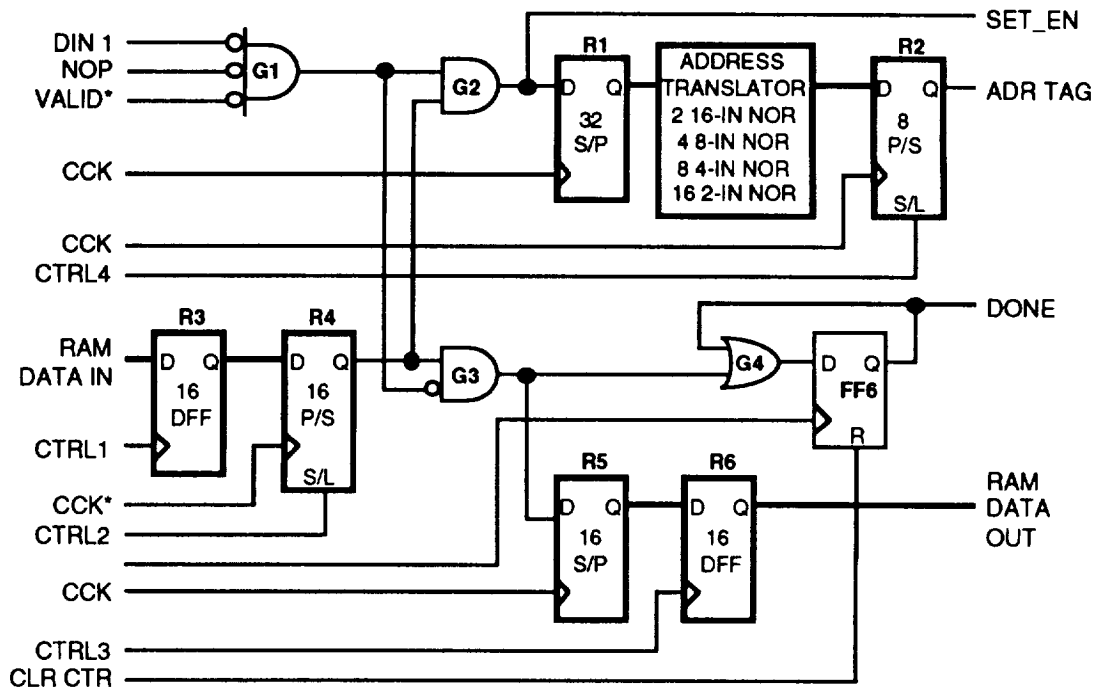
Figure 7-71. Output Port Selection Block Diagram
