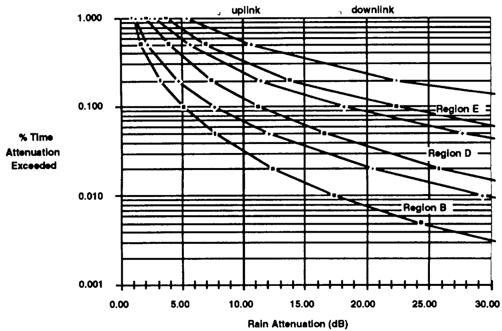
Figure A-3. Rain Attenuation at 20/30 GHz
