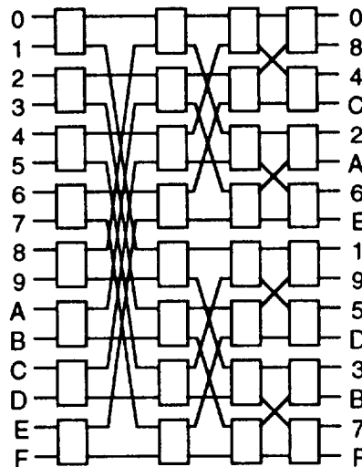
Figure 7-16. Standard 16 \times 16 Banyan Matrix Configurations
