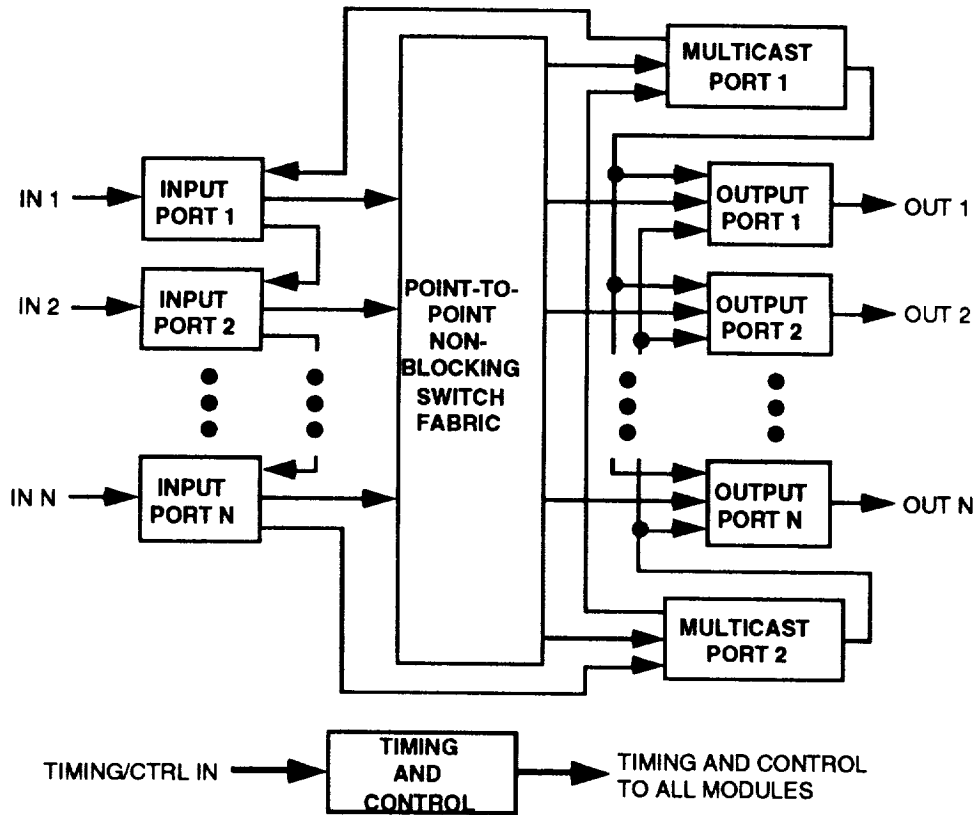
Figure 7-99. Point-To-Point Switch Fabric With Multicast Output Ports Block Diagram
