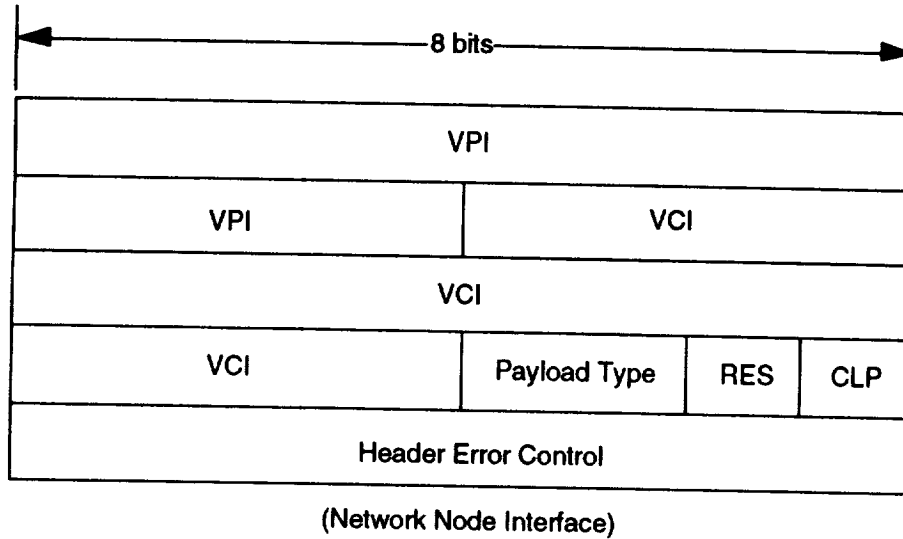
Figure 2-5. NNI ATM Cell Format
