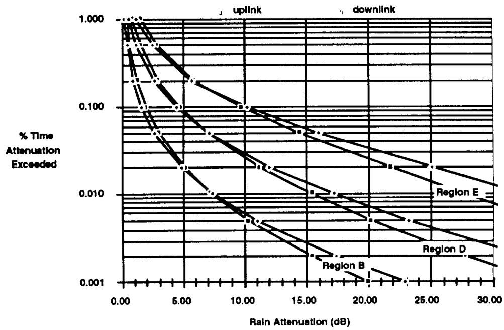
Figure A-2. Rain Attenuation at 12/14 GHz
