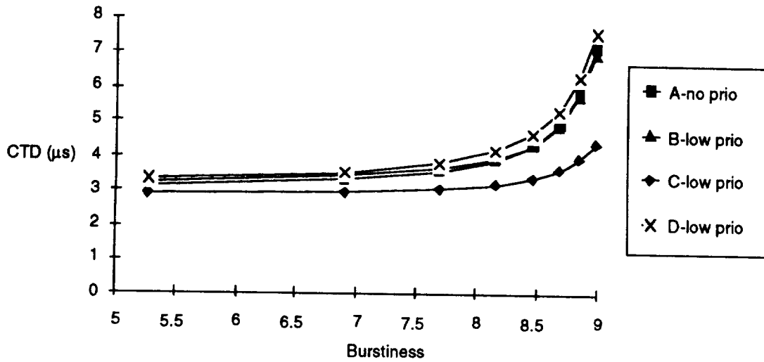
Figure C-38. Cell Transfer Delay of Low Priority Cells vs. Burstiness for Different Models
