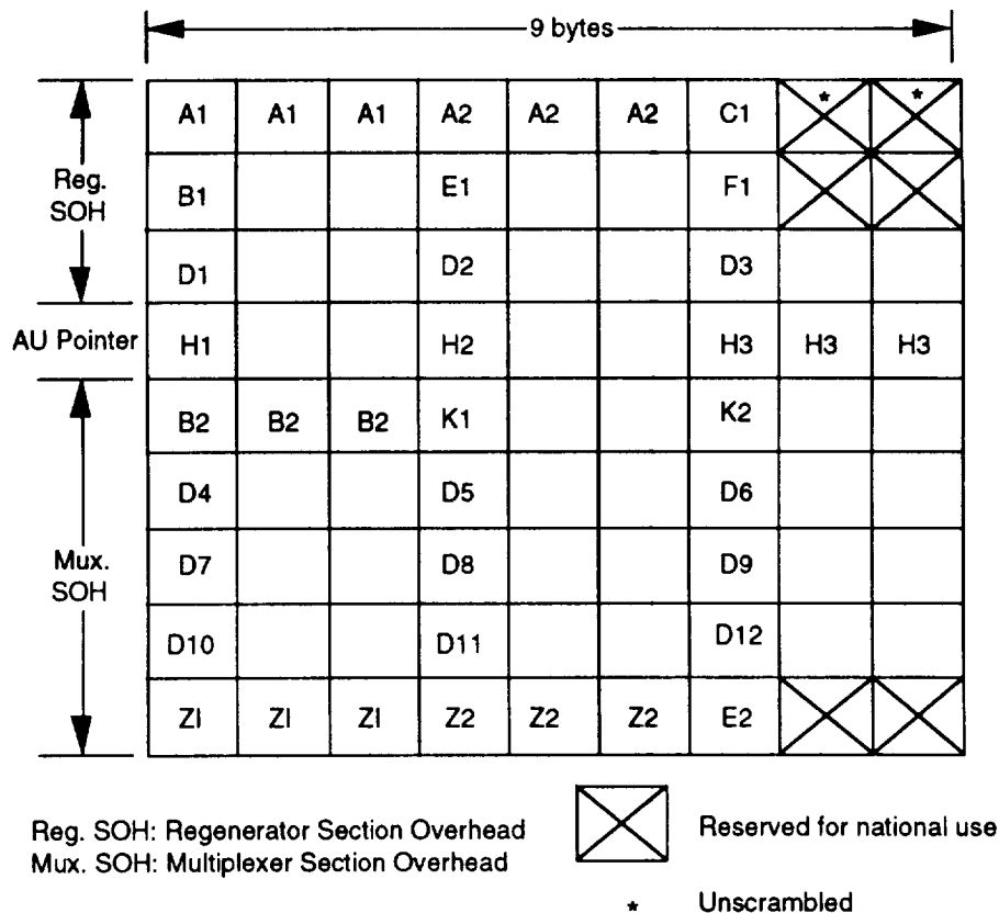
Figure 2-8. Section Overhead and AU Pointer Format
