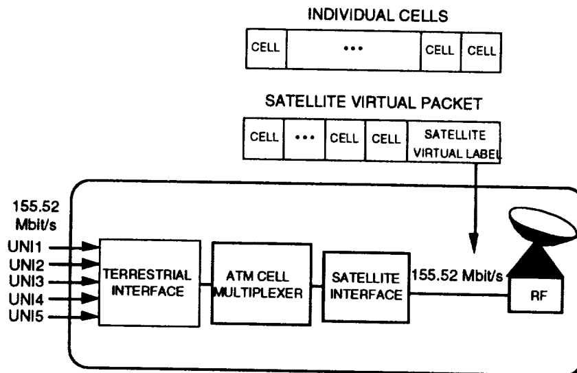
Figure D-1. ATM Earth Station Configuration
