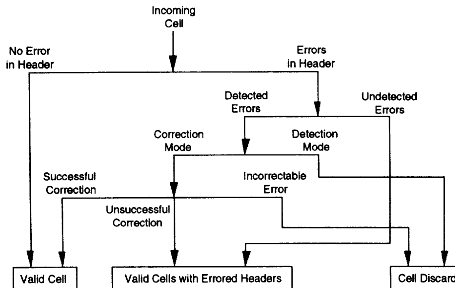
Figure 5-15. Consequences of Errors in ATM Cell Headers
