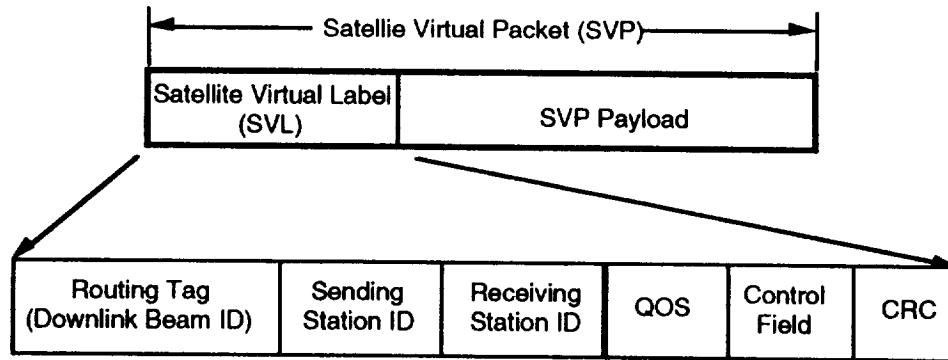
Figure 5-12. Satellite Virtual Label Format
