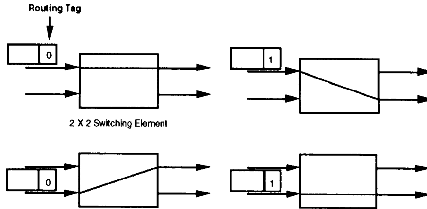
Figure 6-2. Destination Tag Routing Algorithm
