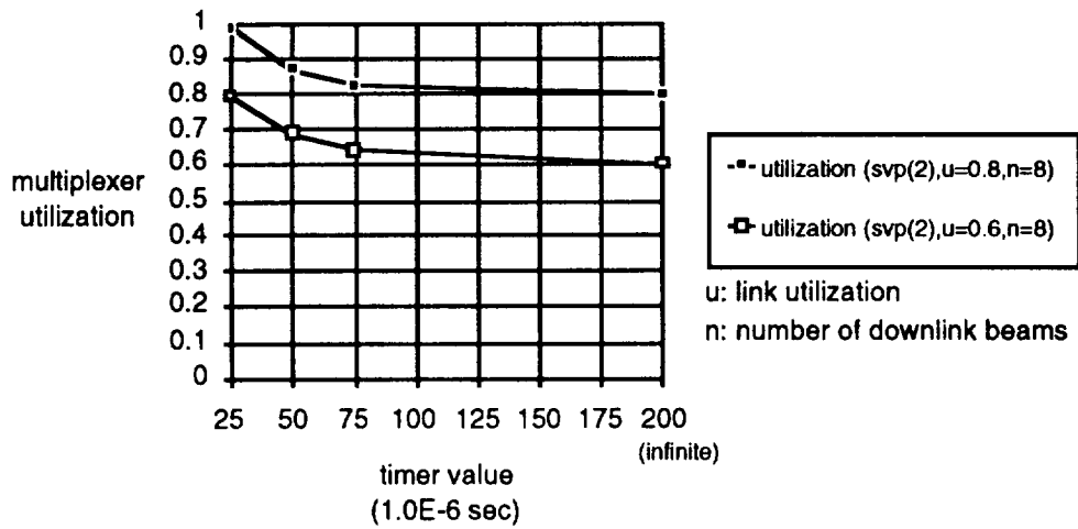
Figure D-7. Multiplexer Utilization vs. Time-out Value for Different Input Link Utilization
