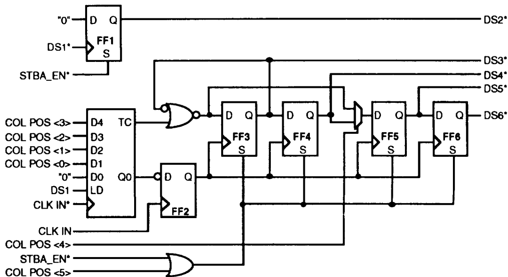
Figure 7-87. DS2* to DS6* Generation Block Diagram
