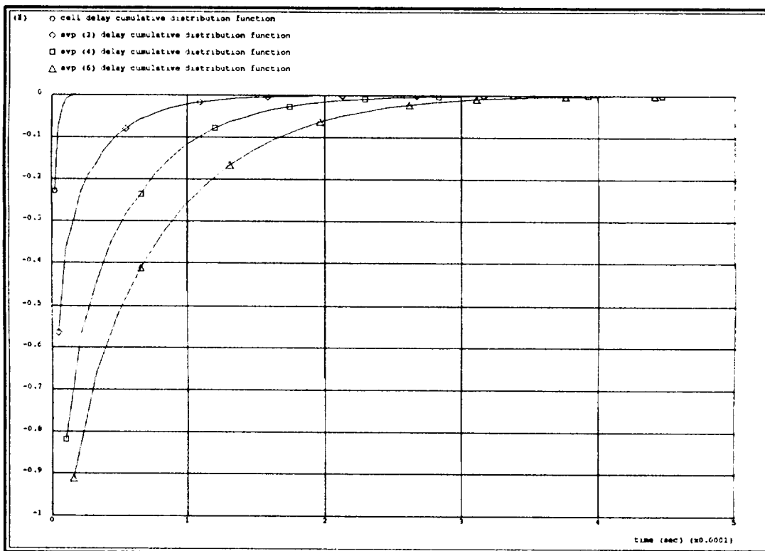
Figure D-5b. Cell Delay Cumulative Distribution for Different SVP Sizes When the Output Link Utilization is 60 Percent
