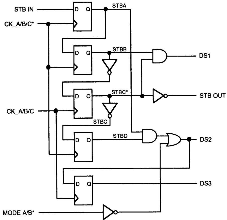
Figure 7-39. Strobe Generation Block Diagram
