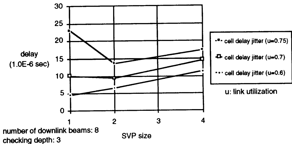
Figure D-21. Cell Delay Jitter vs. SVP Size for Different Input Link Utilization
