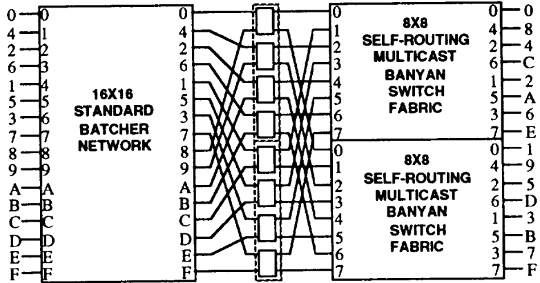
Figure 7-76. 16 x 16 Multicast Banyan Switch Fabric
