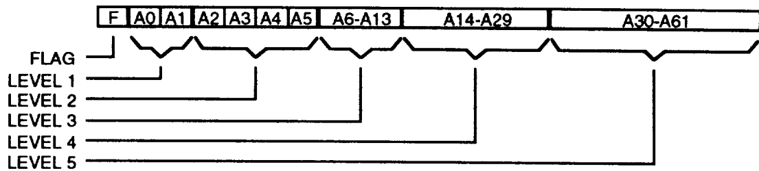
Figure 7-66. Multicast Banyan Routing Tag Format
