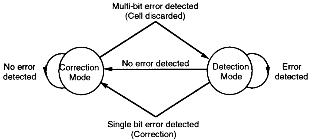
Figure 5-16. HEC Receiver Modes of Operation
