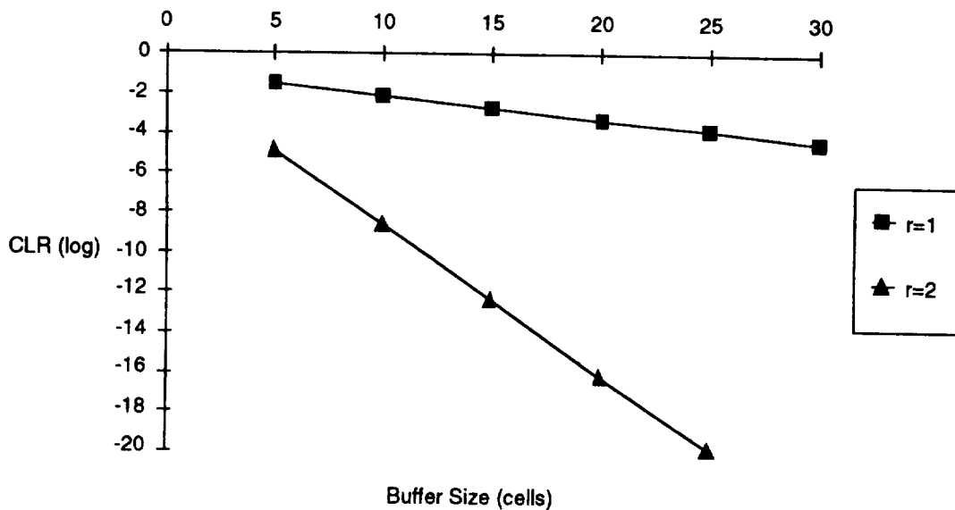
Figure C-17. Cell Loss Ratio vs. Buffer Size for Different Output Transmission Rates
