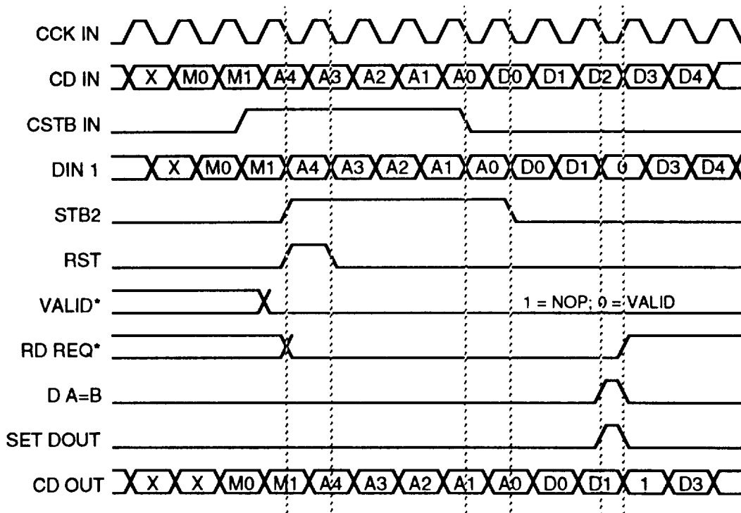
Figure 7-11. Timing Diagram
