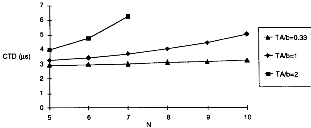
Figure C-25. Cell Transfer Delay vs. Number of Input Lines for Different Ratios of Average Burst Size and Buffer Size
