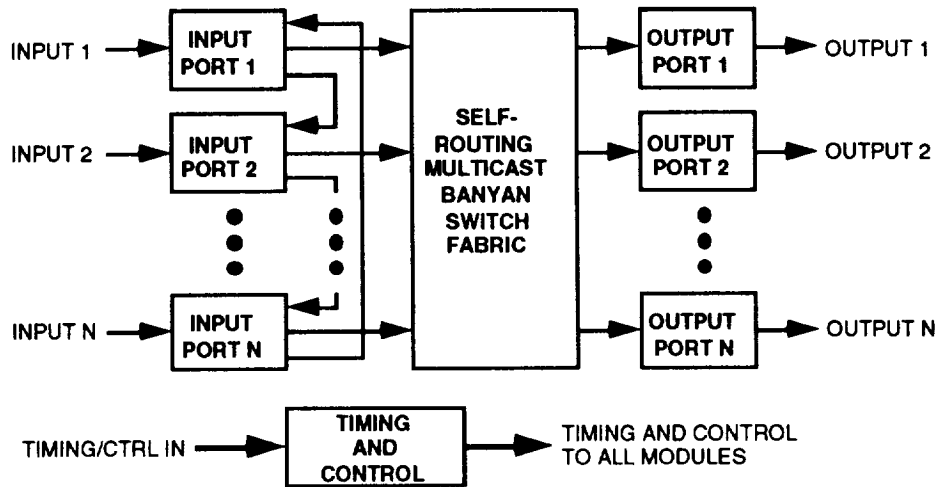
Figure 7-65. Self-Routing Multicast Banyan Network Block Diagram
