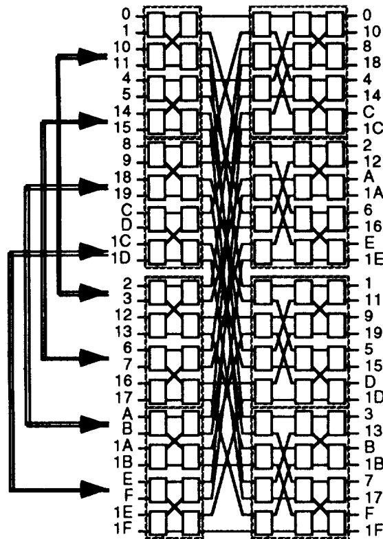
Figure 7-20. 32 x 32 Banyan Matrix Implementation
