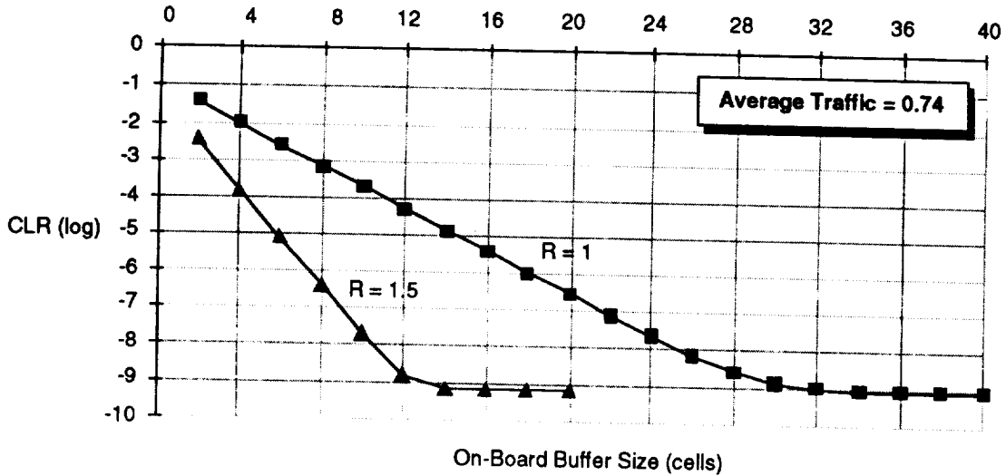
Figure C-41. System Cell Loss Ratio vs. On-Board Buffer Size for Different Output Transmission Rates
