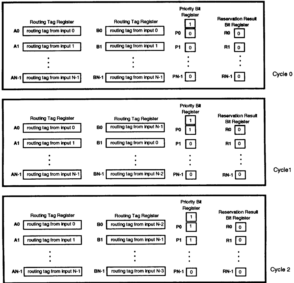
Figure 6-26. Output Contention Resolution Device
