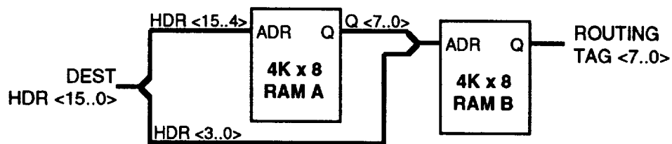
Figure 7-5. Routing Tag Memory Mapping
