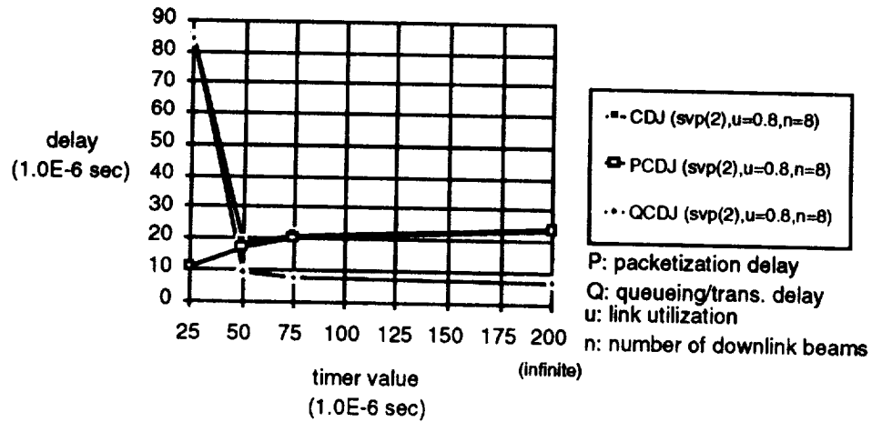
Figure D-9. Cell Delay Jitter vs. Time-out Value When the Input Link Utilization is 80 Percent
