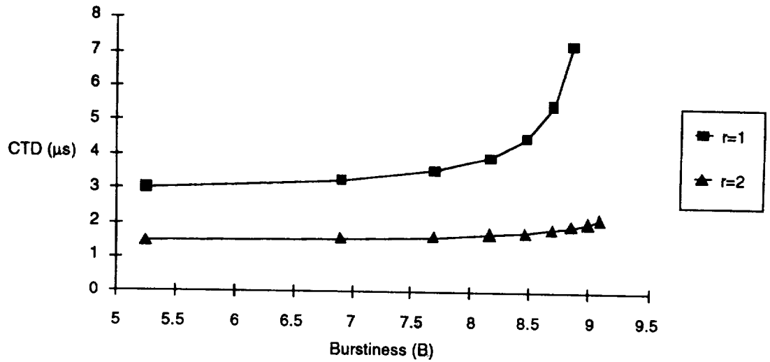
Figure C-10. Cell Transfer Delay vs. Burstiness for Different Output Transmission Rates
