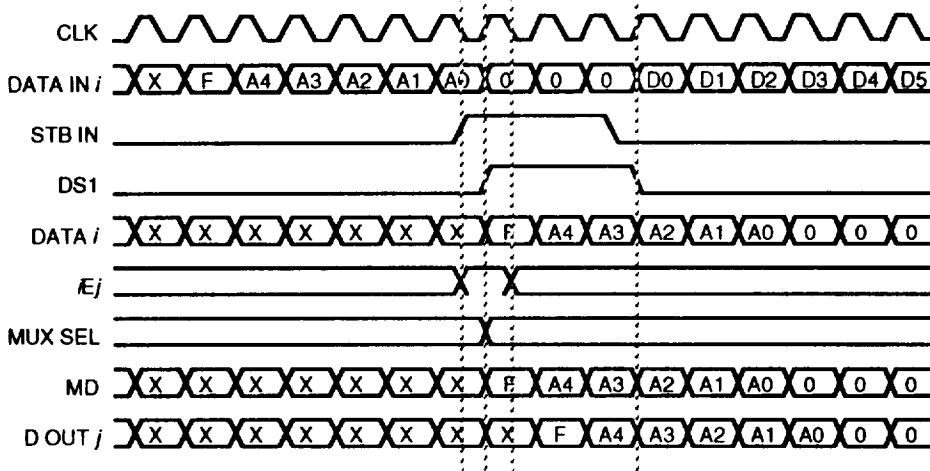
Figure 7-62. Output Selection Timing Diagram
