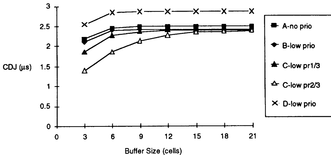
Figure C-33. Cell Transfer Delay of Low Priority Cells vs. Buffer Size of Different Models
