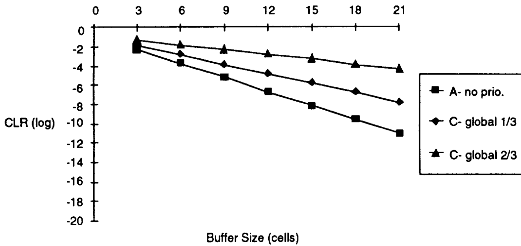
Figure C-29. Average Cell Loss Ratio vs. Buffer Size for Models A and C
