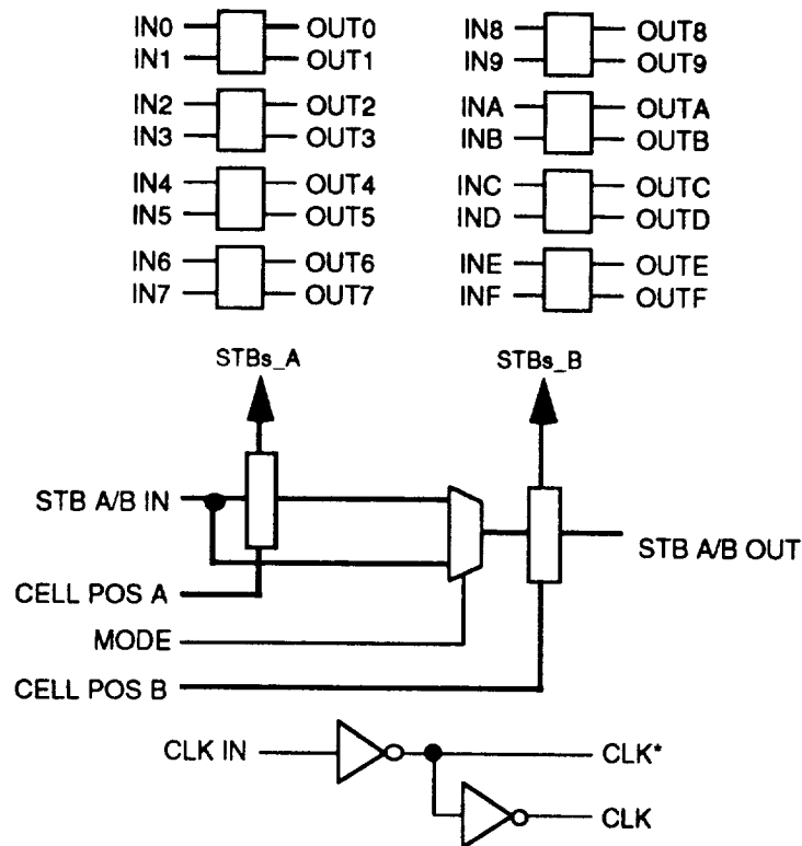
Figure 7-78. Multicast Banyan ASIC Block Diagram
