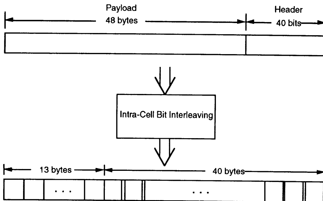
Figure 5-19. Intra-Cell Bit Interleaving
