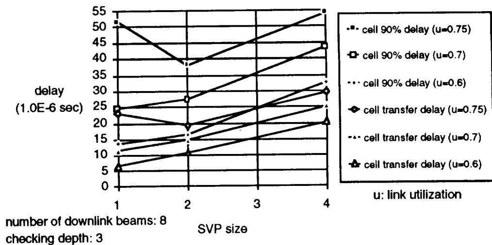
Figure D-22. Cell 90 Percent Delay and Cell Transfer Delay vs. SVP Size for Different Input Link Utilization
