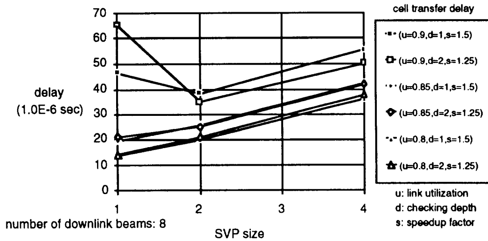
Figure D-26. Cell Transfer Delay vs. SVP Size for Different Link Utilization and Configurations
