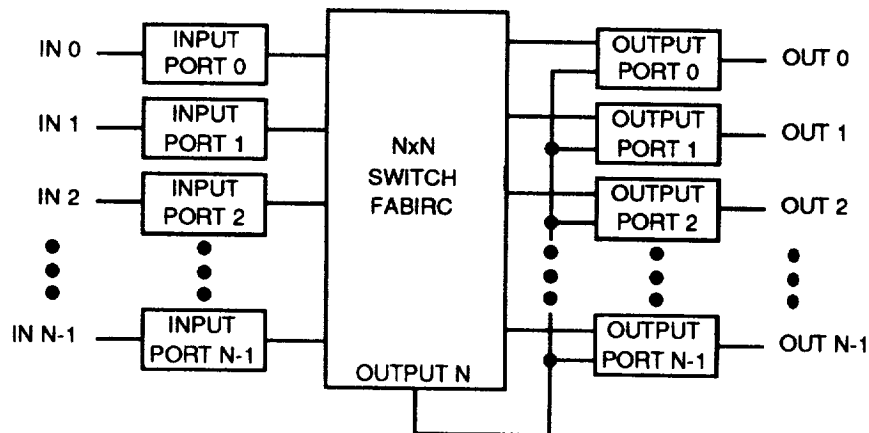
Figure 7-104. 1-For-N Switch Fabric Path Redundancy Block Diagram
