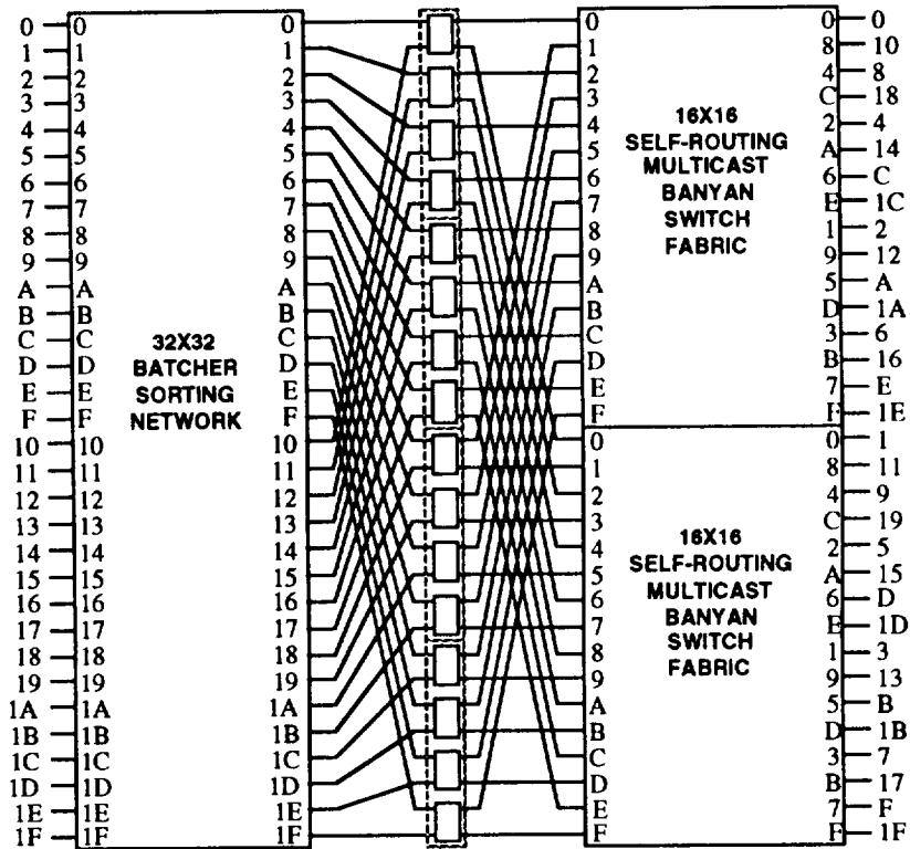
Figure 7-77. 32 x 32 Multicast Banyan Switch Fabric
