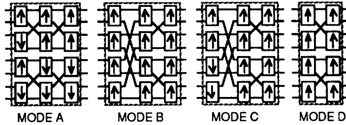
Figure 7-41. Batcher ASIC Modes
