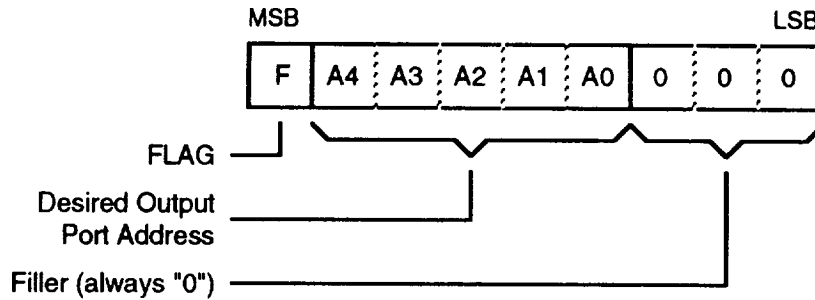
Figure 7-2. Sorted Banyan Routing Tag Format
