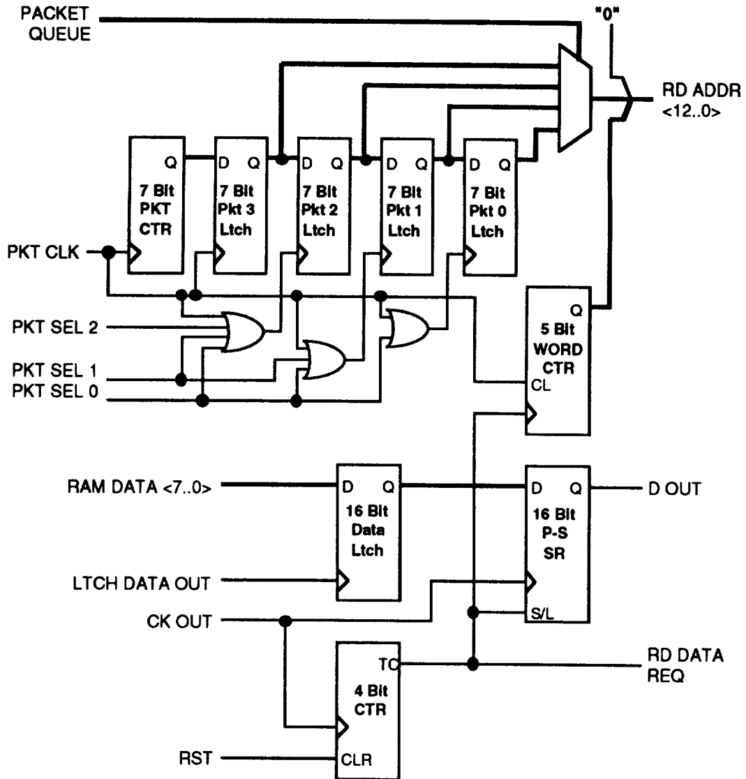
Figure 7-12. Switch Fabric Side Processing Block Diagram
