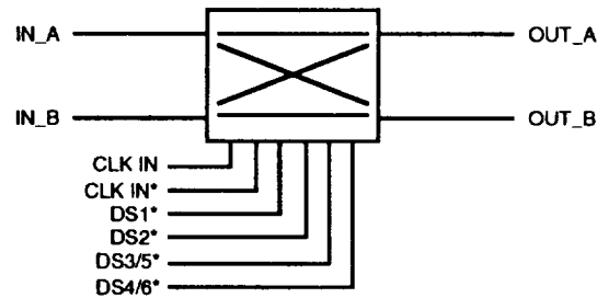
Figure 7-82. Multicast Banyan Switching Cell Block Diagram
