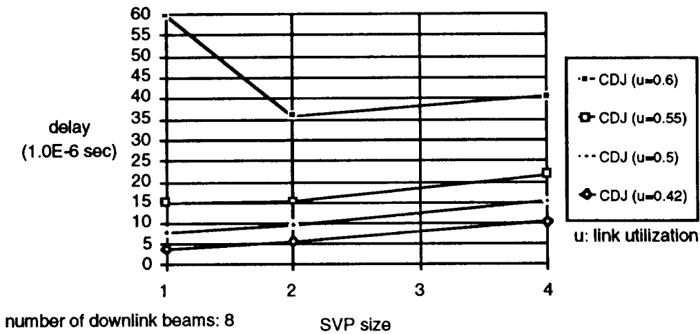
Figure D-16. Cell Delay Jitter vs. SVP Size for Different Input Link Utilization
