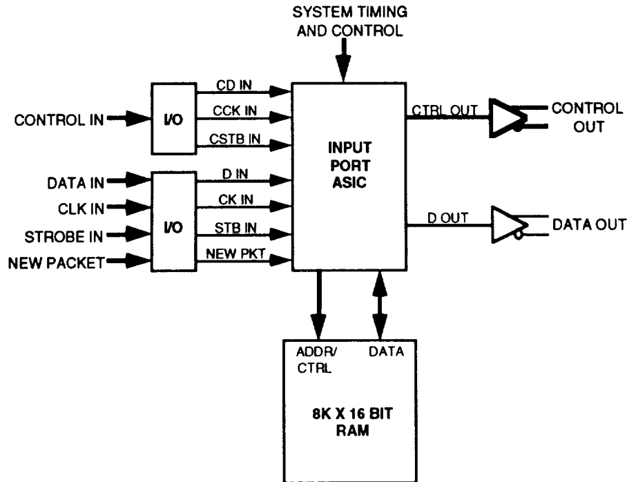
Figure 7-67. Multicast Banyan Input Port Block Diagram
