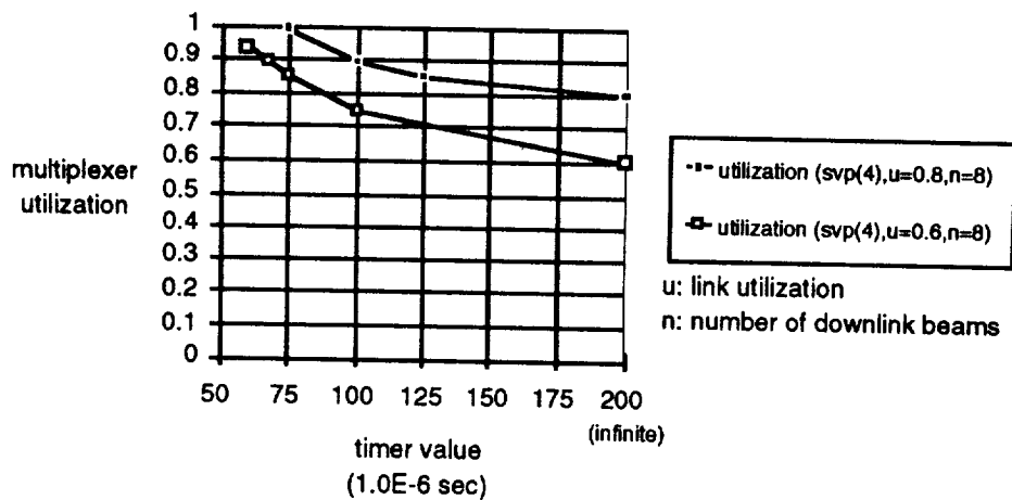
Figure D-10. Multiplexer Utilization vs. Time-out Value for Different Input Link Utilization
