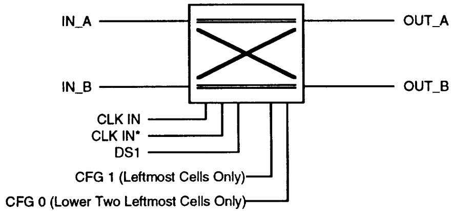
Figure 7-49. Batcher Sorting Cell Block Diagram
