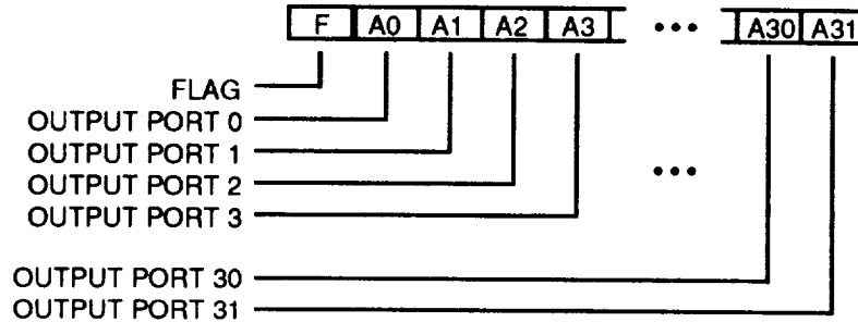
Figure 7-90. Multicast Crossbar Routing Tag Format
