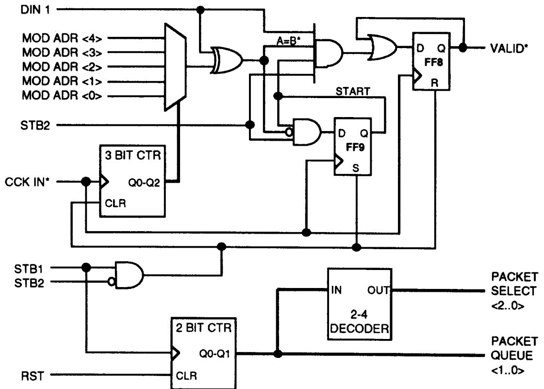
Figure 7-9. Address Filter Block Diagram
