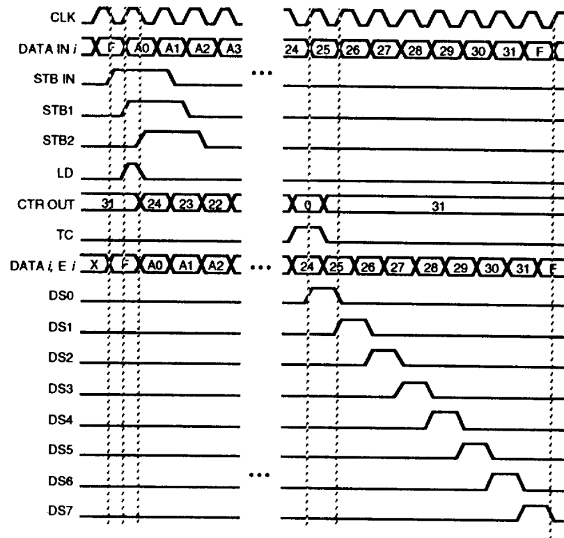
Figure 7-96d. Address Filter Timing Diagram ( M1M0 = 11 )
