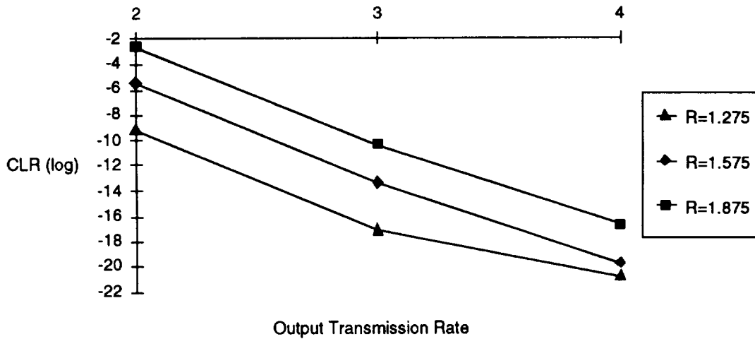
Figure C-18. Cell Loss Ratio vs. Output Transmission Rate for Different Average Arrival Rates
