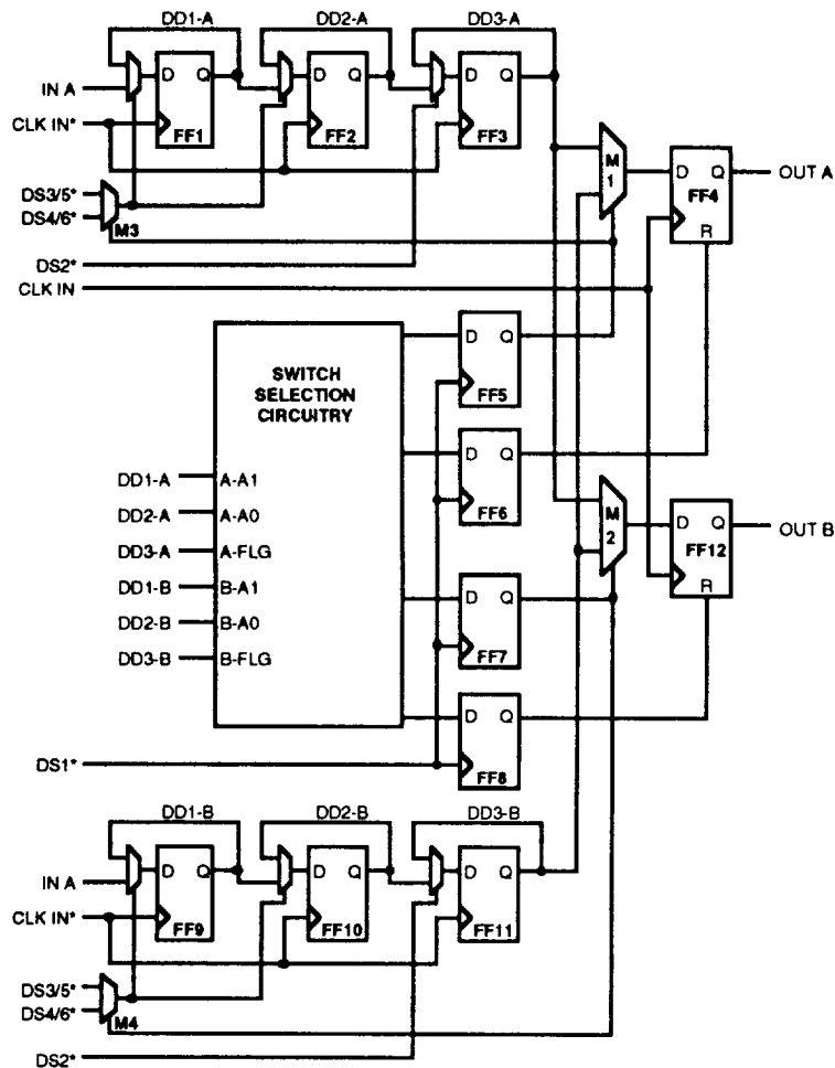
Figure 7-83. Multicast Banyan Switching Cell Detailed Block Diagram
