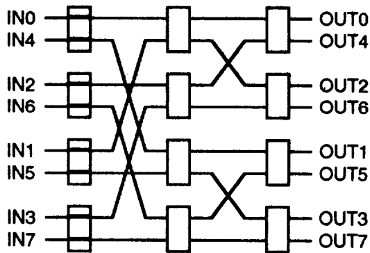
Figure 7-35. MODE B Banyan Routing
