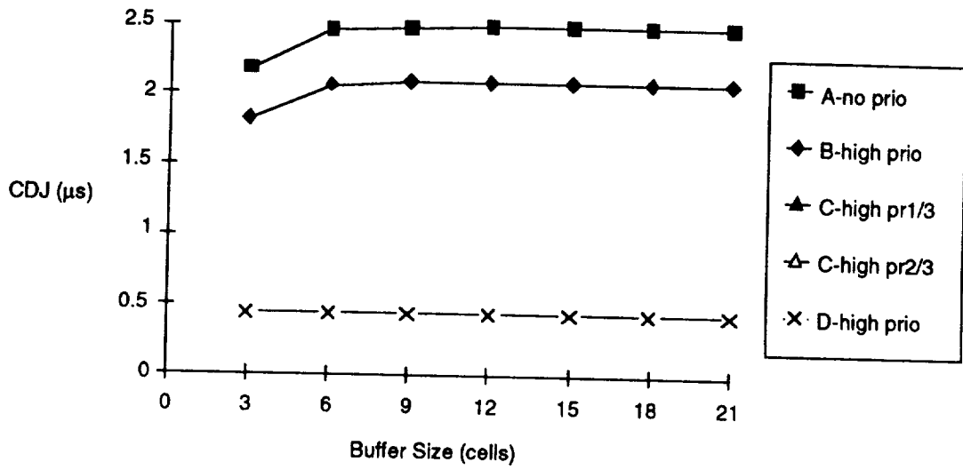
Figure C-31. Cell Delay Jitter of High Priority Cells vs. Buffer Size for Different Models
