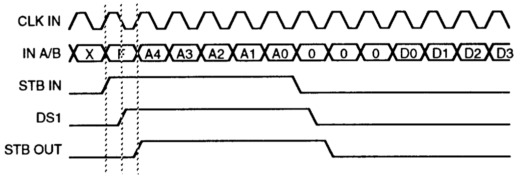
Figure 7-53. Strobe Generation Timing Diagram
