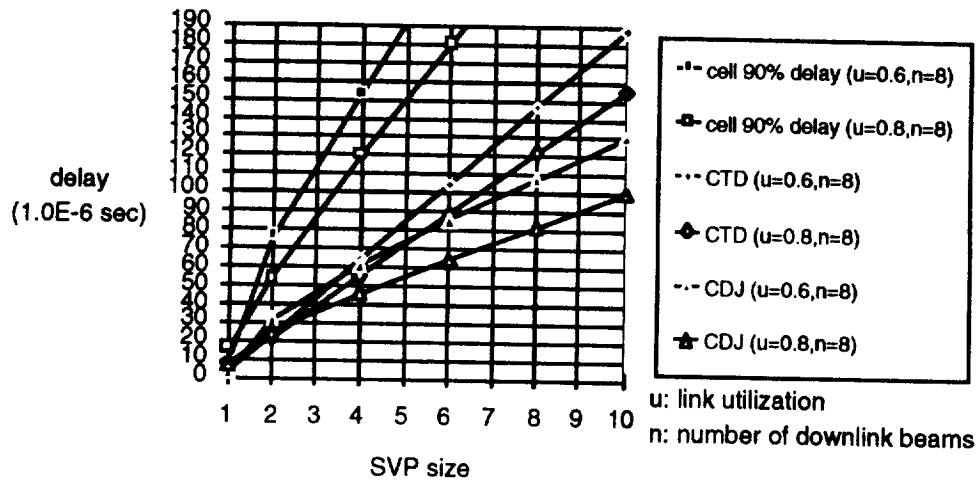
Figure D-3. Cell Delay Performance vs. SVP Sizes for Different Output Link Utilization
