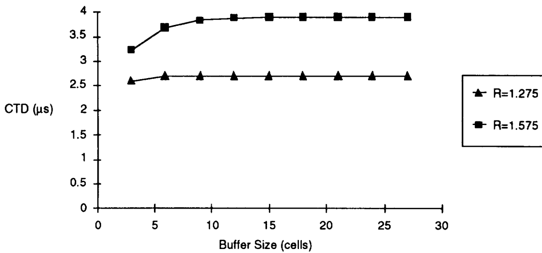
Figure C-15. Cell Transfer Delay vs. Buffer Size for Different Average Arrival Rates
