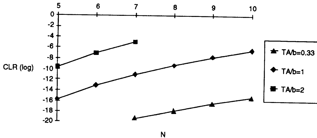
Figure C-24. Cell Loss Ratio vs. Number of Input Lines for Different Ratios of Average Burst Size and Buffer Size
