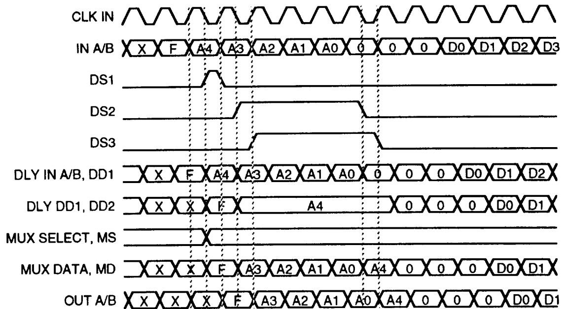
Figure 7-38. Banyan Switching Cell Timing Diagram
