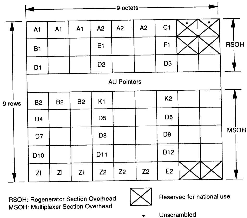
Figure 5-6. SDH Section Overhead
