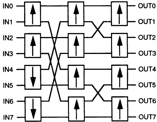
Figure 7-47. MODE C ASIC Configuration (CFG 2,1,0 = "011")
