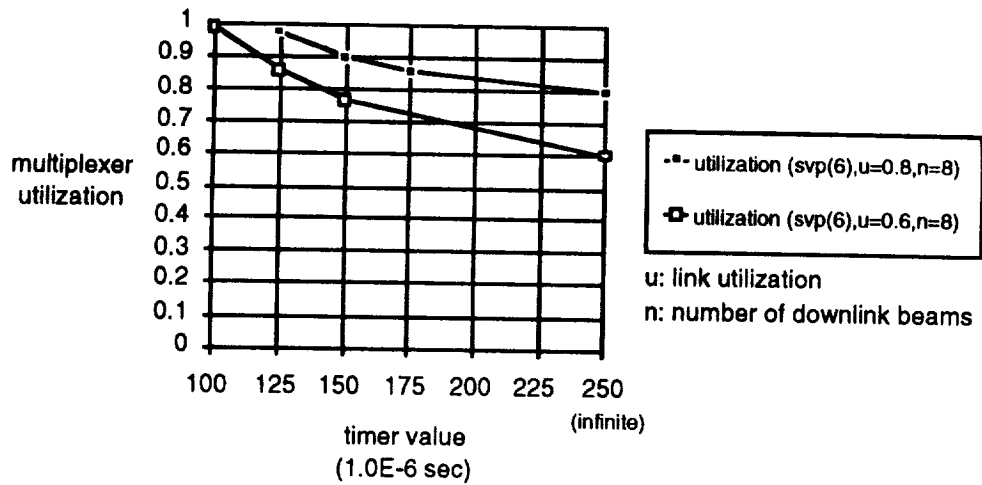
Figure D-13. Multiplexer Utilization vs. Time-out Value for Different Input Link Utilization
