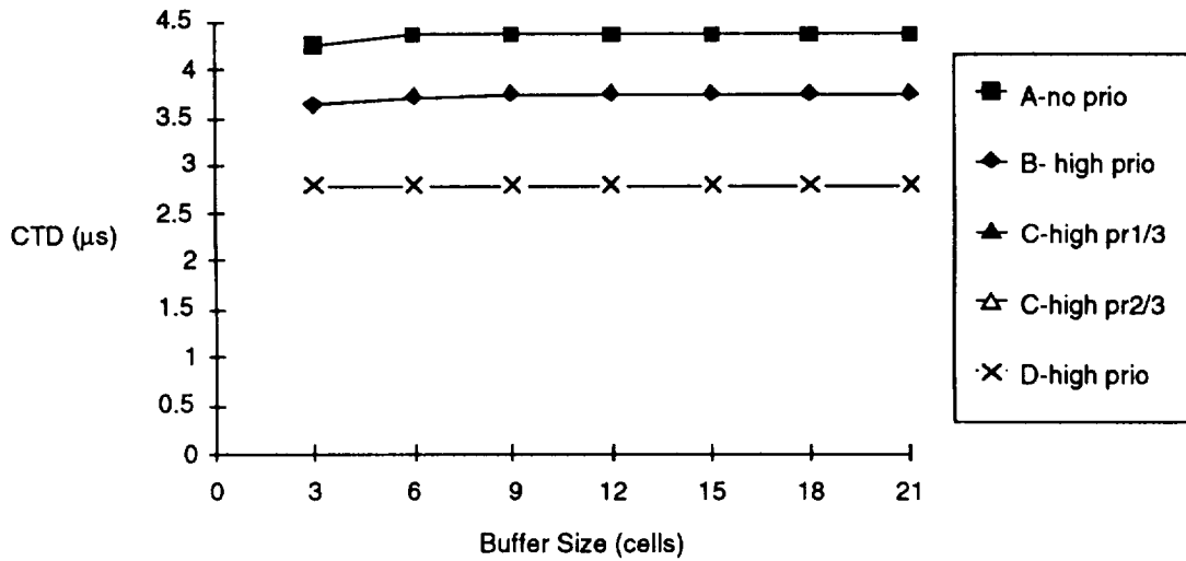
Figure C-30. Cell Transfer Delay of High Priority Cells vs. Buffer Size for Different Models
