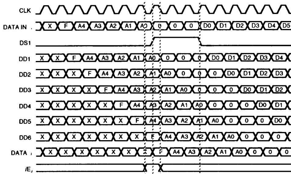
Figure 7-60. Address Filter Timing Diagram
