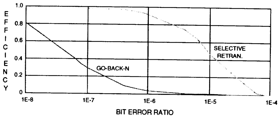
Efficiency of a 45 Mbit/s Satellite Link for a Frame Size of 4096 bytes
