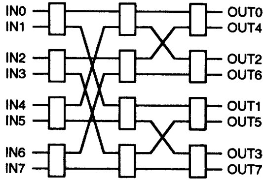
Figure 7-34. MODE A Banyan Routing
