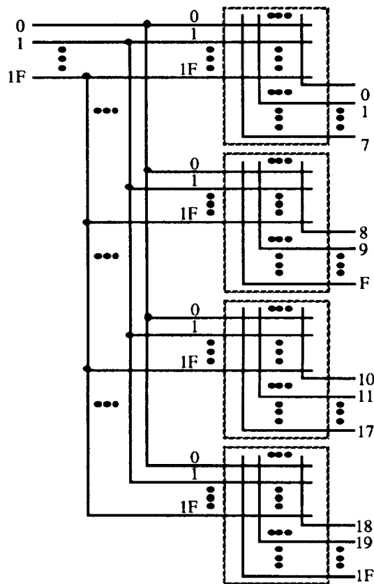
Figure 7-57. 32 x 32 Crossbar-Based Switch Fabric
