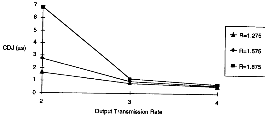
Figure C-20. Cell Delay Jitter vs. Output Transmission Rate for Different Average Arrival Rates
