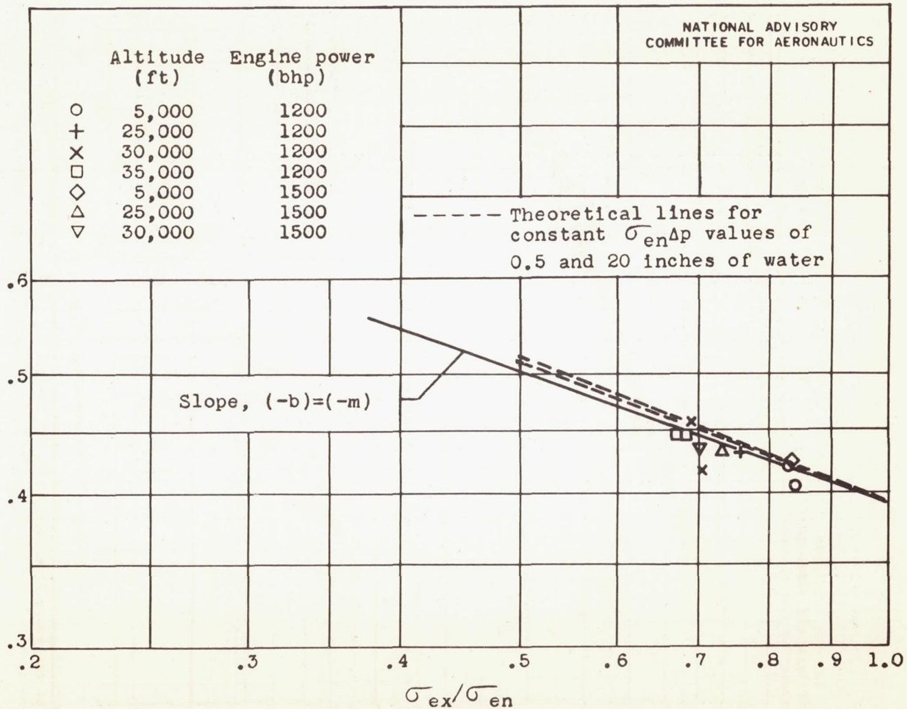
Figure 10.- Test variation of the compressibility function \phi \left( \frac{\sigma_{ex}}{\sigma_{en}} \right) with \sigma_{ex}/\sigma_{en} and comparison with theoretically determined variation.
