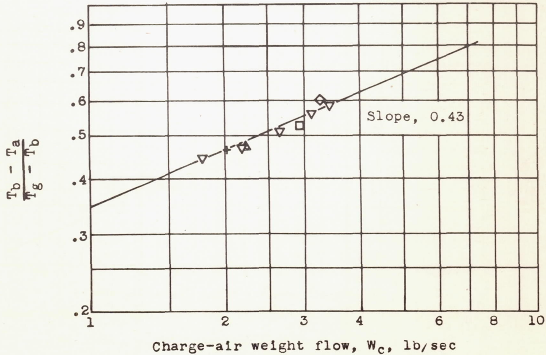
Figure 8.- Variation of \frac{T_h - T_a}{T_g - T_h} and \frac{T_b - T_a}{T_g - T_b} with charge-air weight flow W_c at constant cooling-air pressure drop of 12 and 9 inches of water for heads and barrels, respectively, at altitude of 5000 feet.
