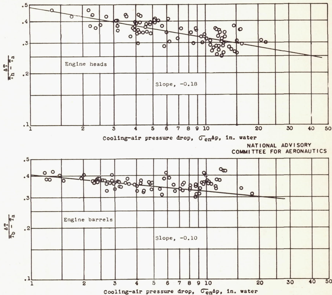
Figure 20.- Variation in cooling-air temperature rise parameter with cooling-air pressure drop \overline{G}_{en}\Delta p for engine heads and barrels.
