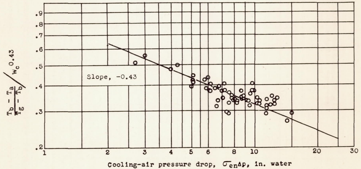
Figure 9. - Cooling-correlation curves based on entrance density for engine heads and barrels at altitude of 5000 feet.
