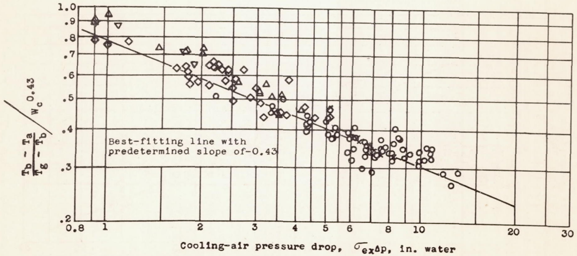
Figure 11.- Cooling-correlation curves based on exit density for engine heads and barrels for altitudes from 5000 to 35,000 feet.
