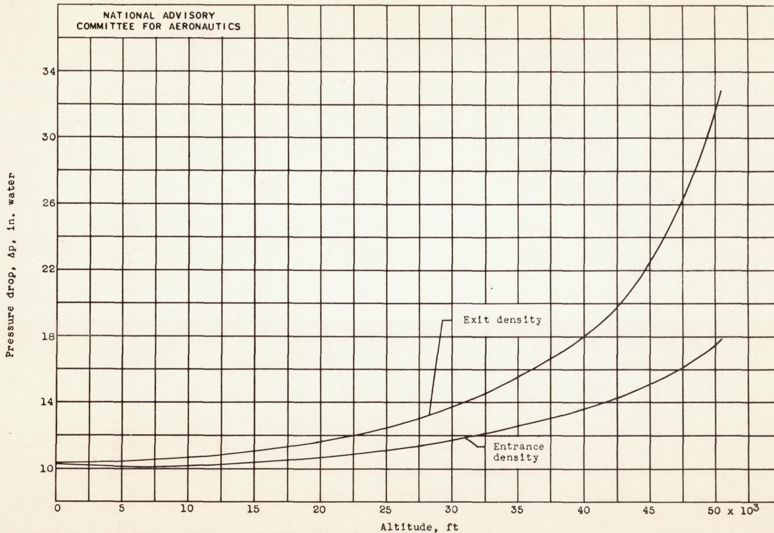
Figure 17. - Calculated variation of pressure drop with altitude necessary to maintain constant head temperature T19. Engine power, 1625 brake horsepower; engine speed, 2400 rpm; charge-air weight flow, 3.5 pounds per second; fuel-air ratio, 0.10; Army summer air.
