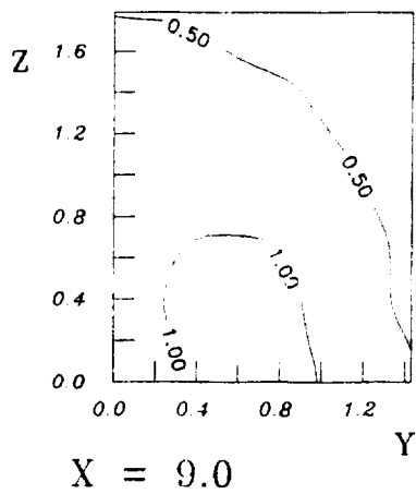
Fig. 43 1x4 Nozzle M=0.09 ww/(UeUe) \times 100
