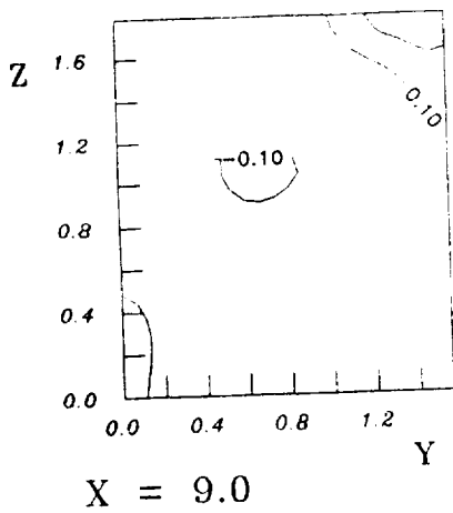
Fig. 30 1x2 Nozzle M=0.09 C.C.(vw)
