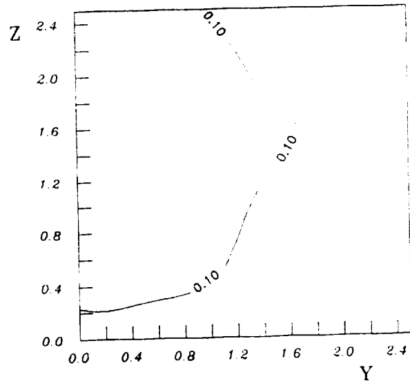
Fig. 45 1x4 Nozzle M=0.09 uw/((UeUe)x100
