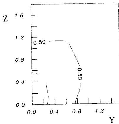
Fig. 63 1x2 Nozzle M=0.9 w_w/(U_e U_e) \times 100
