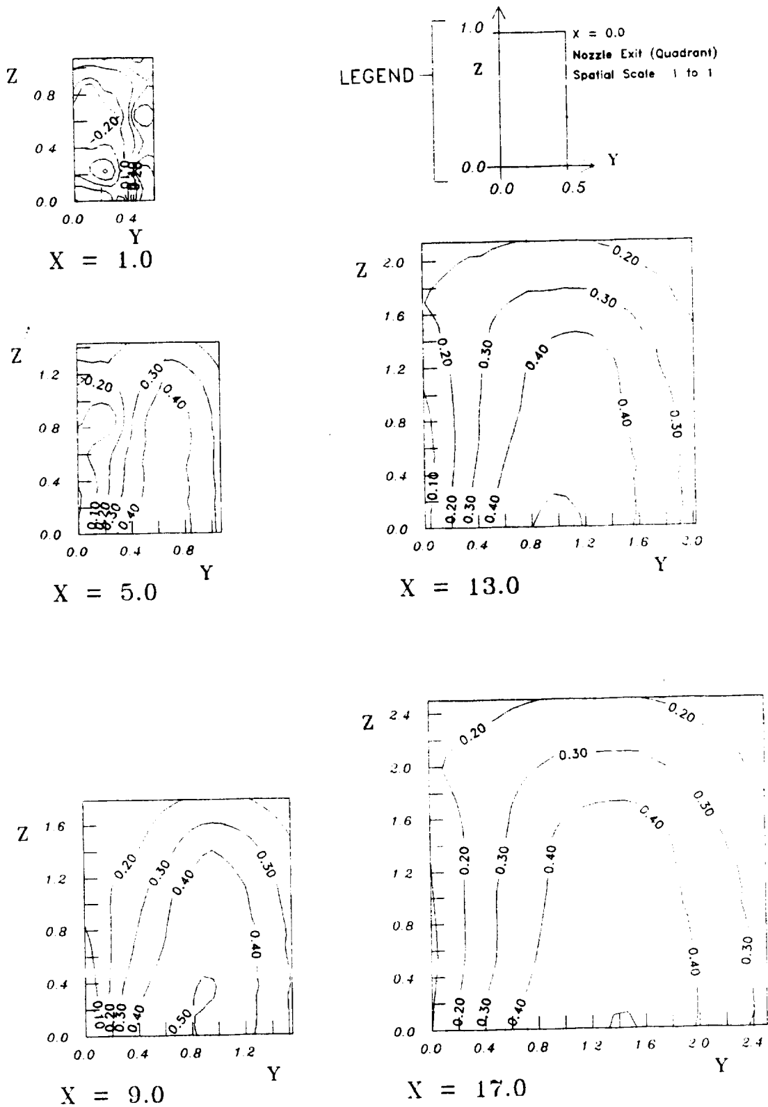
Fig. 68 1x2 Nozzle M=0.9 C.C.(uv)
