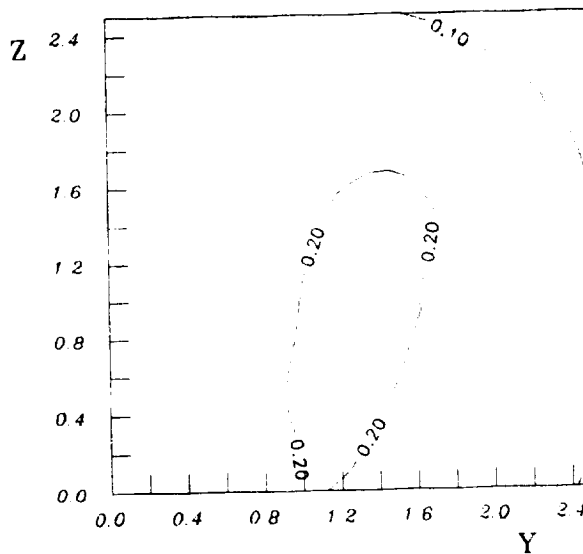
Fig. 70 1x2 Nozzle M=0.9 C.C.(vw)
