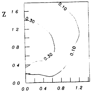
Fig. 45 1x4 Nozzle M=0.09 uw/((UeUe)x100
