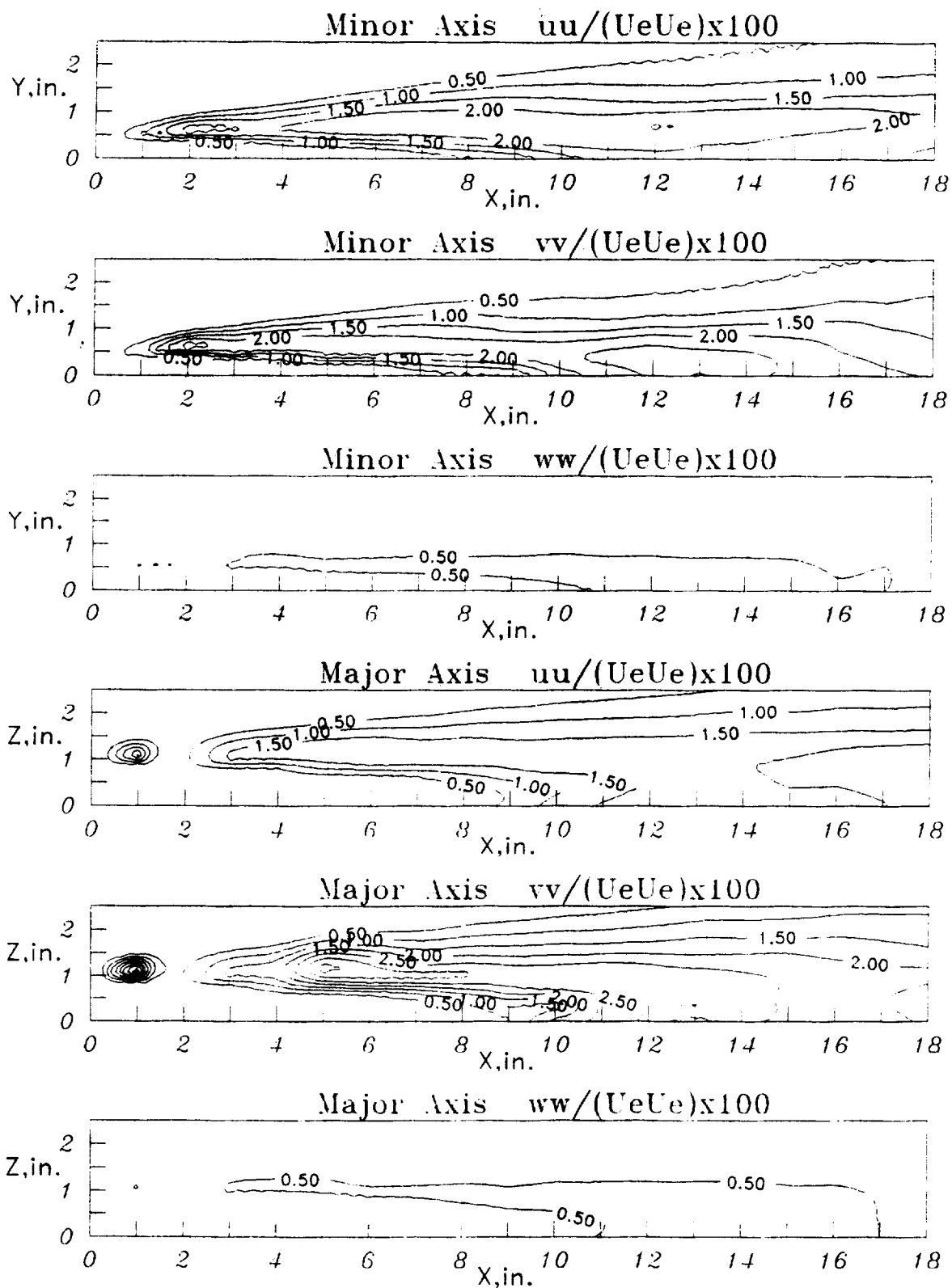
Fig. 53 1x2 Nozzle M=0.9 Velocity Variance
