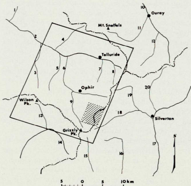
Figure C.5. Generalized geologic location of the Telluride study area. Photo images show region outlined by heavy black lines. Ice Lake Basin training areas outlined by dots. Drainage divides shown by broken lines.
