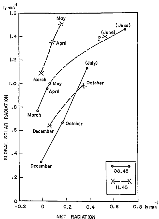
Figure E 2. Comparison of global solar radiation with net radiation.
