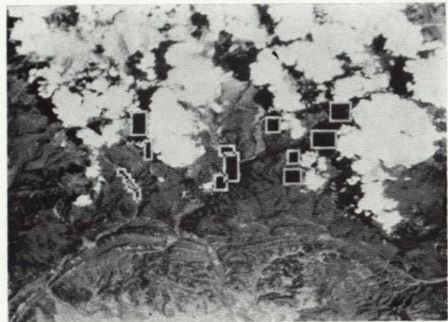
Figure B.16. Training fields of water bodies and shadows.
