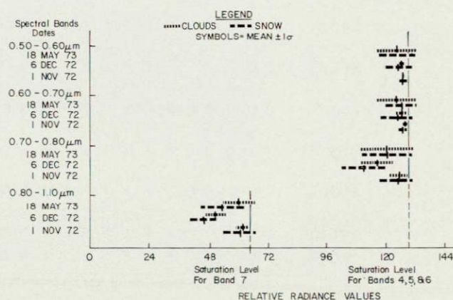
Figure B.15. Statistical analysis of the spectral response of snow and clouds.
