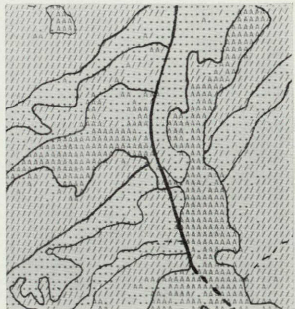
B. Alphanumeric coded DISPLAY image. (A = sandstone, / = shale, . = sandstone.) Photographically reduced from original scale of approximately 1:24,000.
