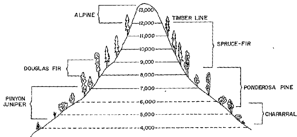
Figure A.2 General elevation ranges of the major cover types found in the San Juan Mountains test site and the Indian Peaks test site.
