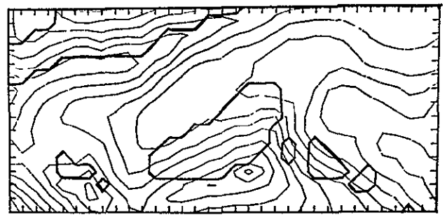
Figure D.1. Examples of output of shadow mapping program. (Shaded areas are outlined by heavier lines superimposed on lighter topographic contour lines; each contour interval represents 200 feet)
