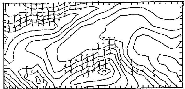
Figure D.2. Modification of output of shadow mapping program. (Arrows indicate areas shaded by nearby topography, whereas S indicates points that are self-shaded)
