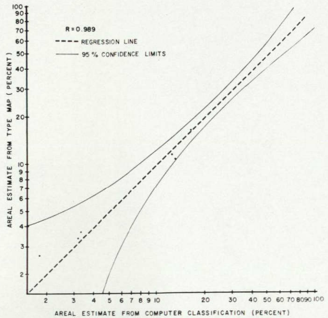
Figure A.15. Ward-Monarch intensive study area comparison between areal estimates obtained by computer classification and those obtained by planimetry of the cover type map.
