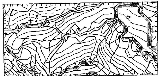
Figure D.4. Output of shadow mapping program showing areas having similar aspects.
