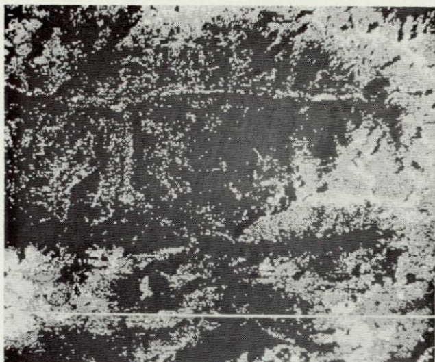
Figure C.4. Distribution of major lithologic classes, based on computer-aided analysis of ERTS MSS data. (Black = areas primarily underlain by sedimentary rocks, gray = areas of intrusive and extrusive igneous rocks, white = areas covered by unconsolidated rock material.)
