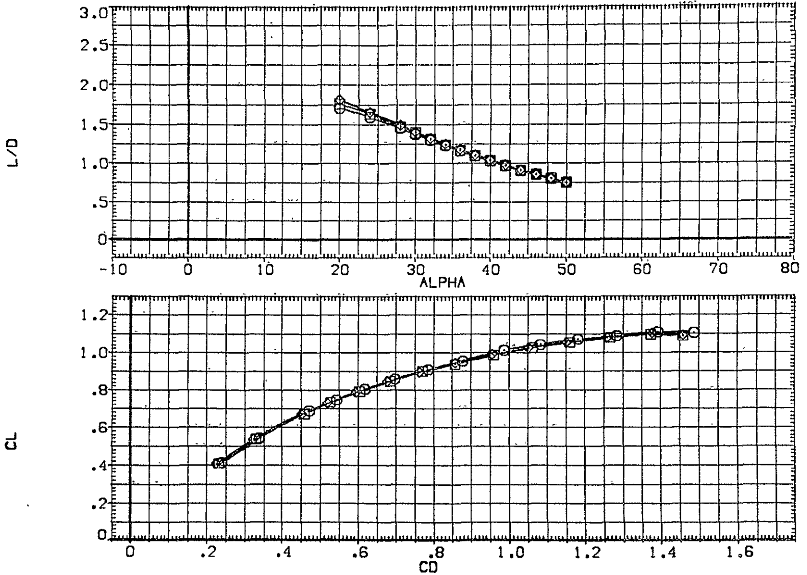
FIGURE 6 EFFECT OF REYNOLDS NUMBER (ELEVON= 10, BDFLAP= 16.3).
