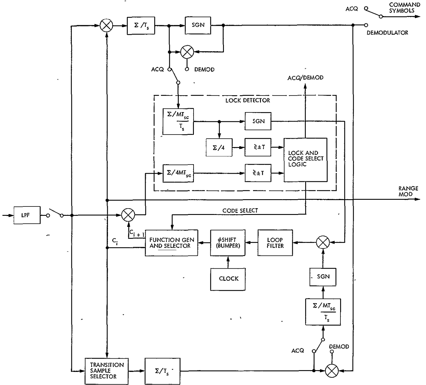
Fig. 4. Revised block diagram of demodulator/detector
