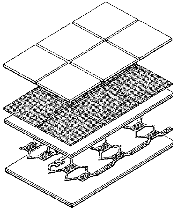
Figure 3.3-4 Lockheed Communications Satellite Substrate Design (Conventional Cells)
