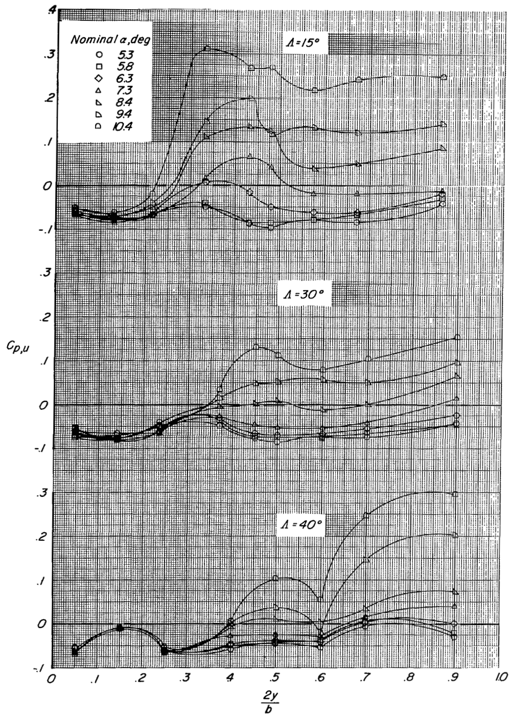
Figure 6.- Effect of angles of attack and sweepback on the trailing-edge flow separation at x/c = 1.00 of a variable-sweep wing. Fuselage off.
