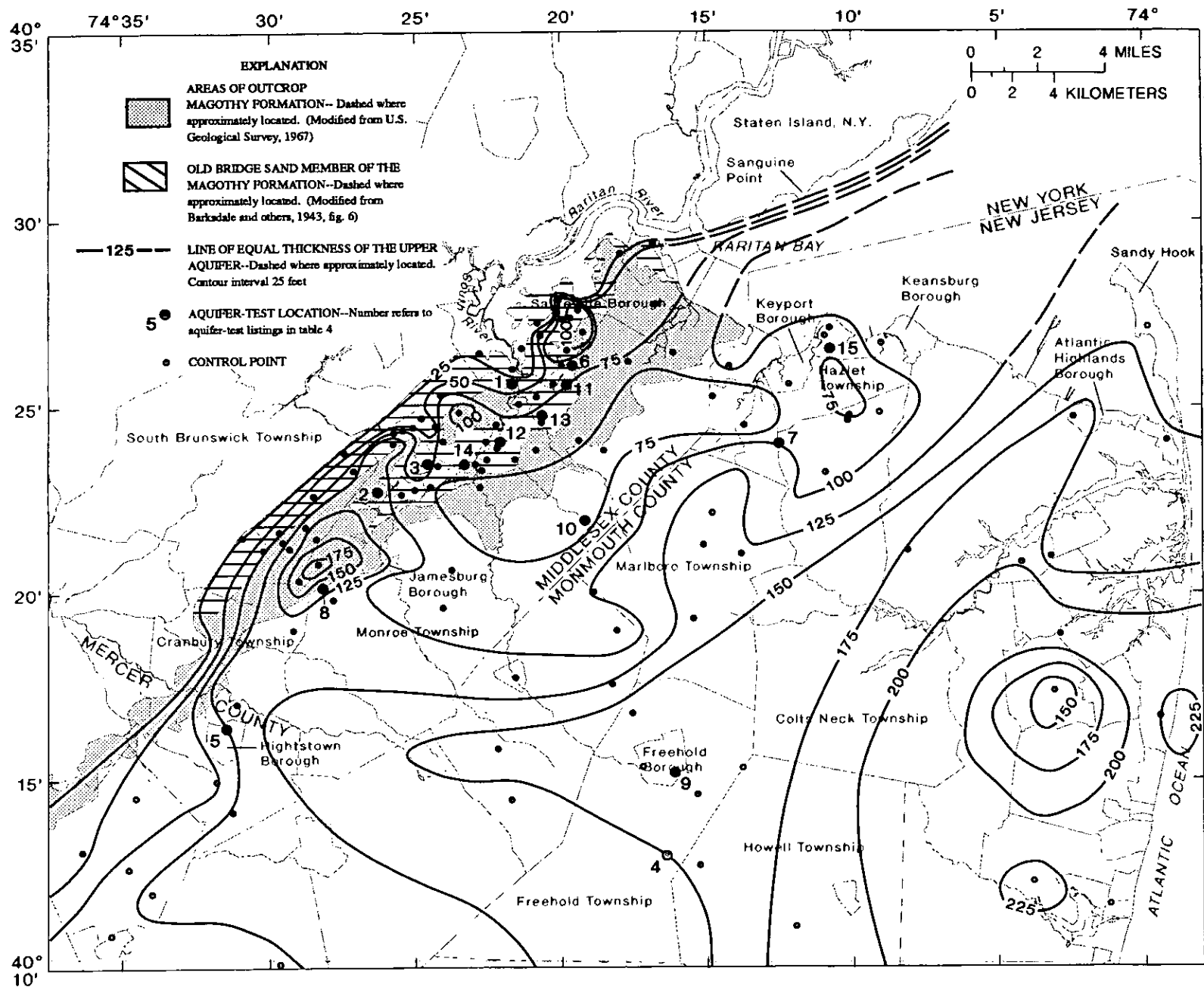
Figure 5.--Thickness of the upper aquifer. (Modified from Gronberg and others, 1991, pl. 7)
