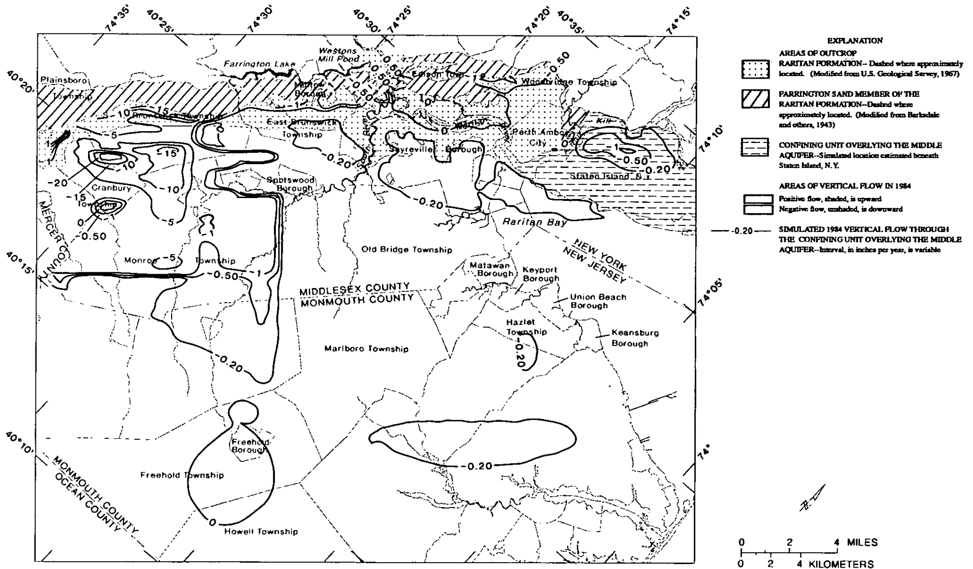
Figure 42.--Simulated vertical flow through the confining unit overlying the middle aquifer, 1984.
