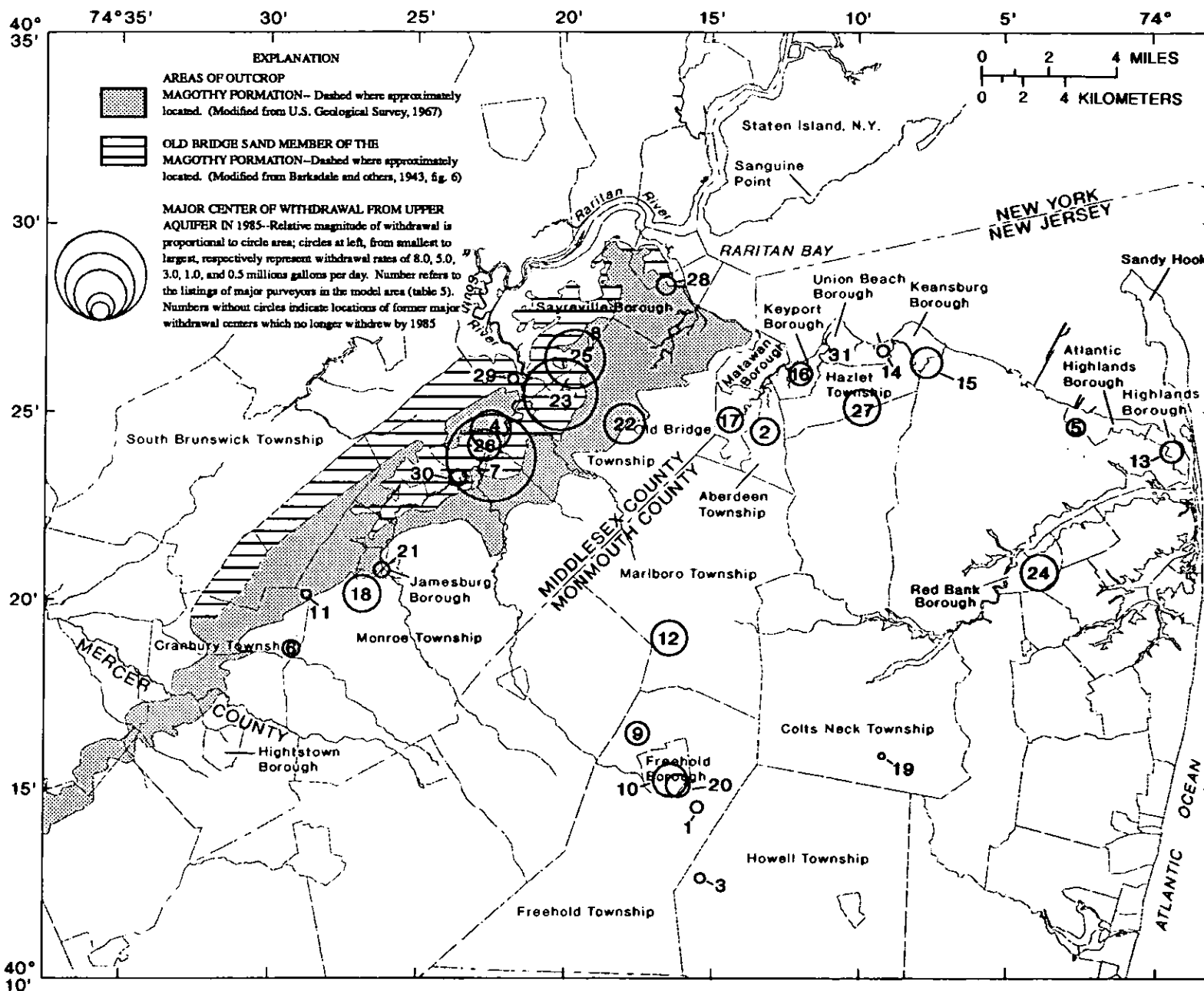
Figure 6.--Locations of major withdrawal centers in the upper aquifer, 1985.
