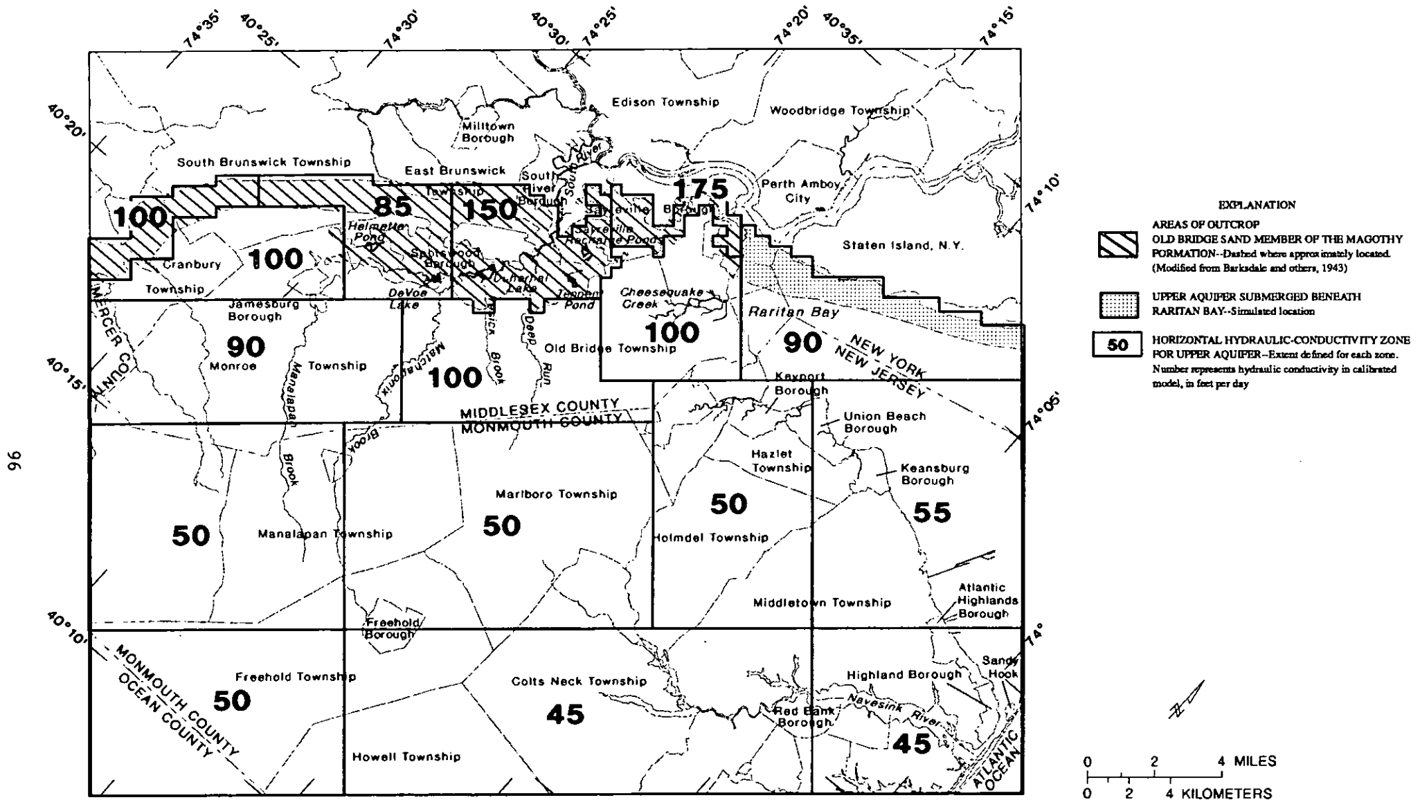
Figure 33.--Horizontal hydraulic conductivities estimated by the calibrated model for the upper aquifer.
