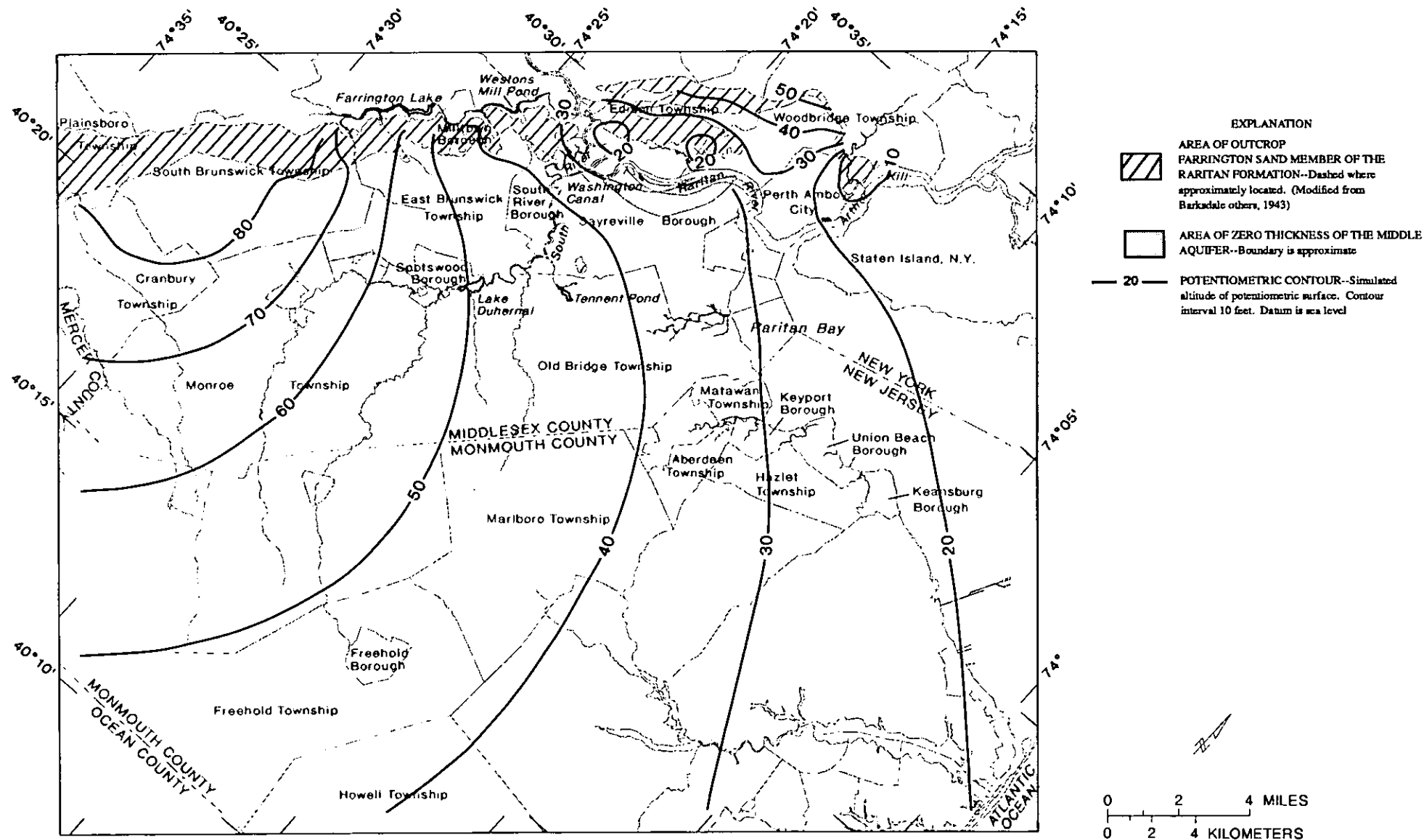
Figure 30.--Simulated predevelopment potentiometric surface in the middle aquifer.
