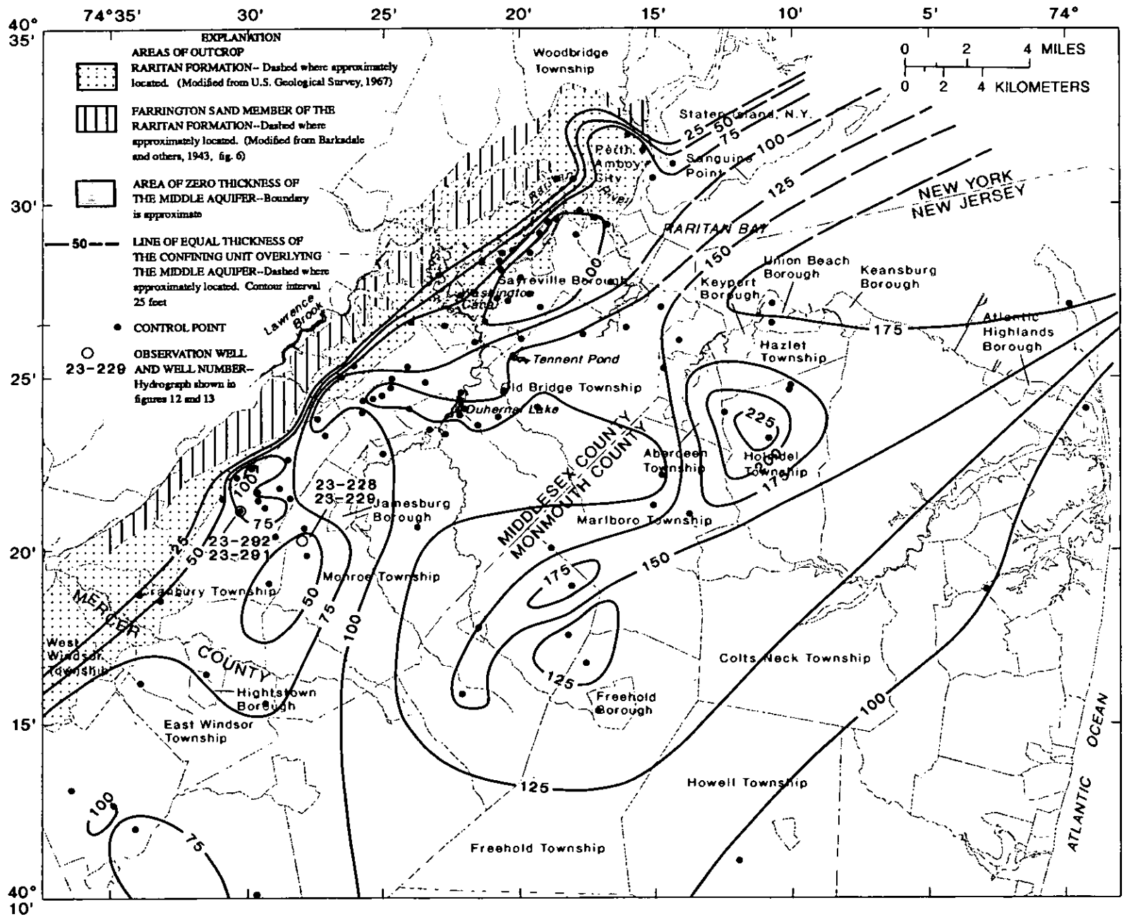
Figure 11.--Thickness of the confining unit overlying the middle aquifer. (Modified from Gronberg and others, 1991, pl.5)
