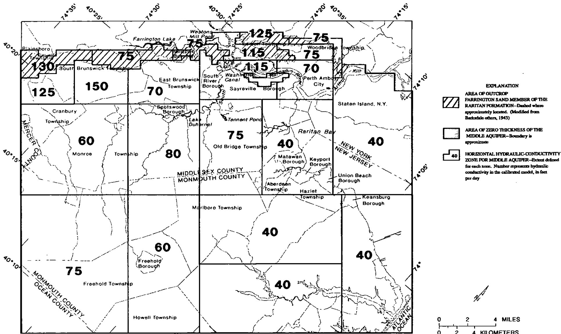
Figure 34.--Horizontal hydraulic conductivities estimated by the calibrated model for the middle aquifer.
