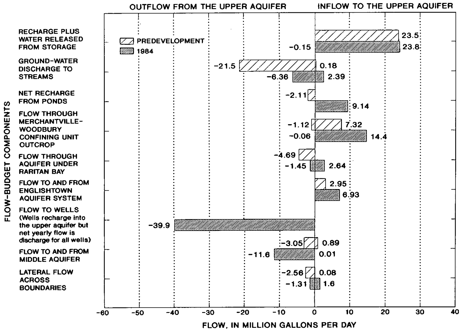
Figure 38.--Flow budgets for the upper aquifer in the predevelopment and 1984 transient flow systems.
