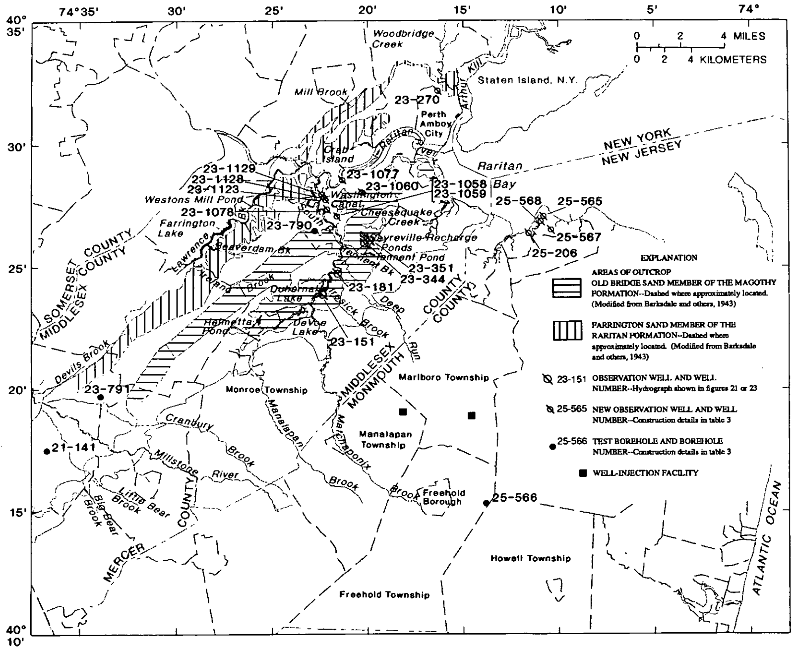
Figure 22.--Locations of selected observation wells, test boreholes, and artificial-recharge ponds, and location of injection-well facility, Potomac-Raritan-Magothy aquifer system.
