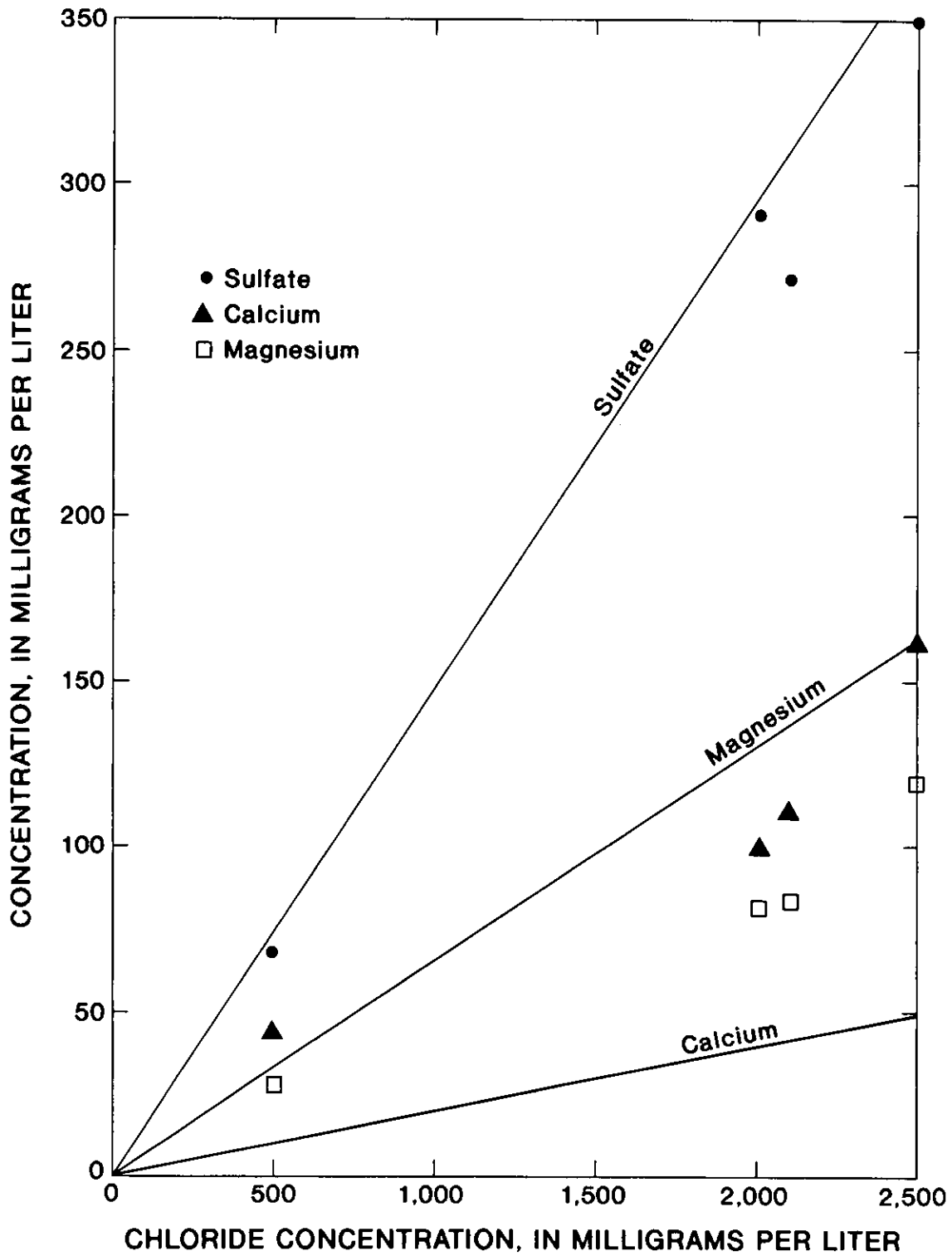
Figure 60 --Relation of sulfate, calcium, and magnesium concentrations to chloride concentrations in water samples from wells 25-207, 25-208, 25-420, and 25-568. (All wells are screened in the upper aquifer within the saltwater plume in Union Beach Borough. Well locations are shown in fig. 55; results of chemical analyses of water samples are listed in table 14)
