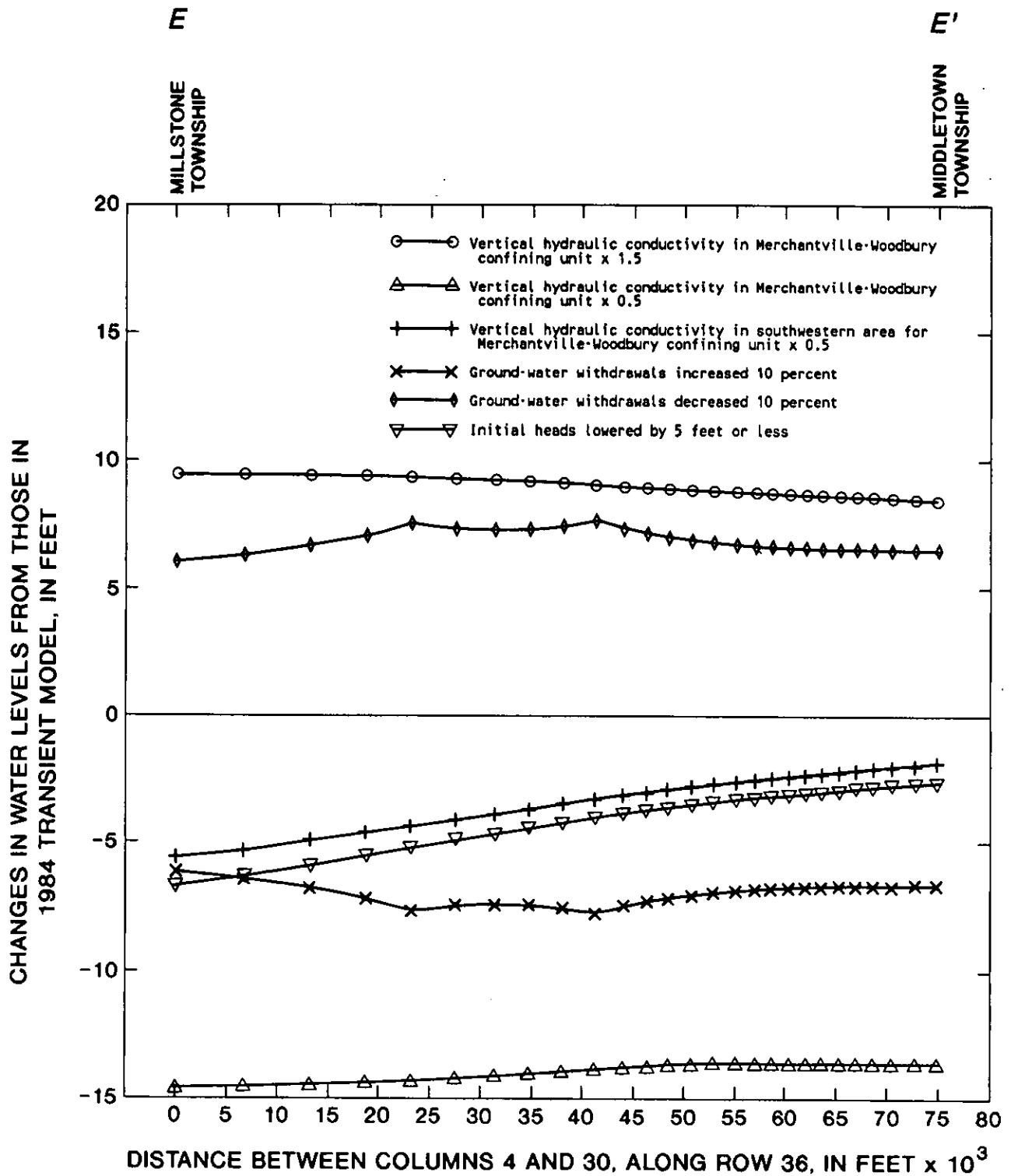
Figure 45.--Simulated head changes in the upper aquifer along model row 36 in response to sensitivity tests of vertical hydraulic conductivity in the Merchantville-Woodbury confining unit, ground-water withdrawals, and initial heads in the aquifer outcrop. (Location of row shown in fig. 25)
