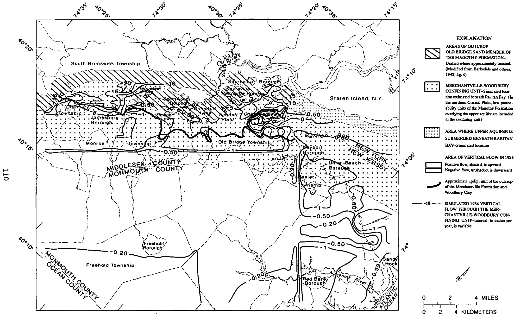
Figure 41.--Simulated vertical flow through the Merchantville-Woodbury confining unit, 1984.
