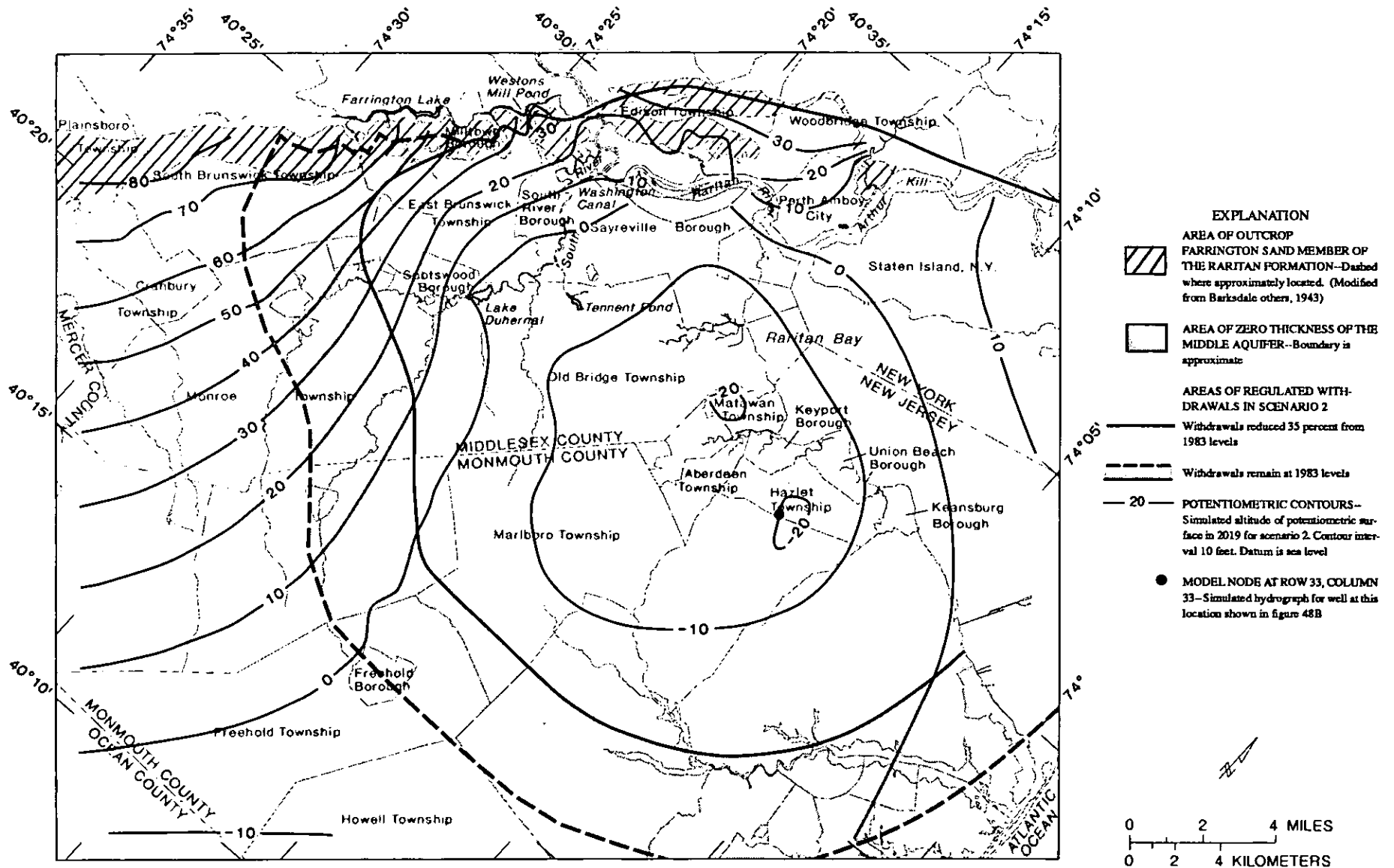
Figure 52.--Simulated potentiometric surface in 2019 in the middle aquifer, scenario 2.
