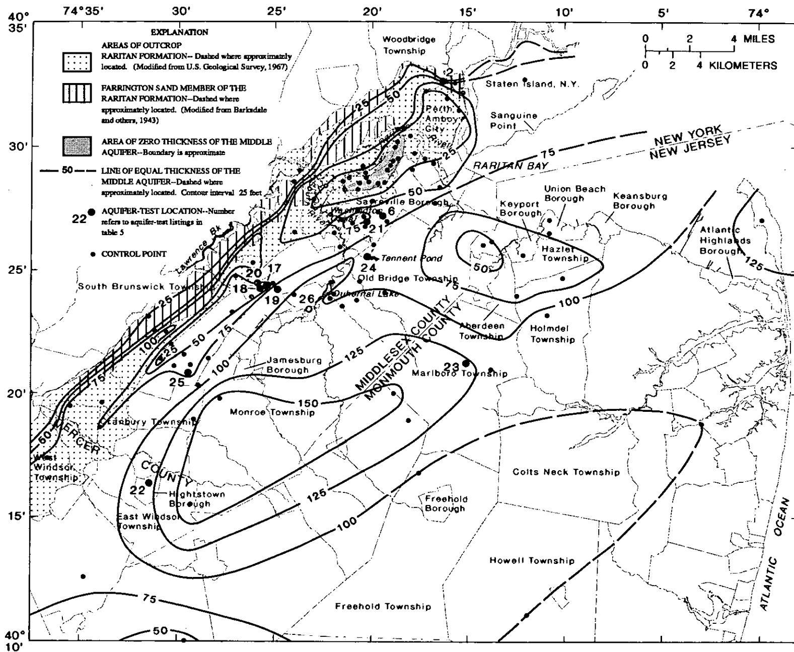
Figure 15.--Thickness of the middle aquifer. (Modified from Gronberg and others, 1991, pl.4)
