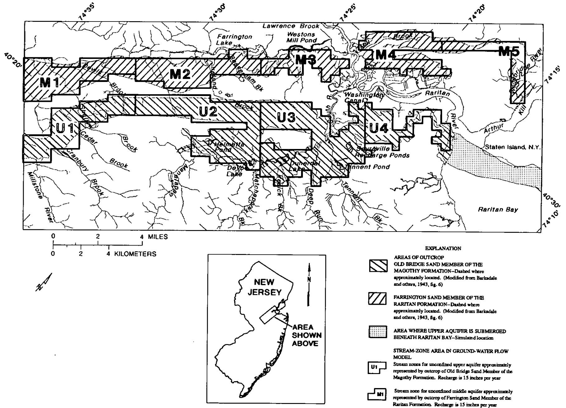
Figure 28.--Simulated stream zones in the outcrop areas of the upper and middle aquifers.
