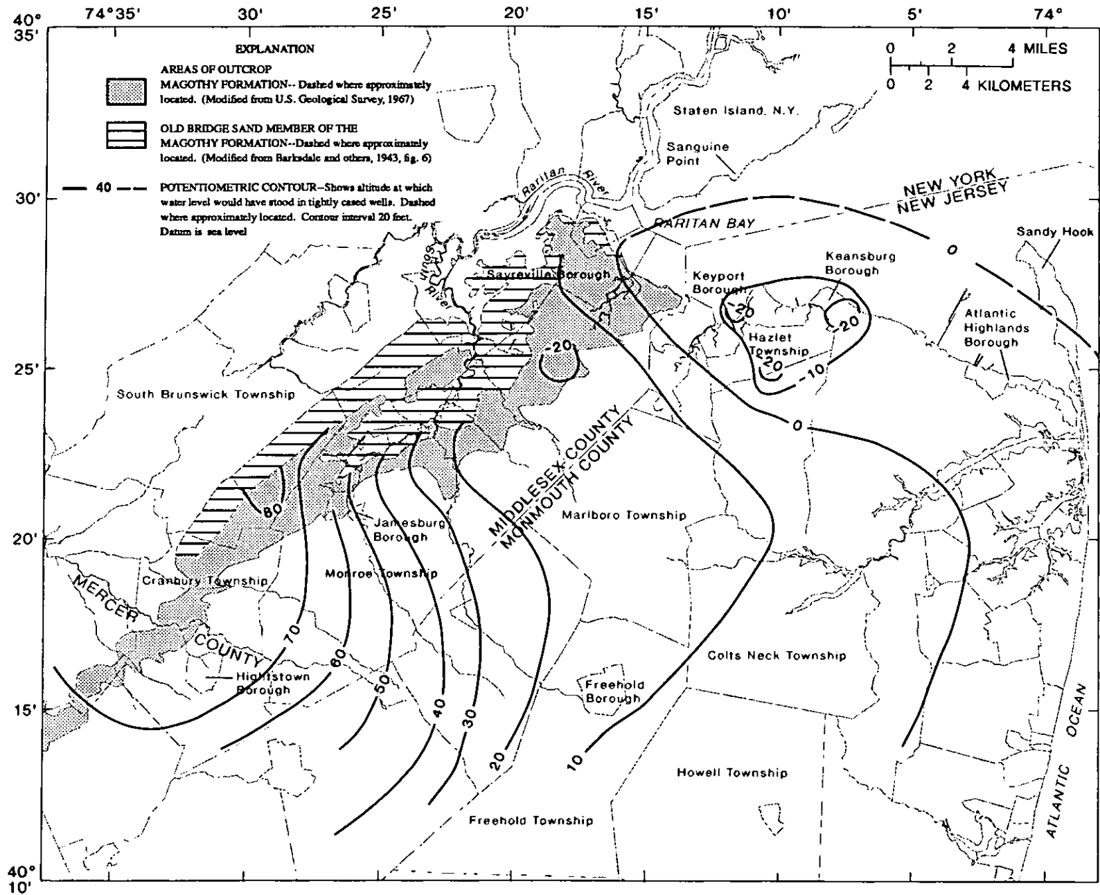
Figure 9.--Potentiometric surface in the upper aquifer, 1959. (From Farlekas, 1979, fig. 10)
