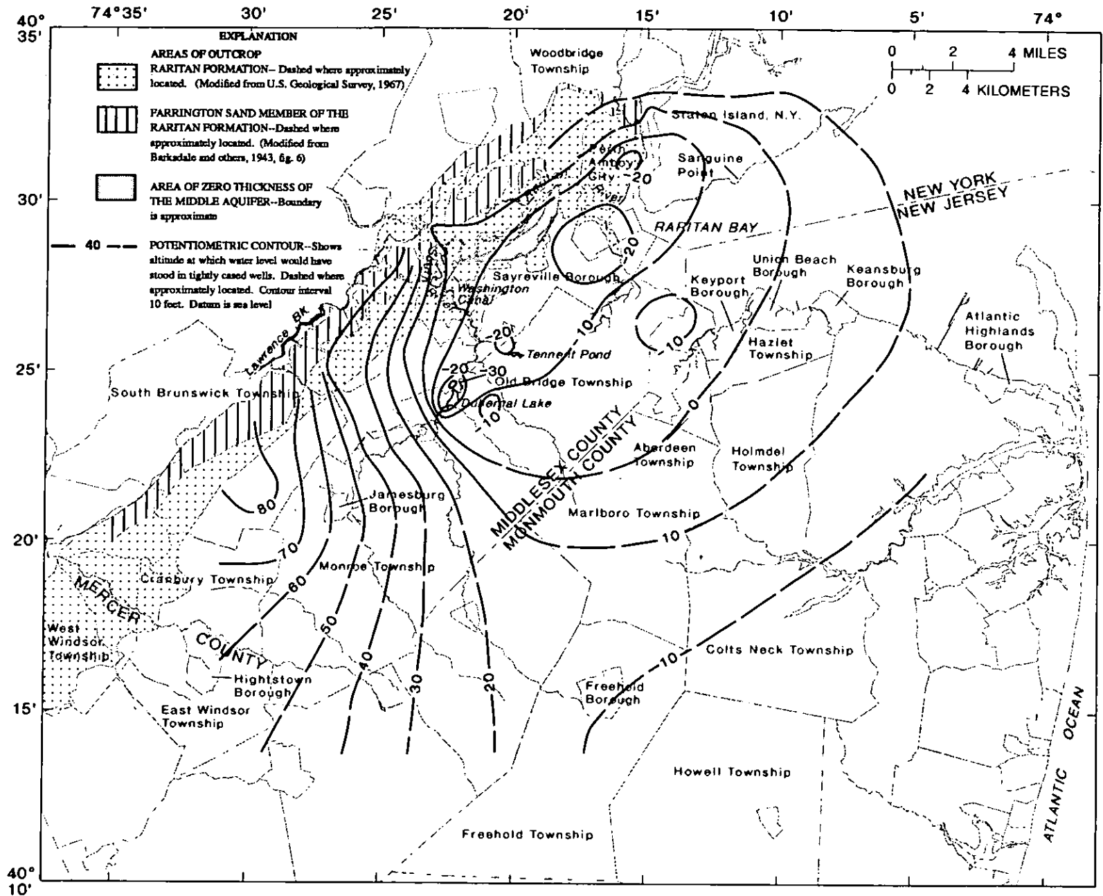
Figure 19.--Potentiometric surface in the middle aquifer, 1983. (From Eckel and Walker, 1986)
