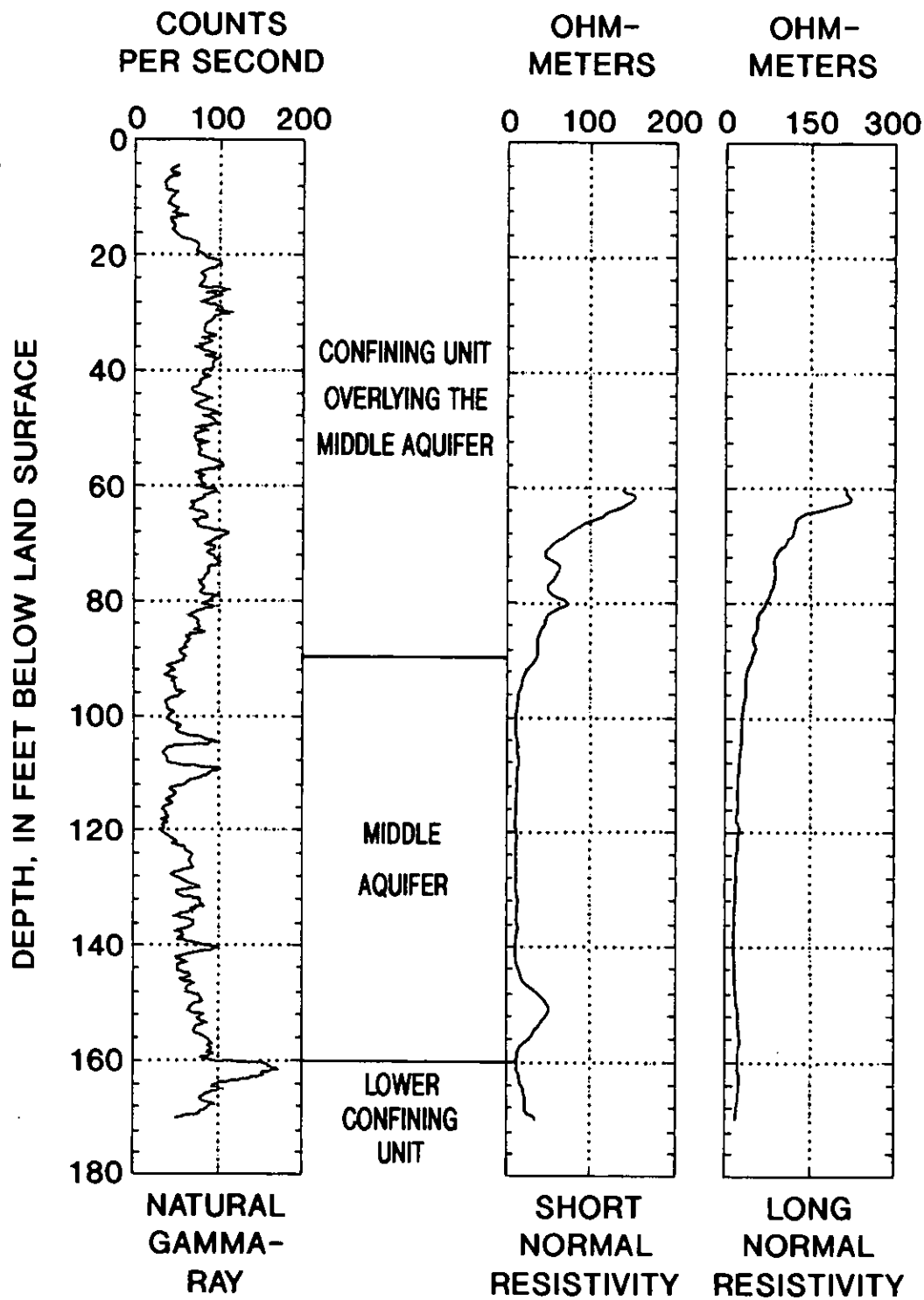
Figure 63.--Natural-gamma and electrical-resistivity logs of test well 23-1059. (Location of well shown in fig. 62)
