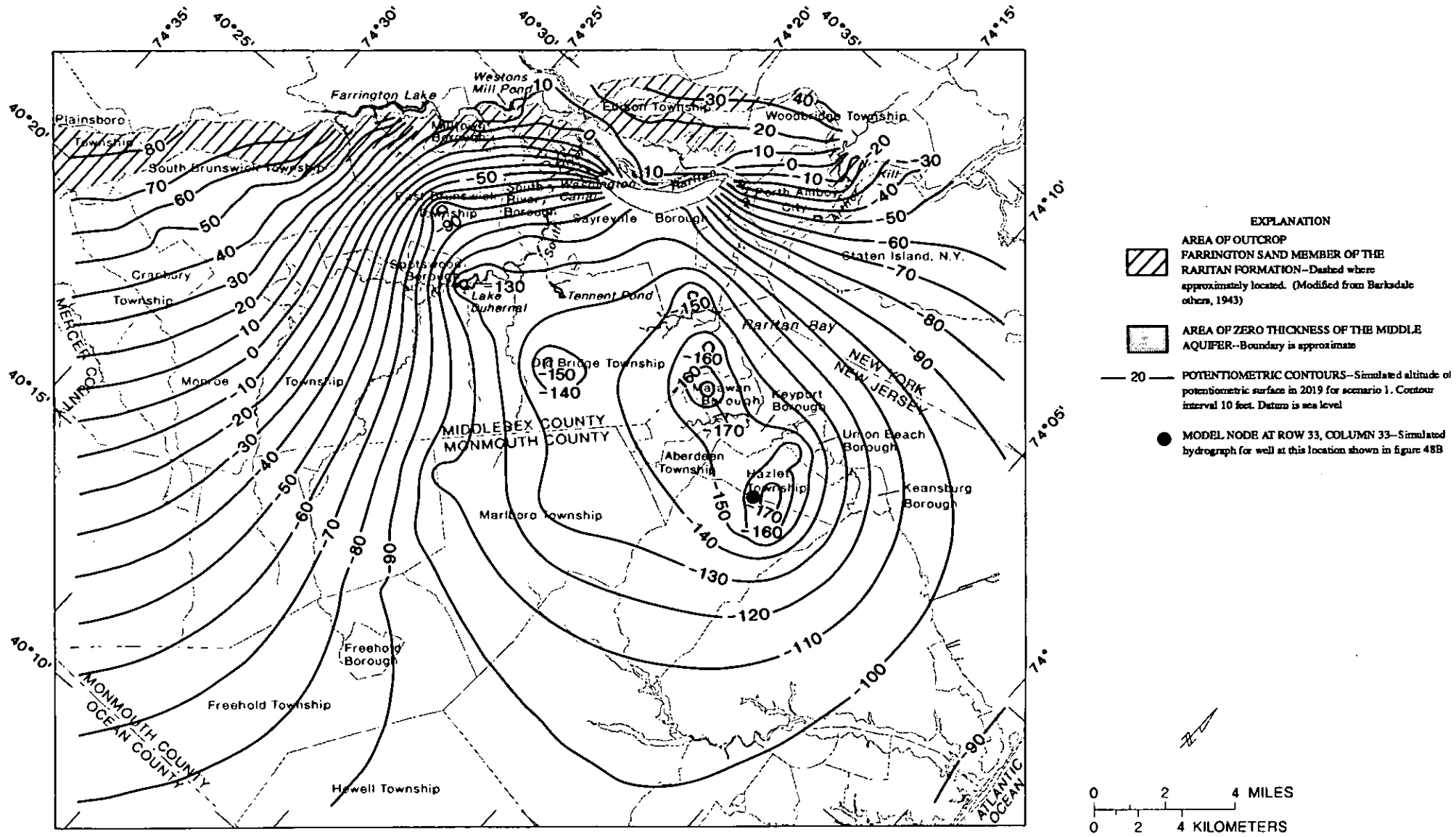
Figure 50.--Simulated potentiometric surface in 2019 in the middle aquifer, scenario 1.
