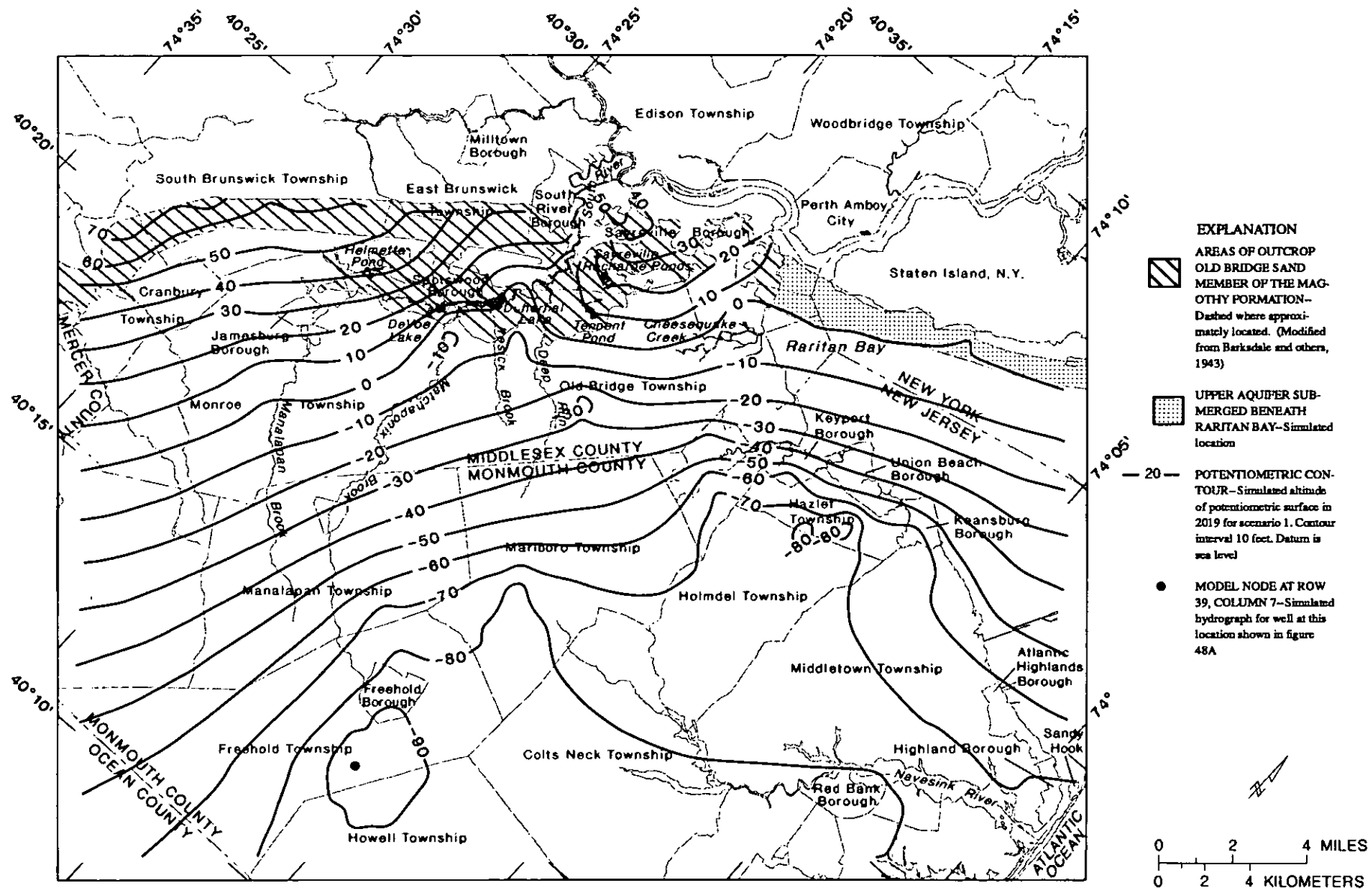
Figure 49.--Simulated potentiometric surface in 2019 in the upper aquifer, scenario 1.
