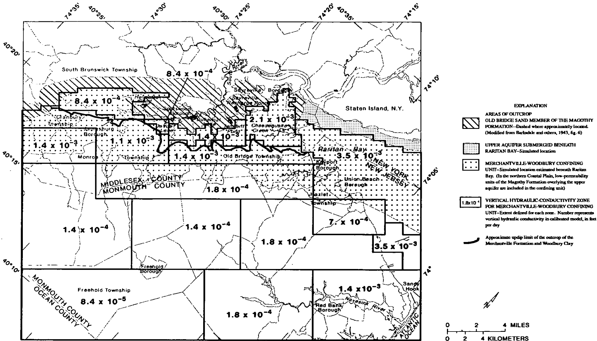
Figure 35.--Vertical hydraulic conductivities estimated by the calibrated model for the Merchantville-Woodbury confining unit.
