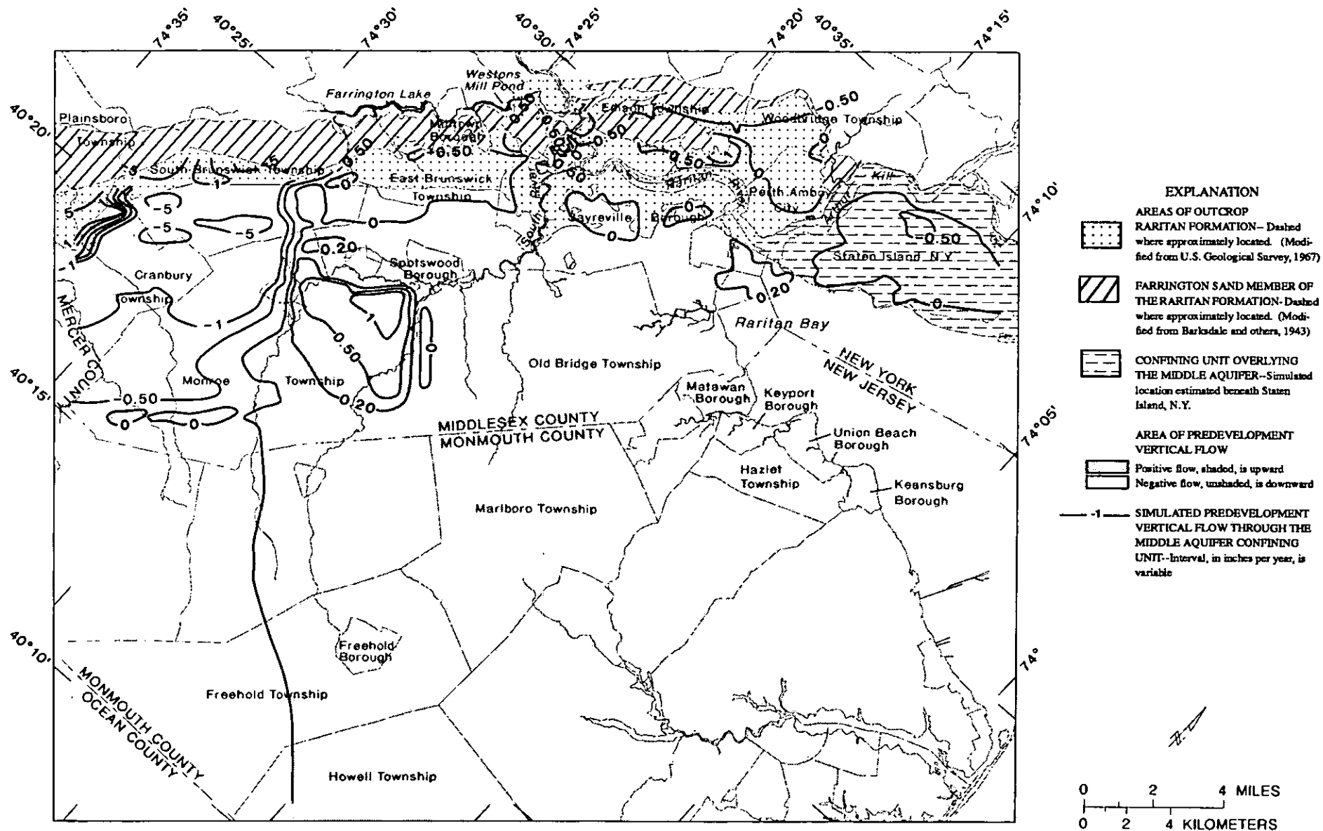
Figure 39.--Simulated predevelopment vertical flow through the confining unit overlying the middle aquifer.
