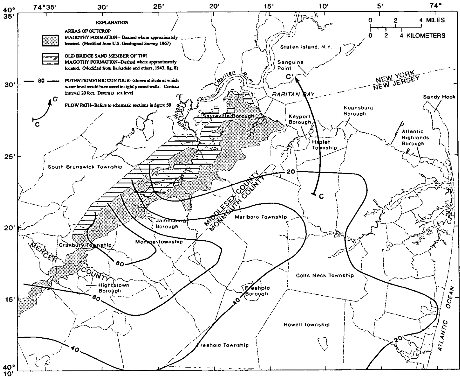
Figure 8.--Predevelopment potentiometric surface in the upper aquifer. (Modified from Zapecza and others, 1987, fig. 4)
