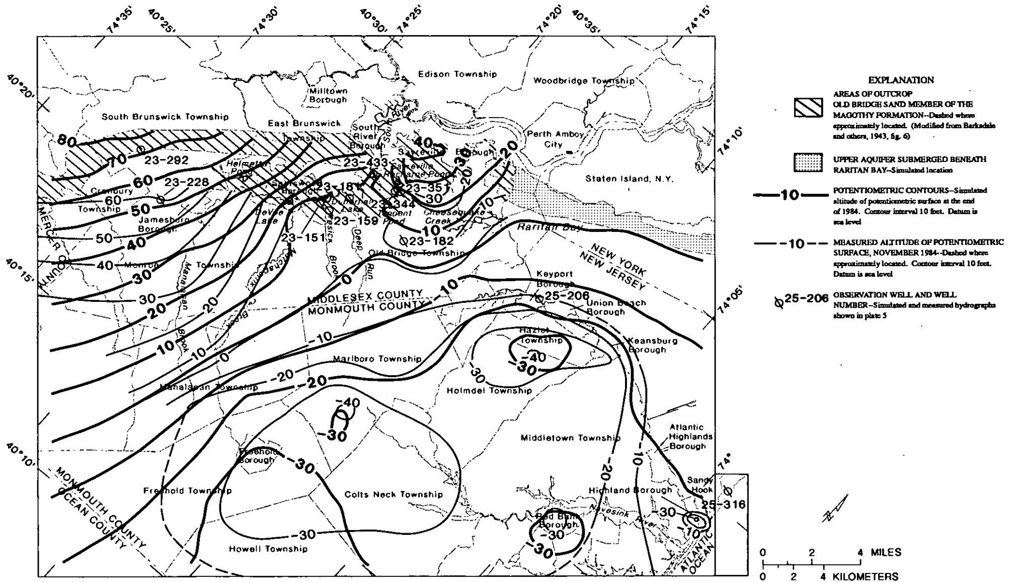
Figure 31.--Simulated and interpreted potentiometric surfaces in the upper aquifer, 1984.
