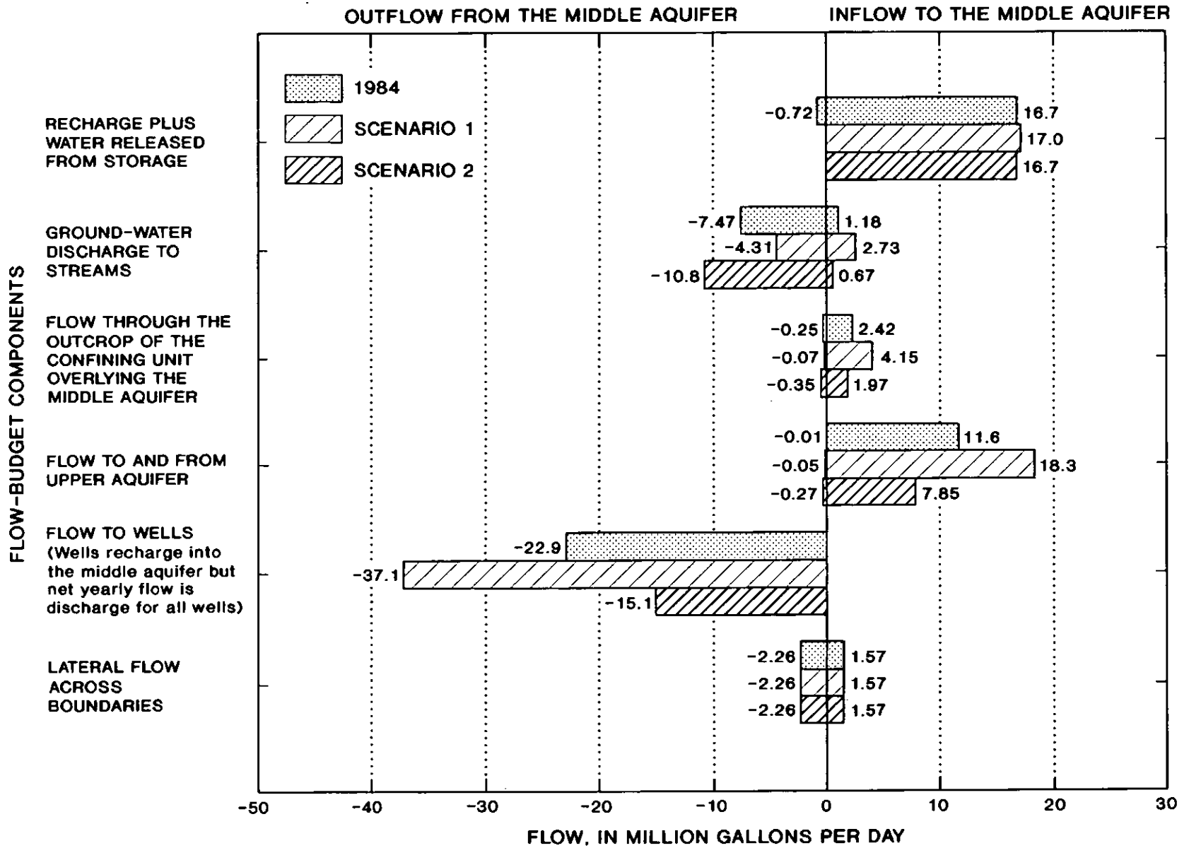
Figure 54.--Flow budget for simulated ground-water flow in 2019 for scenarios 1 and 2 in the middle aquifer.
