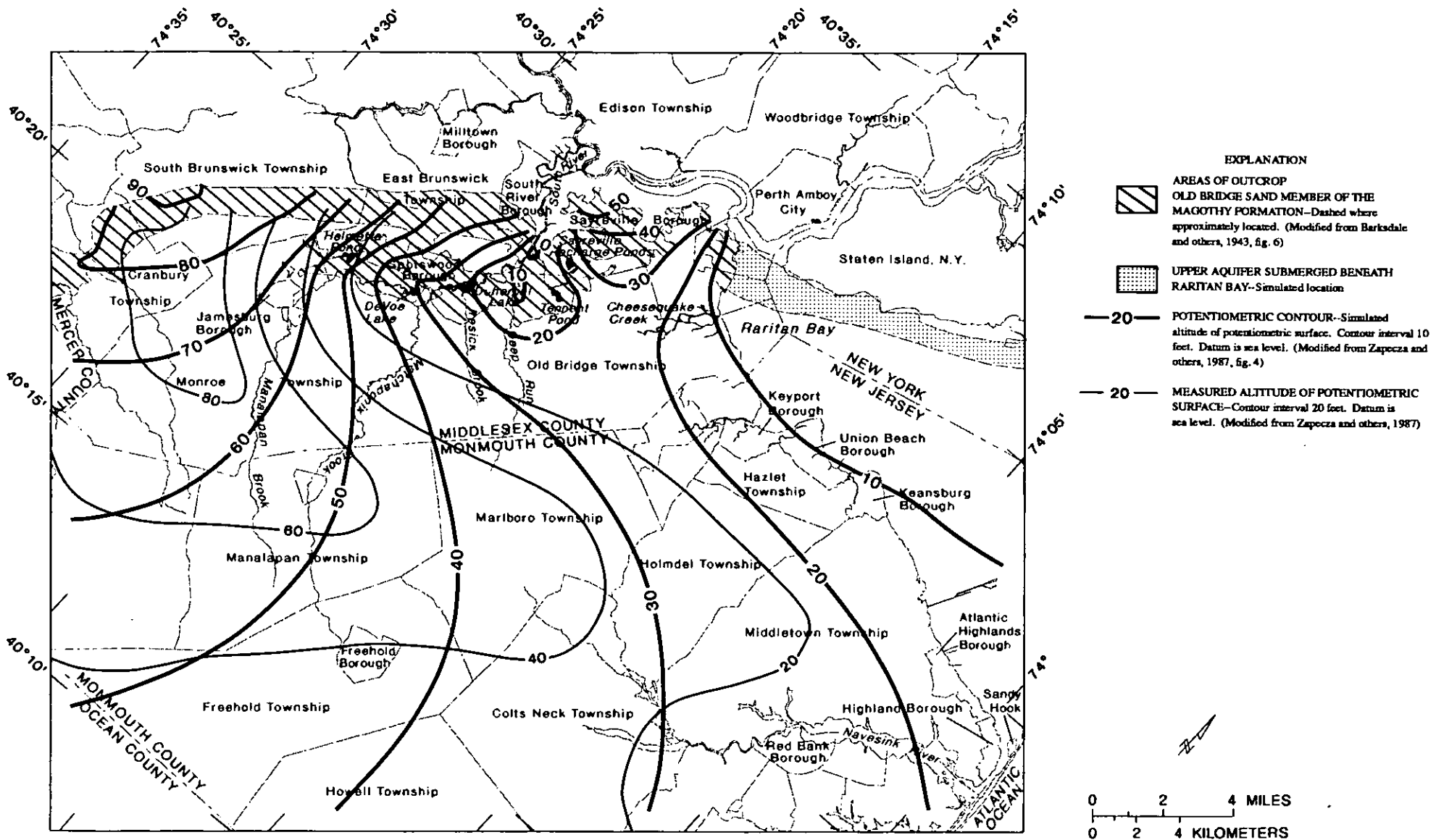
Figure 29.--Simulated and interpreted predevelopment potentiometric surfaces in the upper aquifer.
