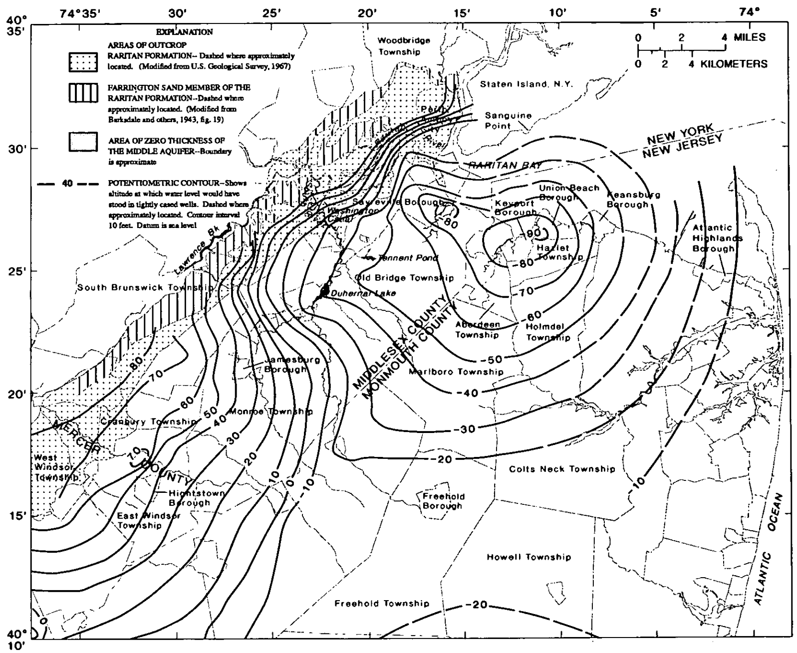
Figure 18.--Potentiometric surface in the middle aquifer, 1959. (From Farlekas, 1979)
