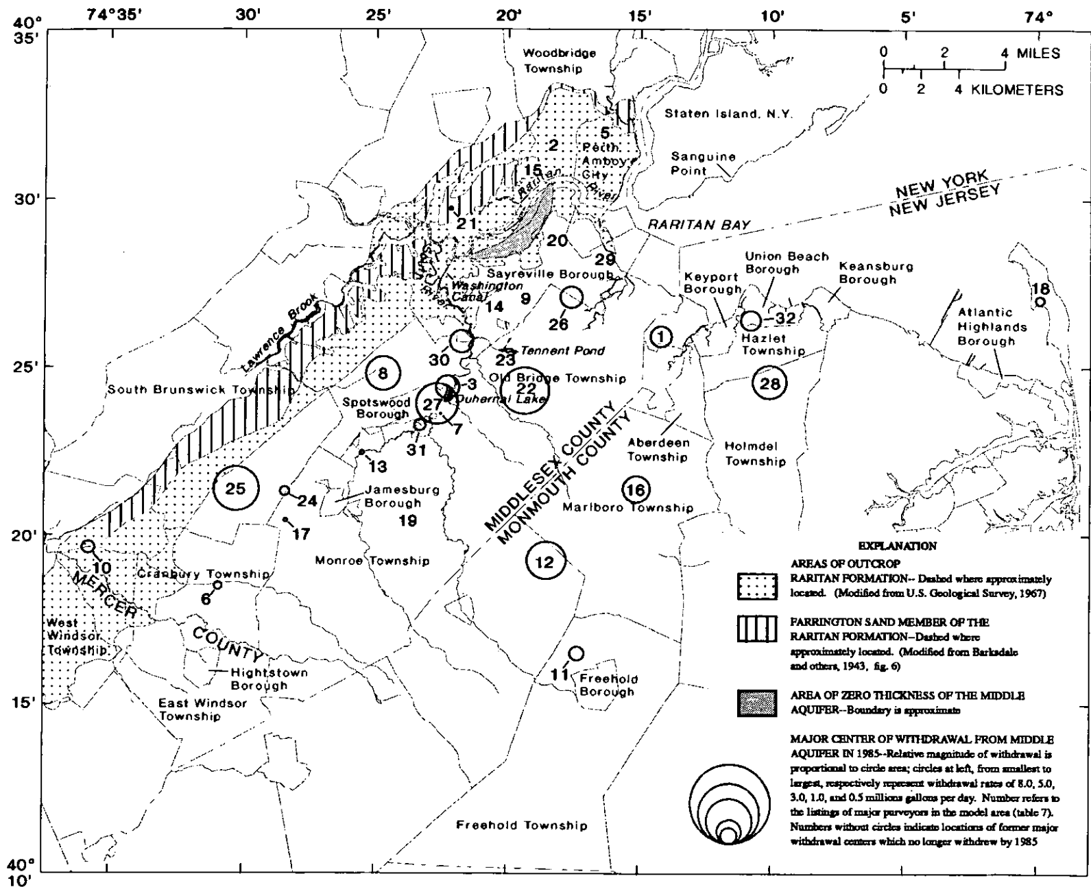
Figure 16.--Locations of major withdrawal centers in the middle aquifer, 1985.
