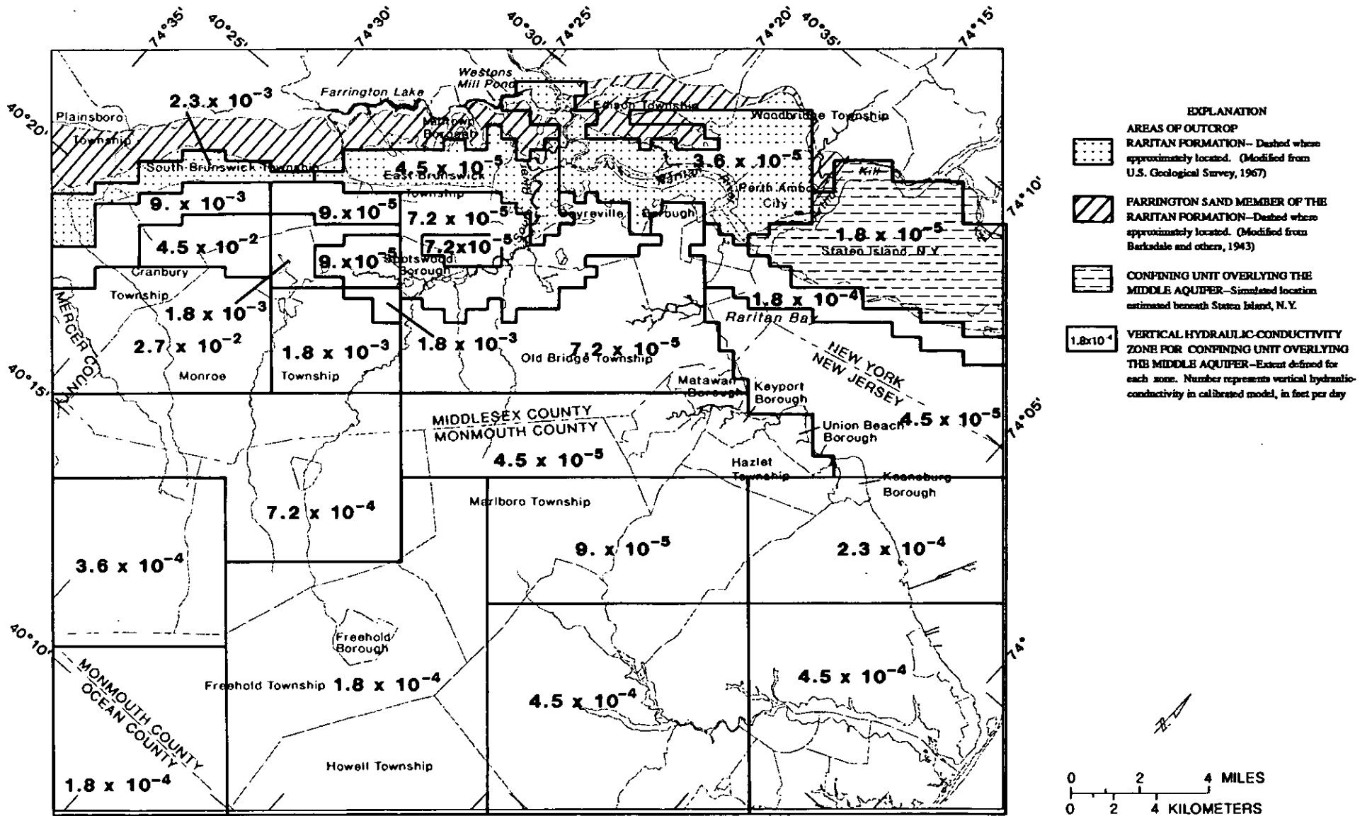
Figure 36.--Vertical hydraulic conductivities estimated by the calibrated model for the confining unit overlying the middle aquifer.
