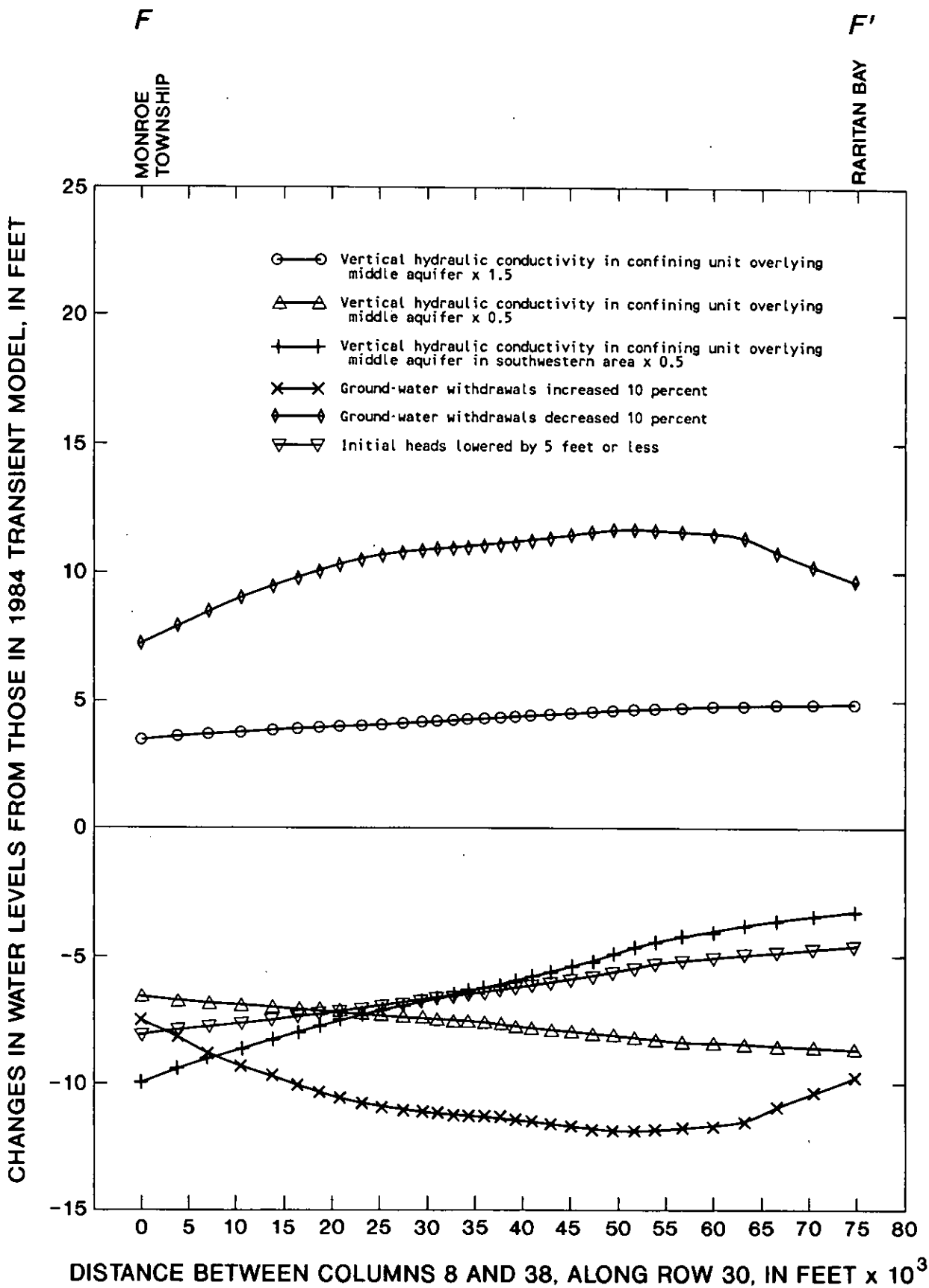
Figure 46.--Simulated head changes in the middle aquifer along model row 30 in response to sensitivity tests of vertical hydraulic conductivity in the confining unit overlying the middle aquifer, ground-water withdrawals, and initial heads in the aquifer outcrop. (Location of row shown in fig. 25)
