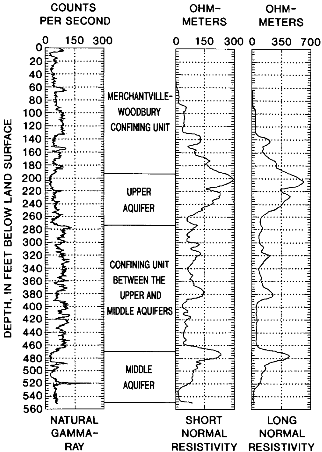
Figure 57.--Natural-gamma and electrical-resistivity logs of test borehole 25-565. (Location of borehole shown in fig. 55)
