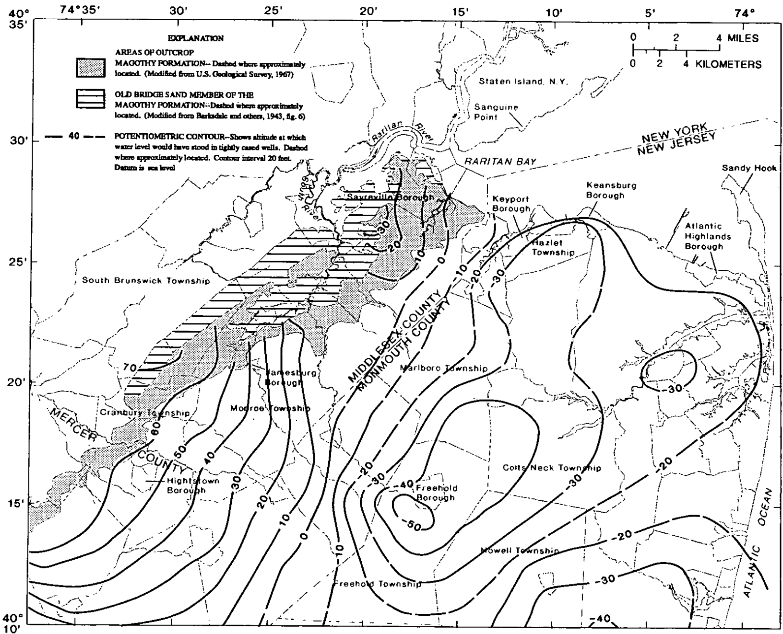
Figure 10.--Potentiometric surface in the upper aquifer, 1983. (Modified from Eckel and Walker, 1986, pl. 3)
