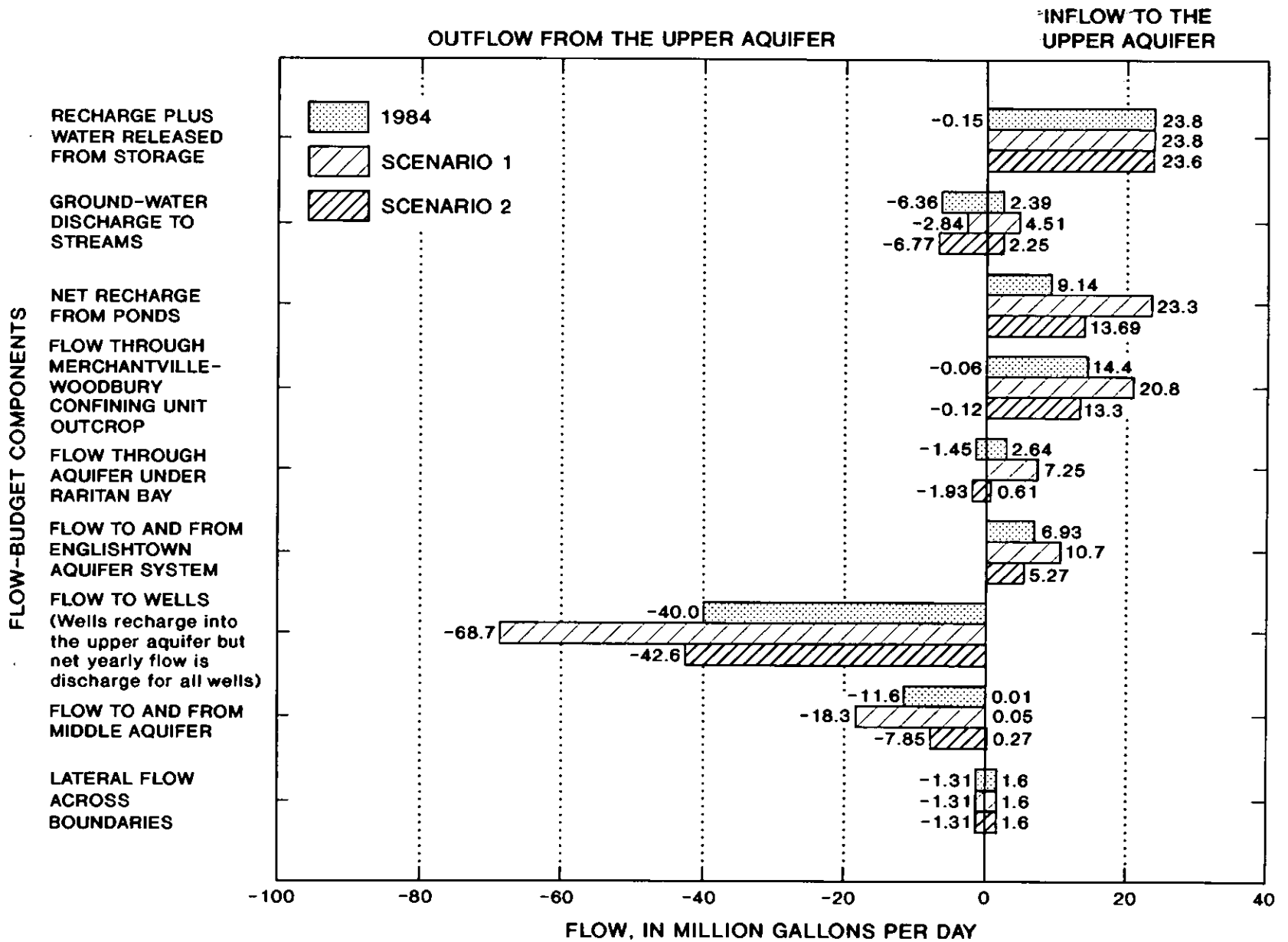
Figure 53.--Flow budget for simulated ground-water flow in 2019 for scenarios 1 and 2 in the upper aquifer.
