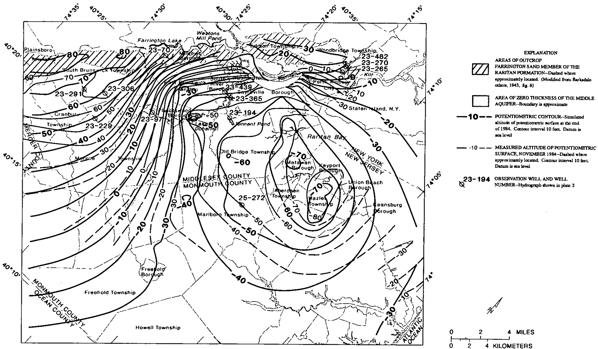
Figure 32.--Simulated and interpreted potentiometric surfaces in the middle aquifer, 1984.
