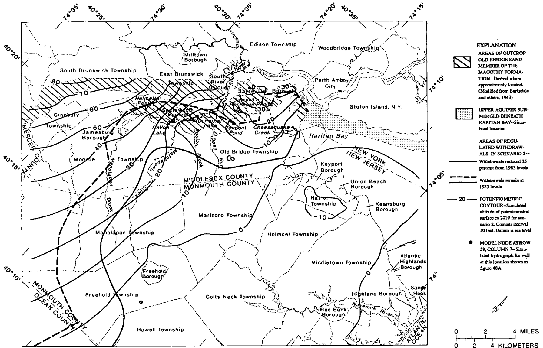
Figure 51.--Simulated potentiometric surface in 2019 in the upper aquifer, scenario 2.
