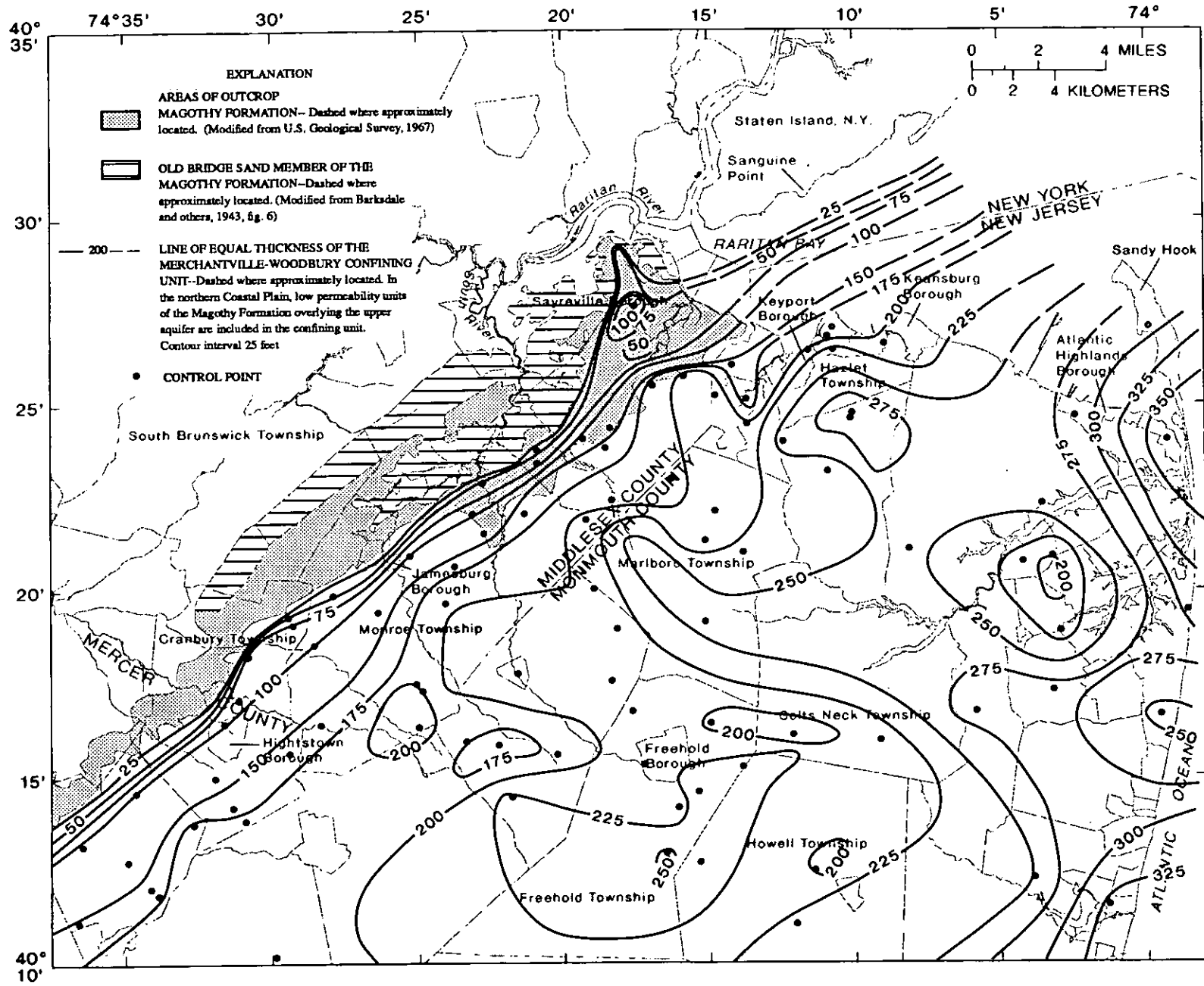
Figure 3.--Thickness of the Merchantville-Woodbury confining unit. (Modified from Gronberg and others, 1991, pl. 8)
