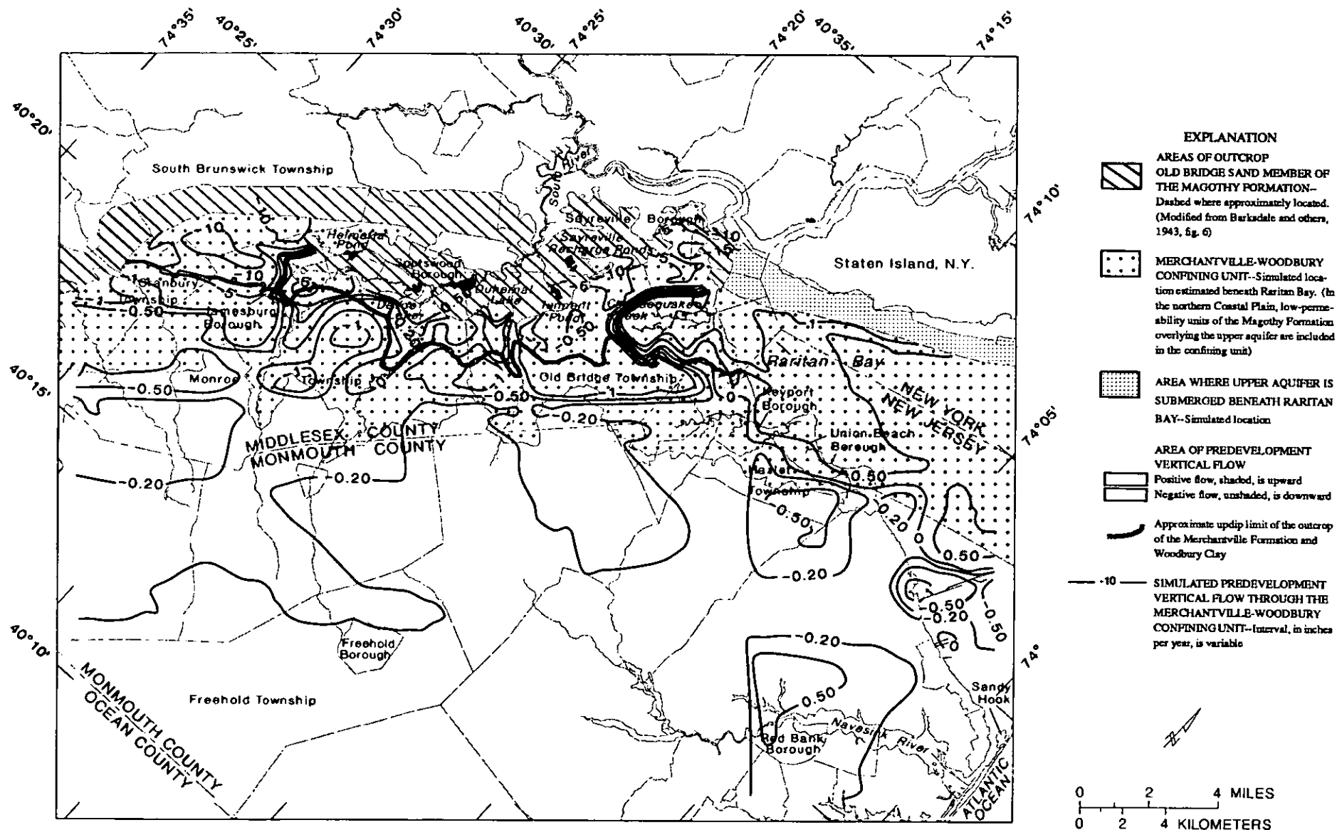
Figure 37.--Simulated predevelopment vertical flow through the Merchantville-Woodbury confining unit.
