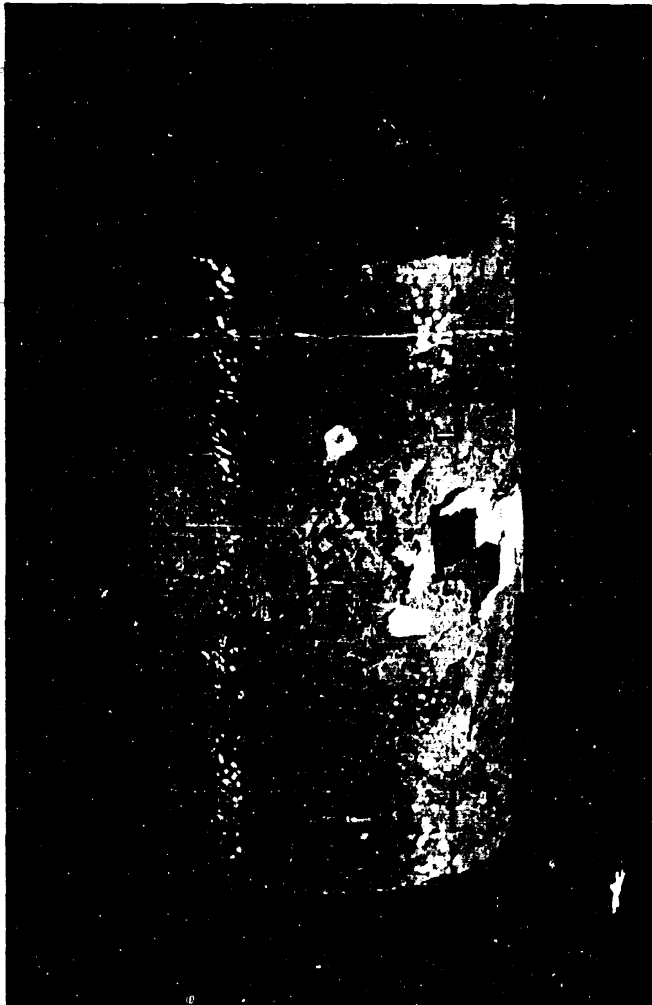
Figure 46. Typical surface spallation pattern of SIFCON specimens after drop testing. (Corresponds to "Minor Damage" in Table 2.)
