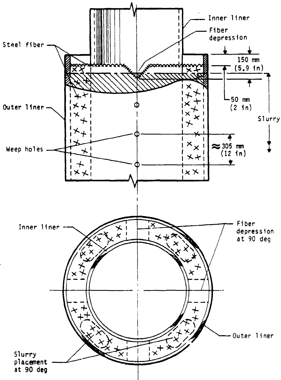
Figure 19. Fiber and slurry placement.
