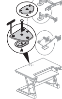
98-017 Grommet Mount
