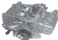
0702-416 CARBURETOR: HOLLEY 4160 454 PREMIUM / 502
