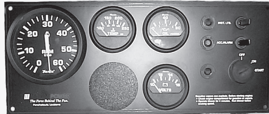
0945-000 PANEL: INSTRUMENT WITH GAUGES 0945-002* GAUGE: WATER TEMP 0945-003* GAUGE: VOLTMETER 0945-004* GAUGE: TACHOMETER 0945-005* GAUGE: OIL PRESSURE 0945-015 GAUGE: FUEL 0945-476 GAUGE: HOUR METER * Gauge Included with Panel
