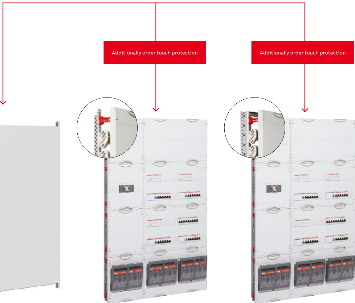
Mounting plate installation Expansion for the control technology with mounting plate, by removing the EDF adapter
