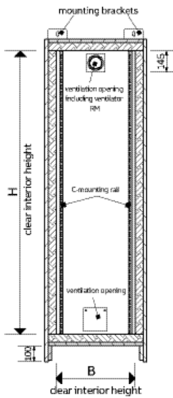
Internal view
