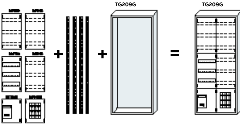
Modules (mounted) + EDF mounting frame + empty cabinet = wall-mounted distributor
