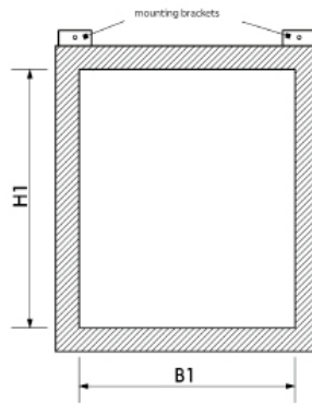
Internal view
