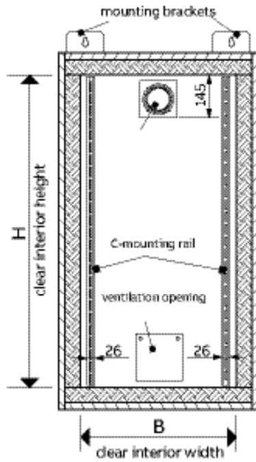
Internal view
