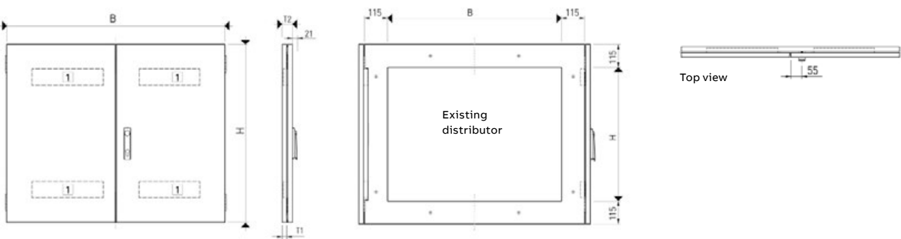
Front view
