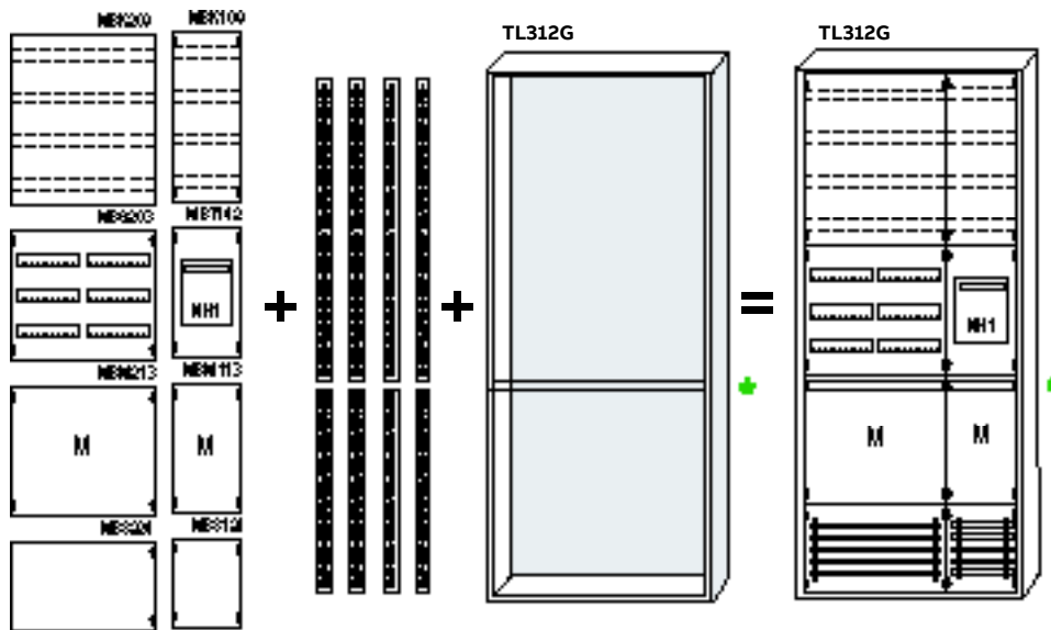
Modules (kit) + EDF mounting frame + empty cabinet = standalone distributor
