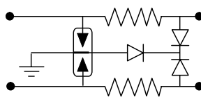
OVR TC / xx V / 200 FR in series
